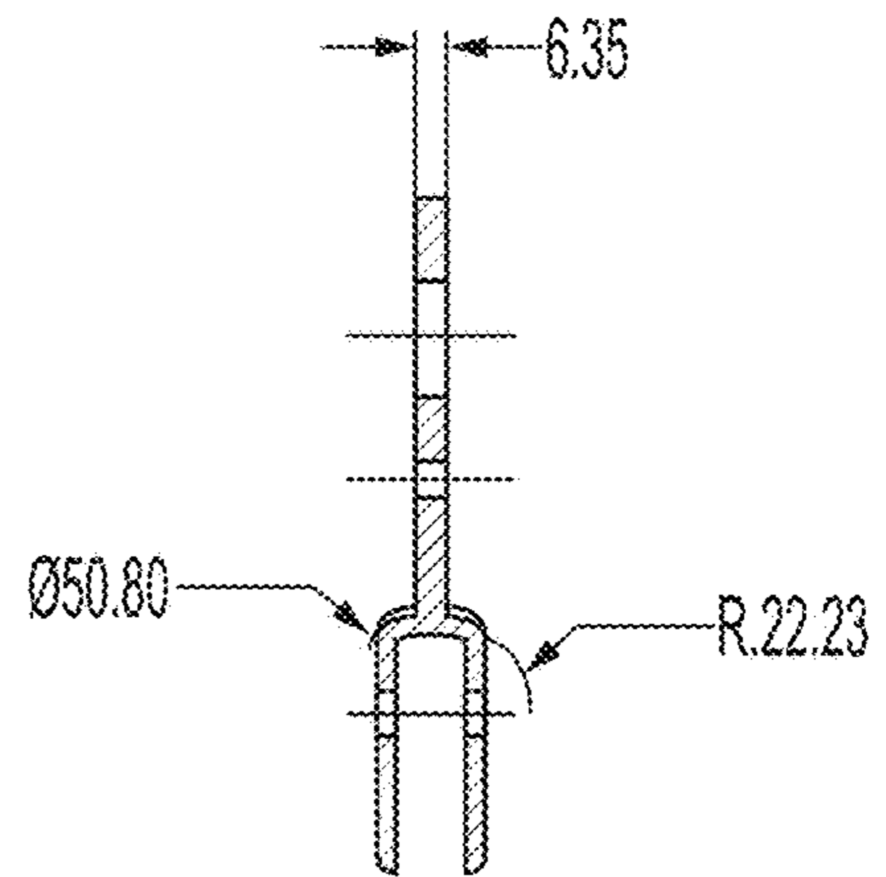
SECTION C-C
