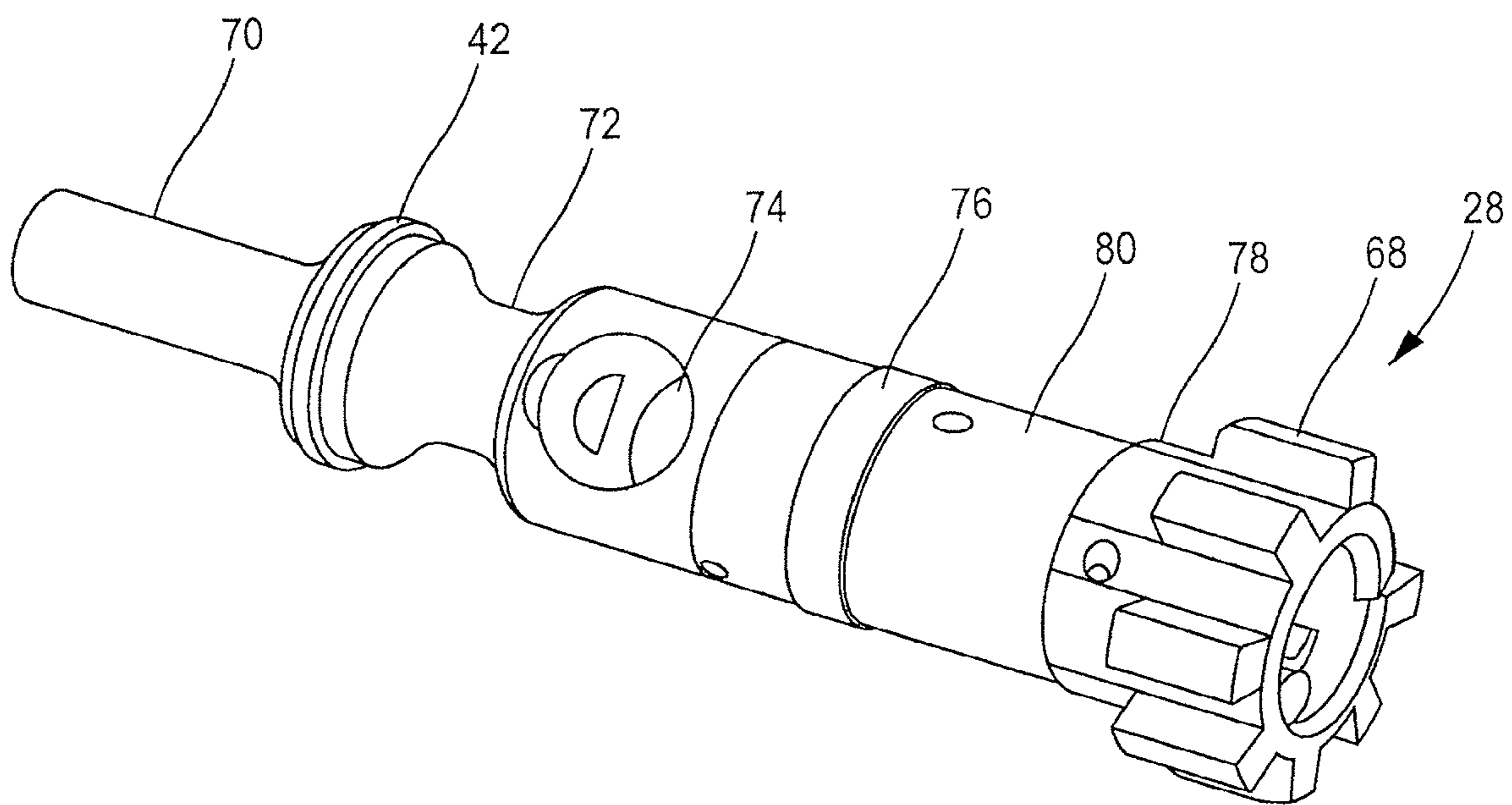
Fig. 16 PRIOR ART
