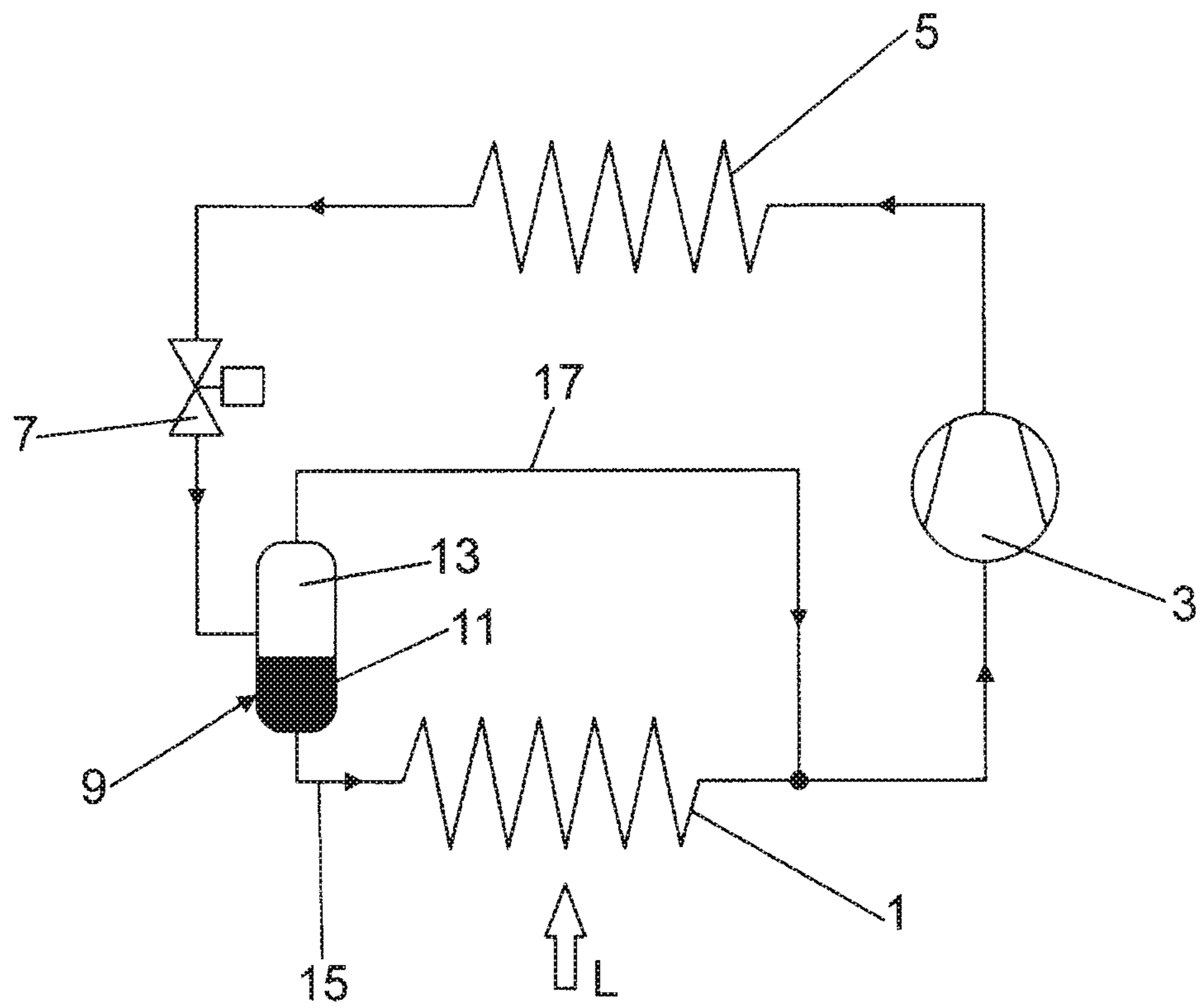
Fig. 1 (prior art)
