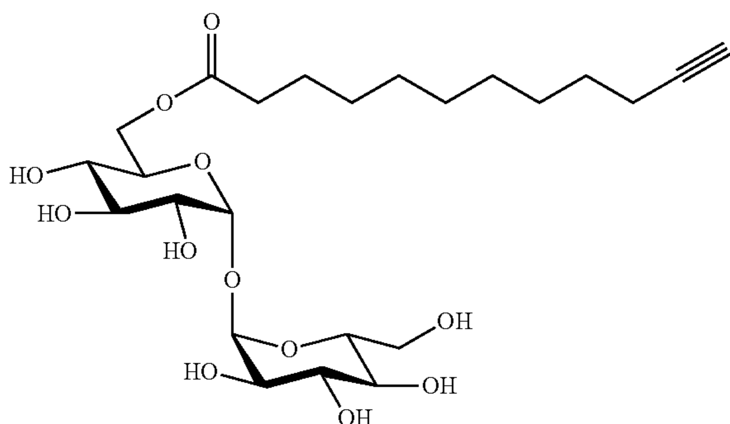
6-O-(10-undecynoyl)-α,α-D-trehalose (O-AlkTMM-C11)
