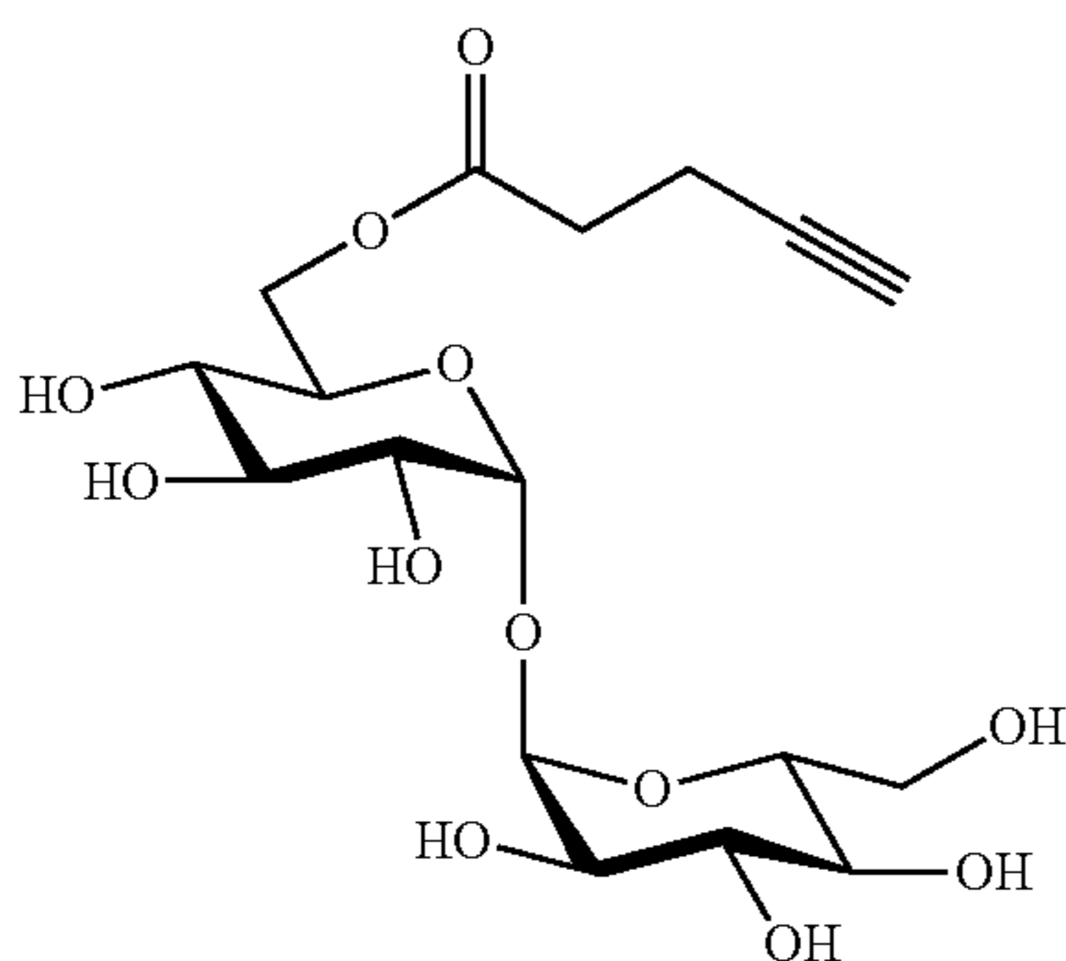
6-O-(4-pentynoyl)-α,α-D-trehalose (O-AlkTMM-C5)
