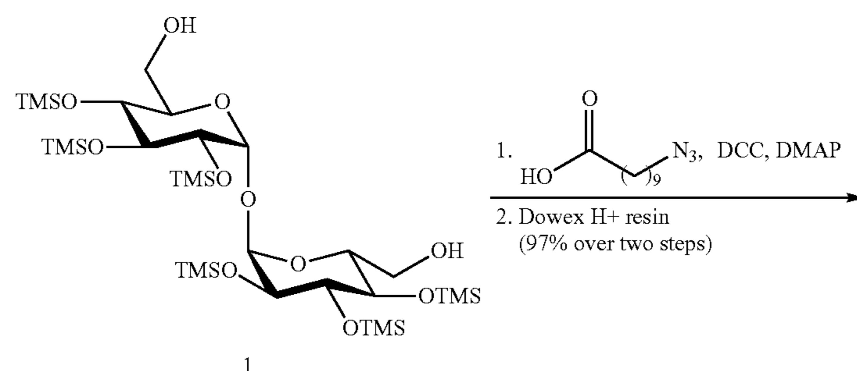
Scheme 4:
