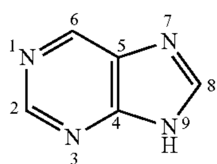
Purine
