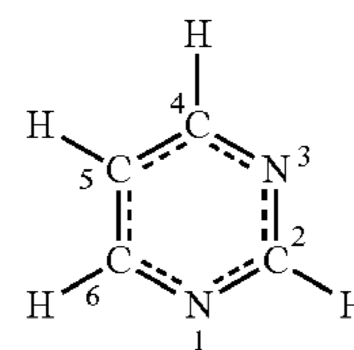
Pyrimidine
