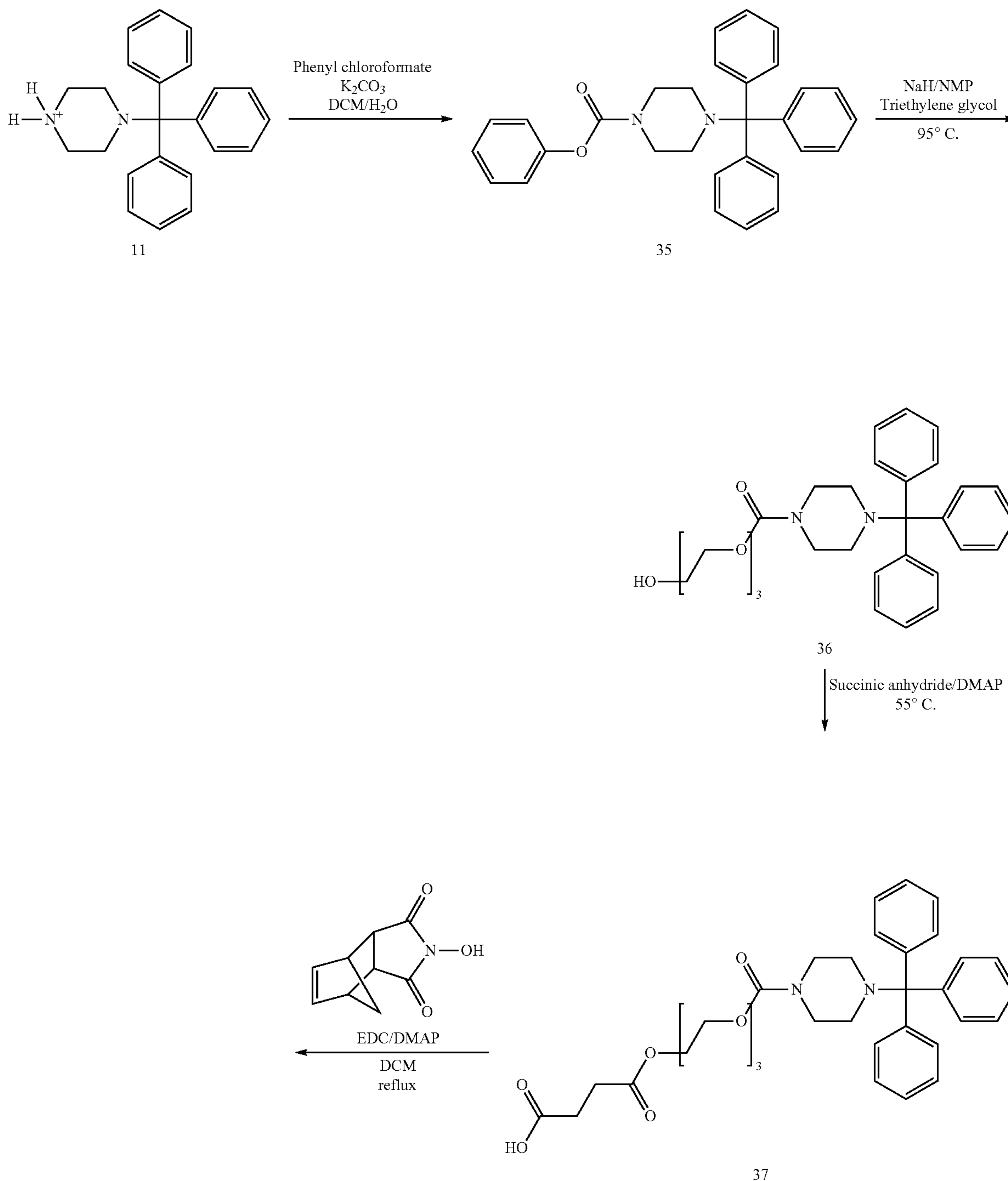
Scheme 2: Preparation of Activated Tail Acid
