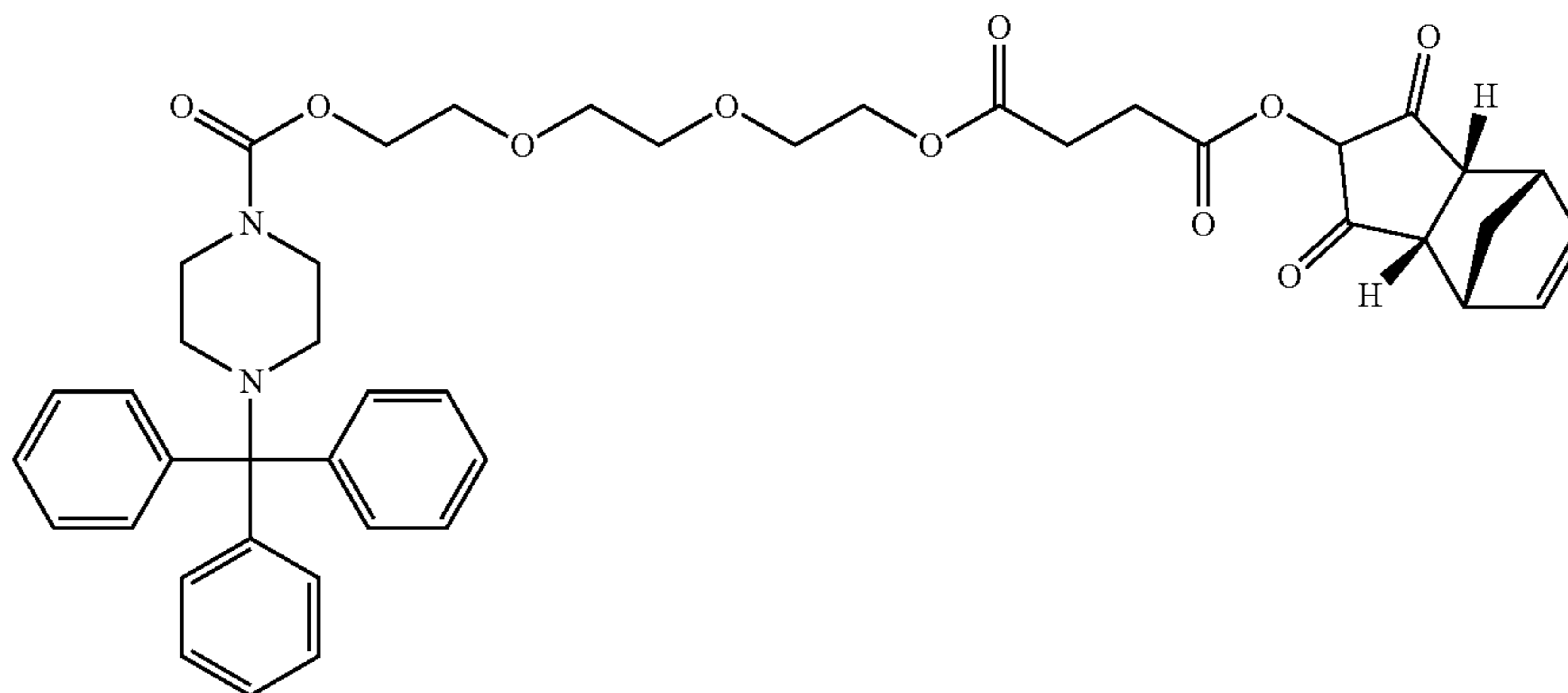
Chemical Structures of Starting Materials: A. Activated EG3 Tail
