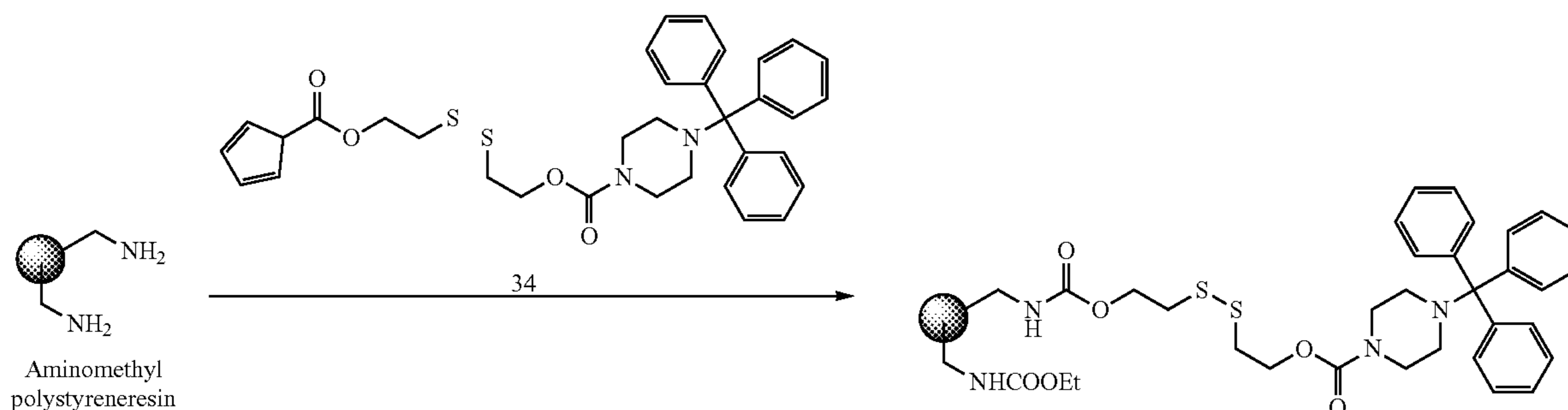
Scheme 3: Preparation of the Solid Support for Synthesis of Morpholino Oligomers
