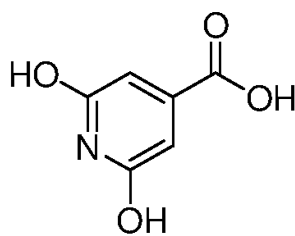
citrazinic acid
