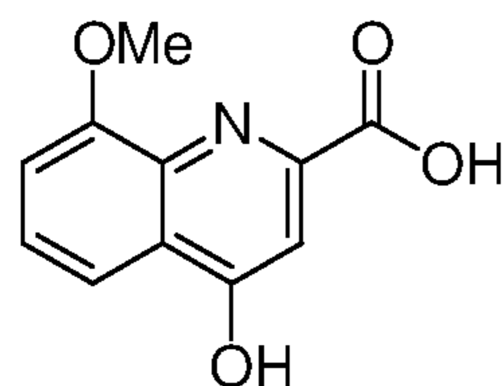
8-methoxykynurenic acid
