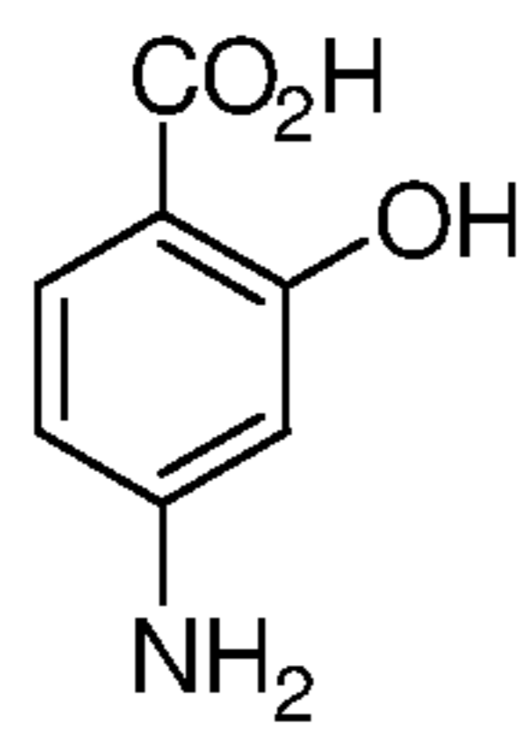
4-aminosalicylic acid
