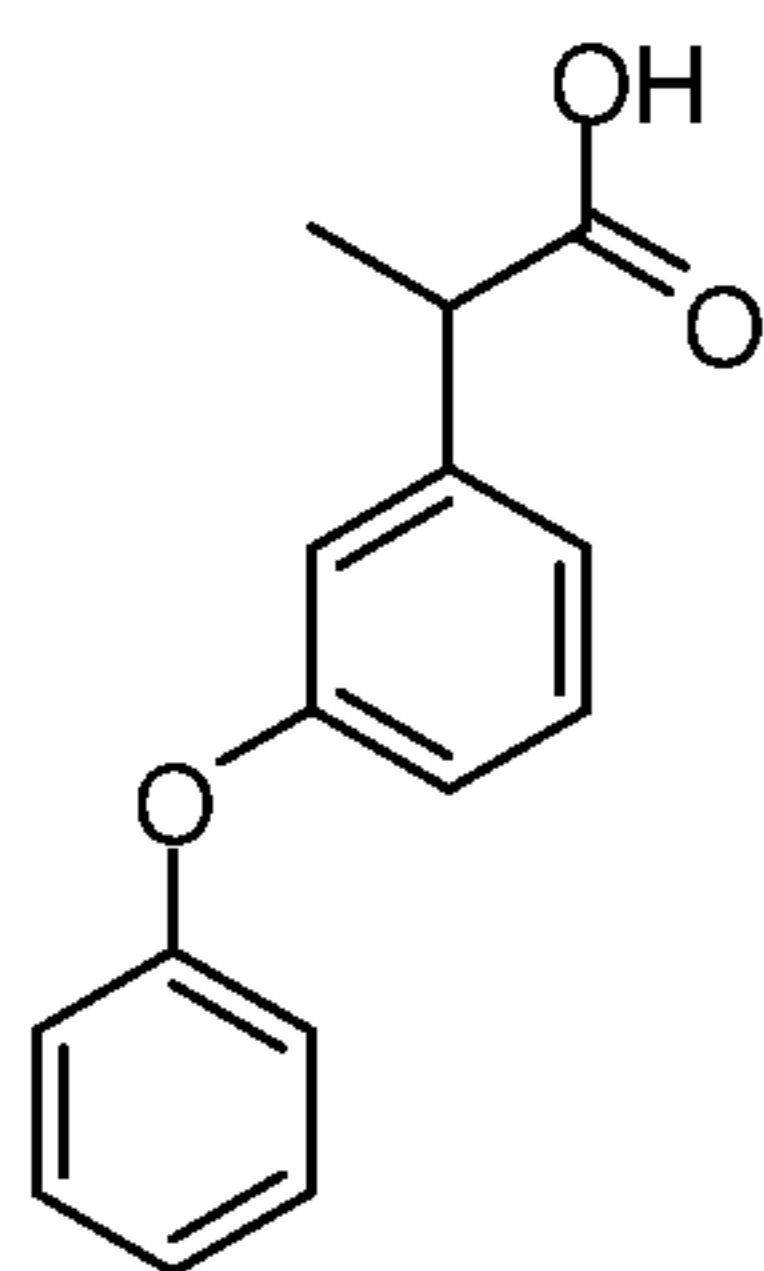
Fenoprofen
