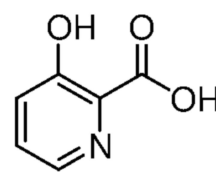
3-hydroxypicolinic acid
