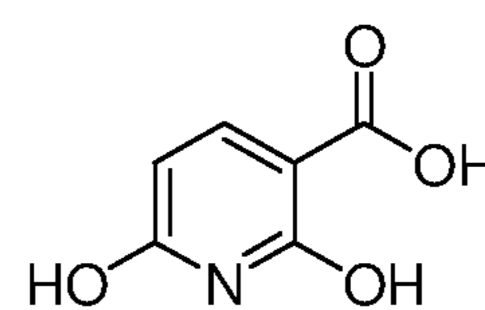
2,6-dihydroxynicotinic acid
