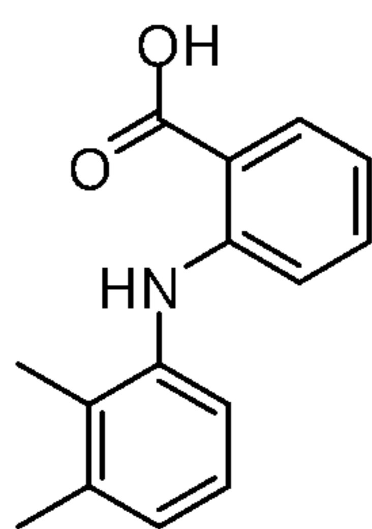
Mefenamic acid
