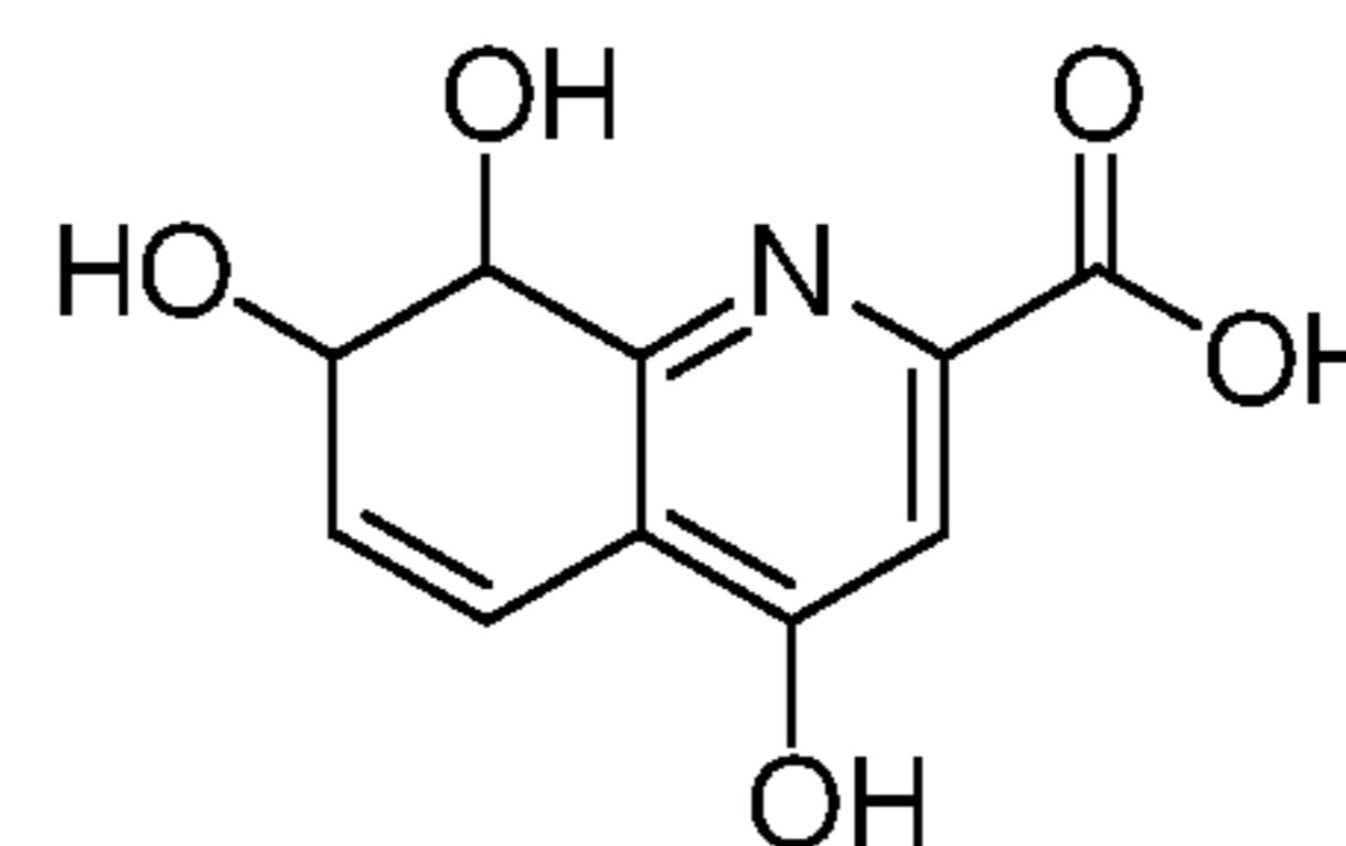
7,8-dihydro-7,8-dihydroxykynurenic acid
