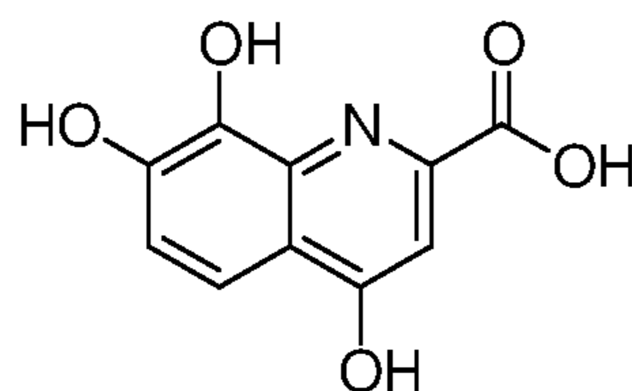
7,8-dihydroxykynurenic acid
