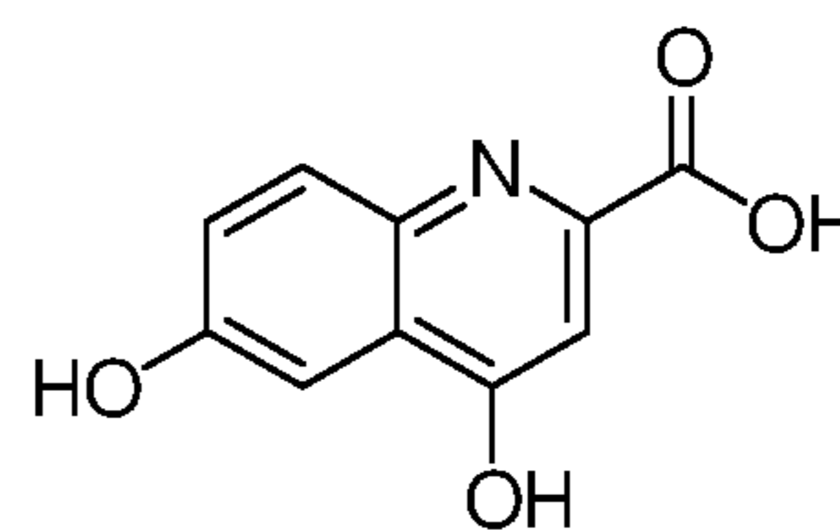
6-hydroxykynurenic acid
