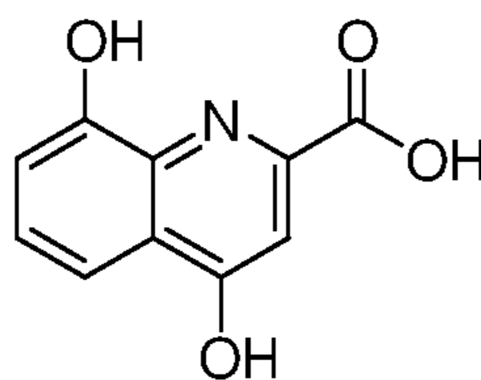
xanthurenic acid
