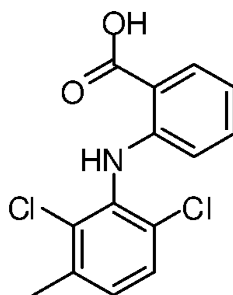
Meclofenamic acid
