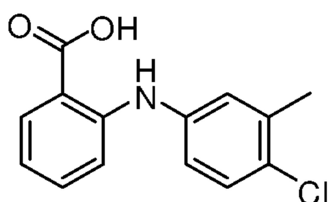
Tolfenamic acid
