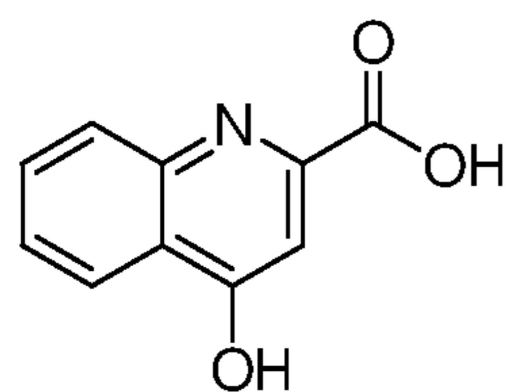
kynurenic acid
