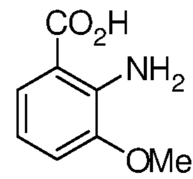
3-methoxyanthranilic acid
