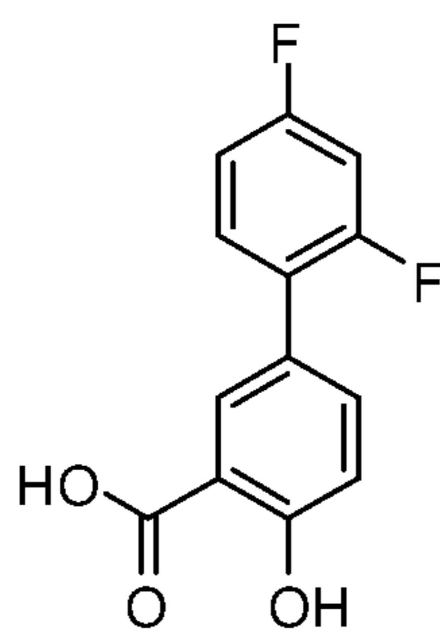
Diflusal
