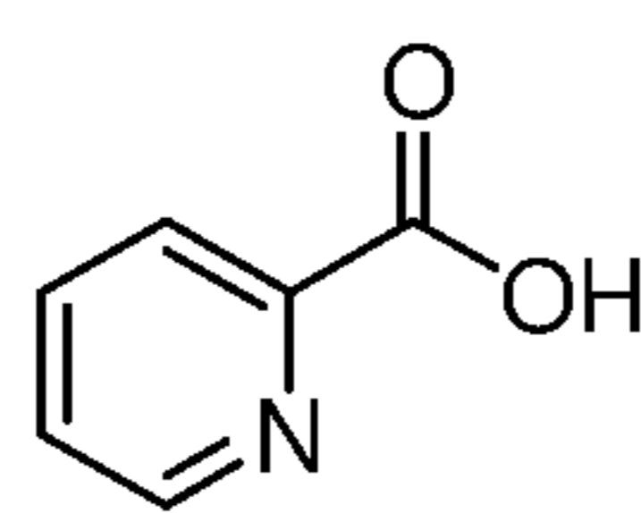
picolinic acid
