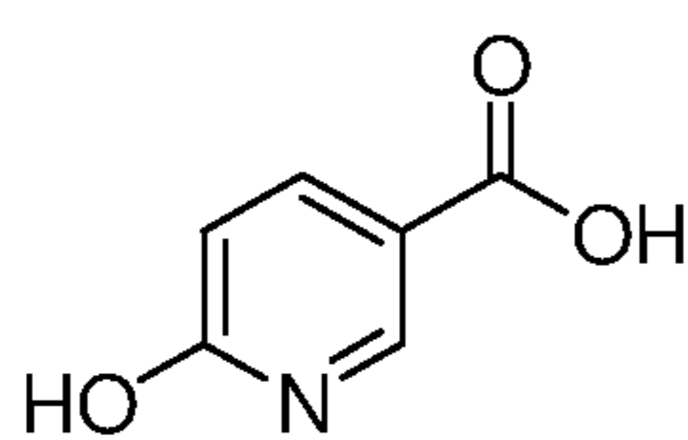
6-hydroxynicotinic acid
