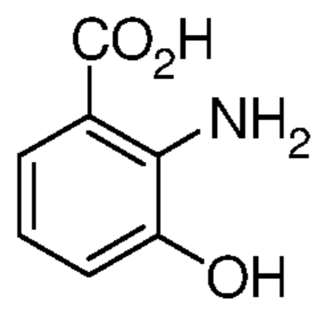
3-hydroxyanthranilic acid
