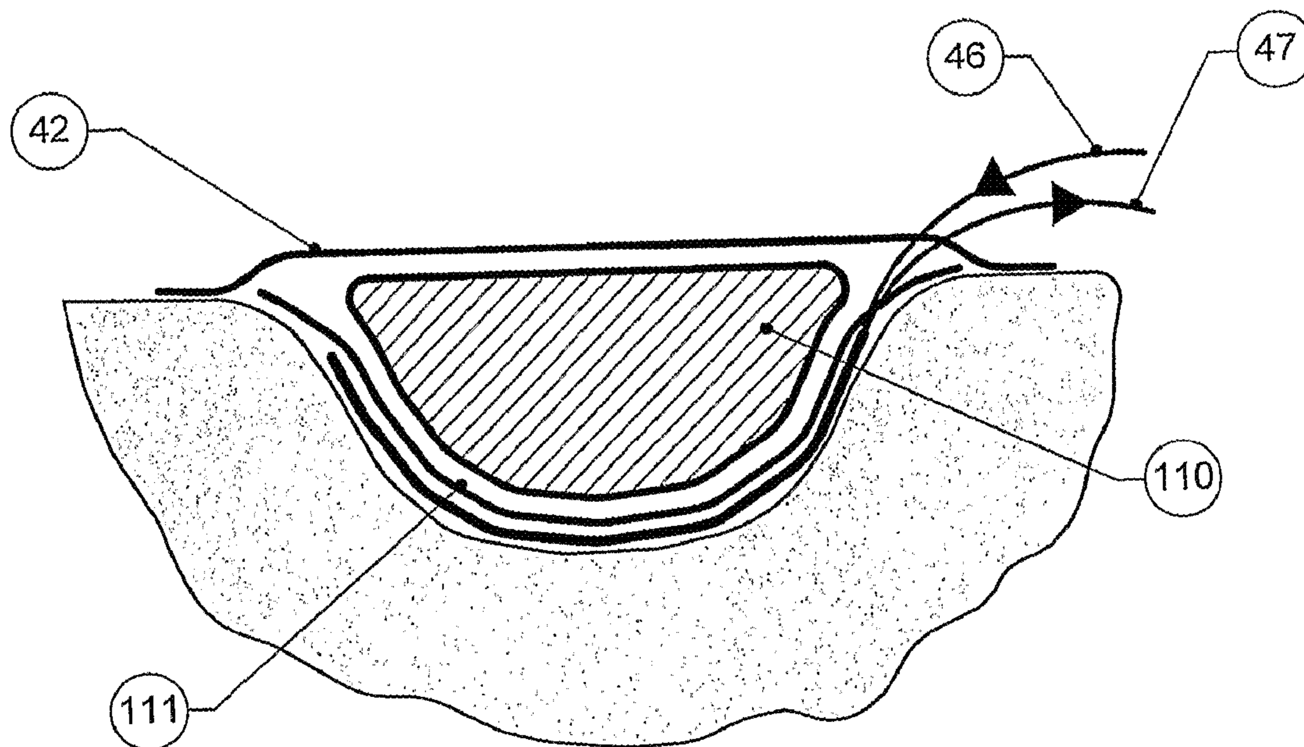
Section Through X-X
