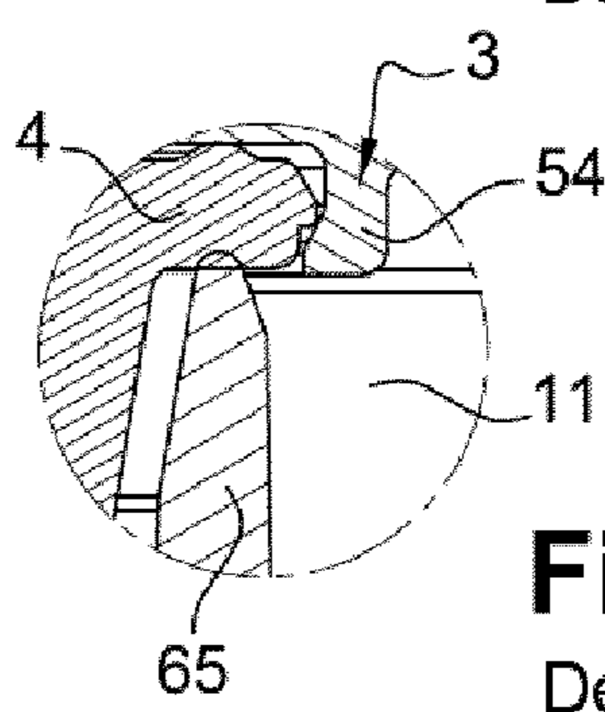
Fig. 6 Detail C
