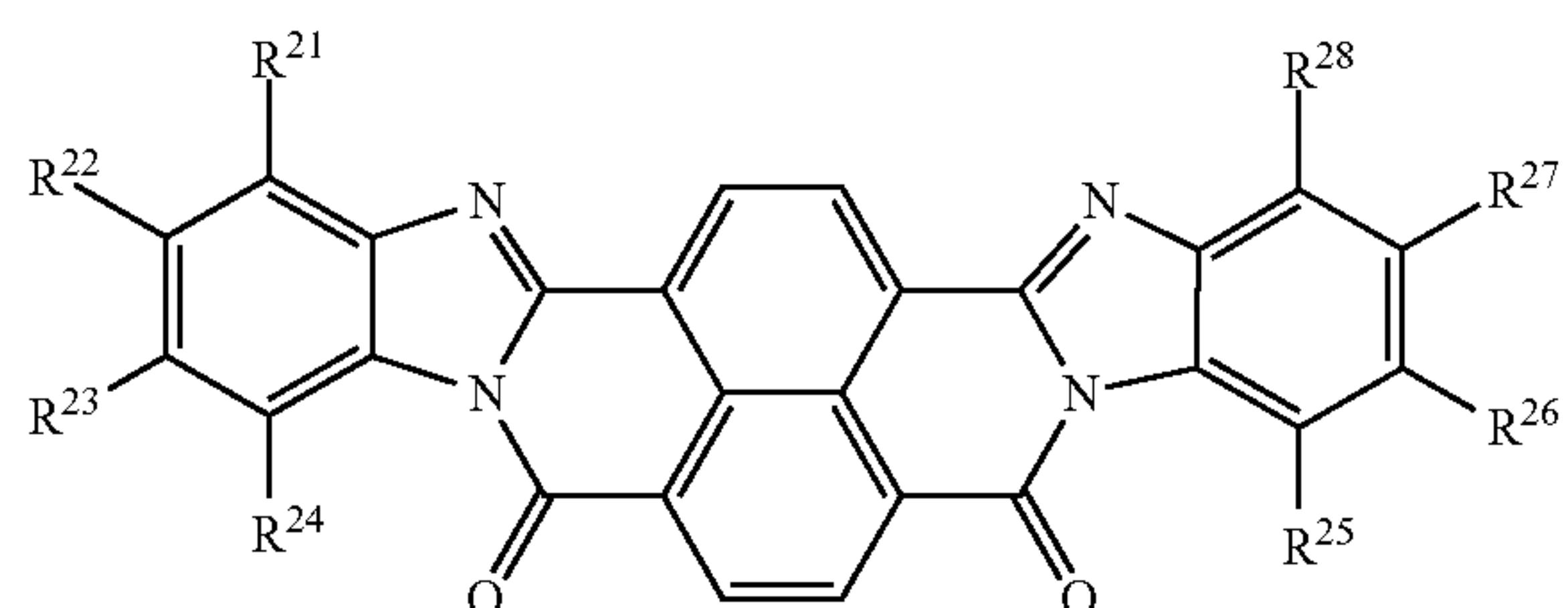
Formula (2)
