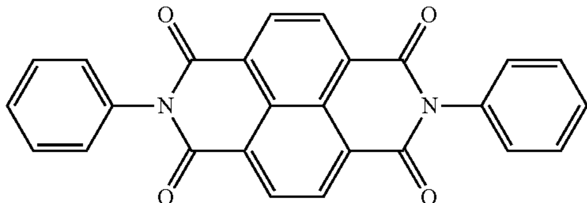
Imide compound (17-1)
