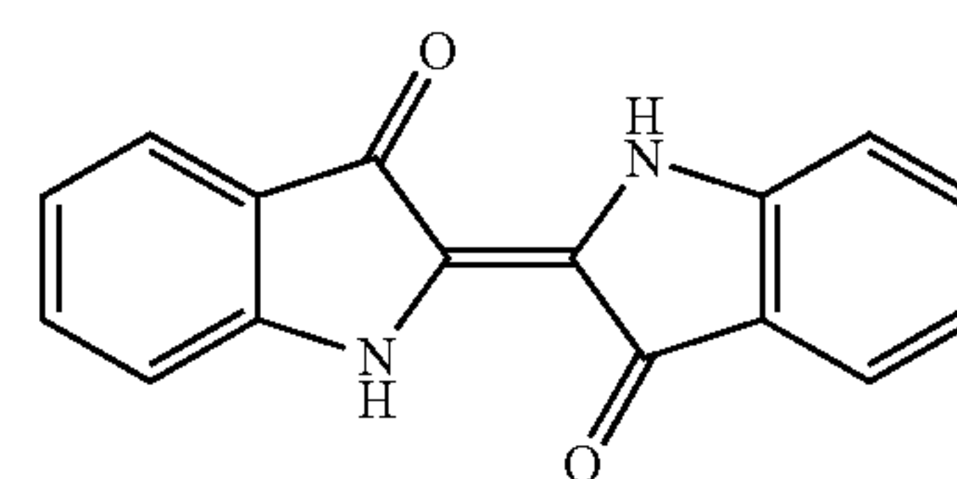
Example 17B
