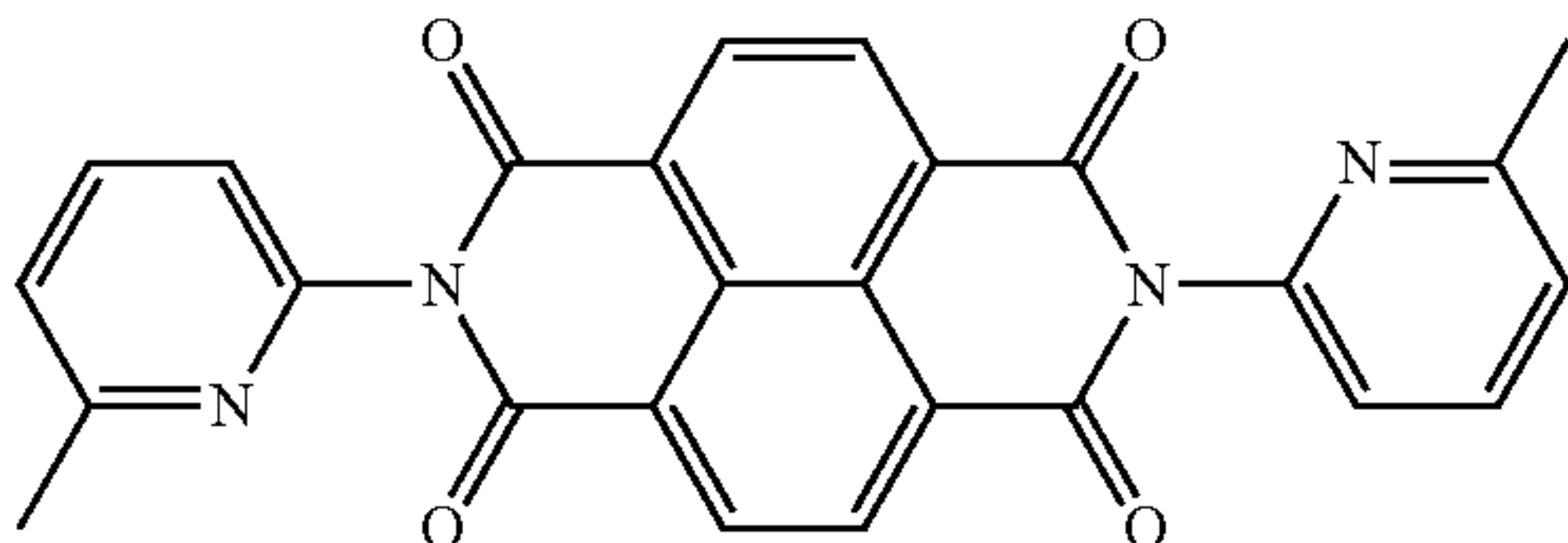
Imide compound (17-2)
