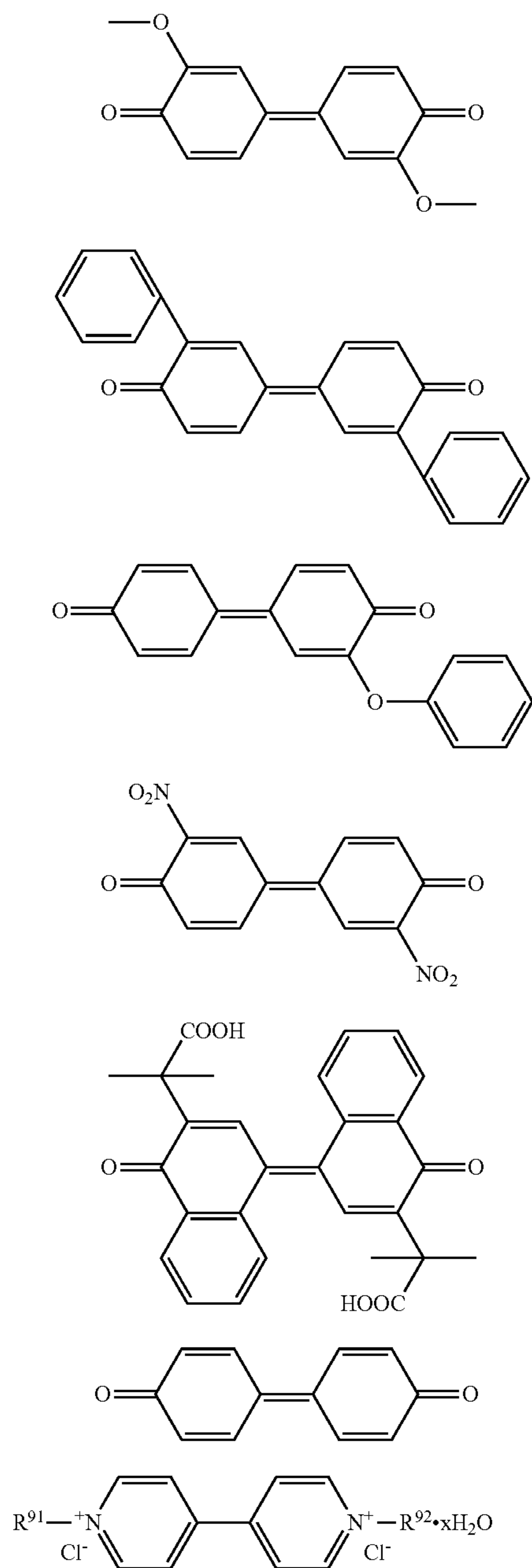
Formula (9)
