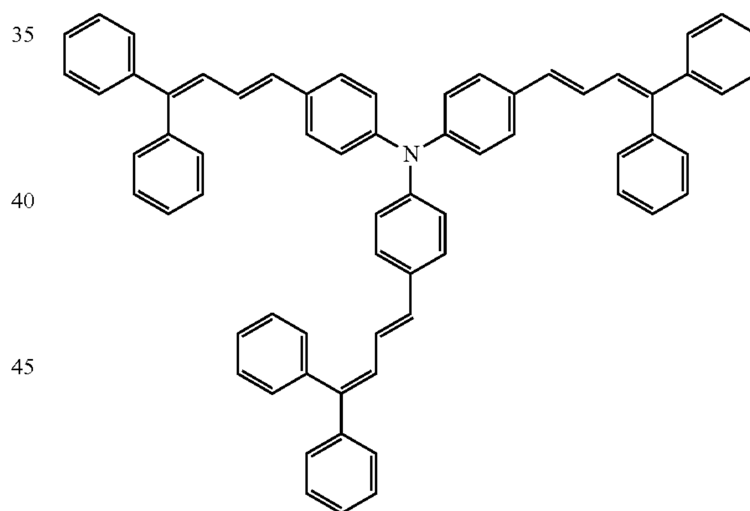
Formula (A)
