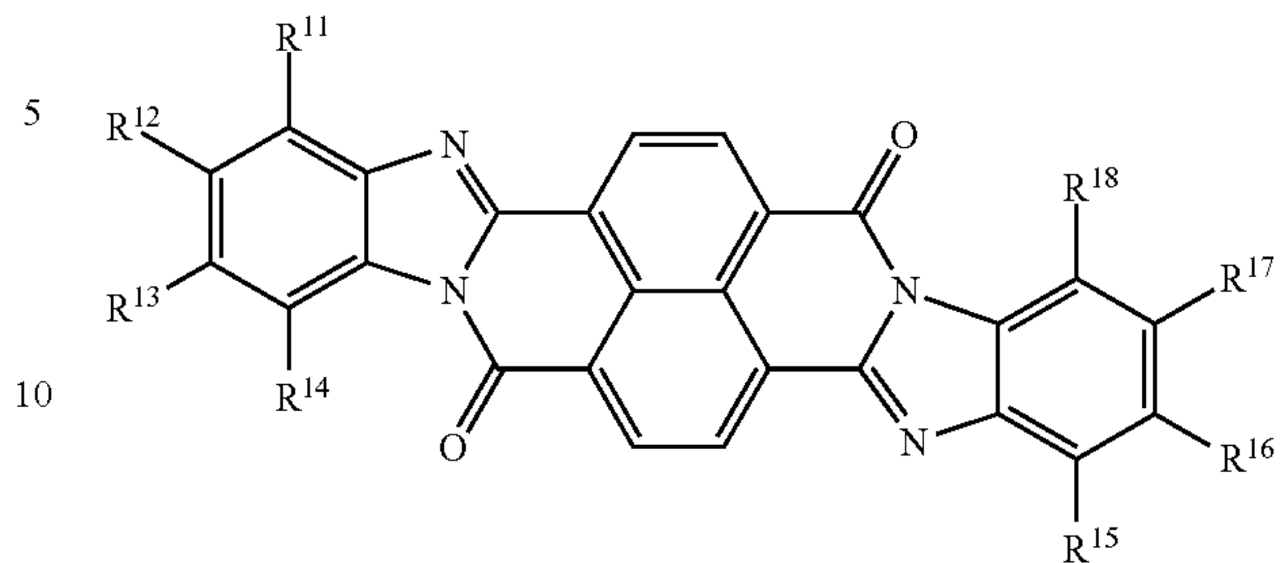
Formula (2)
