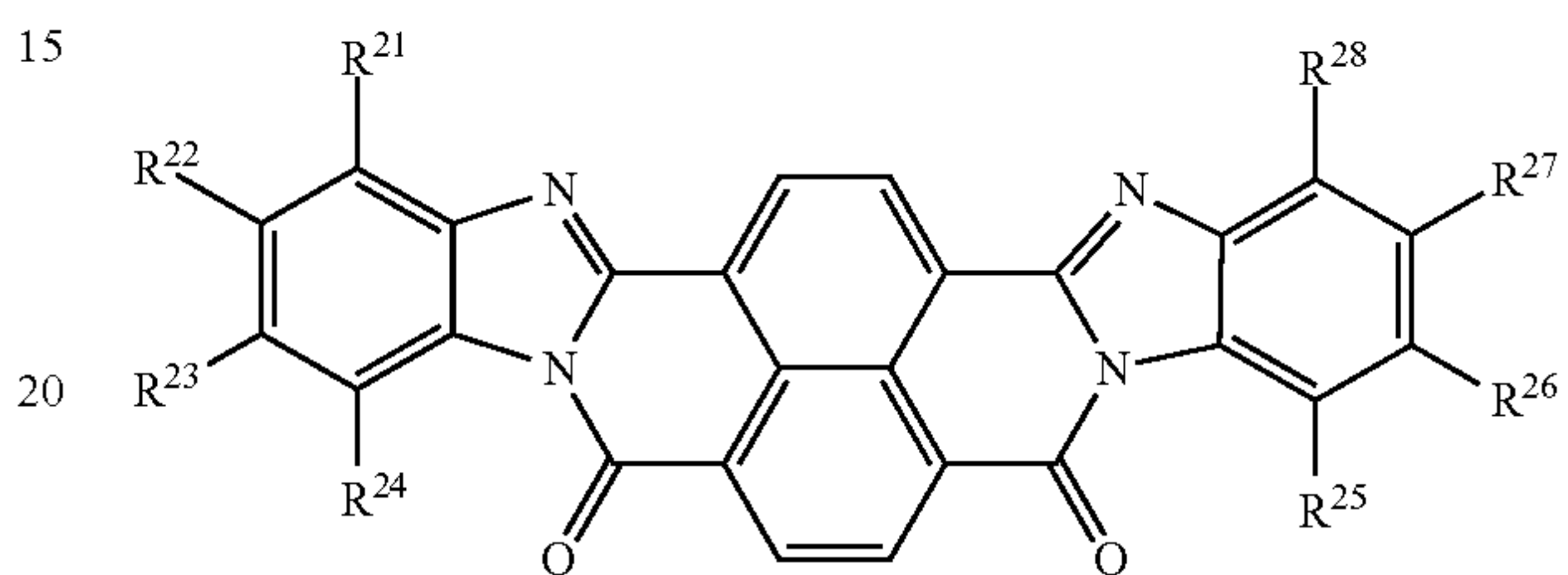
Formula (2)
