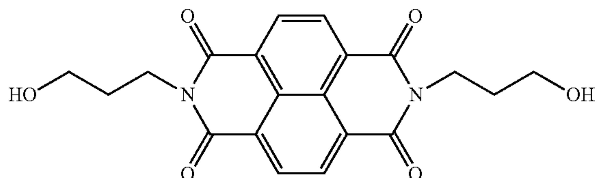
Imide compound (17-3)
