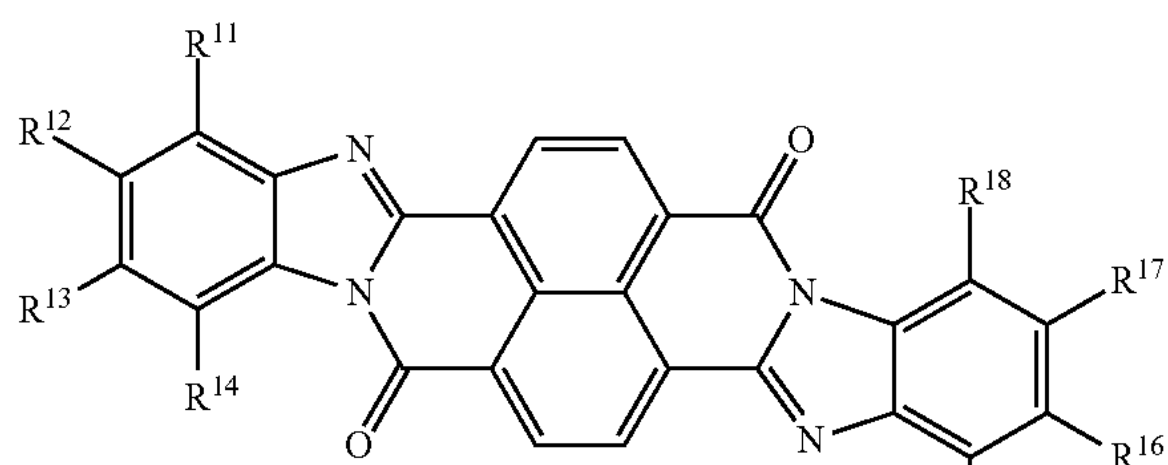
Formula (1)
