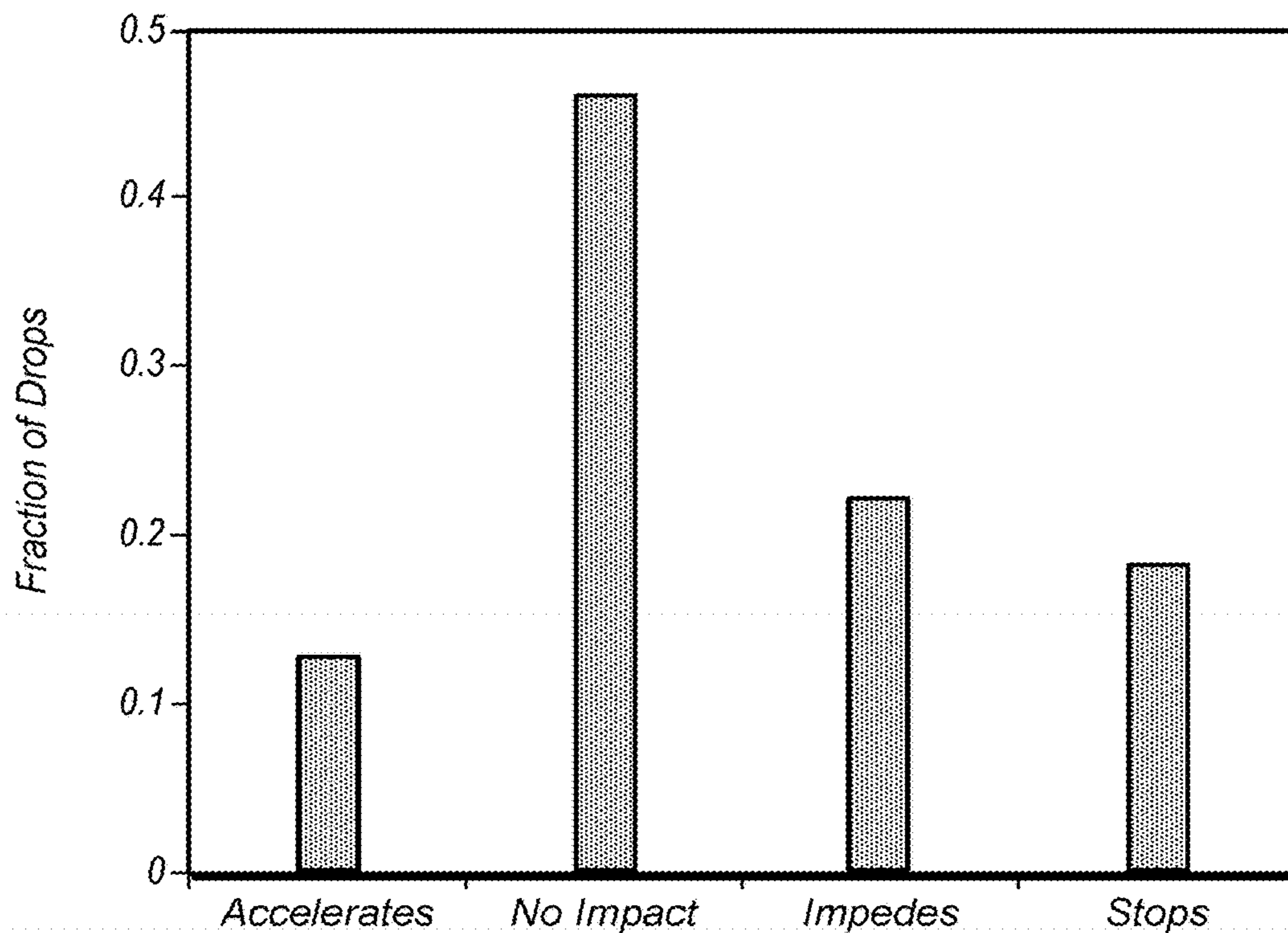
Impact of Drop on Growth of Largest Fracture
