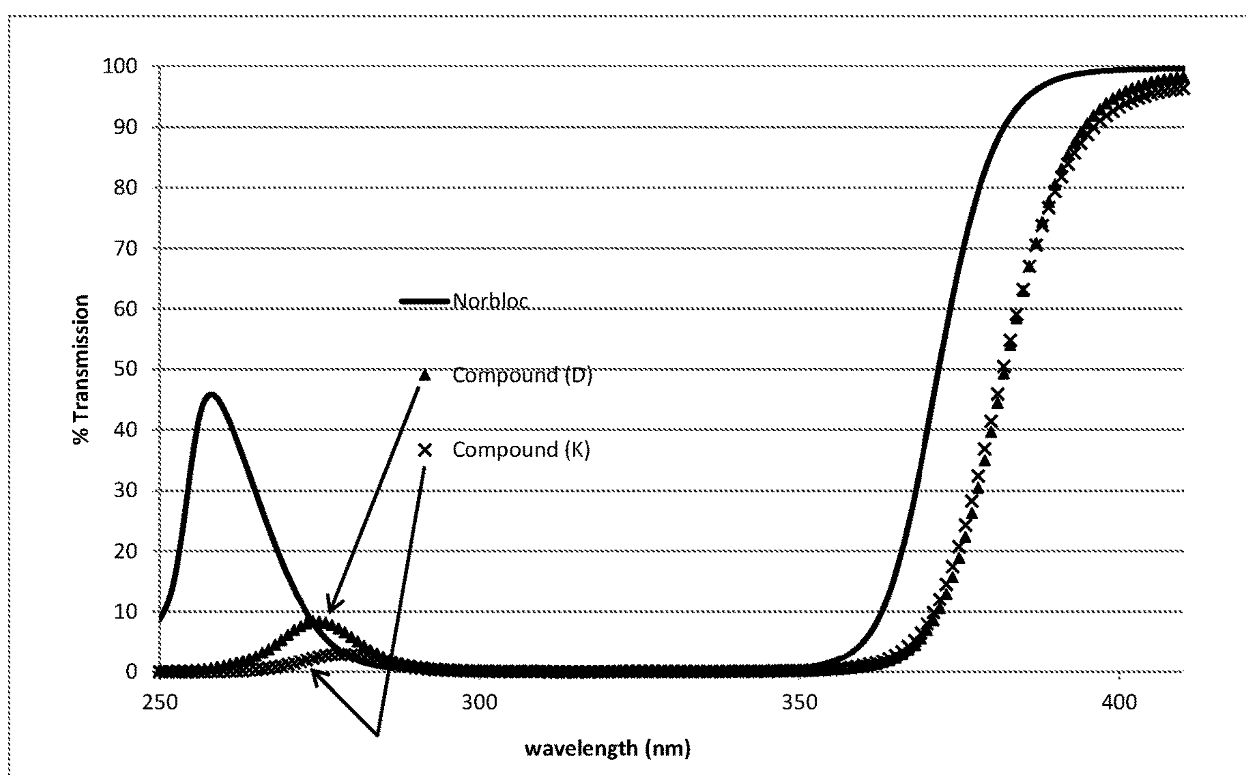
FIG. 1 - Transmission Spectra of 0.2 mM solutions of Norbloc, Compound (D), and Compound (K) in methanol
