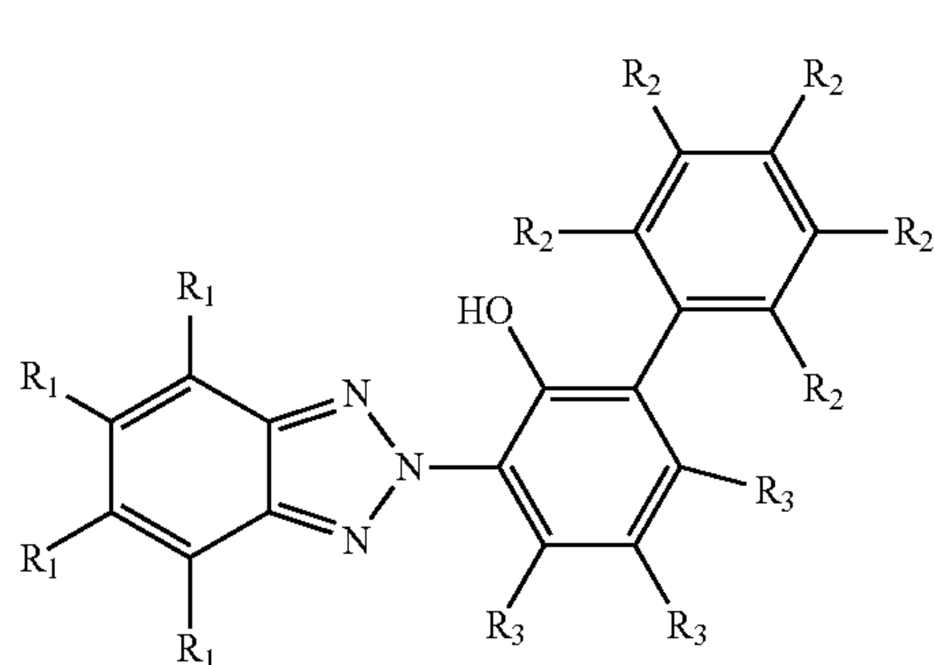
Formula I
