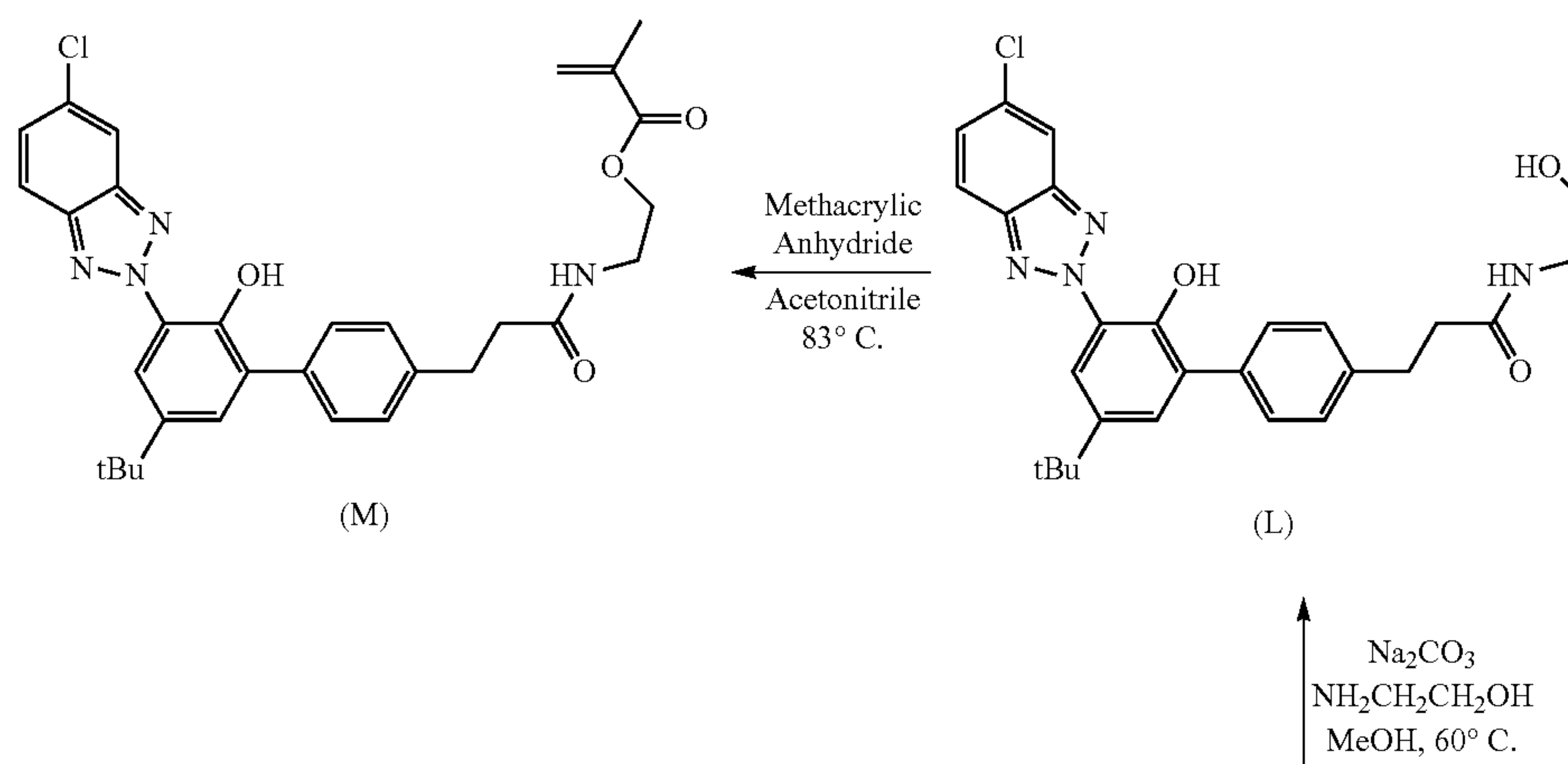
Scheme 3
