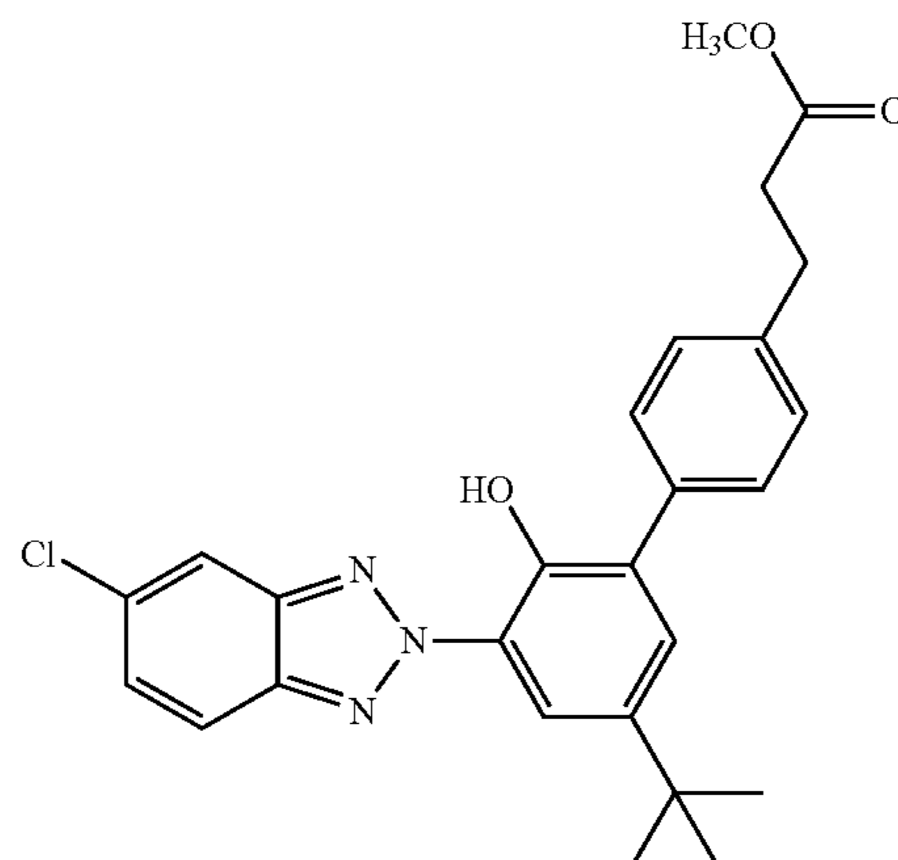
methyl 3-(5'-(tert-butyl)-3'-(5-chloro-2H-benzo[d][1,2,3]triazol-2-yl)-2'-hydroxy-[1,1'-biphenyl]-4-yl)propanoate
