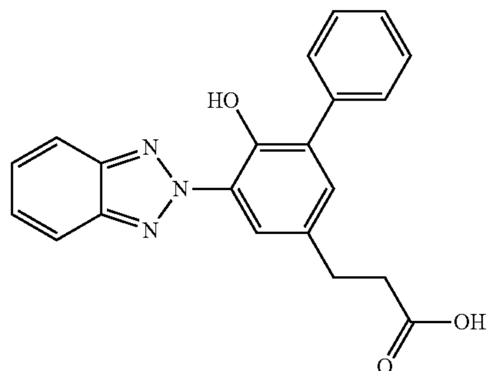
3-(5-(2H-benzo[d][1,2,3]triazol-2-yl)-6-hydroxy-[1,1'-biphenyl]-3-yl)propanoic acid
