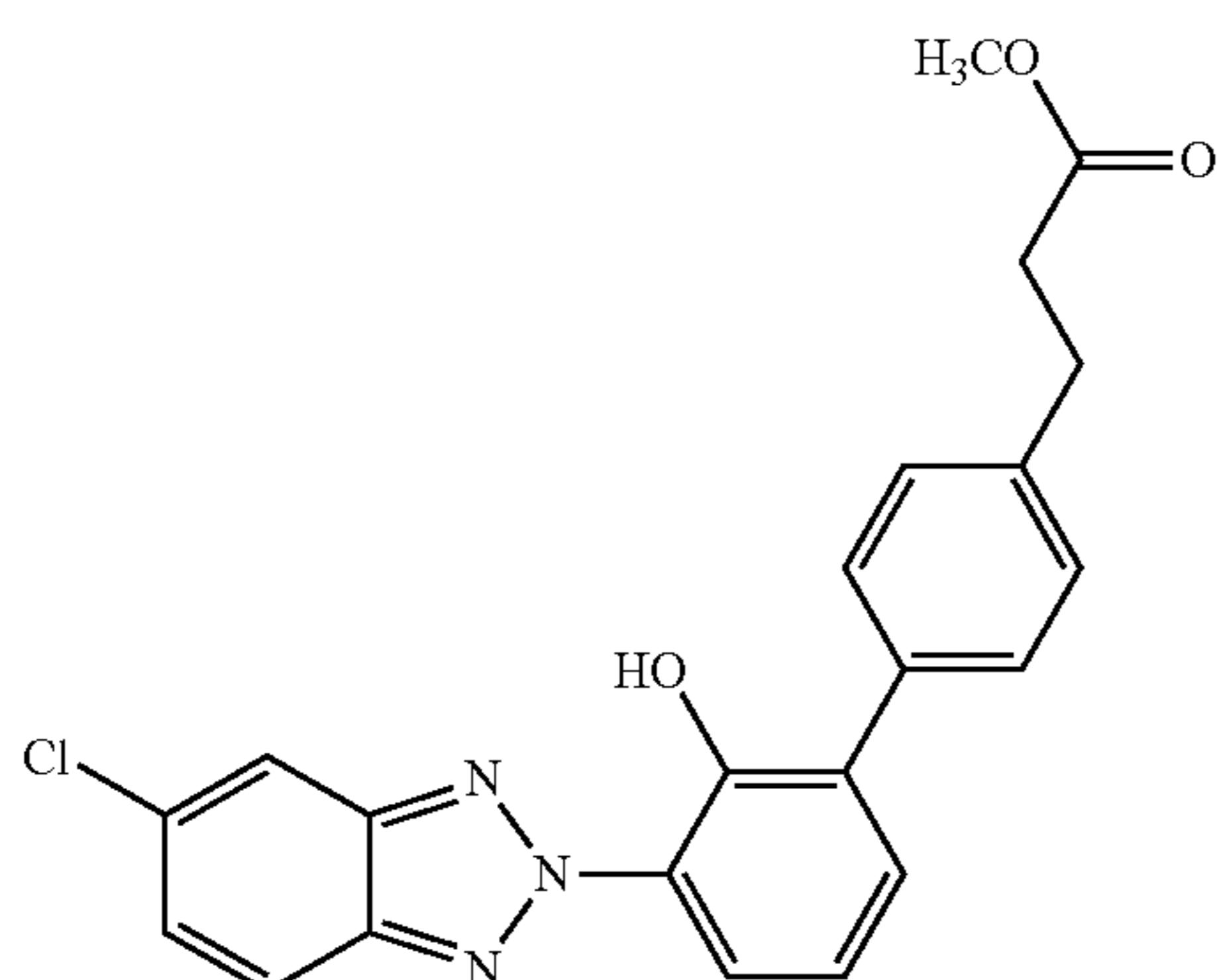
methyl 3-(3'-(5-chloro-2H-benzo[d][1,2,3]triazol-2-yl)-2'-hydroxy-[1,1'-biphenyl]-4-yl)propanoate
