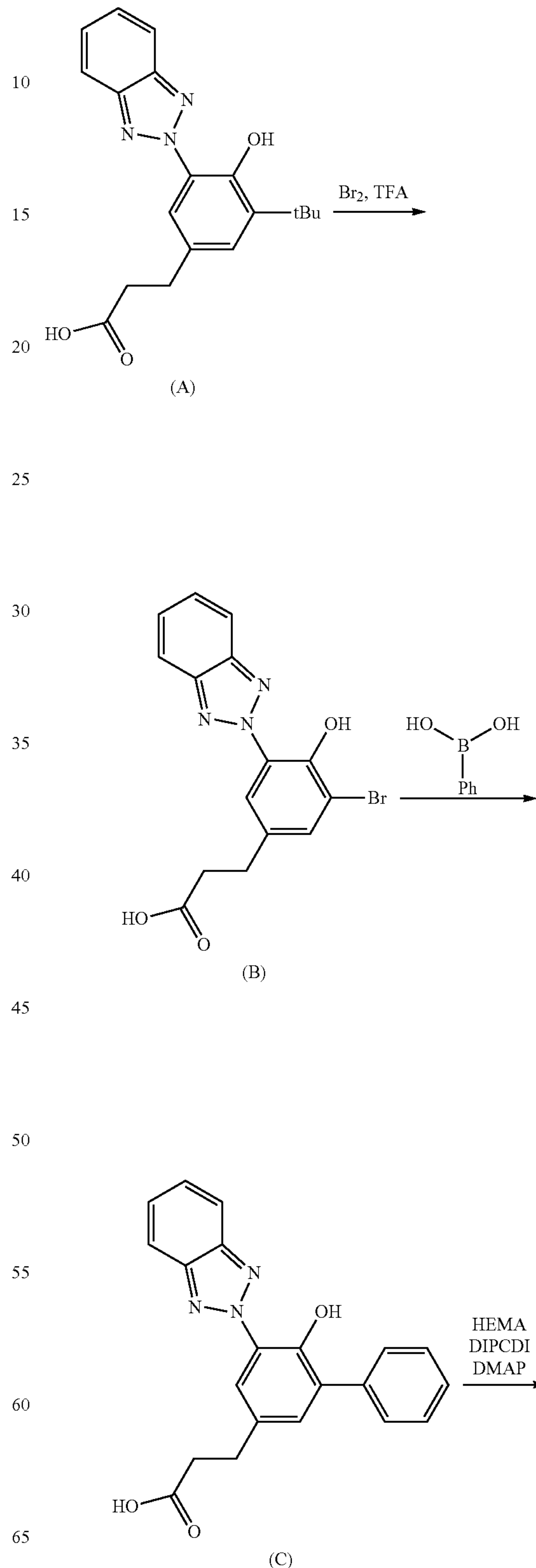
Scheme 2
