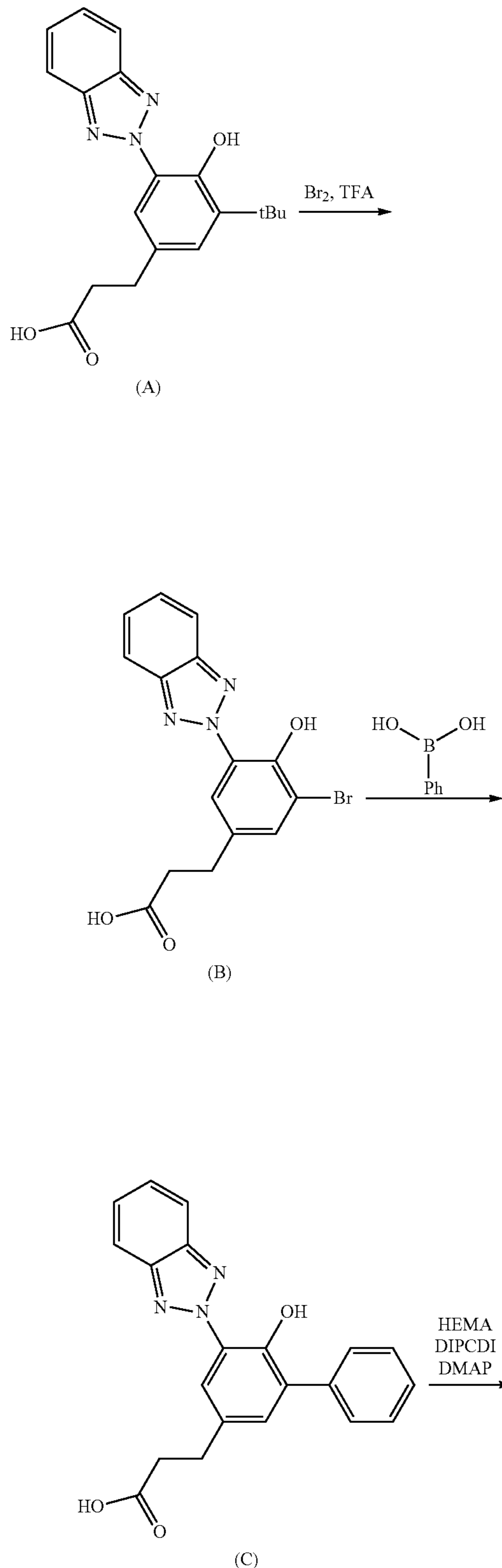
Scheme 2
