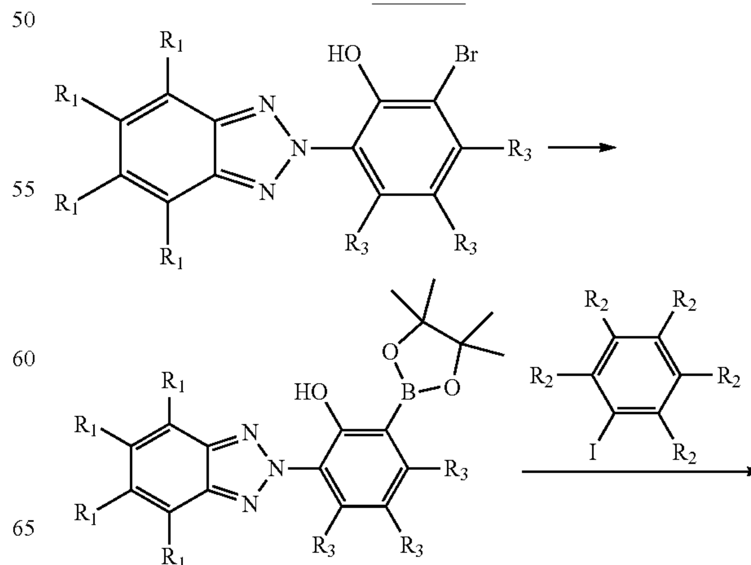
Scheme 1
