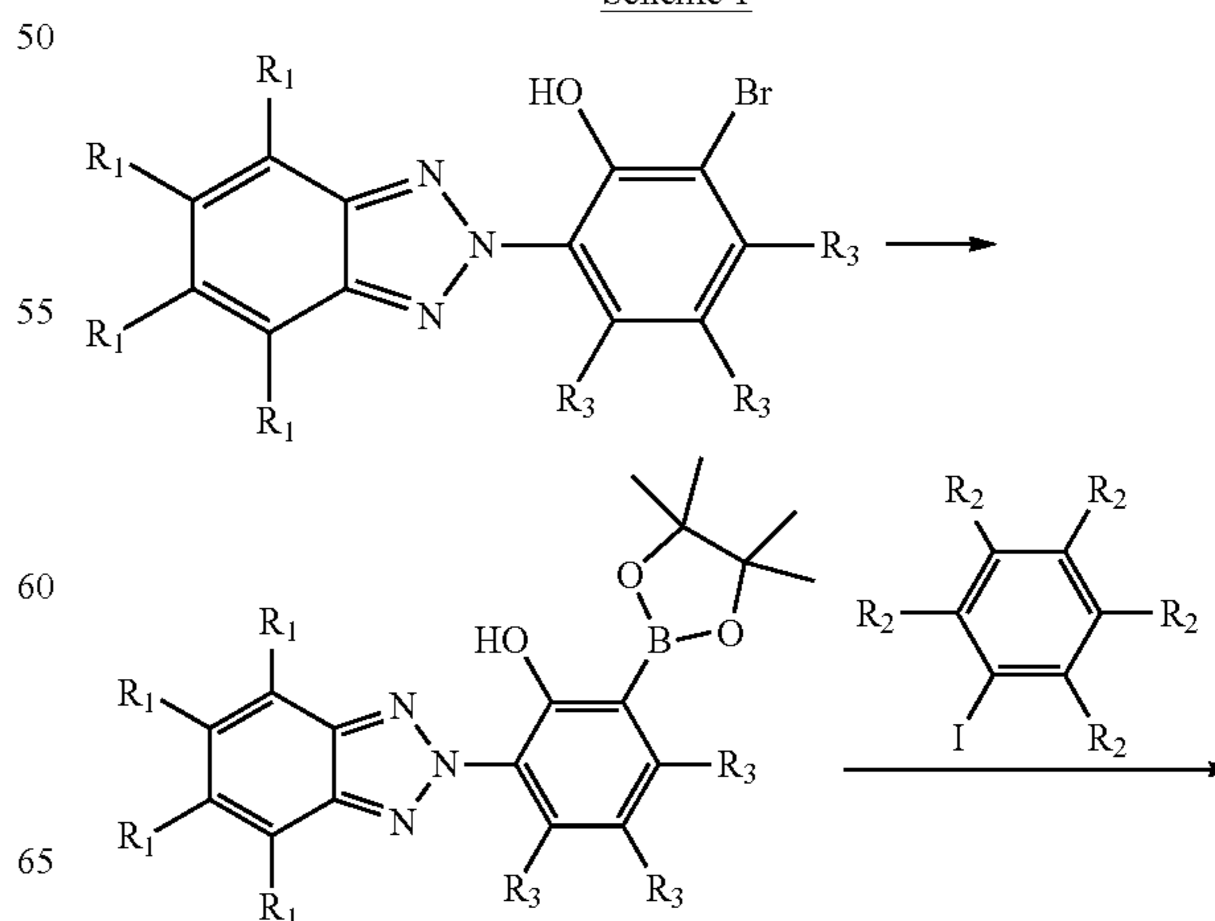
Scheme 1
