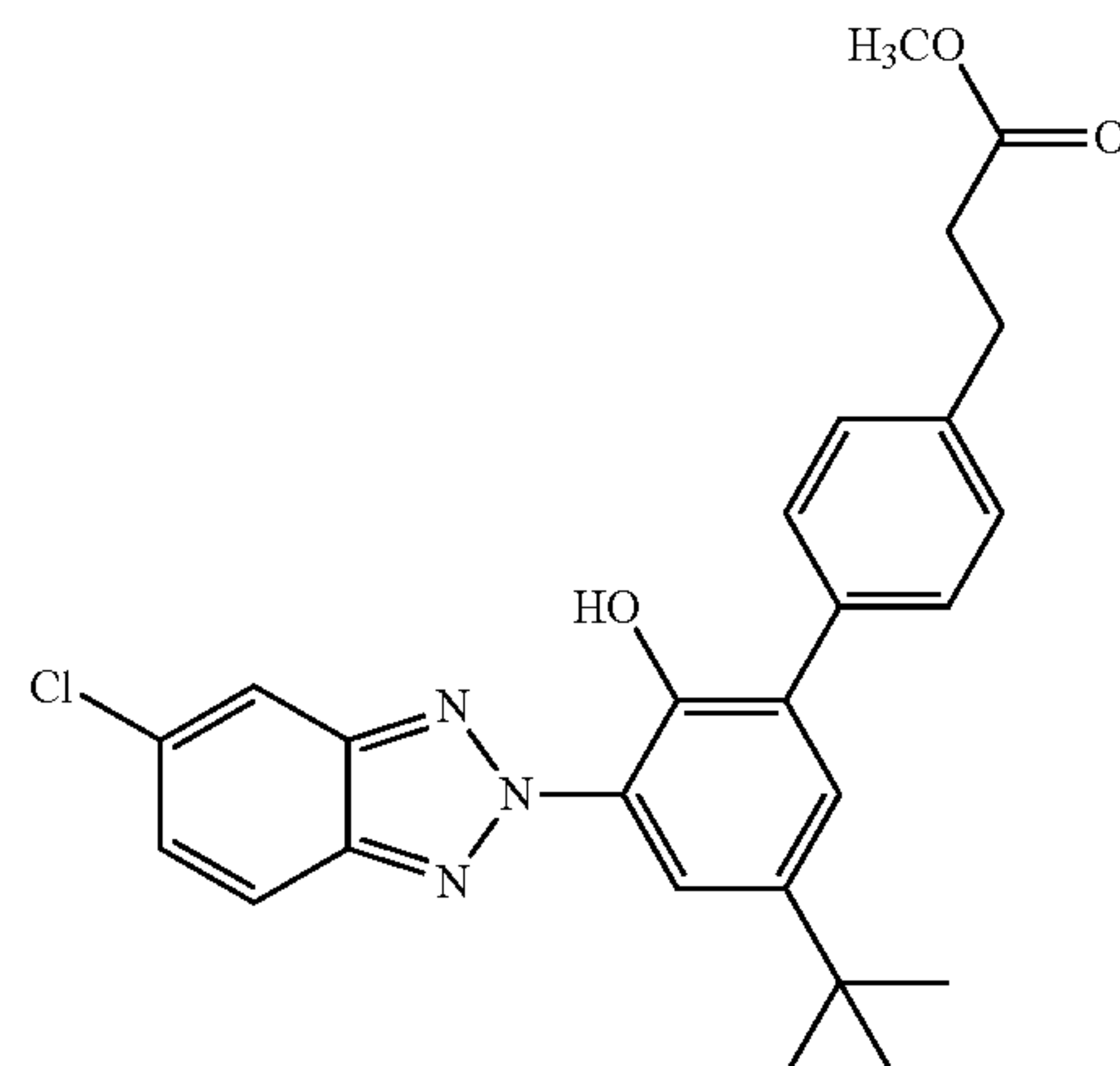
methyl 3-(5'-(tert-butyl)-3'-(5-chloro-2H-benzo[d][1,2,3]triazol-2-yl)-2'-hydroxy-[1,1'-biphenyl]-4-yl)propanoate
