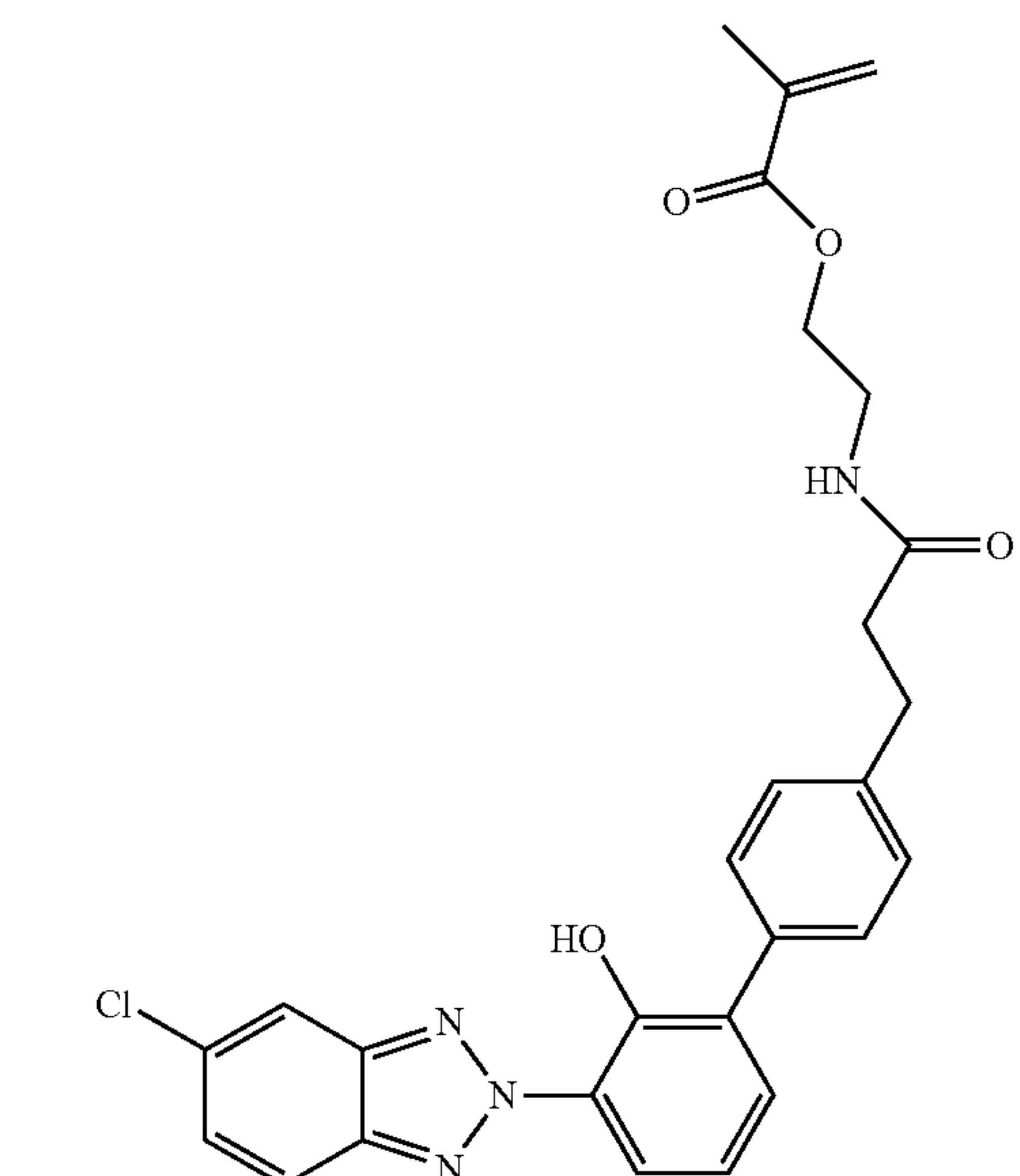
2-(3-(3'-(5-chloro-2H-benzo[d][1,2,3]triazol-2-yl)-2'-hydroxy-[1,1'-biphenyl]-4-yl)propanamido)ethyl methacrylate (Compound K)
