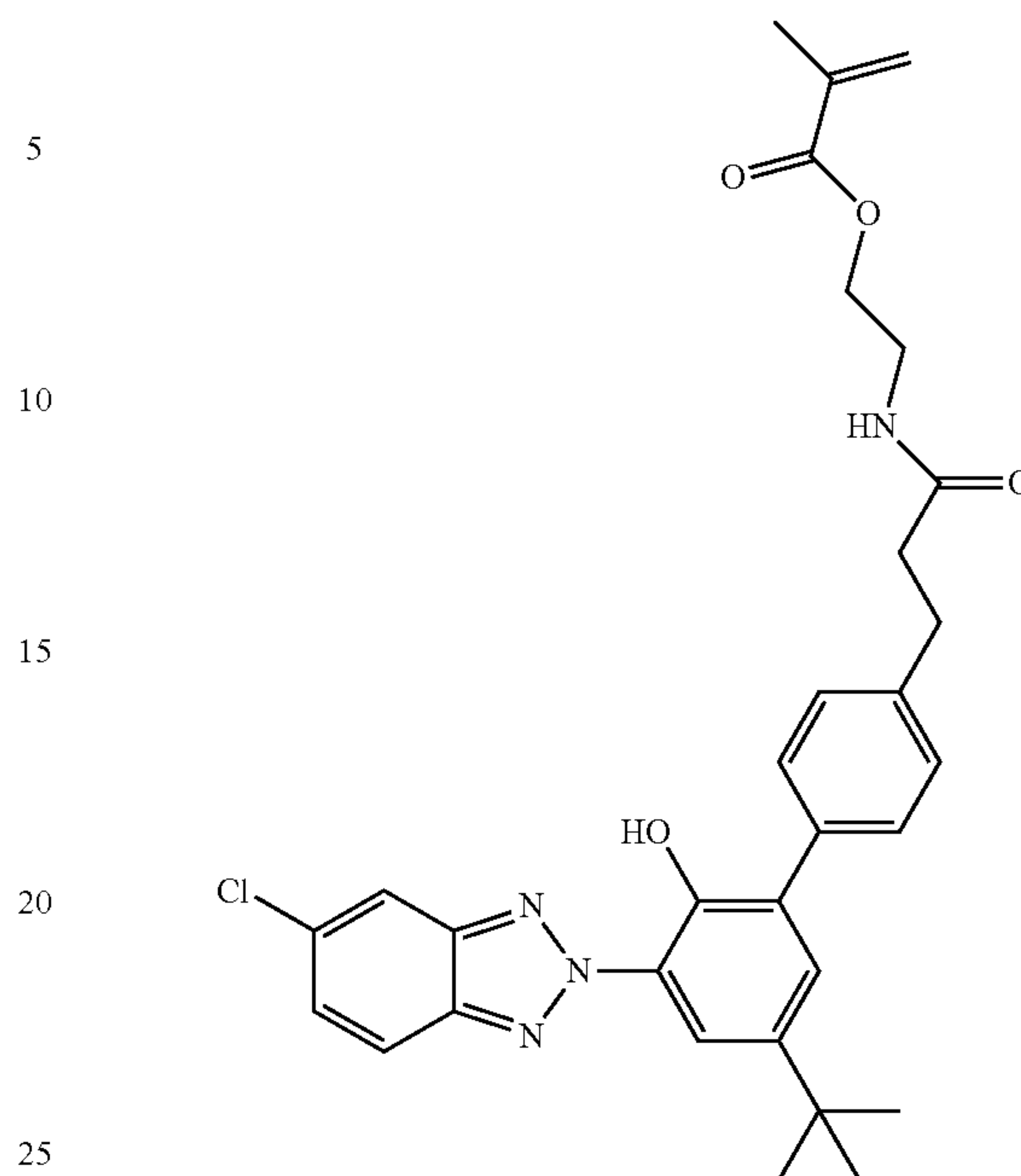
2-(3-(5'-(tert-butyl)-3'-(5-chloro-2H-benzo[d][1,2,3]triazol-2-yl)-2'-hydroxy-[1,1'-biphenyl]-4-yl)propanamido)ethyl methacrylate (Compound M)
