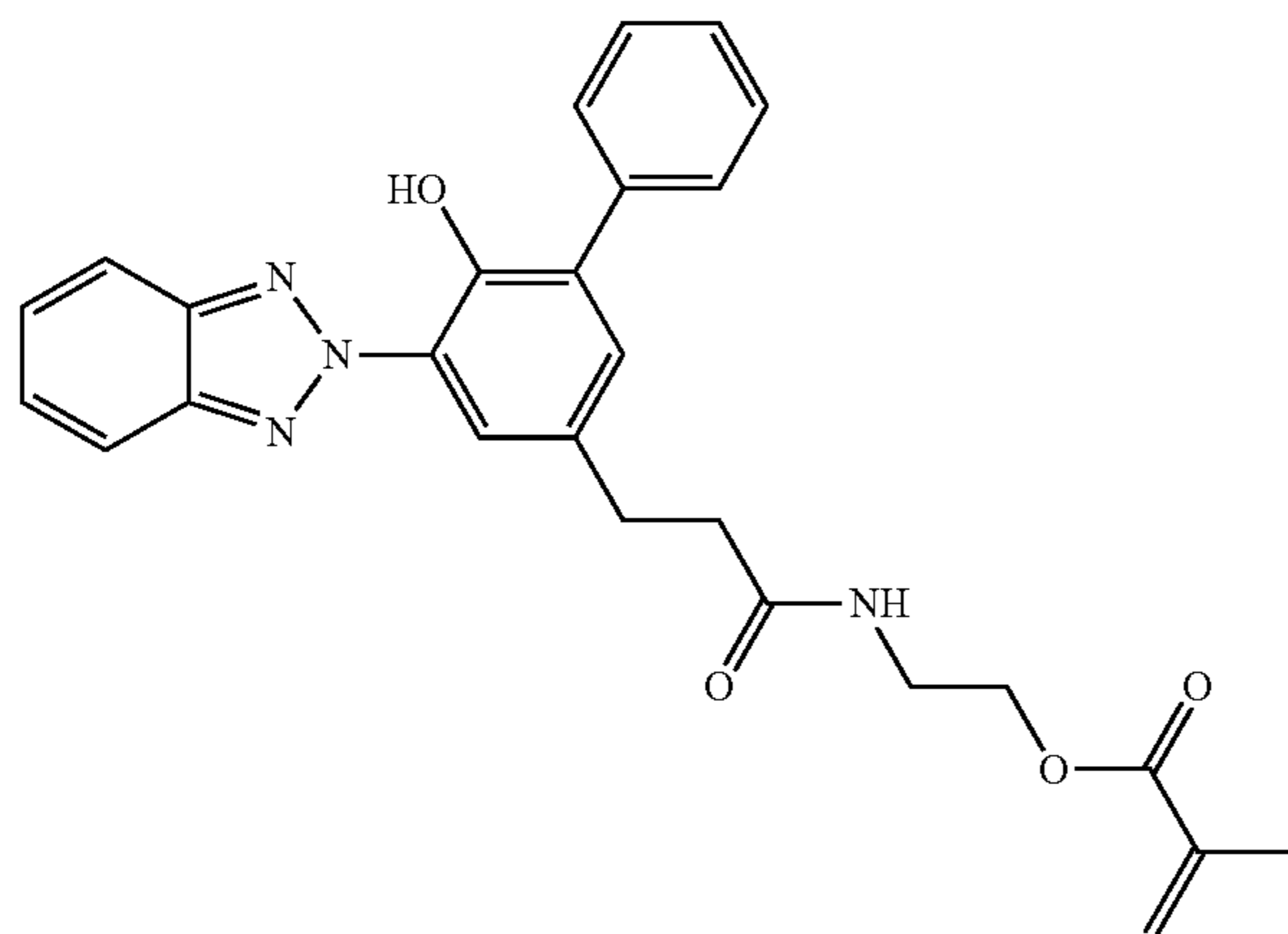
2-(3-(5-(2H-benzo[d][1,2,3]triazol-2-yl)-6-hydroxy-[1,1'-biphenyl]-3-yl)propanamido)ethyl methacrylate
