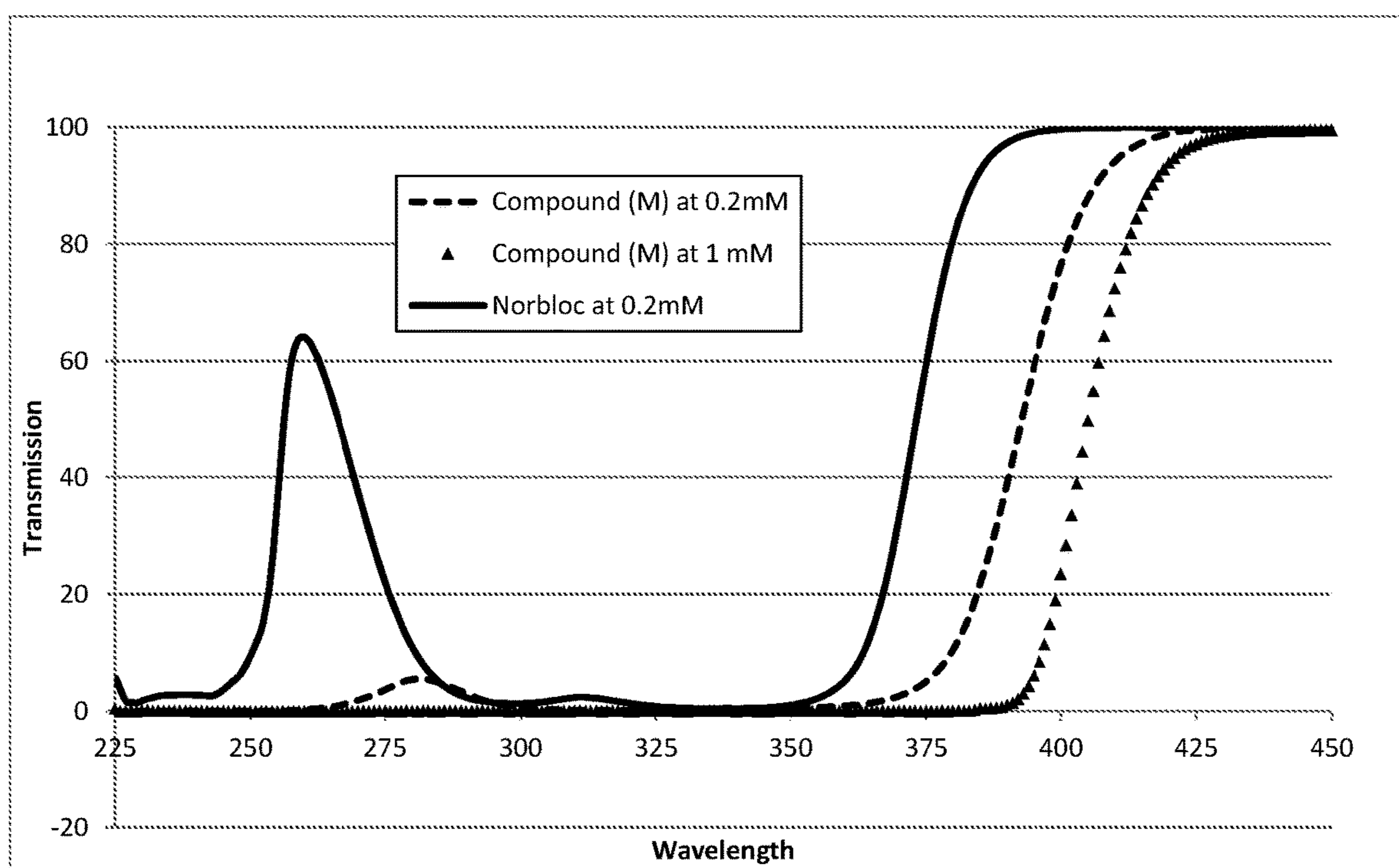
FIG. 2 - Transmission Spectra - 0.2 mM solutions of Norbloc and compound (M) in methylene chloride and 1 mM Compound (M) in methylene chloride
