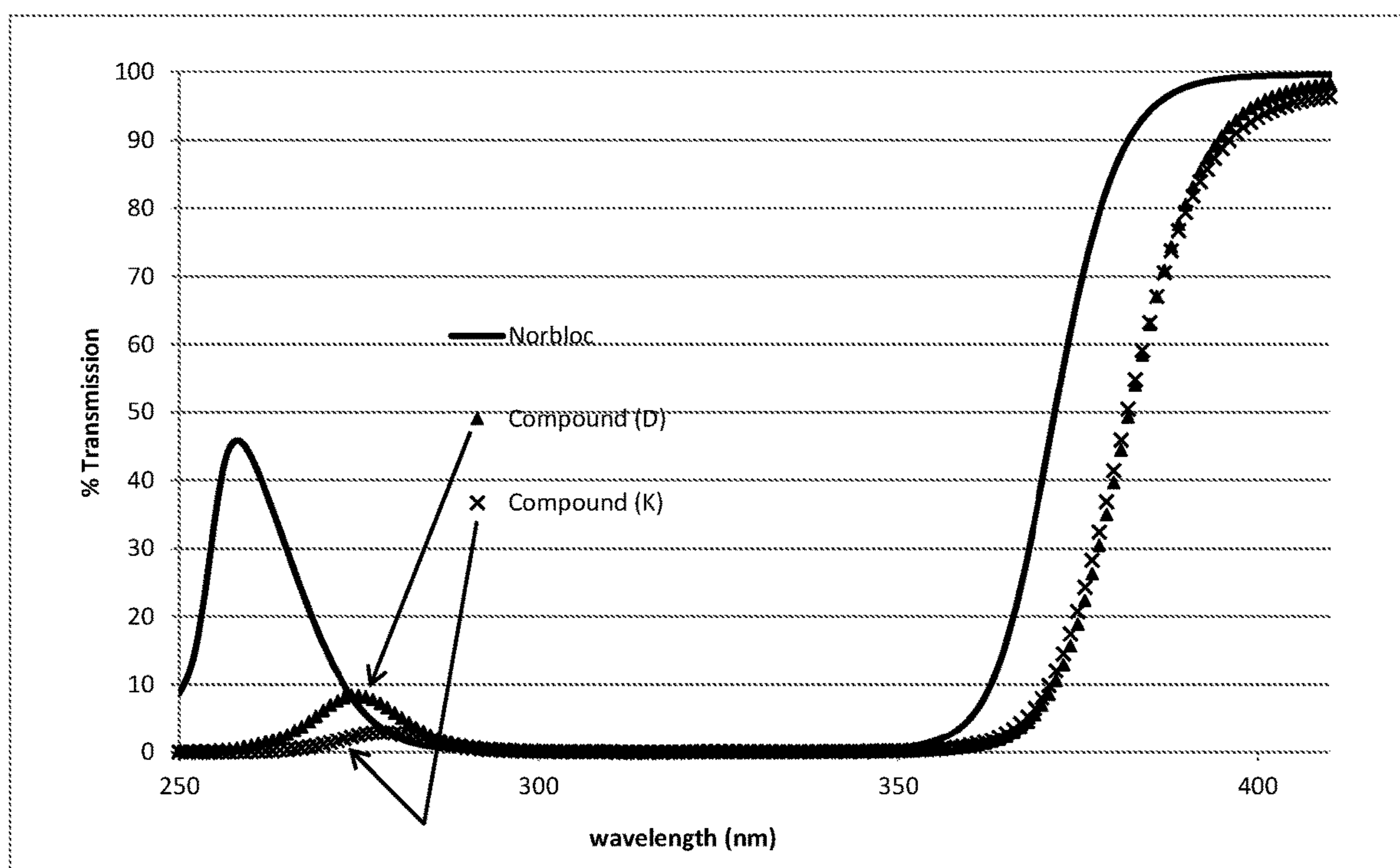
FIG. 1 - Transmission Spectra of 0.2 mM solutions of Norbloc, Compound (D), and Compound (K) in methanol
