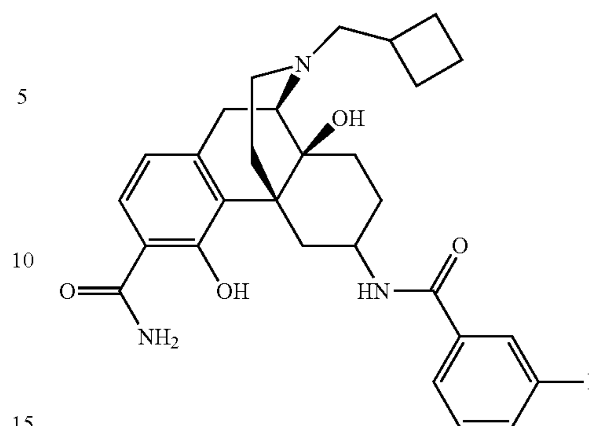
Compound 6
