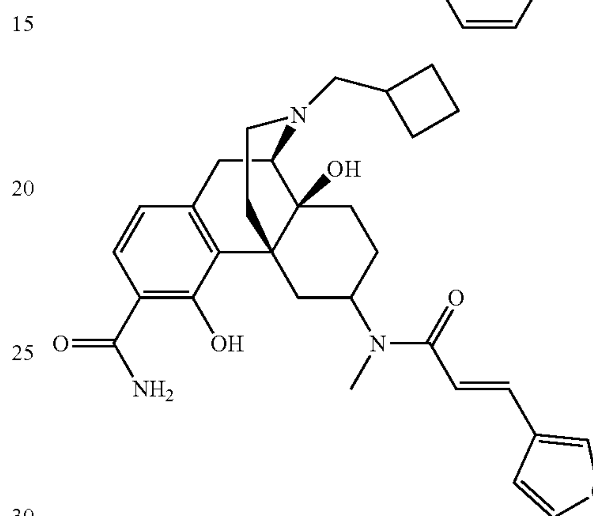
Compound 7
