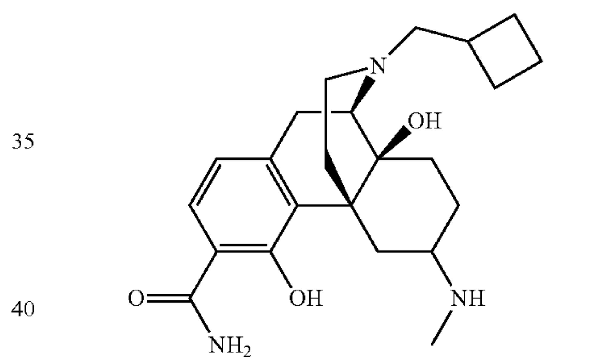
Compound 13
