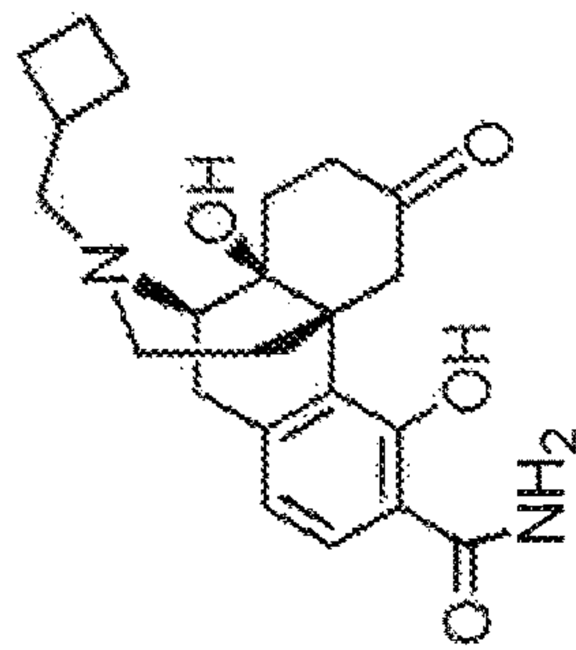
Compound A
