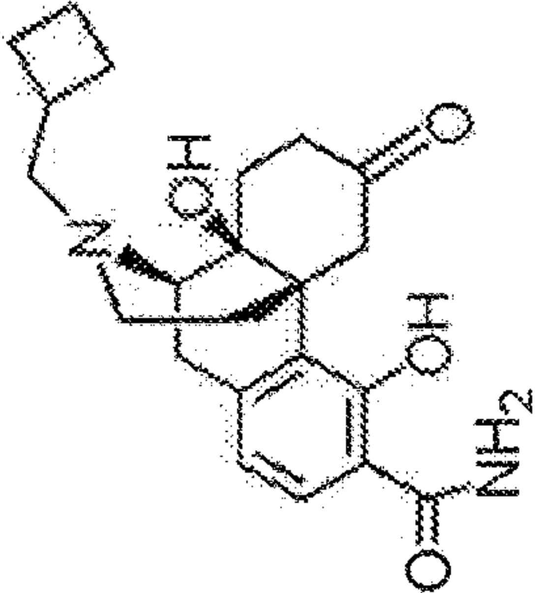
Compound A
