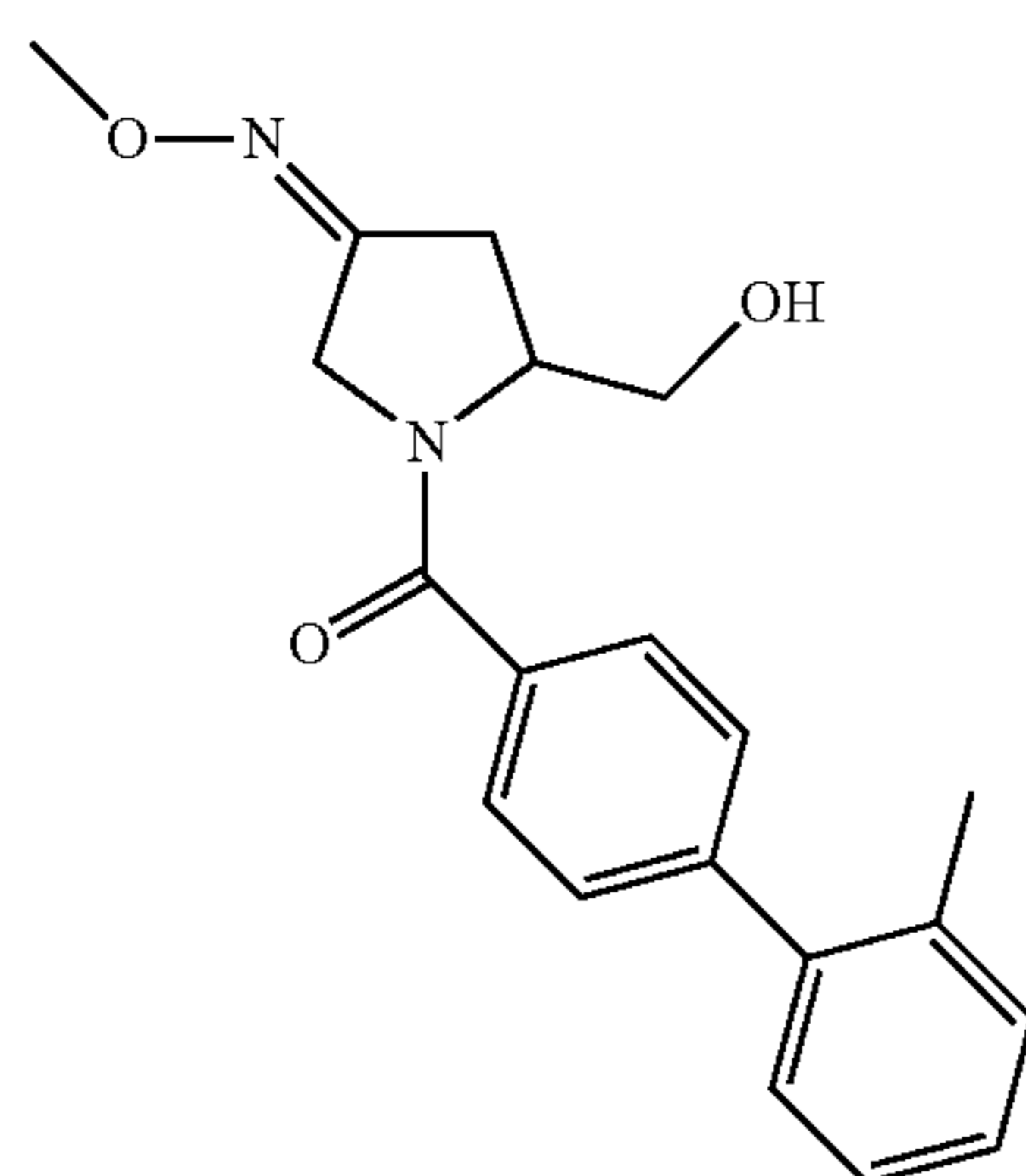
\text{C}_{20}\text{H}_{22}\text{N}_2\text{O}_3 Mol. Wt.: 338.40
