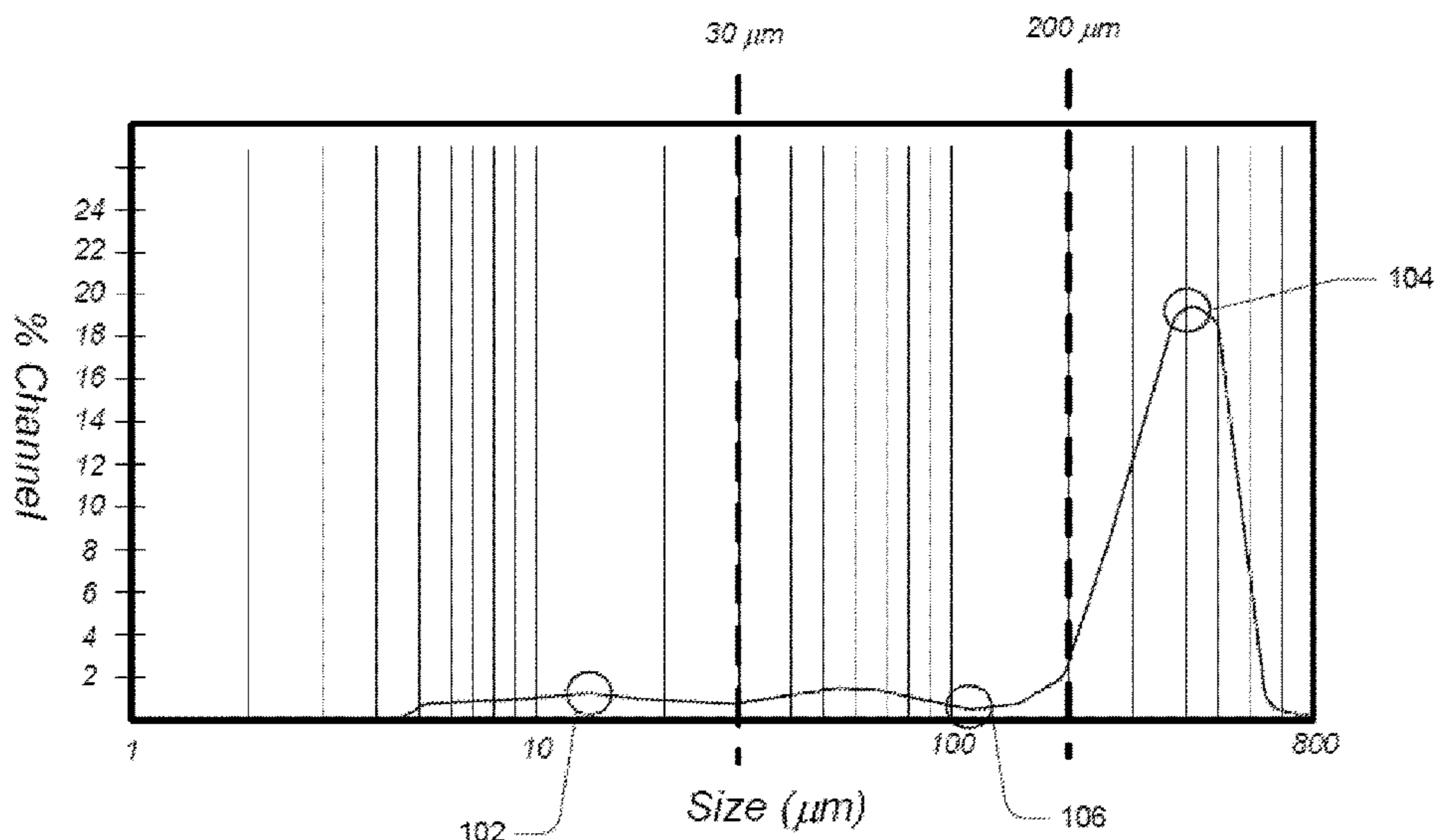
Particle Size Distribution Plot
