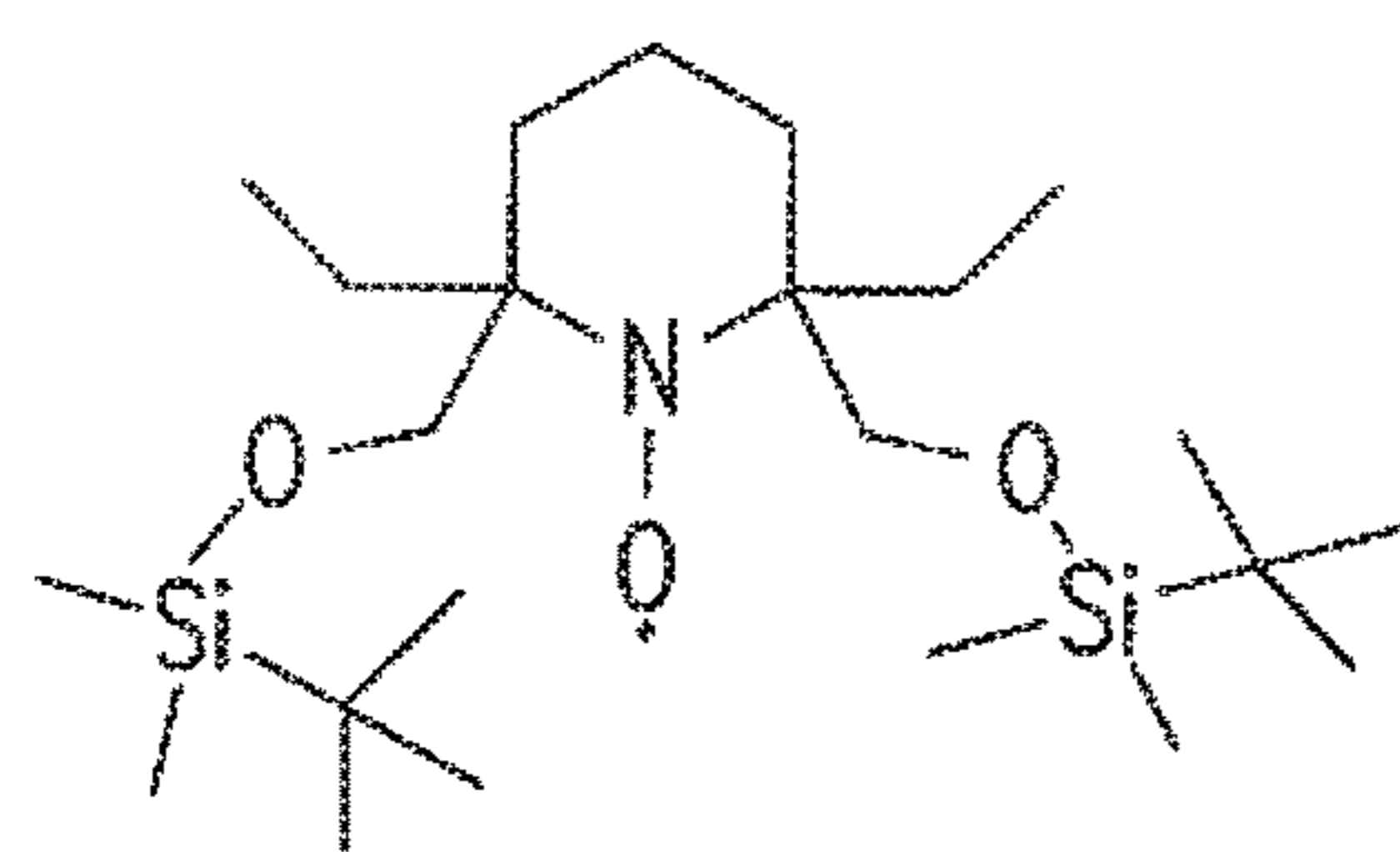
G5, LogP=8.2
