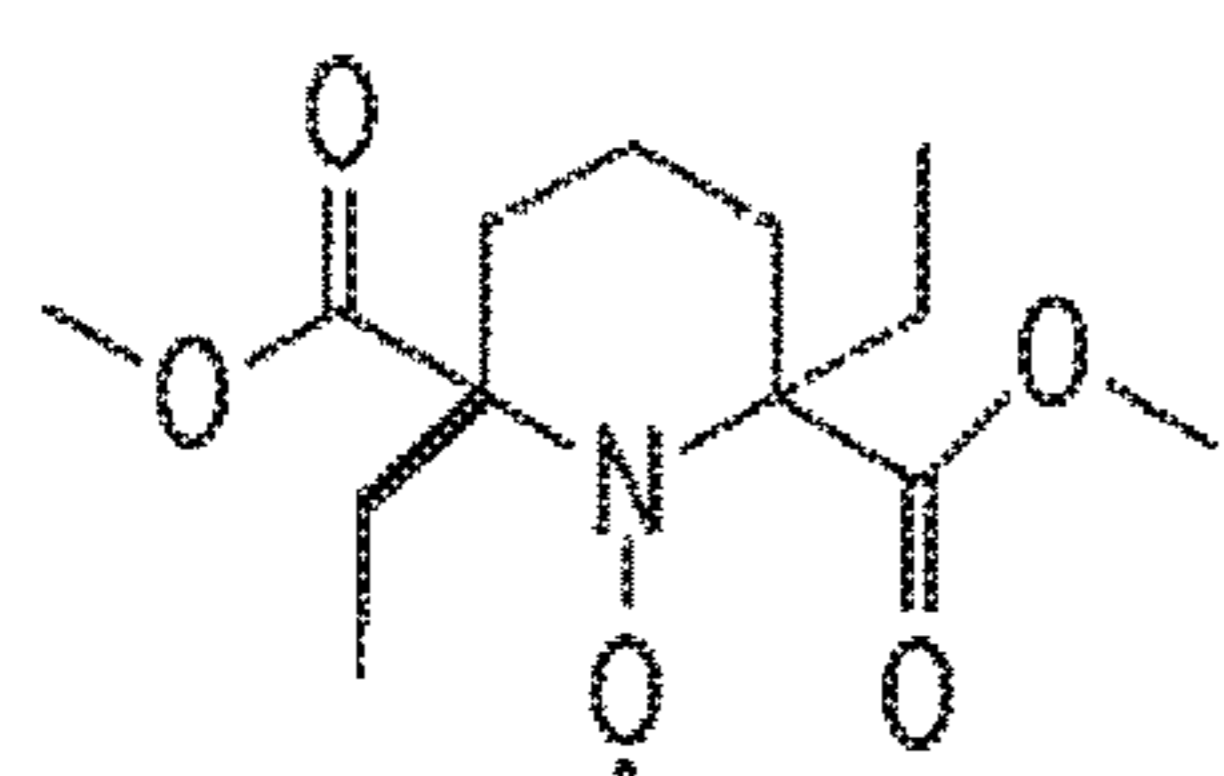
G1, LogP=2.0
