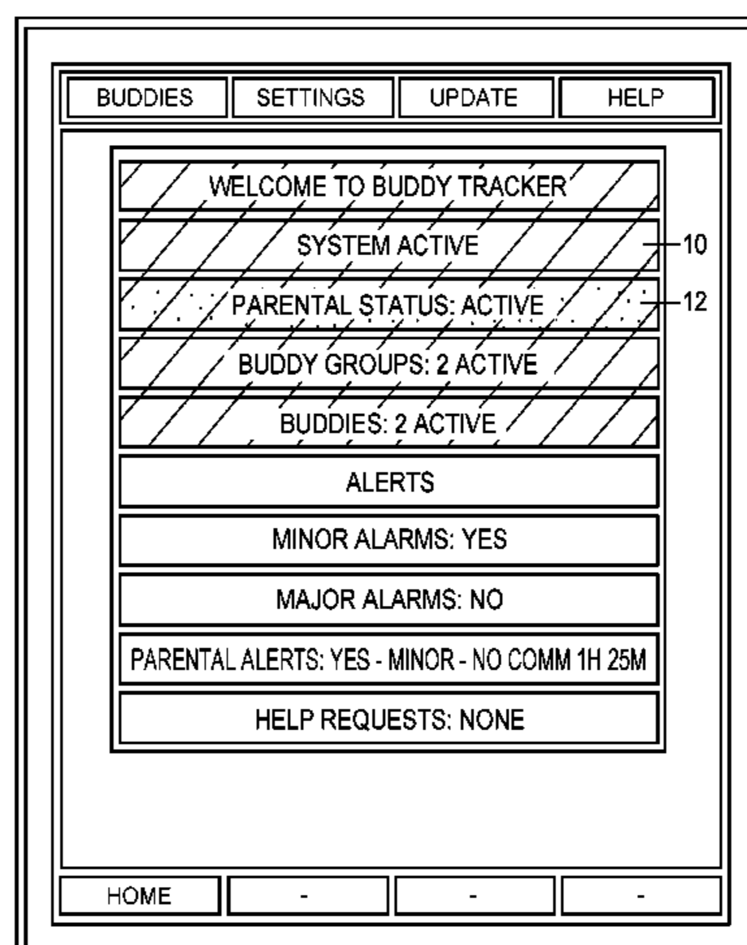
OPENING SCREEN
