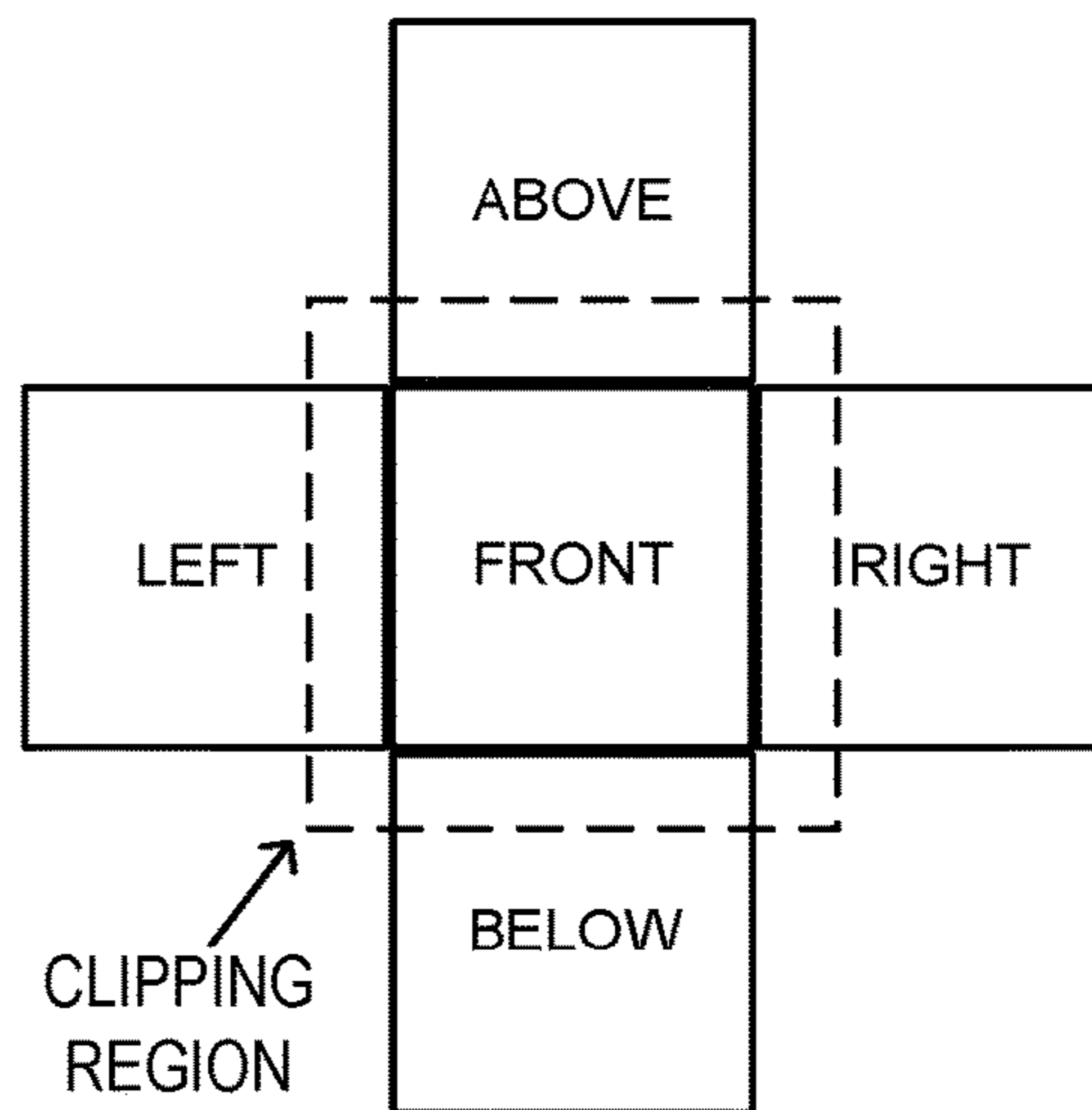
CLIPPED CUBEMAP
