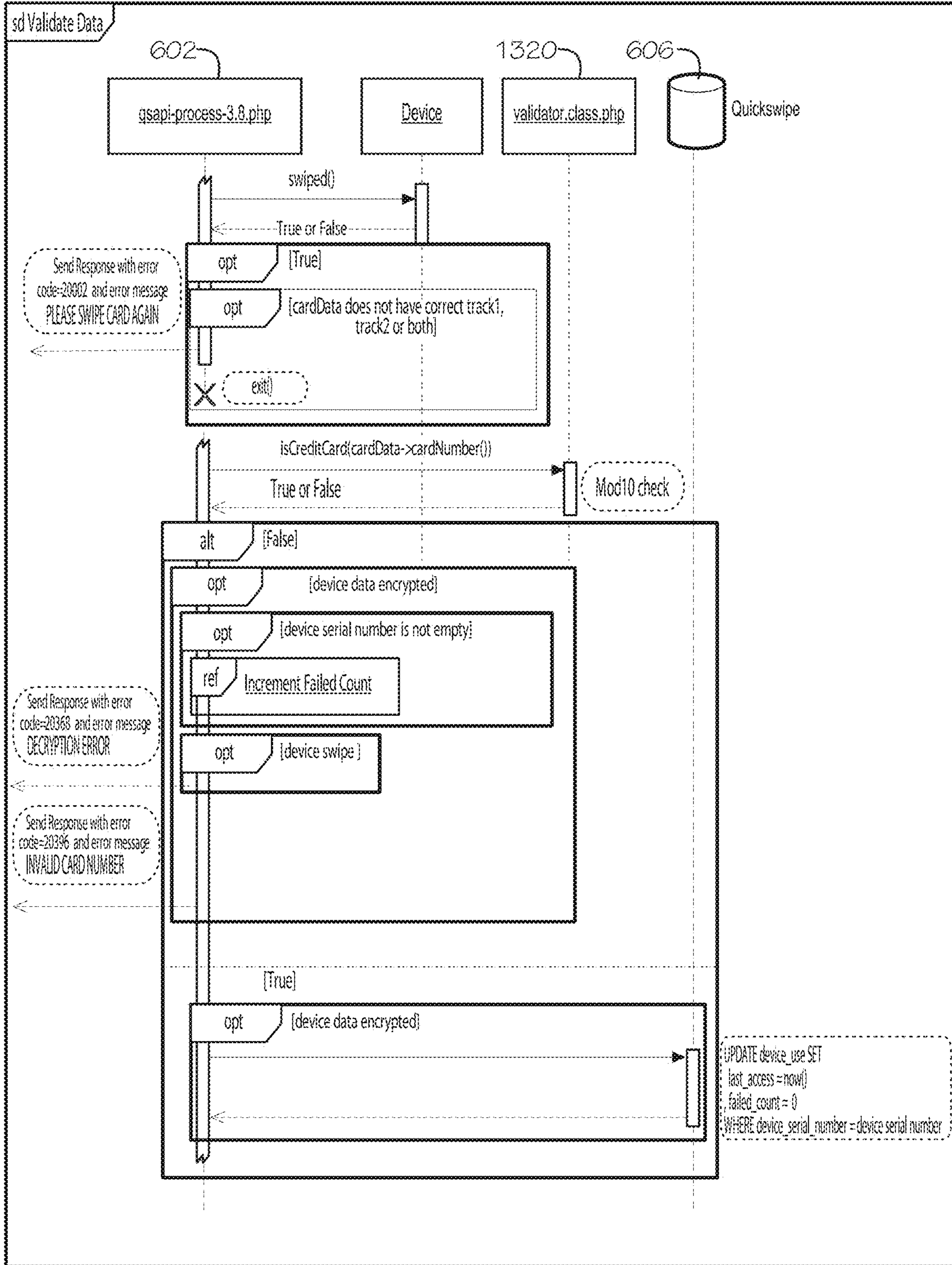
UML OF EXEMPLARY VALIDATION SEQUENCE
