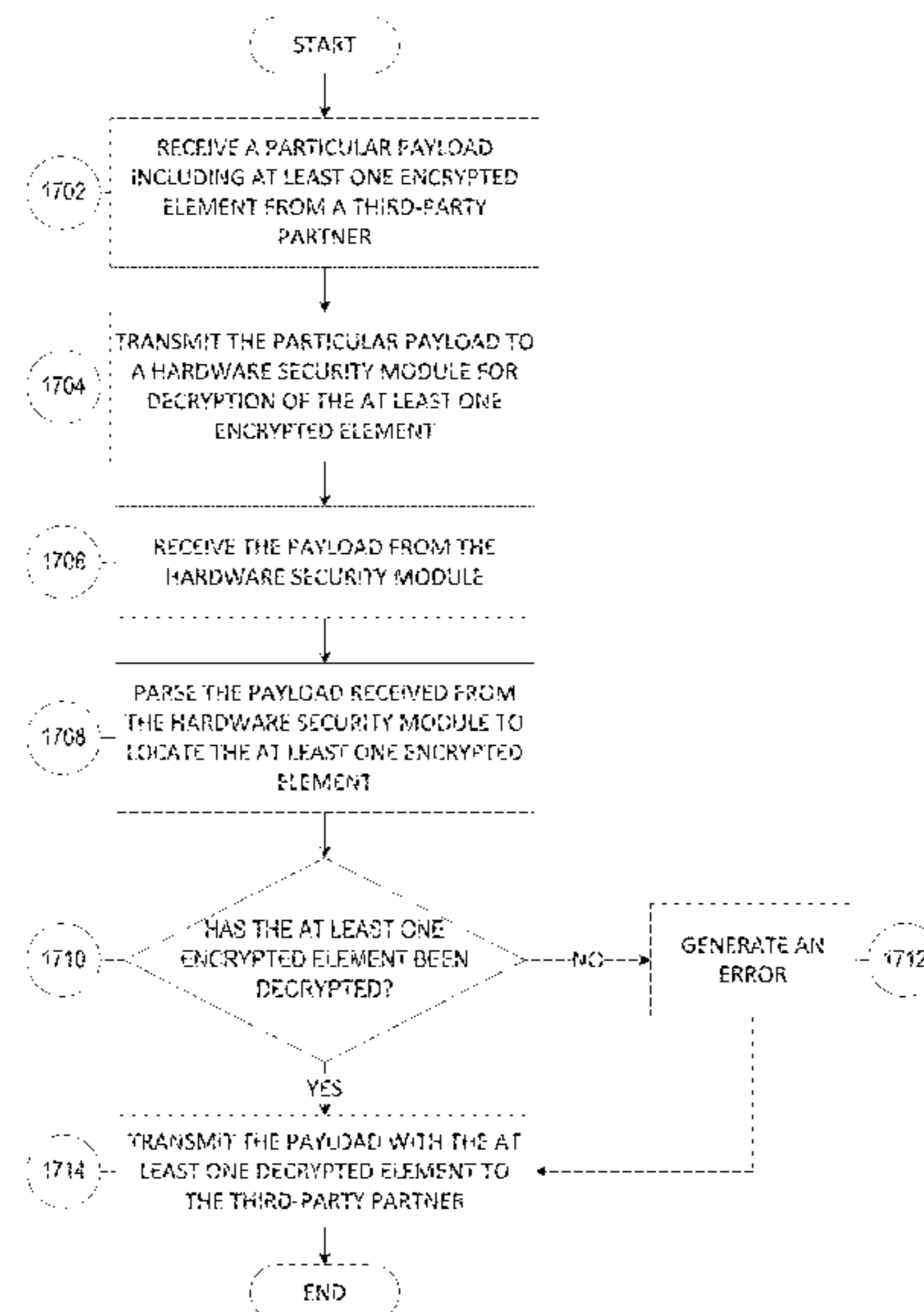
EXEMPLARY DECRYPTION VERIFICATION PROCESS
