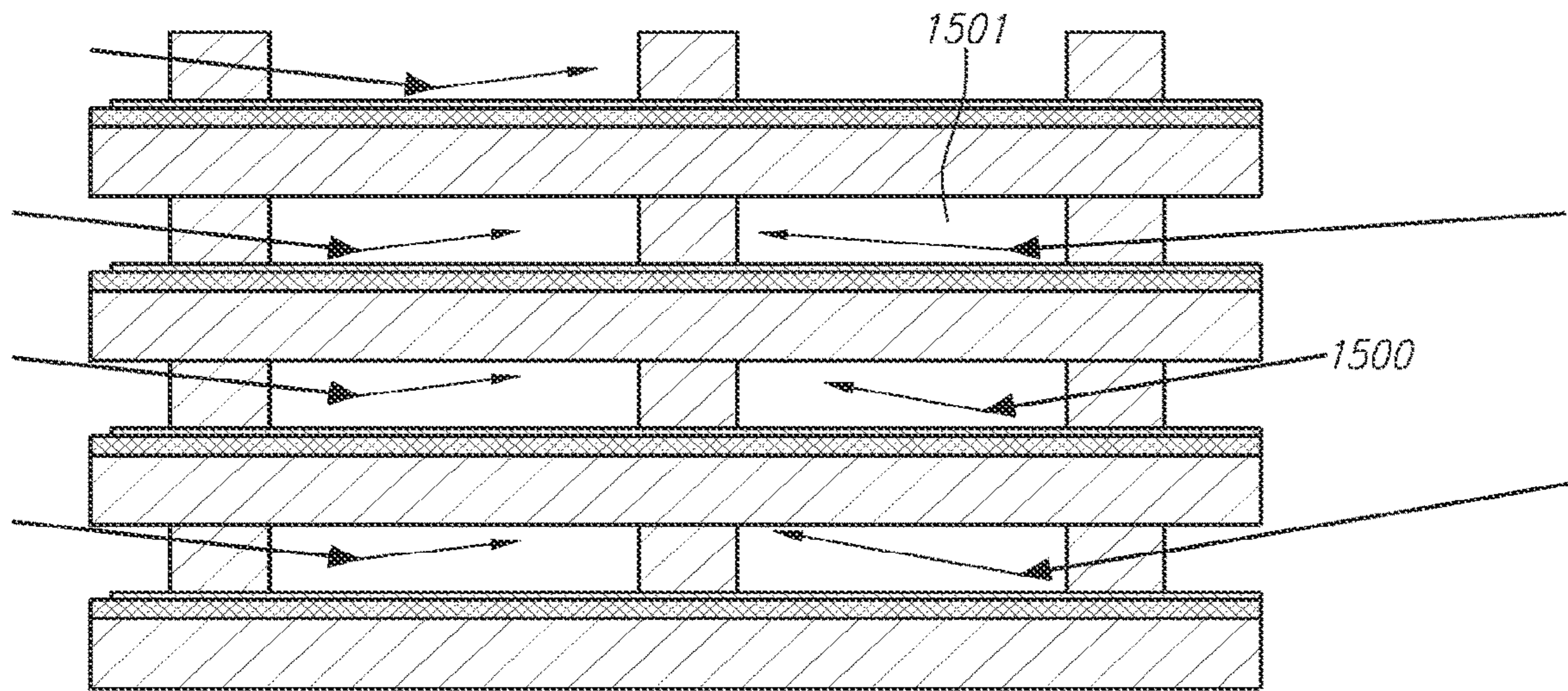
Simple stacking, end view
