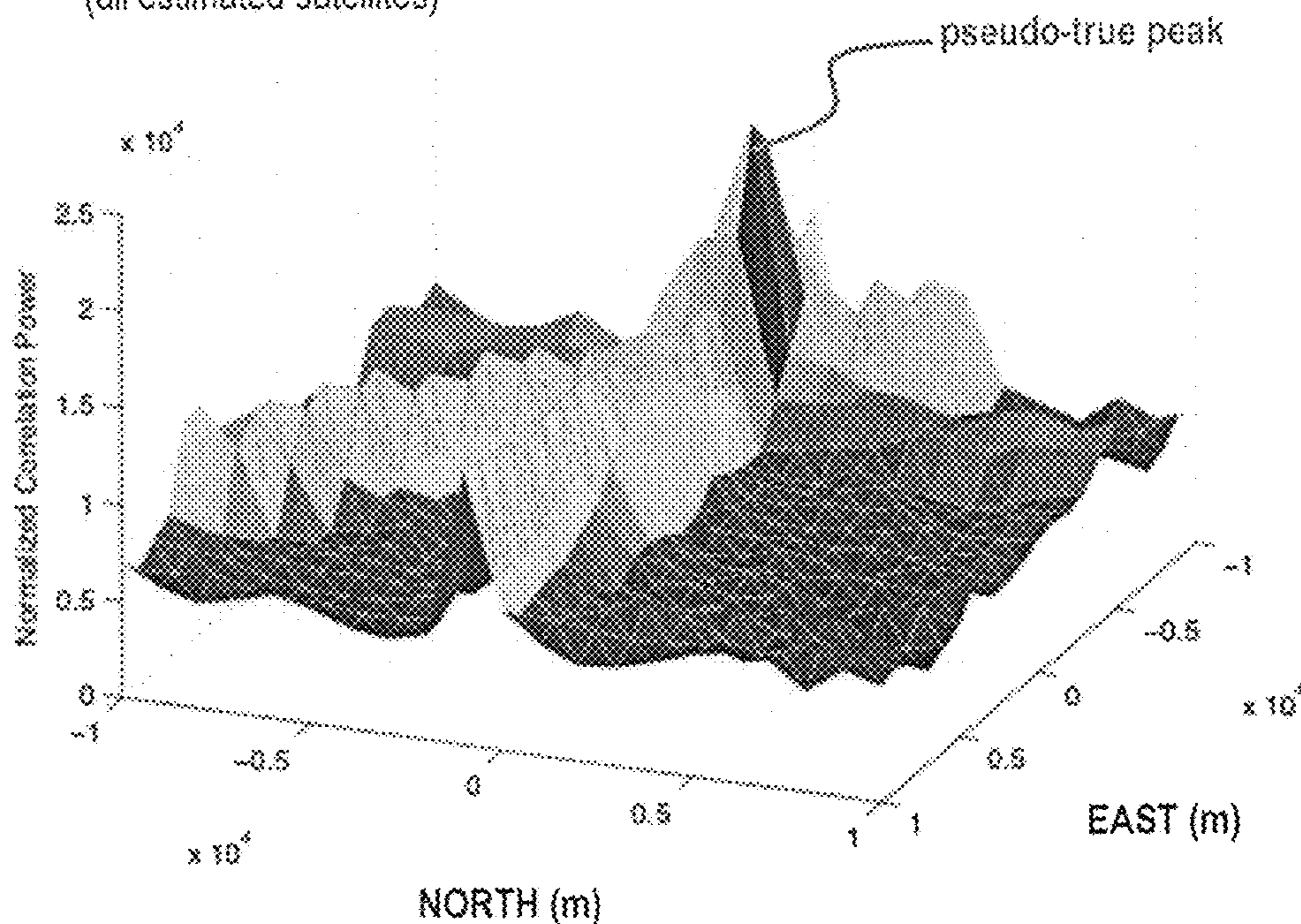
POSITION DOMAIN CORRELOGRAM (all estimated satellites)
