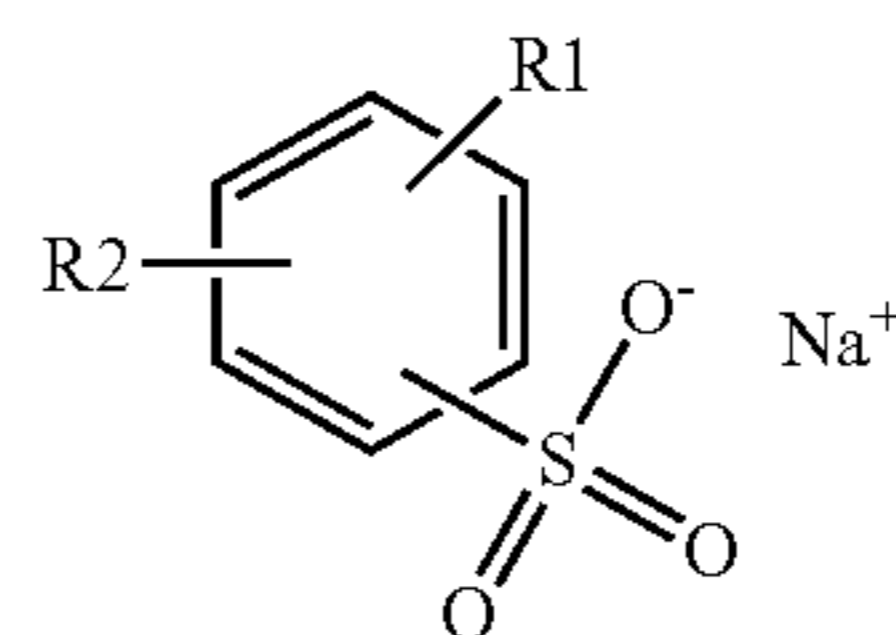
ALKYLBENZENE SULFONATE
