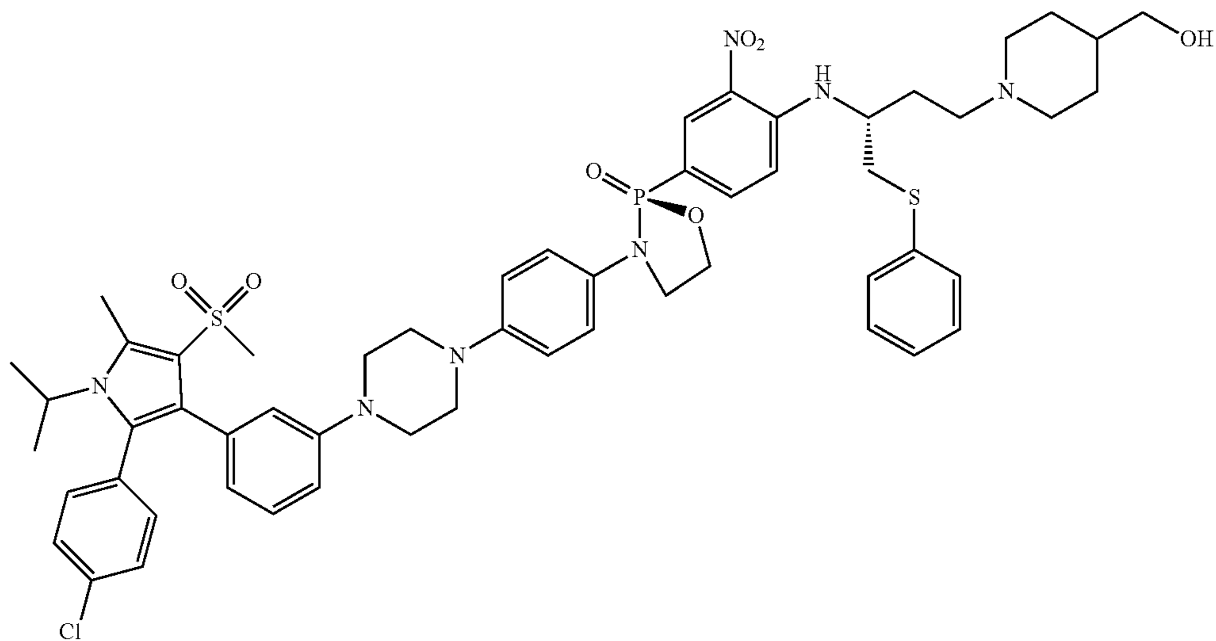
(S)-3-(4-(4-(3-(2-(4-chlorophenyl)-1-isopropyl-5-methyl-4-(methylsulfonyl)-1H-pyrrol-3-yl)phenyl)piperazin-1-yl)phenyl)-2-(4-(((R)-4-(hydroxymethyl)piperidin-1-yl)-1-(phenylthio)butan-2-yl)amino)-3-nitrophenyl)-1,3,2-oxazaphospholidine 2-oxide
