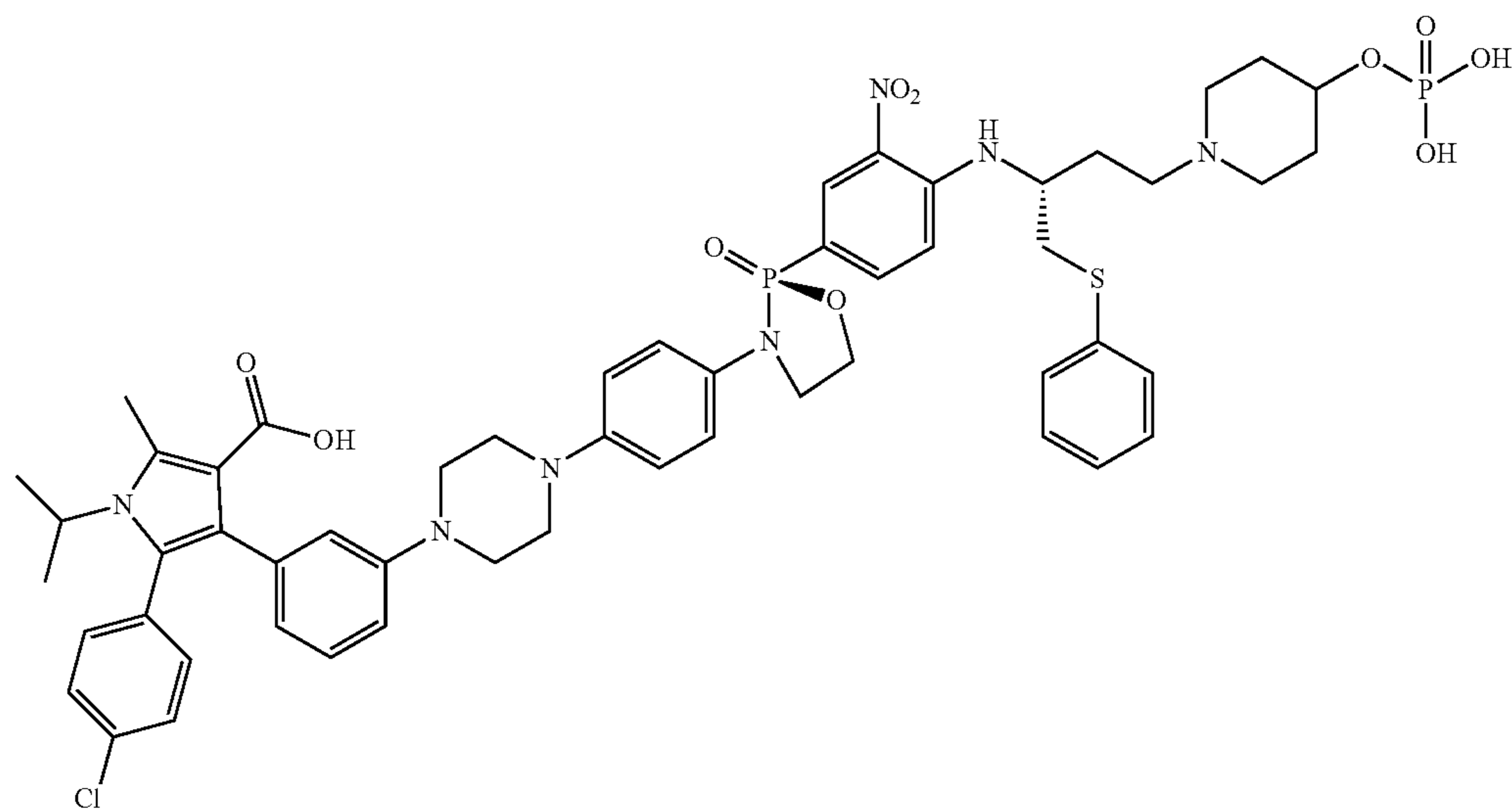
5-(4-chlorophenyl)-1-isopropyl-2-methyl-4-(3-(4-(4-((S)-2-(3-nitro-4-(((R)-1-(phenylthio)-4-(4-(phosphonoxy)piperidin-1-yl)butan-2-yl)amino)phenyl)-2-oxido-1,3,2-oxazaphospholidin-3-yl)phenyl)piperazin-1-yl)phenyl)-1H-pyrrole-3-carboxylic acid
