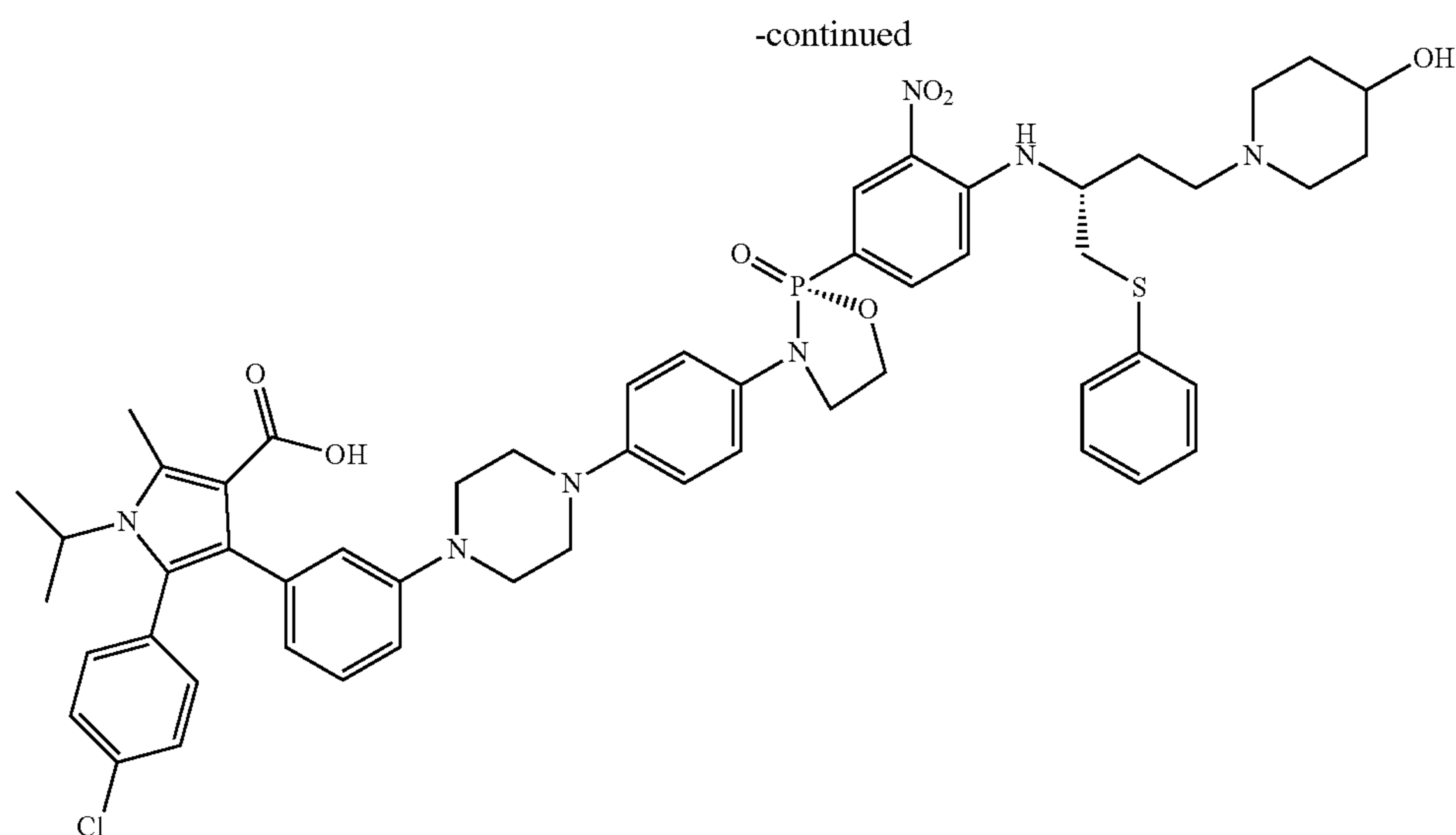
5-(4-chlorophenyl)-4-(3-(4-(4-((R)-2-(4-(((R)-2-(4-((R)-4-(4-hydroxypiperidin-1-yl)-1-(phenylthio)butan-2-yl)amino)-3-nitrophenyl)-2-oxido-1,3,2-oxazaphospholidin-3-yl)phenyl)piperazin-1-yl)phenyl)-1-isopropyl-2-methyl-1H-pyrrole-3-carboxylic acid
