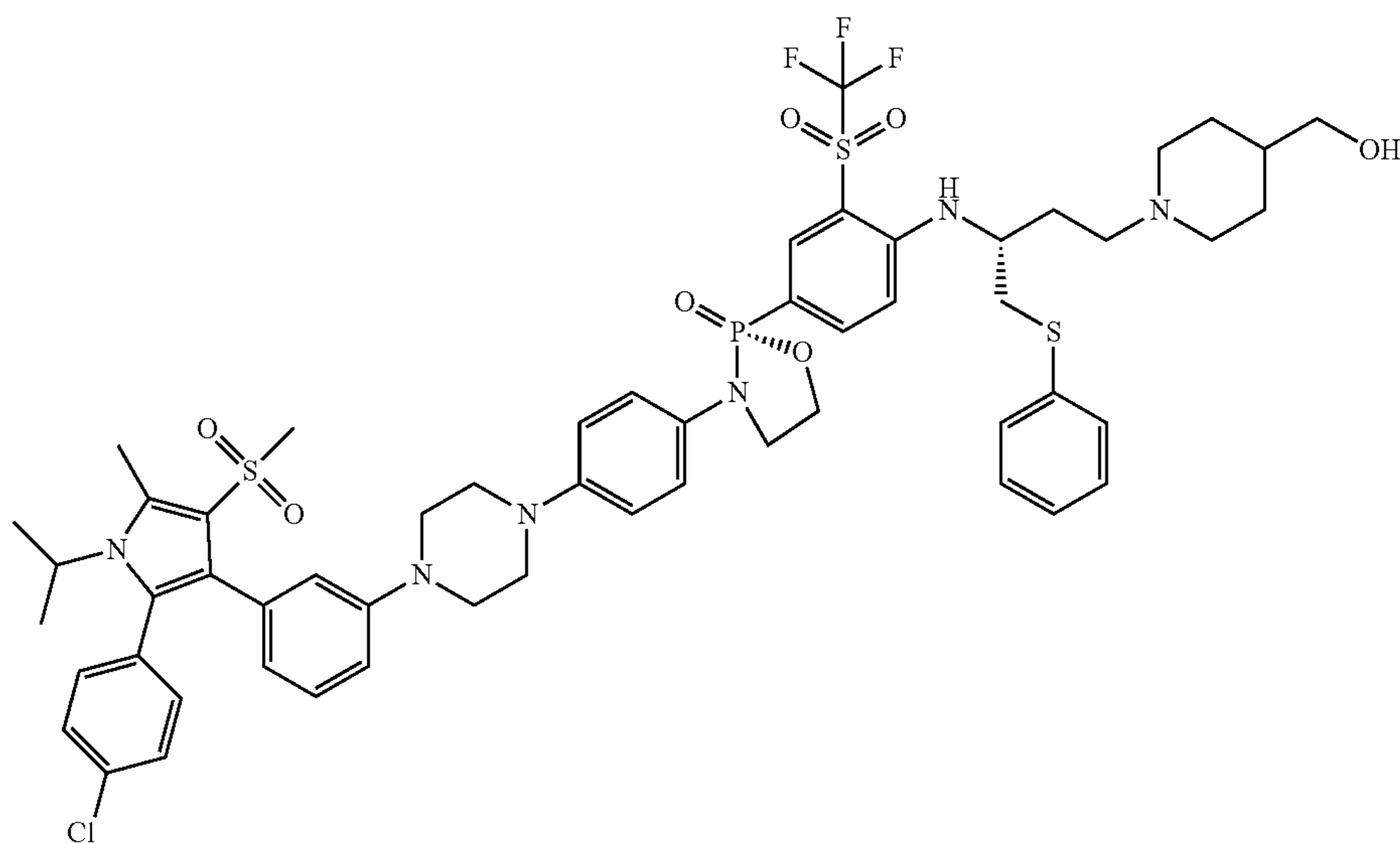
(R)-3-(4-(3-(2-(4-chlorophenyl)-1-isopropyl-5-methyl-4-(methylsulfonyl)-1H-pyrrol-3-yl)phenyl)piperazin-1-yl)phenyl-2-(4-(((R)-4-(4-(hydroxymethyl)piperidin-1-yl)-1-(phenylthio)butan-2-yl)amino)-3-(trifluoromethyl)sulfonyl)phenyl)-1,3,2-oxazaphospholidine 2-oxide
