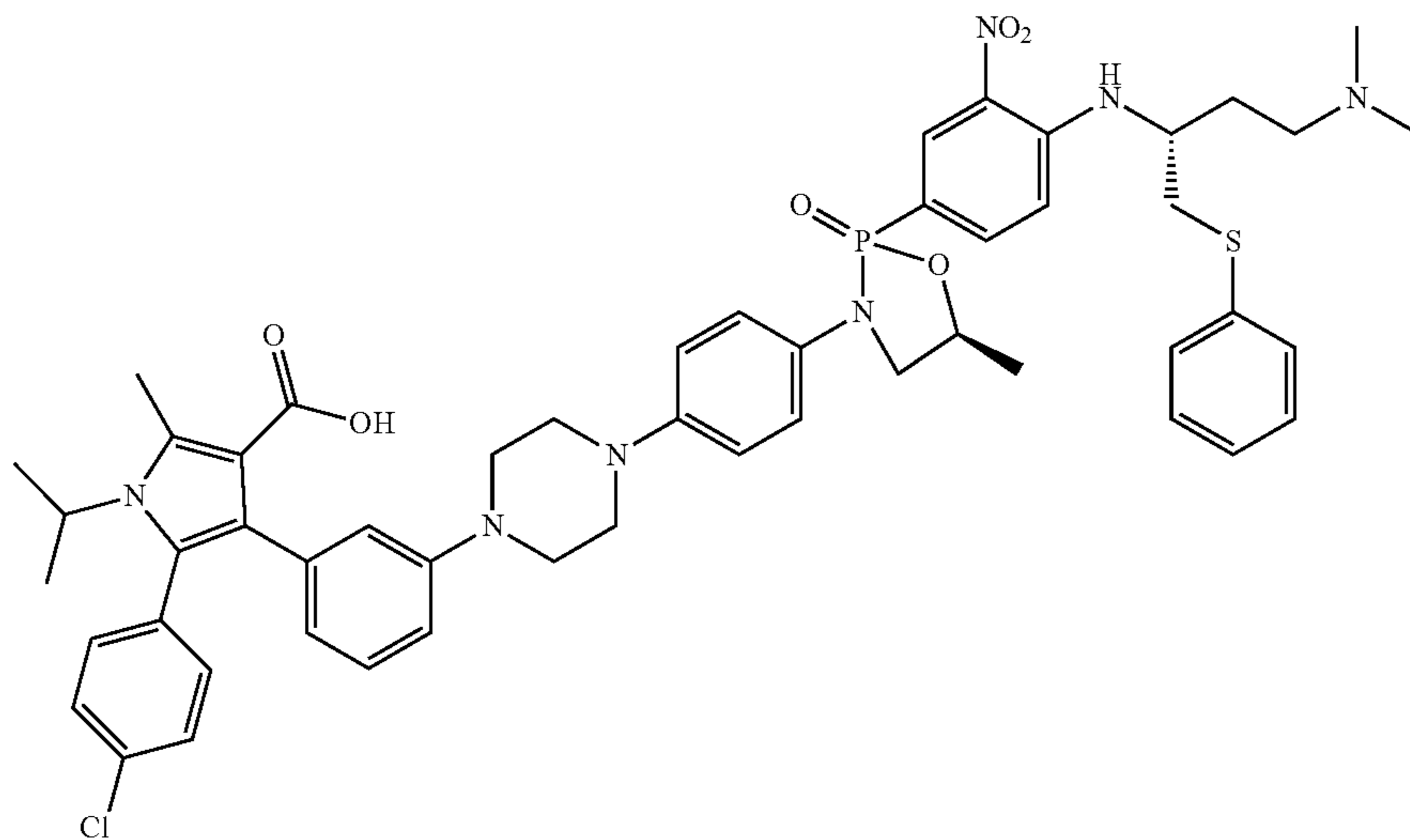
5-(4-chlorophenyl)-4-(3-(4-(4-((S)-2-(4-((R)-4-dimethylamino)-1-(phenylthio)butan-2-yl)amino-3-nitrophenyl)-5-methyl-2-oxido-1,3,2-oxazaphospholidin-3-yl)phenyl)piperazin-1-yl)phenyl)-1-isopropyl-2-methyl-1H-pyrrole-3-carboxylic acid
