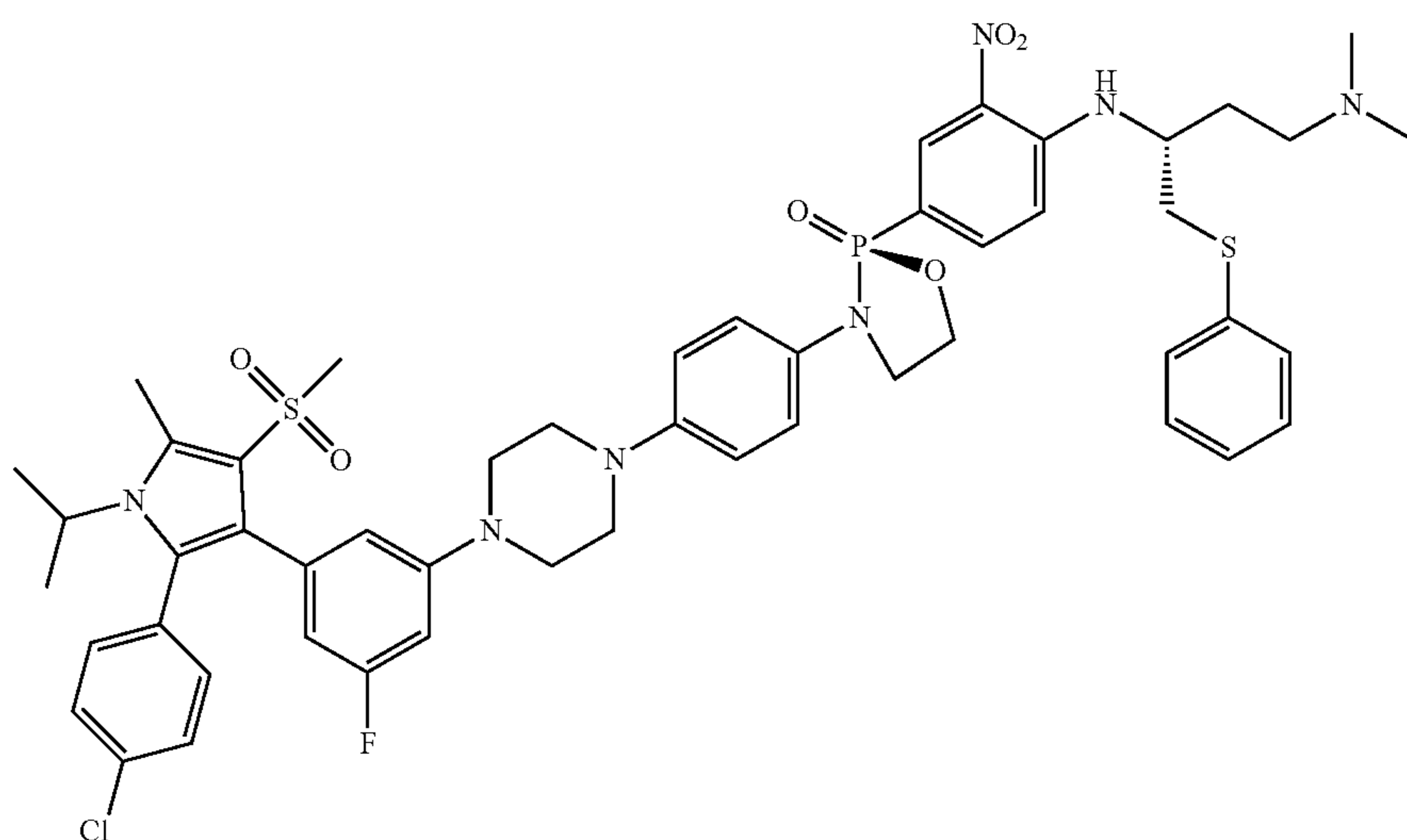
(S)-3-(4-(4-(3-(2-(4-chlorophenyl)-1-isopropyl-5-methyl-4-(methylsulfonyl)-1H-pyrrol-3-yl)-5-fluorophenyl)piperazin-1-yl)phenyl)-2-(4-(((R)-4-(dimethylamino)-1-(phenylthio)butan-2-yl)amino))-3-nitrophenyl)-1,3,2-oxazaphospholidine 2-oxide
