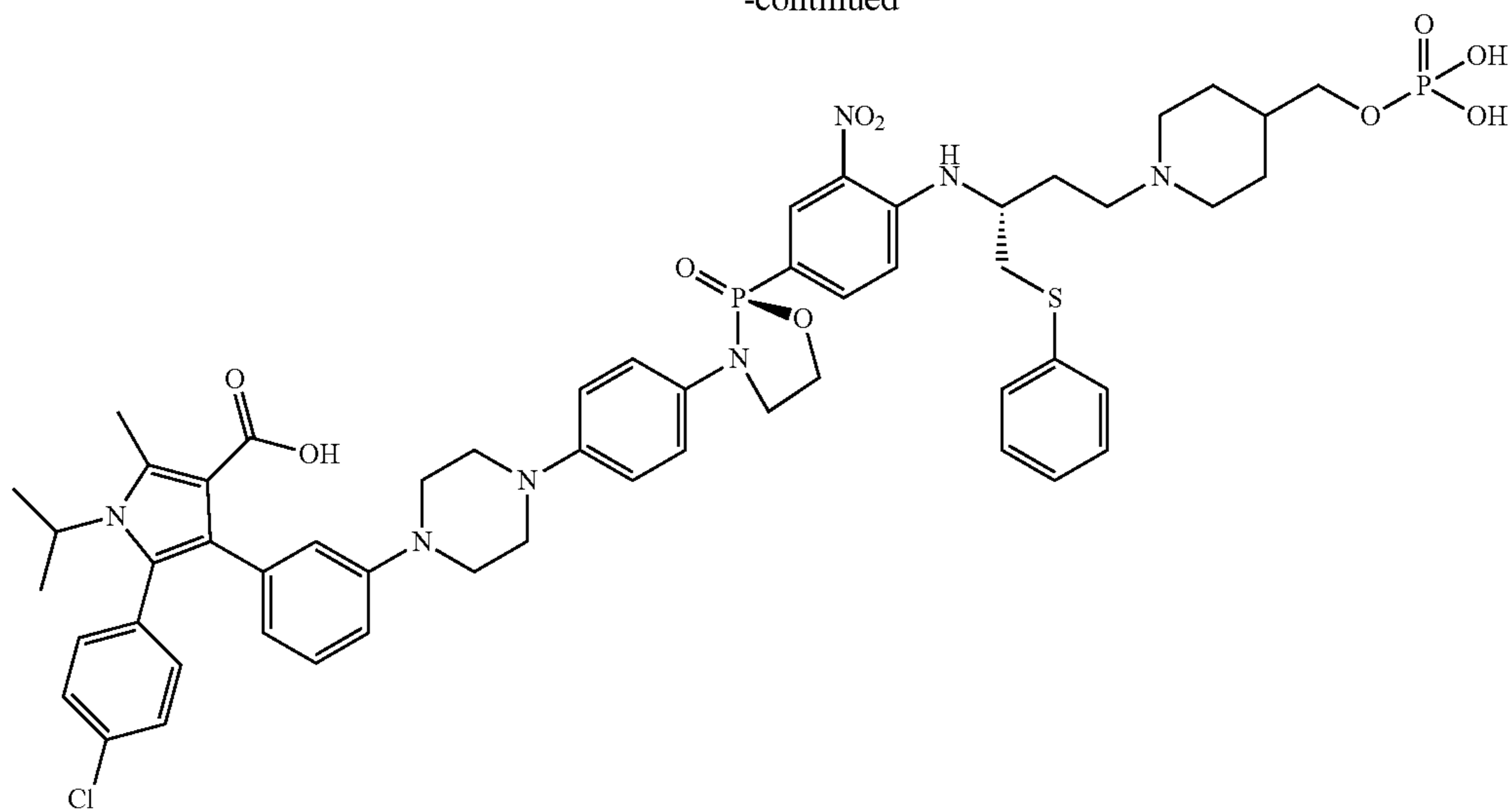
5-(4-chlorophenyl)-1-isopropyl-2-methyl-4-(3-(4-(4-((S)-2-(3-nitro-4-((R)-1-(phenylthio)-4-(4-(phosphonooxy)piperidin-1-yl)butan-2-yl)amino)phenyl)-2-oxido-1,3,2-oxazaphospholidin-3-yl)phenyl)piperazin-1-yl)phenyl)-1H-pyrrole-3-carboxylic acid
