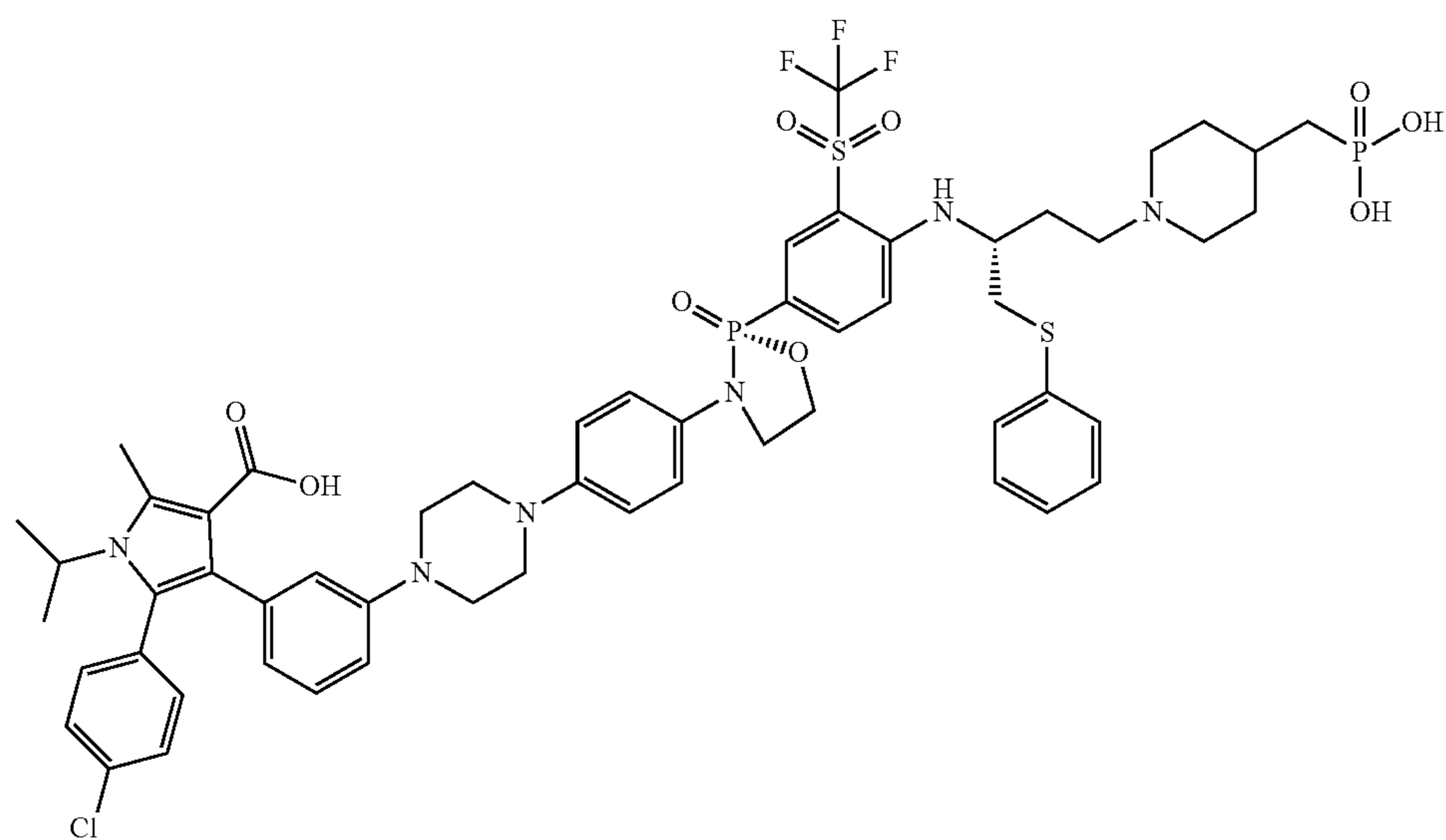
5-(4-chlorophenyl)-1-isopropyl-2-methyl-4-(3-(4-(4-((R)-2-oxido-2-(4-((R)-1-(phenylthio)-4-(4-(phosphonomethyl)piperidin-1-yl)butan-2-yl)amino)-3-((trifluoromethyl)sulfonyl)phenyl)-1,3,2-oxazaphospholidin-3-yl)phenyl)piperazin-1-yl)phenyl)-1H-pyrrole-3-carboxylic acid
