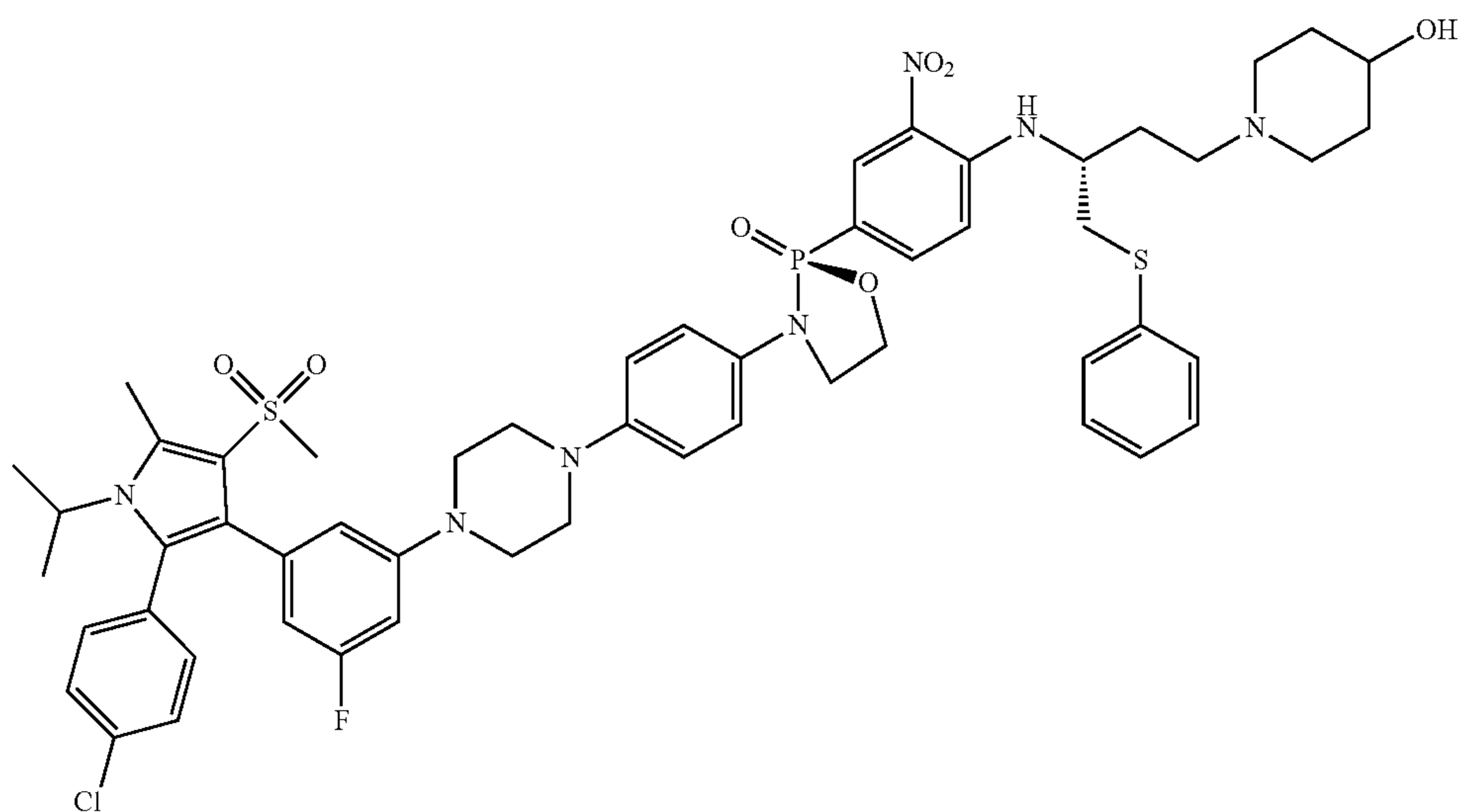
(S)-3-(4-(4-(3-(2-(4-chlorophenyl)-1-isopropyl-5-methyl-4-(methylsulfonyl)-1H-pyrrol-3-yl)-5-fluorophenyl)piperazin-1-yl)phenyl)-2-(4-(((R)-4-(4-(hydroxymethyl)piperidin-1-yl)-(phenylthio)butan-2-yl)amino)-3-nitrophenyl)-1,3,2-oxazaphospholidine 2-oxide
