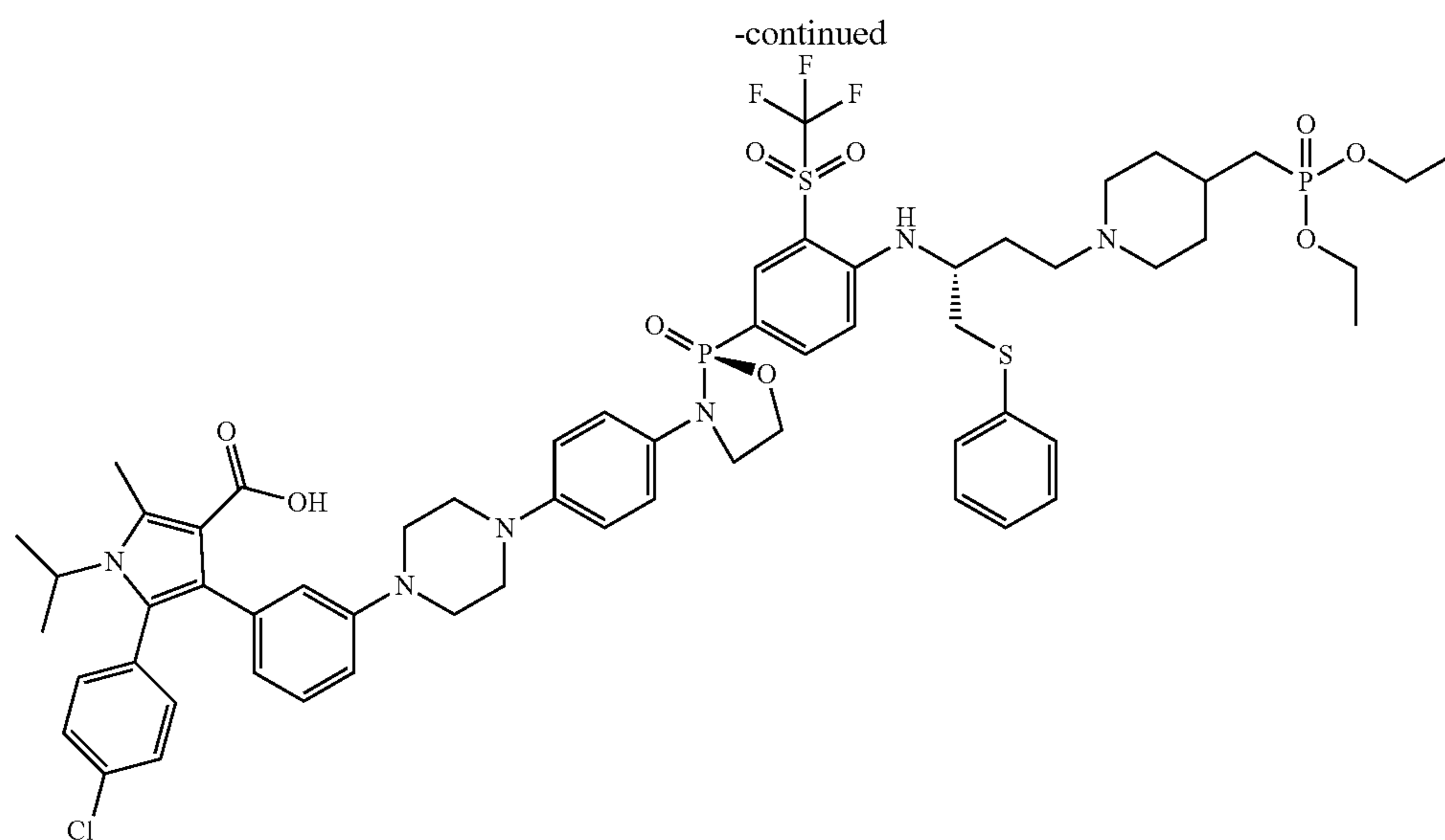
5-(4-chlorophenyl)-4-(3-(4-(4-((S)-2-(4-(((R)-4-(4-((diethoxyphosphoryl)methyl)piperidin-1-yl)-1-(phenylthio)butan-2-yl)amino)-3-((trifluoromethyl)sulfonyl)phenyl)-2-oxido-1,3,2-oxazaphospholidin-3-yl)phenyl)piperazin-1-yl)phenyl)-1-isopropyl-2-methyl-1H-pyrrole-3-carboxylic acid
