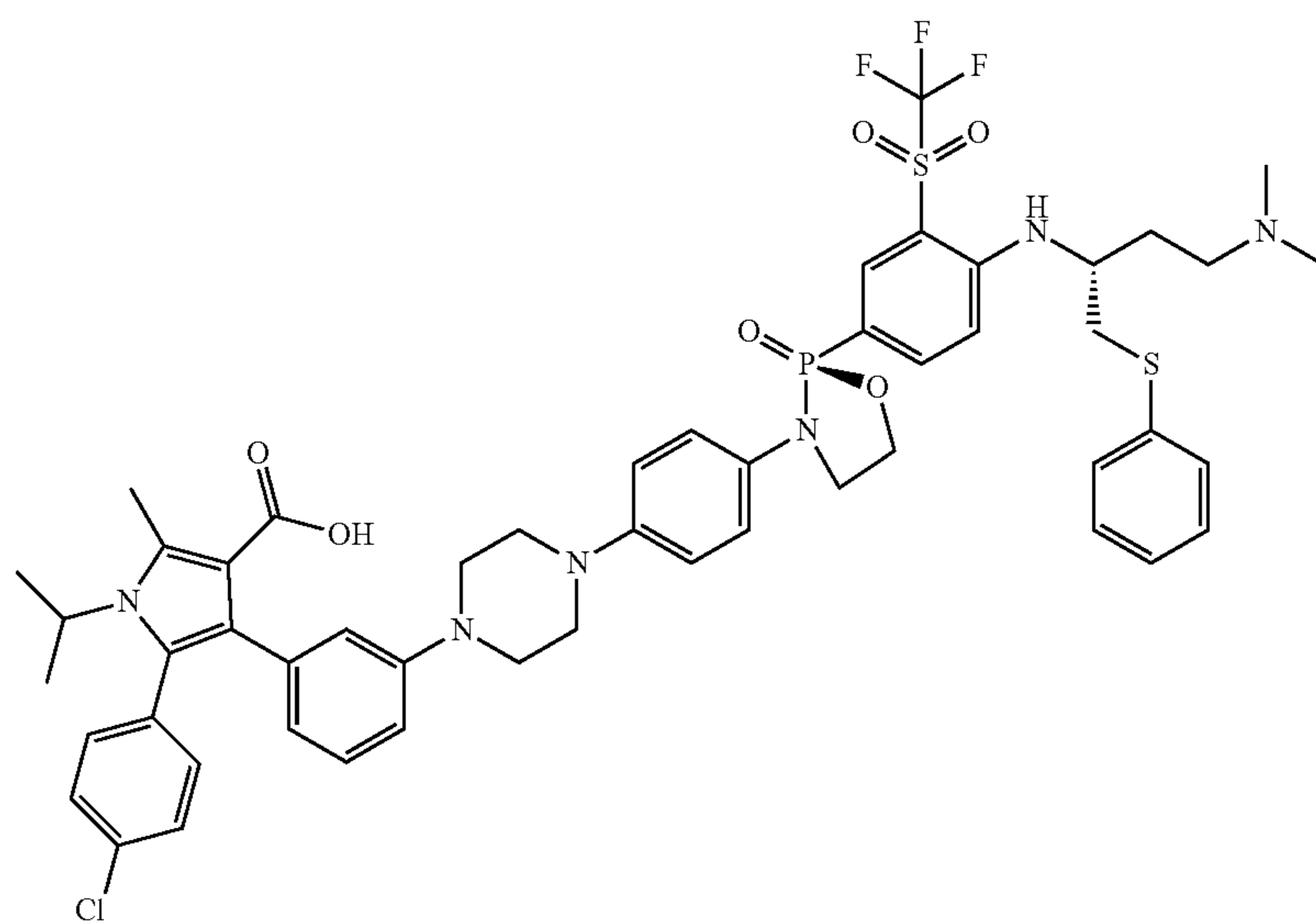
5-(4-chlorophenyl)-4-(3-(4-(4-((S)-2-(4-(((R)-4-(dimethylamino)-1-(phenylthio)butan-2-yl)amino)-3-((trifluoromethyl)sulfonyl)phenyl)-2-oxido-1,3,2-oxazaphospholidin-3-yl)phenyl)piperazin-1-yl)phenyl)-1-isopropyl-2-methyl-1H-pyrrole-3-carboxylic acid
