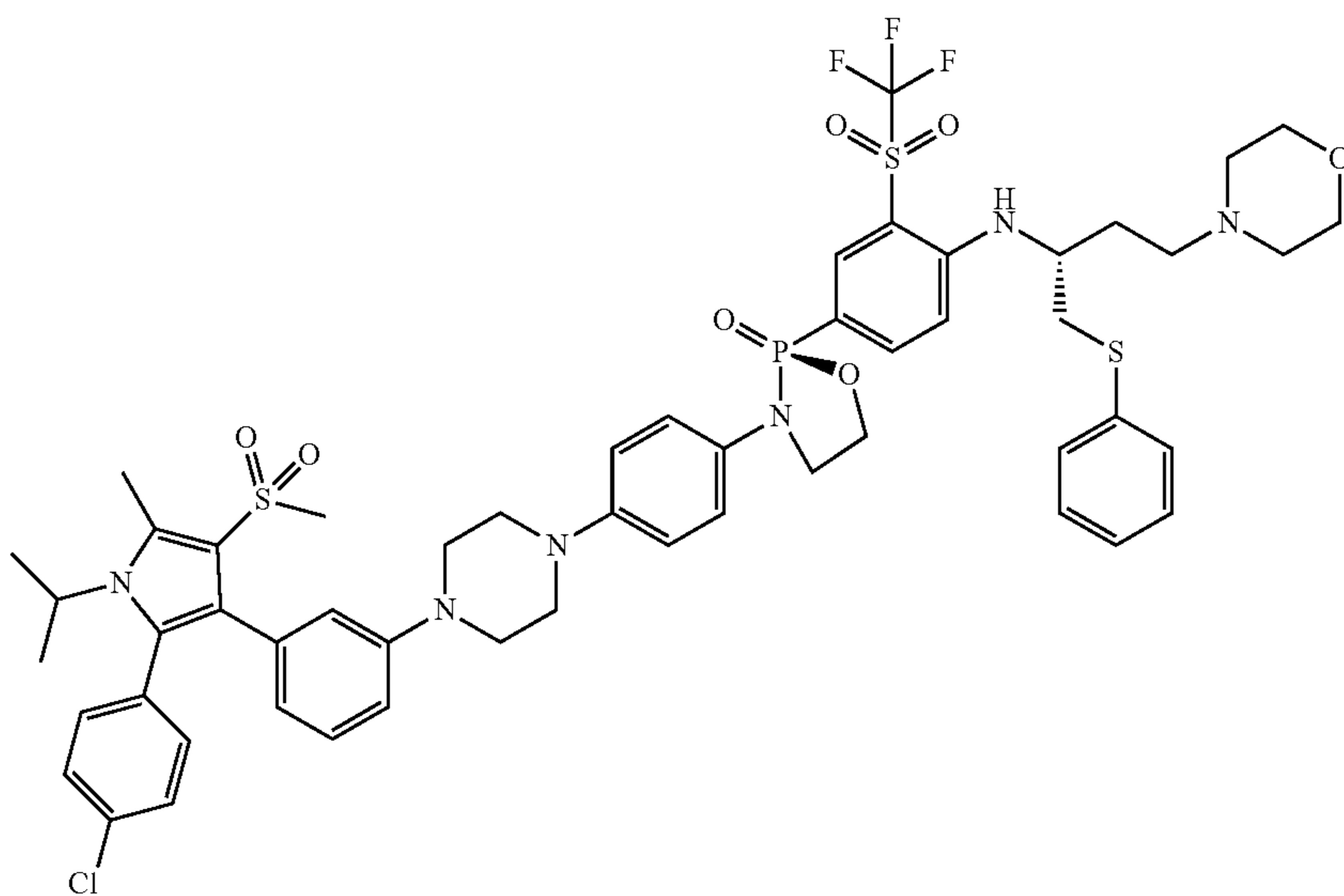
(S)-3-(4-(4-(3-(2-(4-chlorophenyl)-1-isopropyl-5-methyl-4-(methylsulfonyl)-1H-pyrrol-3-yl)phenyl)piperazin-1-yl)phenyl)-2-(4-(((R)-4-(morpholino-1-(phenylthio)butan-2-yl)amino)-3-((trifluoromethyl)sulfonyl)phenyl)-1,3,2-oxazaphospholidine 2-oxide
