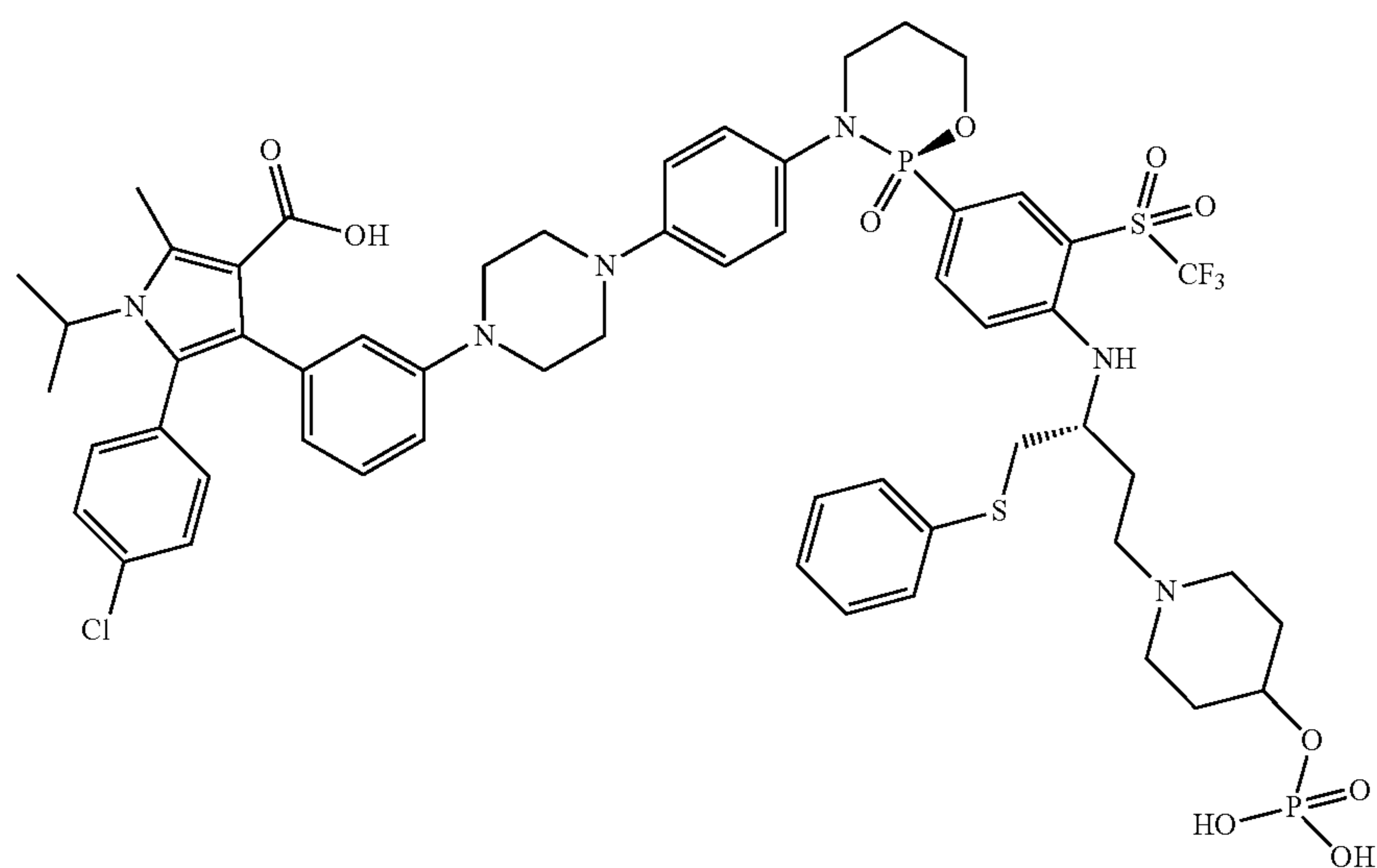
5-(4-chlorophenyl)-1-isopropyl-2-methyl-4-(3-(4-(4-((R)-2-oxido-2-(4-(((R)-1-(phenylthio)-4-(4-((phosphonooxy)piperidin-1-yl)butan-2-yl)amino)-3-((trifluoromethyl)sulfonyl)phenyl)-1,3,2-oxazaphosphinan-3-yl)phenyl)piperazin-1-yl)phenyl)-1H-pyrrole-3-carboxylic acid
