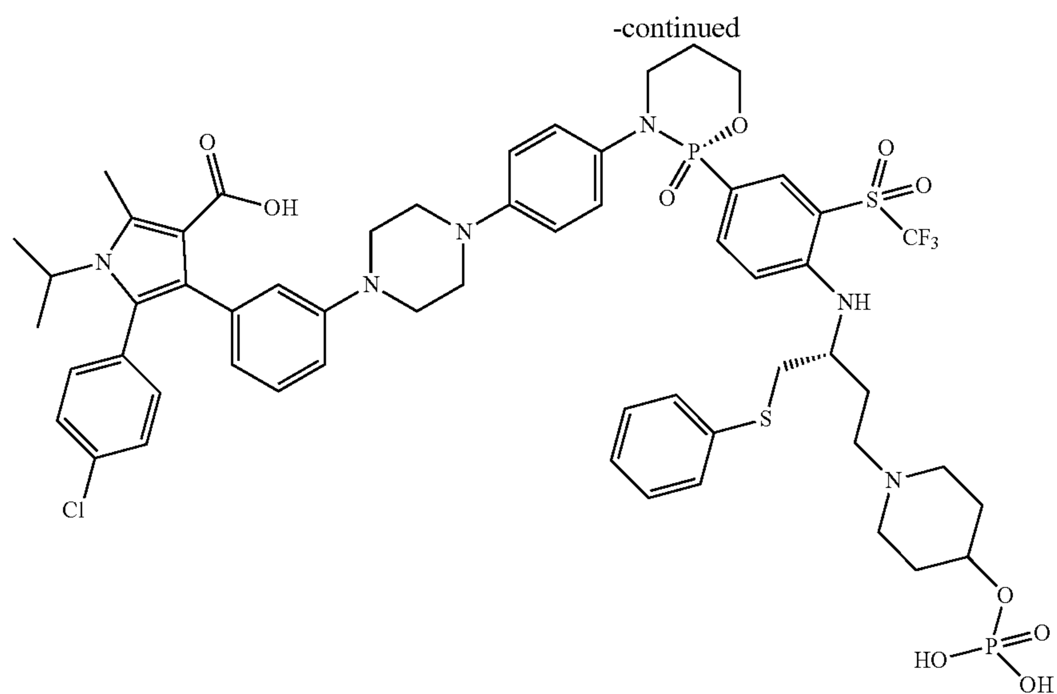
5-(4-chlorophenyl)-1-isopropyl-2-methyl-4-(3-(4-(4-((S)-2-oxido-2-(4-(((R)-1-(phenylthio)-4-(4-(phosphonooxy)piperidin-1-yl)butan-2-yl)amino)-3-((trifluoromethyl)sulfonyl)phenyl)-1,3,2-oxazaphosphinan-3-yl)phenyl)piperazin-1-yl)phenyl)-1H-pyrrole-3-carboxylic acid
