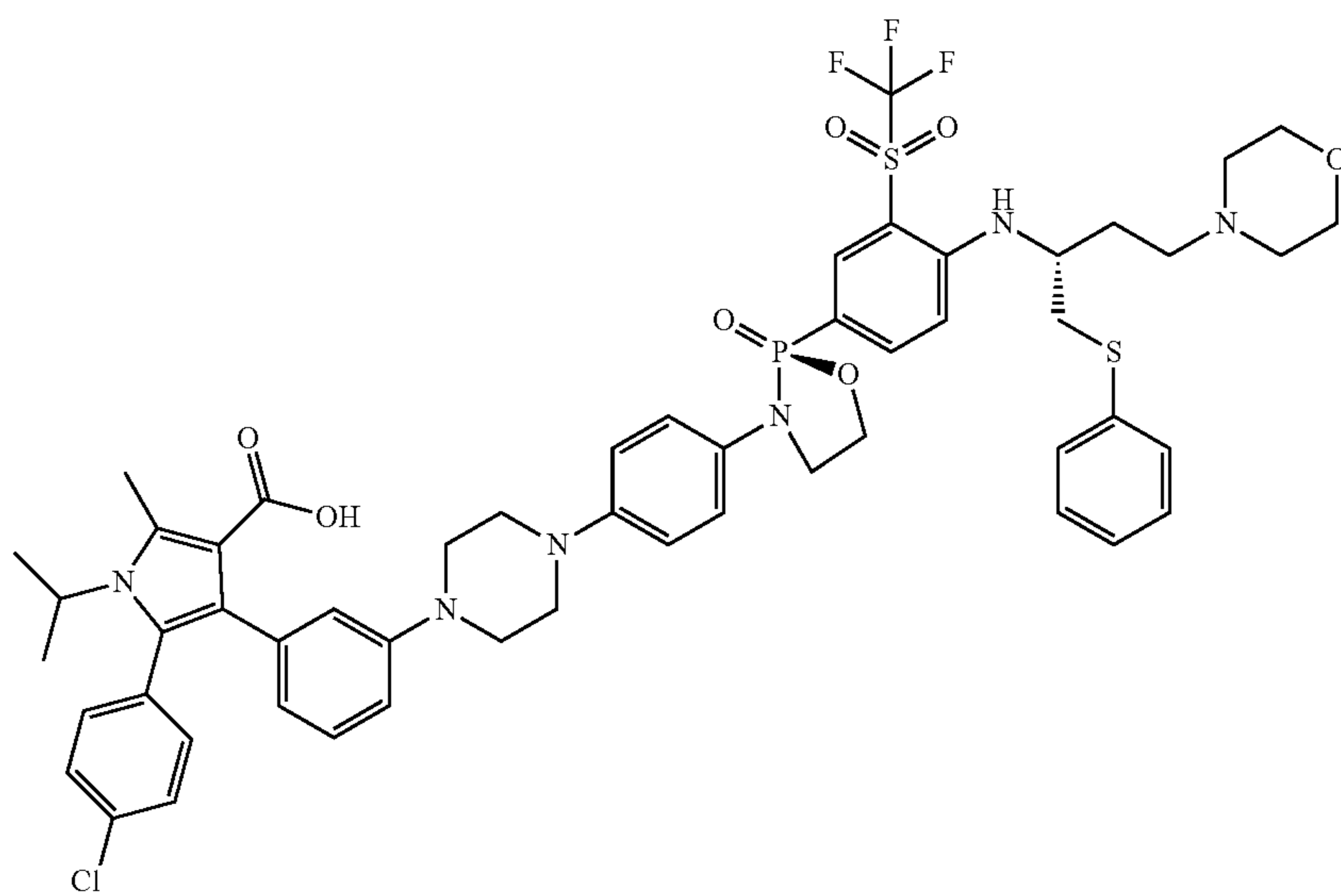
5-(4-chlorophenyl)-1-isopropyl-2-methyl-4-(3-(4-(4-((S)-2-(4-(((R)-4-morpholino-1-(phenylthio)butan-2-yl)amino)-3-((trifluoromethyl)sulfonyl)phenyl)-2-oxido-1,3,2-oxazaphospholidin-3-yl)phenyl)piperazin-1-yl)phenyl)-1H-pyrrole-3-carboxylic acid
