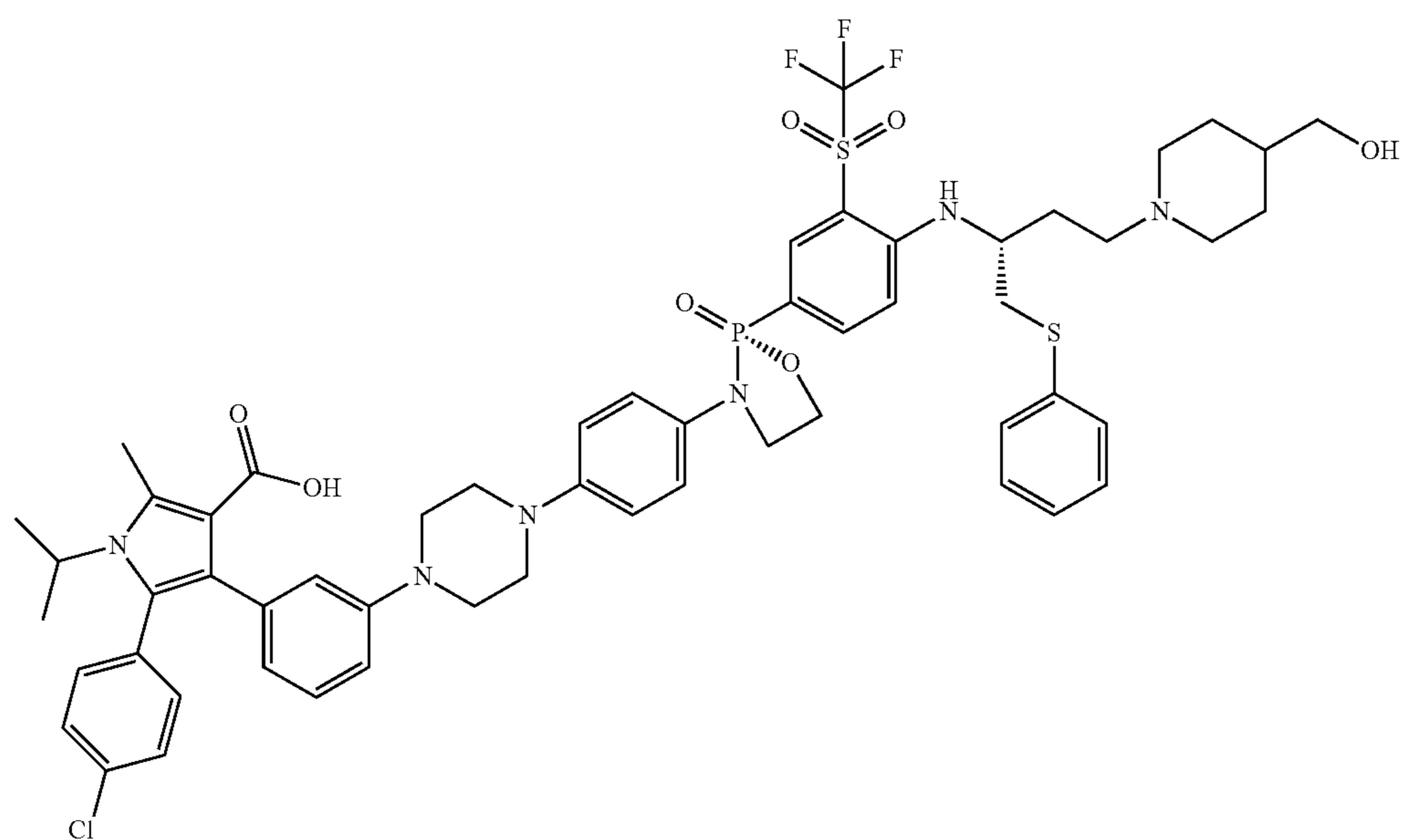
5-(4-chlorophenyl)-4-(3-(4-(4-((R)-2-(4-(((R)-4-(4-hydroxymethyl)piperidin-1-yl)-1-(phenylthio)butan-2-yl)amino)-3-((trifluoromethyl)sulfonyl)phenyl)-2-oxido-1,3,2-oxazaphospholidin-3-yl)phenyl)piperazin-1-yl)phenyl)-1-isopropyl-2-methyl-1H-pyrrole-3-carboxylic acid,
