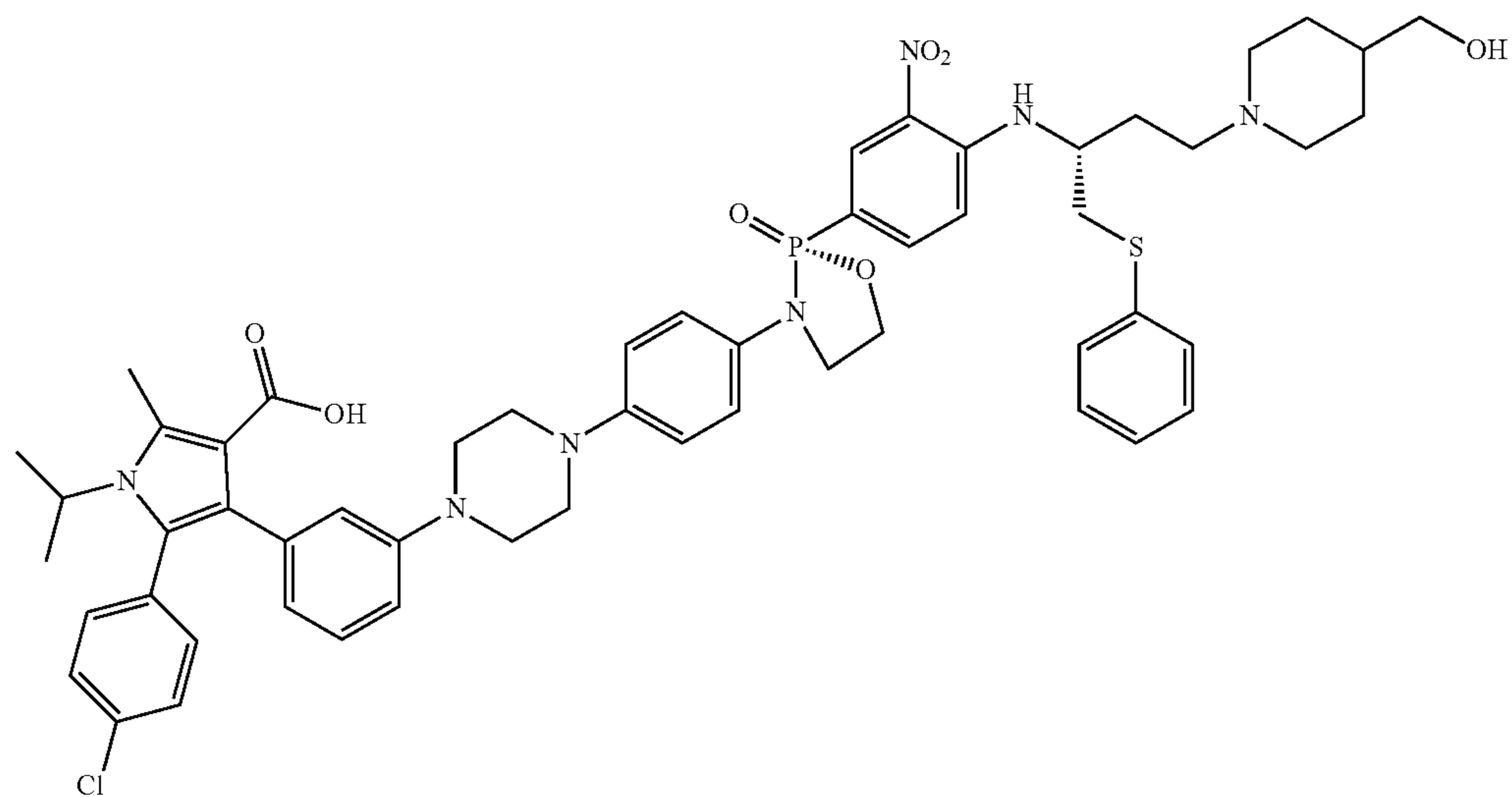
5-(4-chlorophenyl)-4-(3-(4-(4-((R)-2-(4-(((R)-4-(4-(hydroxymethyl)piperidin-1-yl)-1-(phenylthio)butan-2-yl)amino)-3-nitrophenyl)-2-oxido-1,3,2-oxazaphospholidin-3-yl)phenyl)piperazin-1-yl)phenyl)-1-isopropyl-2-methyl-1H-pyrrole-3-carboxylic acid
