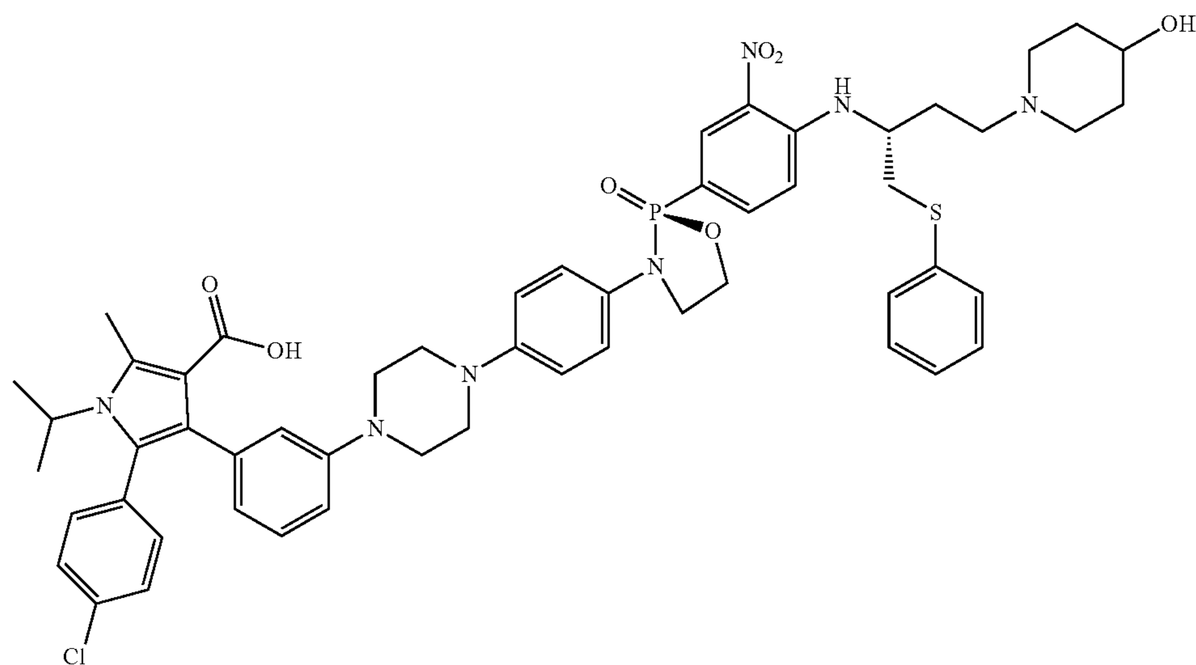
5-(4-chlorophenyl)-4-(3-(4-(4-((S)-2-(4-(((R)-4-(4-hydroxypiperidin-1-yl)-1-(phenylthio)butan-2-yl)amino)-3-nitrophenyl)-2-oxido-1,3,2-oxazaphospholidin-3-yl)phenyl)piperazin-1-yl)phenyl)-1-isopropyl-2-methyl-1H-pyrrole-3-carboxylic acid
