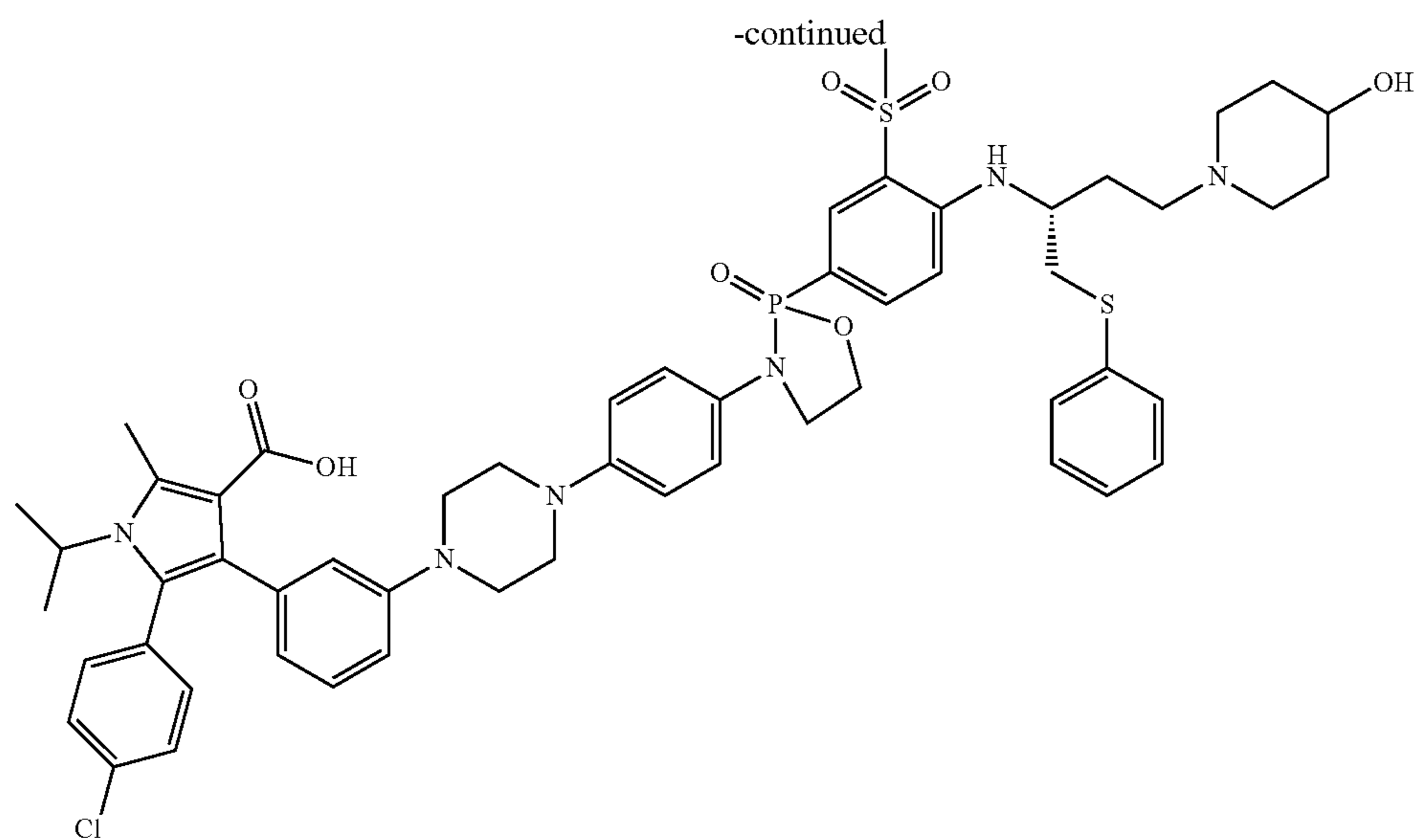
5-(4-chlorophenyl)-4-(3-(4-(4-(2-(4-(((R)-4-(4-hydroxypiperidin-1-yl)-1-(phenylthio)butan-2-yl)amino)-3-(methylsulfonyl)phenyl)-2-oxido-1,3,2-oxazaphospholidin-3-yl)phenyl)piperazin-1-yl)phenyl)-1-isopropyl-2-methyl-1H-pyrrole-3-carboxylic acid
