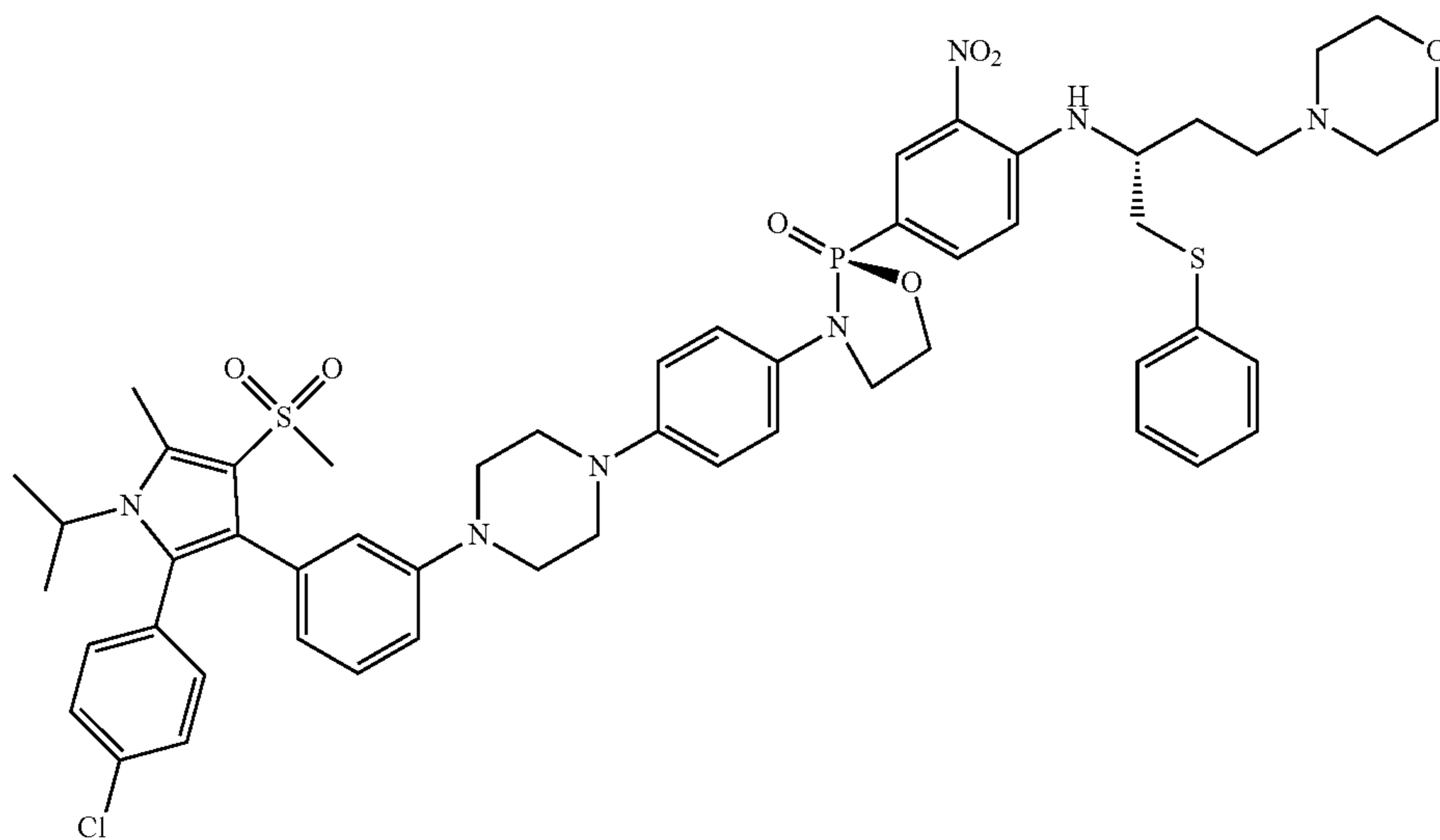
(S)-3-(4-(4-(3-(2-(4-chlorophenyl)-1-isopropyl-5-methyl-4-(methylsulfonyl)-1H-pyrrol-3-yl)phenyl)piperazin-1-yl)phenyl)-2-(4-(((S)-4-morpholino-1-(phenylthio)butan-2-yl)amino)-3-nitrophenyl)-1,3,2-oxazaphospholidine 2-oxide
