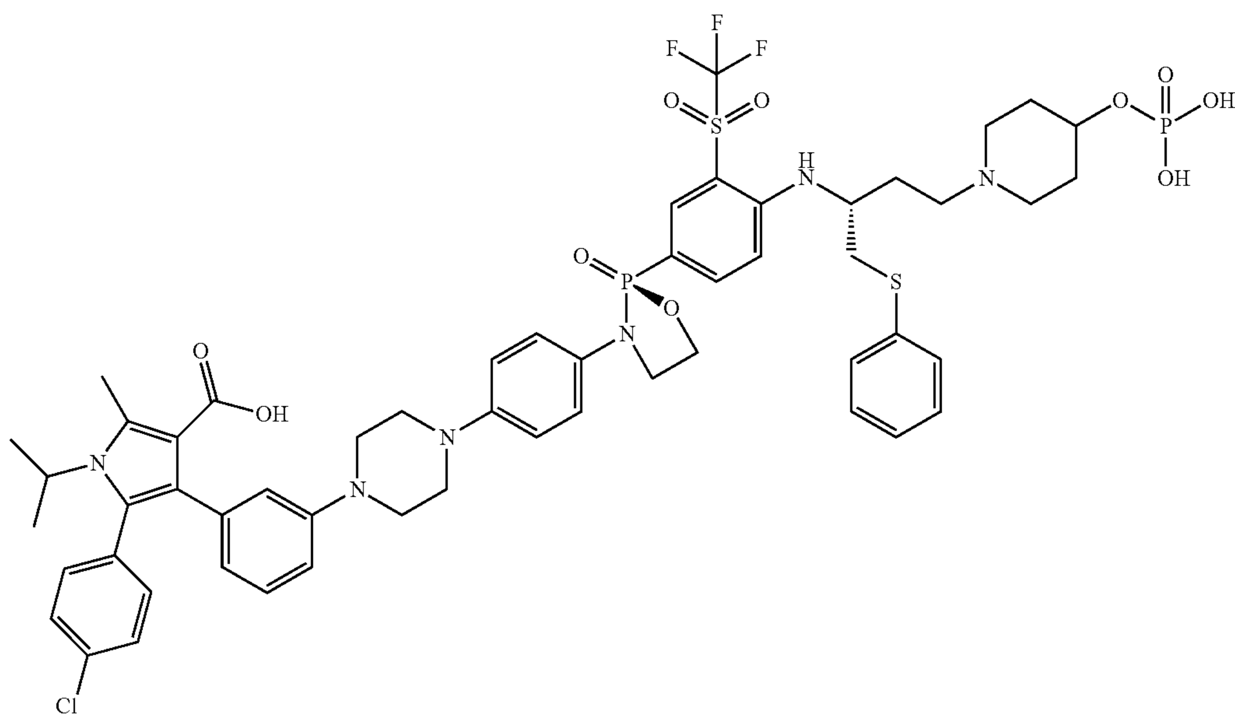
5-(4-chlorophenyl)-1-isopropyl-2-methyl-4-(3-(4-(4-((S)-2-oxido-2-(4-(((R)-1-(phenylthio)-4-(4-(phosphonoxy)piperidin-1-yl)butan-2-yl)amino)-3-((trifluoromethyl)sulfonyl)phenyl)-1,3,2-oxazaphospholidin-3-yl)phenyl)piperazin-1-yl)phenyl)-1H-pyrrole-3-carboxylic acid,
