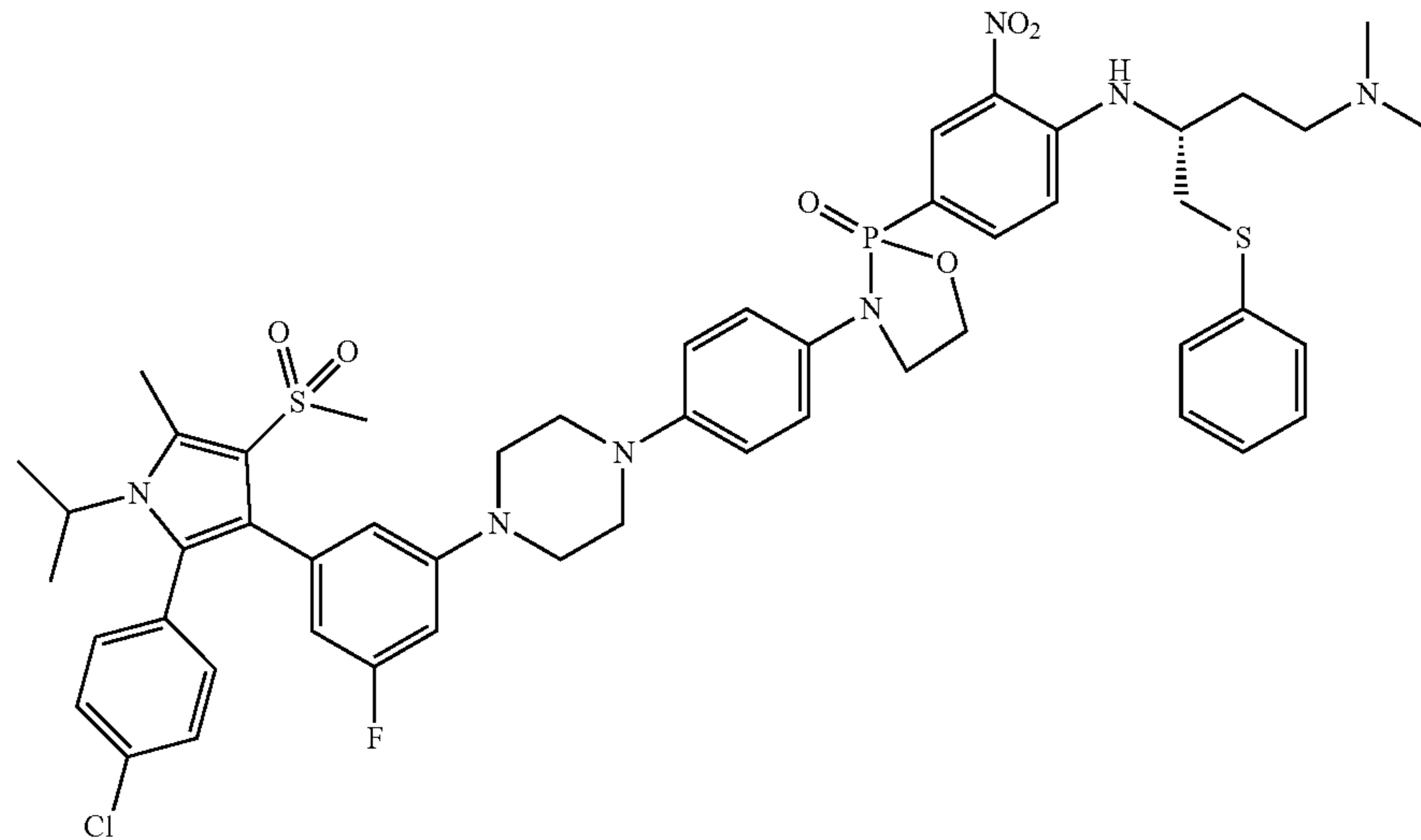
3-(4-(4-(3-(2-(4-chlorophenyl)-1-isopropyl-5-methyl-4-(methylsulfonyl)-1H-pyrrol-3-yl)-5-fluorophenyl)piperazin-1-yl)phenyl)-2-(4-(((R)-4-(dimethylamino)-1-(phenylthio)butan-2-yl)amino)-3-nitrophenyl)-1,3,2-oxazaphospholidine 2-oxide
