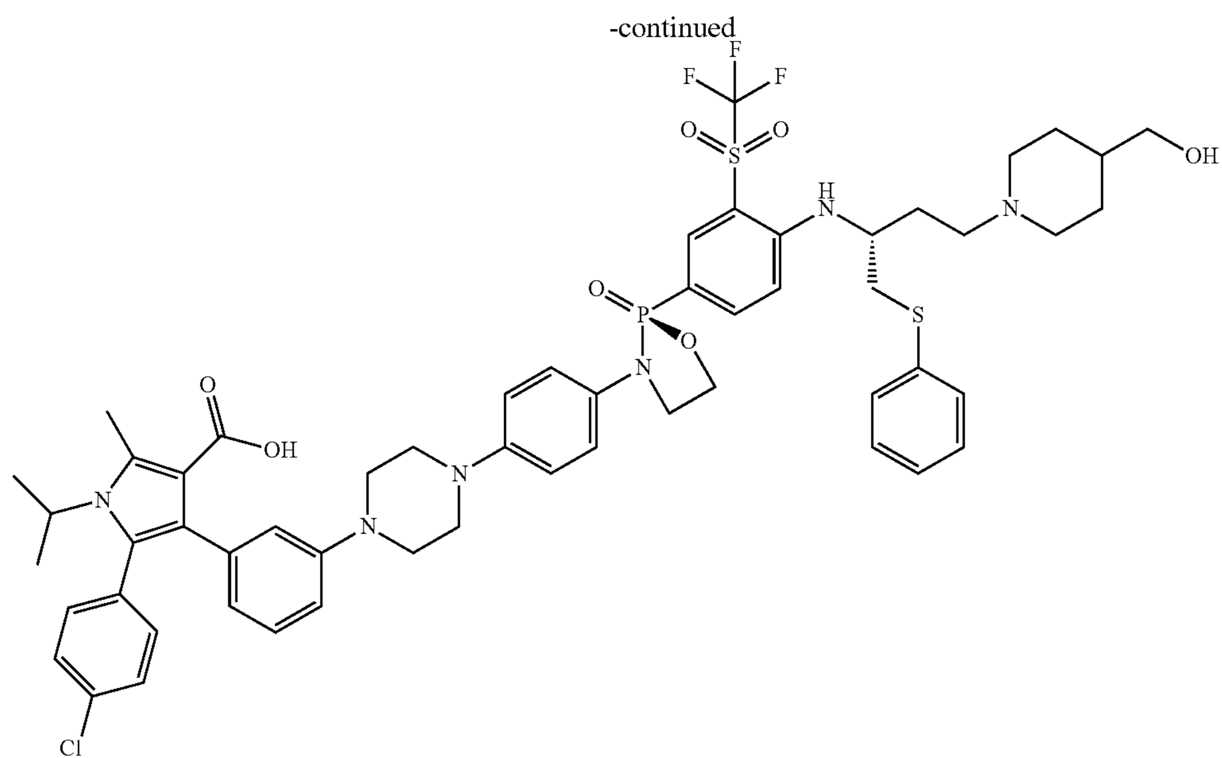
5-(4-chlorophenyl)-4-(3-(4-(4-((S)-2-(4-((R)-4-(4-(hydroxymethyl)piperidin-1-yl)-1-(phenylthio)butan-2-yl)amino)-3-((trifluoromethyl)sulfonyl)phenyl)-2-oxido-1,3,2-oxazaphospholidin-3-yl)phenyl)piperazin-1-yl)phenyl)-1-isopropyl-2-methyl-1H-pyrrole-3-carboxylic acid,
