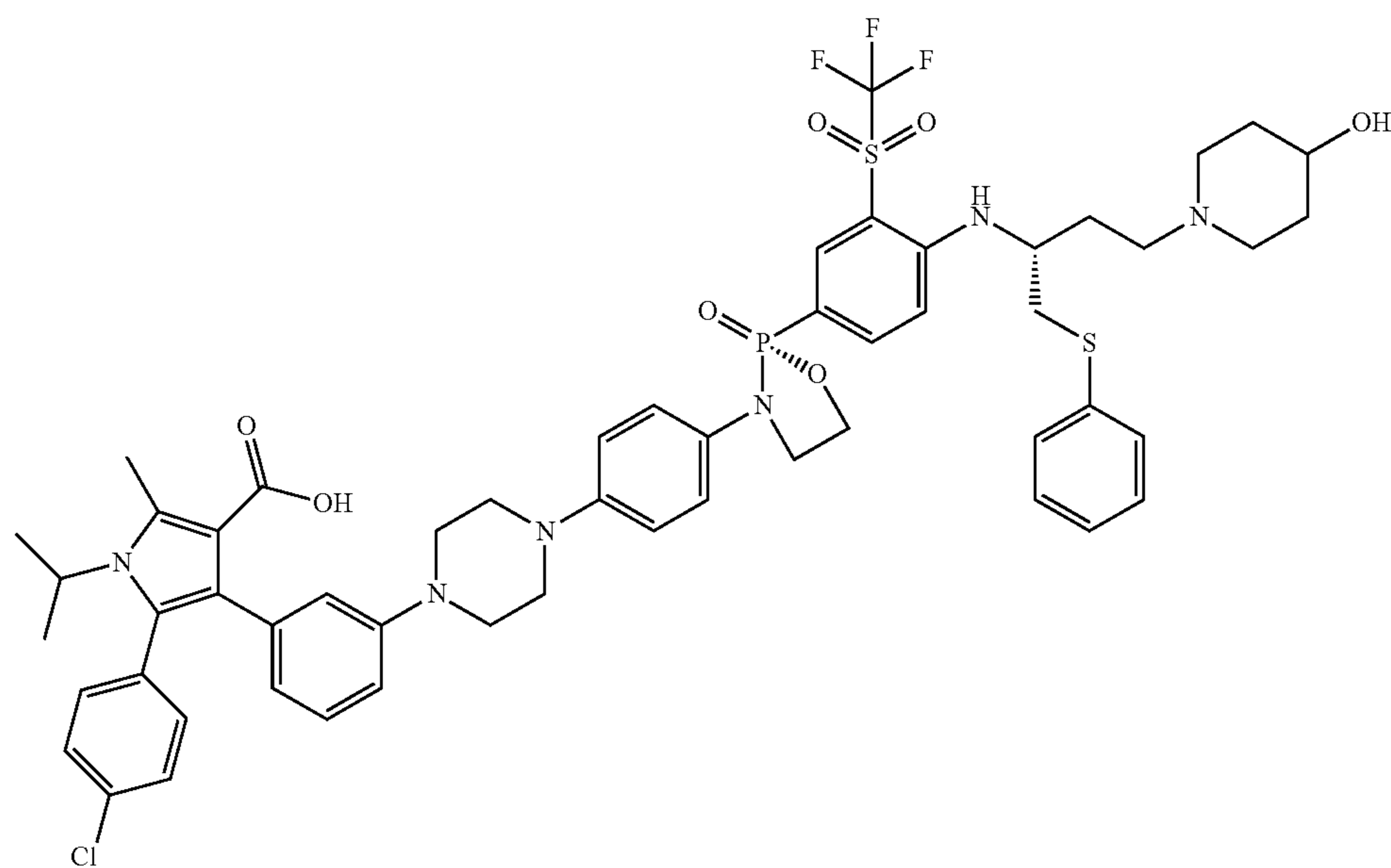
5-(4-chlorophenyl)-4-(3-(4-(4-((R)-2-(4-(((R)-4-(4-hydroxypiperidin-1-yl)-1-(phenylthio)butan-2-yl)amino)-3-(trifluoromethyl)sulfonyl)phenyl)-2-oxido-1,3,2-oxazaphospholidin-3-yl)phenyl)piperazin-1-yl)phenyl)-1-isopropyl-2-methyl-1H-pyrrole-3-carboxylic acid,
