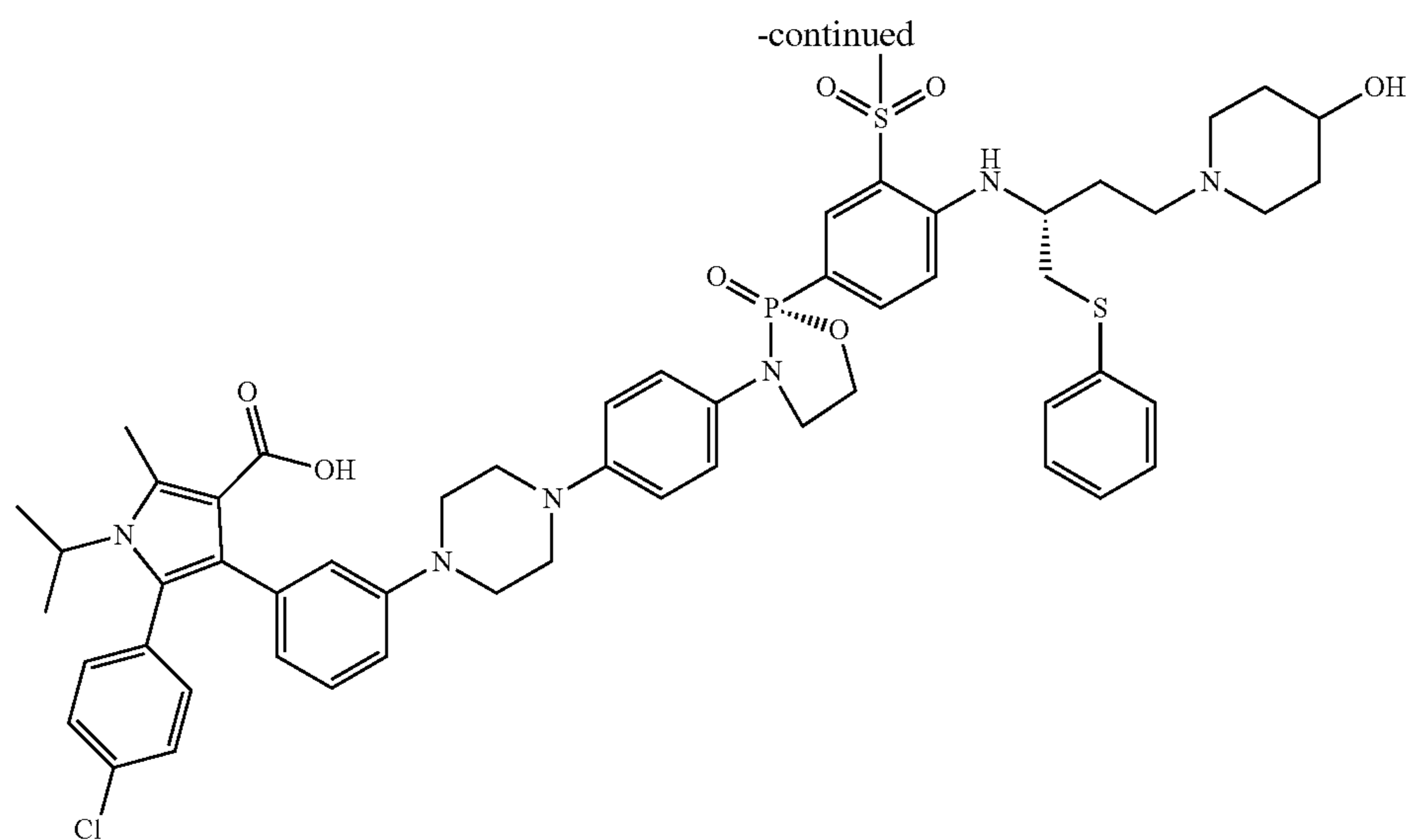
5-(4-chlorophenyl)-4-(3-(4-(4-((R)-2-(4-(((R)-4-(4-(hydroxypiperidin-1-yl)-1-(phenylthio)butan-2-yl)amino)-3-(methylsulfonyl)phenyl)-2-oxido-1,3,2-oxazaphospholidin-3-yl)phenyl)piperazin-1-yl)phenyl)-1-isopropyl-2-methyl-1H-pyrrole-3-carboxylic acid
