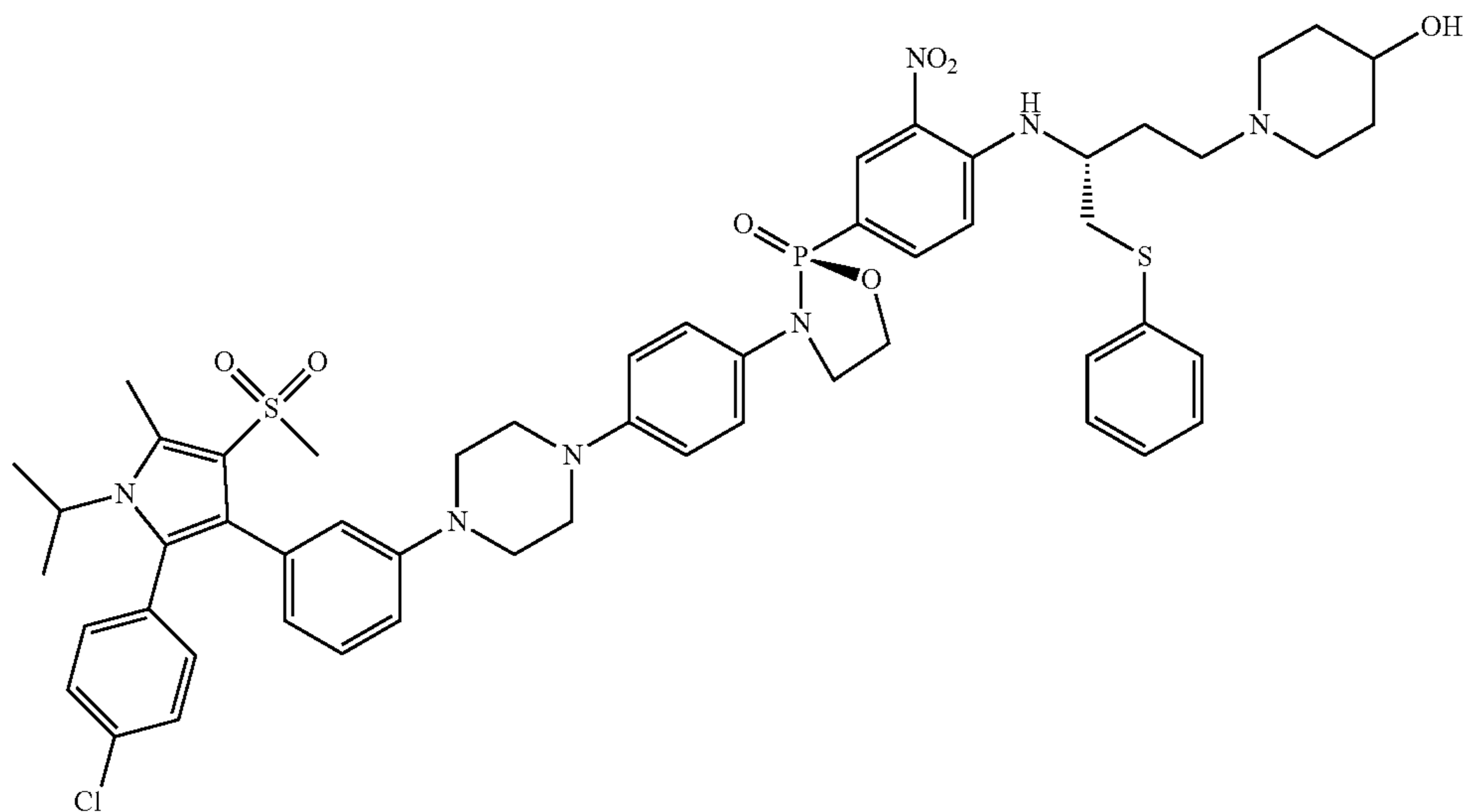
(S)-3-(4-(4-(3-(2-(4-chlorophenyl)-1-isopropyl-5-methyl-4-(methylsulfonyl)-1H-pyrrol-3-yl)-phenyl)piperazin-1-yl)phenyl)-2-(4-(((R)-4-(4-hydroxypiperidin-1-yl)-1-(phenylthio)butan-2-yl)amino)-3-nitrophenyl)-1,3,2-oxazaphospholidine 2-oxide
