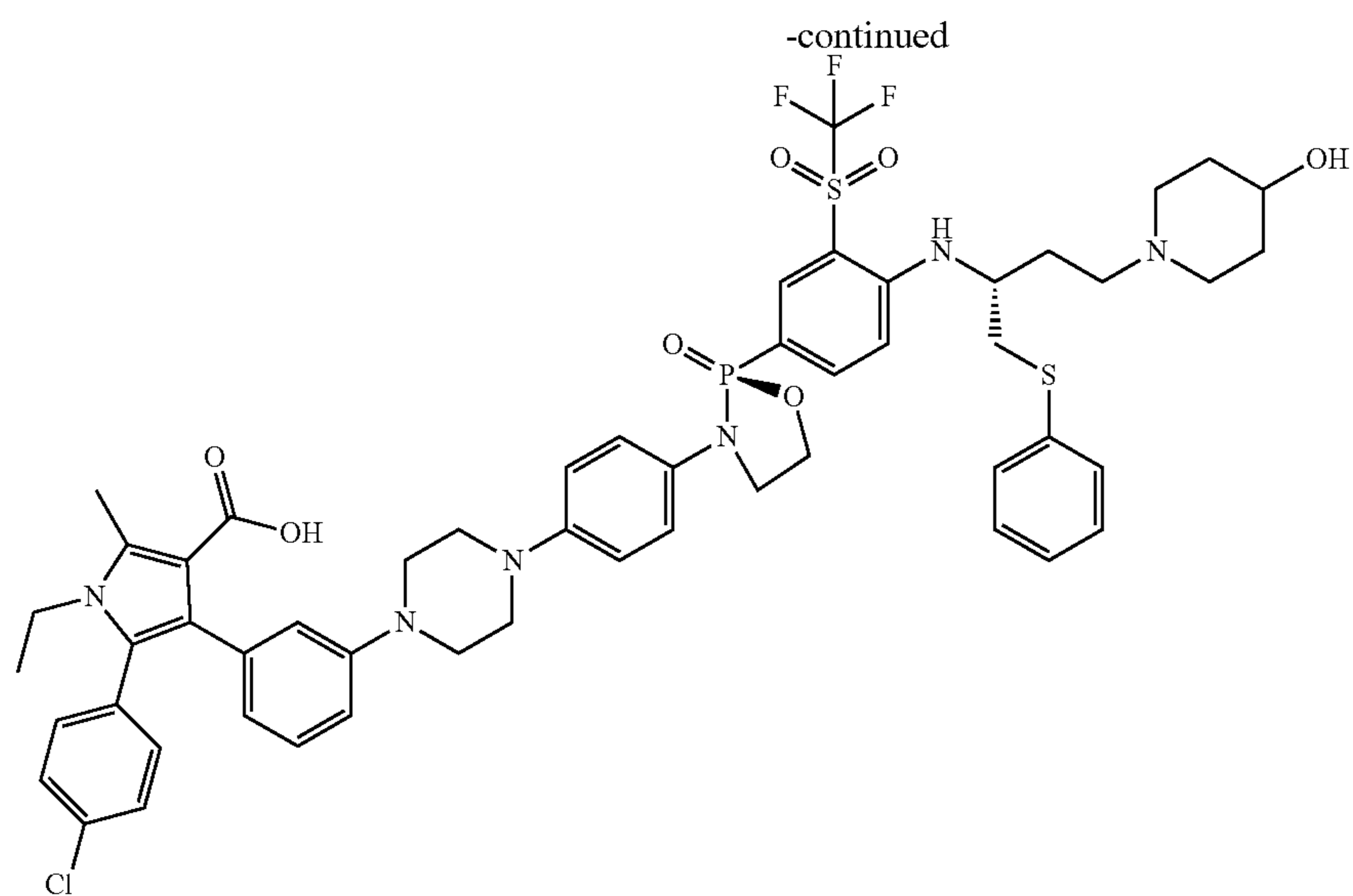
5-(4-chlorophenyl)-1-ethyl-4-(3-(4-(4-((S)-2-(4-(((R)-4-(4-hydroxypiperidin-1-yl)-1-(phenylthio)butan-2-yl)amino)-3-((trifluoromethyl)sulfonyl)phenyl)-2-oxido-1,3,2-oxazaphospholidin-3-yl)phenyl)piperazin-1-yl)phenyl)-2-methyl-1H-pyrrole-3-carboxylic acid
