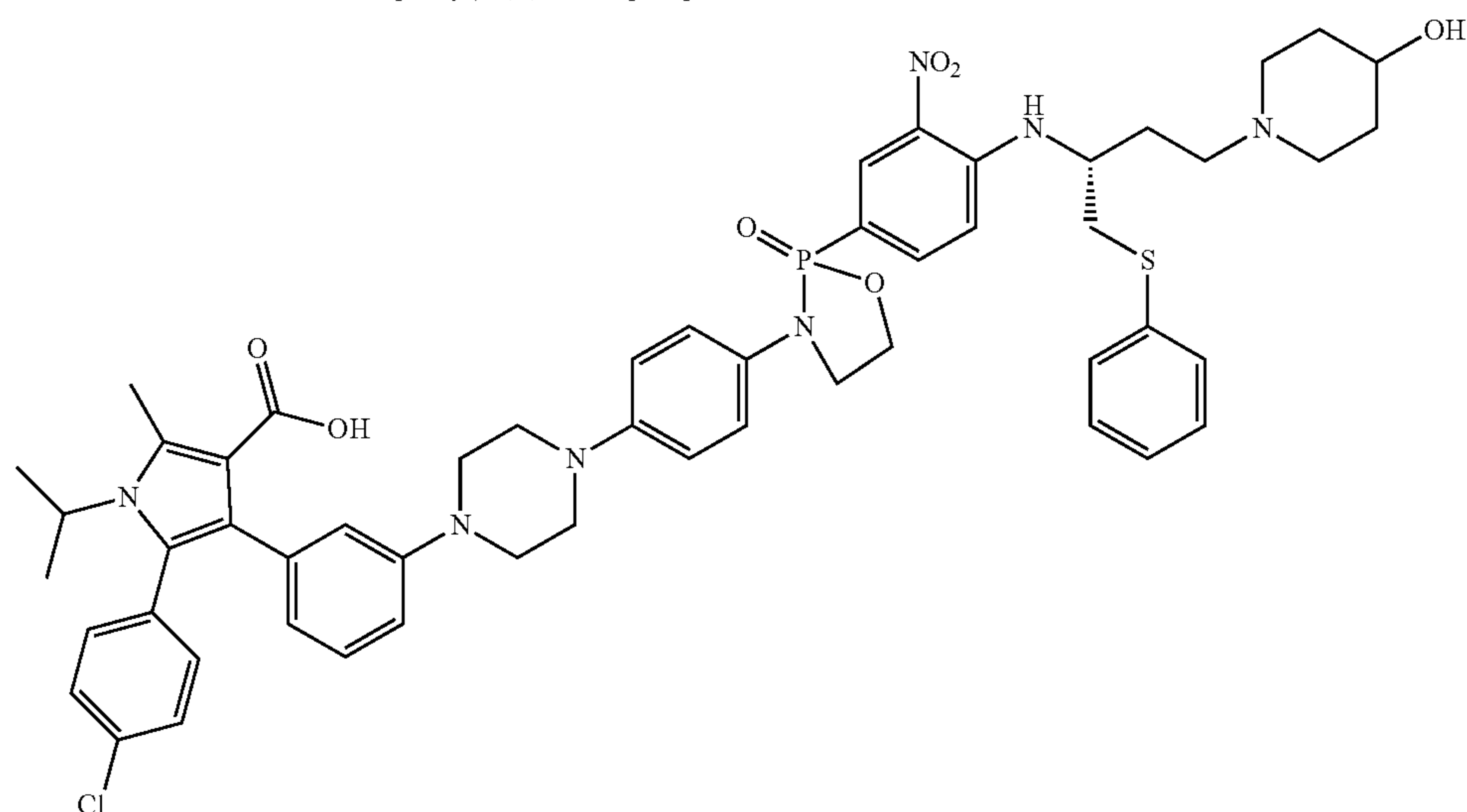
3-(4-(4-(3-(2-(4-chlorophenyl)-1-isopropyl-5-methyl-4-(methylsulfonyl)-1H-pyrrol-3-yl)-5-fluorophenyl)piperazin-1-yl)phenyl)-2-(4-(((R)-4-(dimethylamino)-1-(phenylthio)butan-2-yl)amino)-3-nitrophenyl)-1,3,2-oxazaphospholidine 2-oxide
