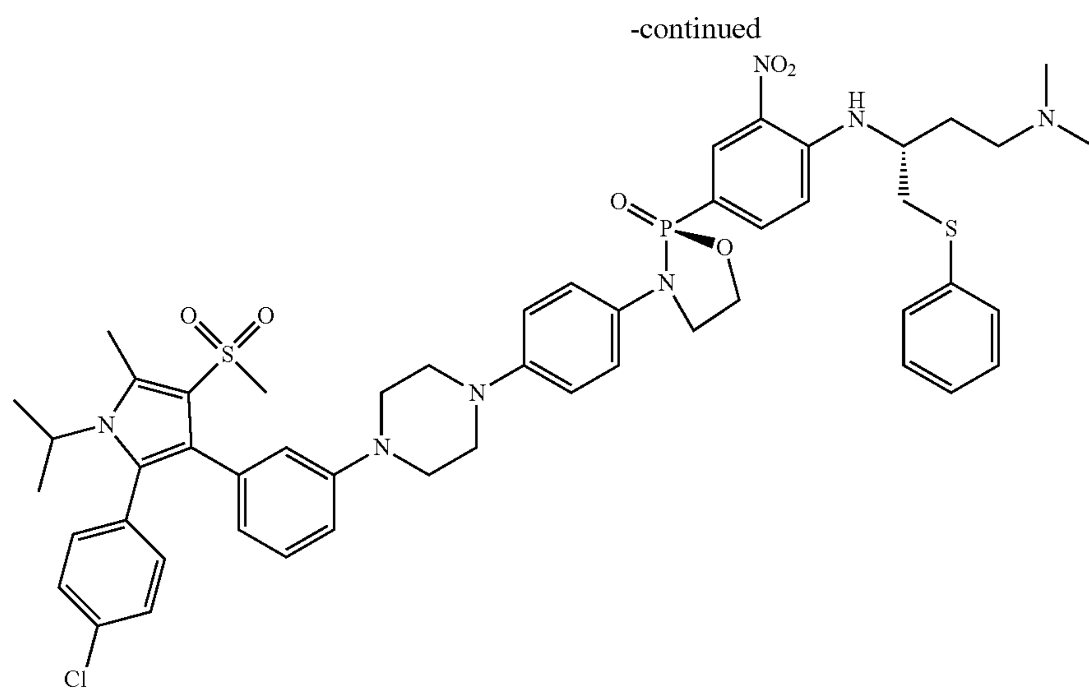
(S)-3-(4-(4-(3-(2-(4-chlorophenyl)-1-isopropyl-5-methyl-4-(methylsulfonyl)-1H-pyrrol-3-yl)phenyl)piperazin-1-yl)phenyl)-2-(4-(((R)-4-(dimethylamino)-1-(phenylthio)butan-2-yl)amino)-3-nitrophenyl)-1,3,2-oxazaphospholidine 2-oxide
