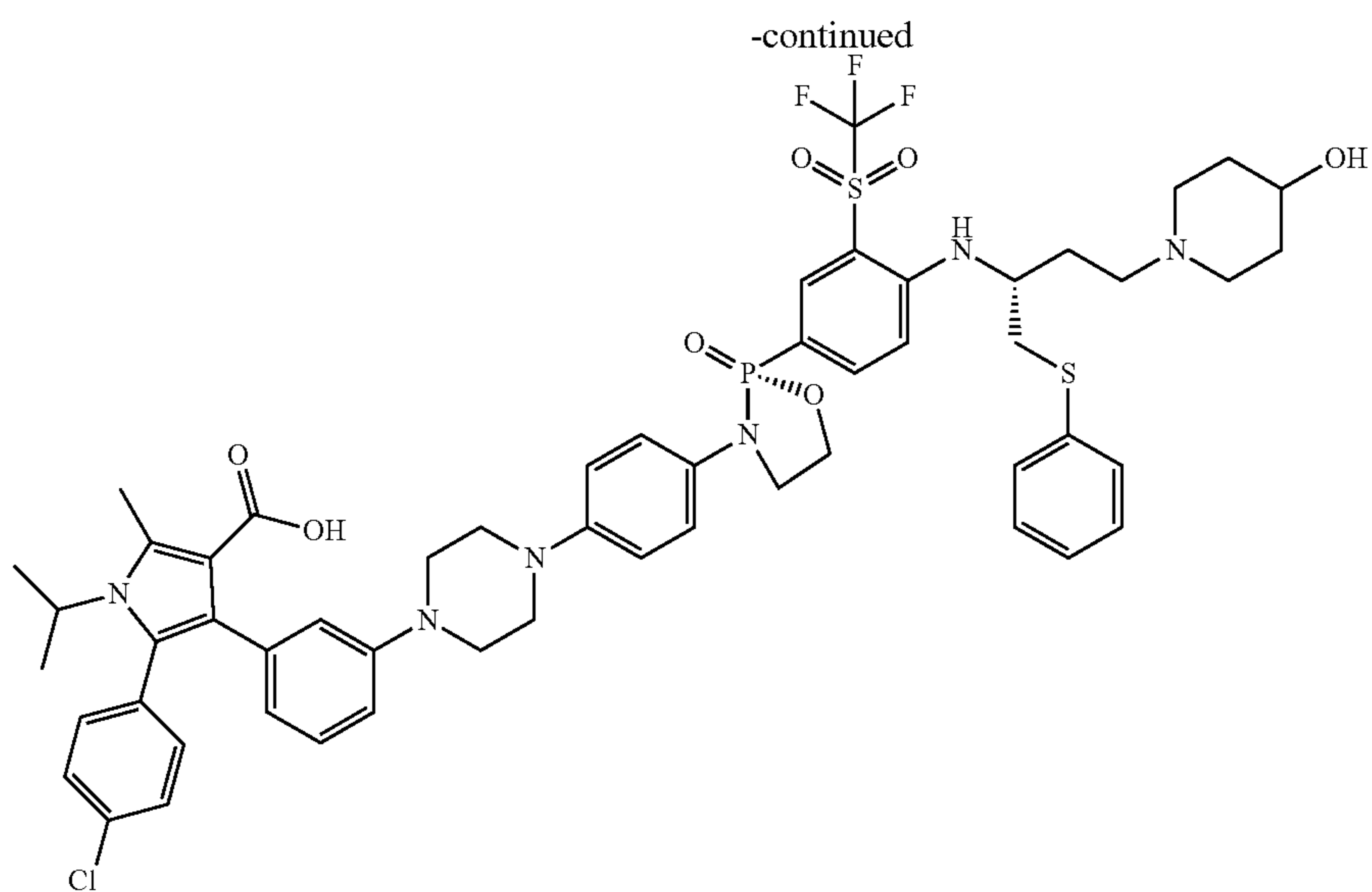
5-(4-chlorophenyl)-4-(3-(4-(4-((R)-2-(4-((R)-4-((R)-4-(4-hydroxypiperidin-1-yl)-1-(phenylthio)butan-2-yl)amino)-3-((trifluoromethyl)sulfonyl)phenyl)-2-oxido-1,3,2-oxazaphospholidin-3-yl)phenyl)piperazin-1-yl)phenyl)-1-isopropyl-2-methyl-1H-pyrrole-3-carboxylic acid
