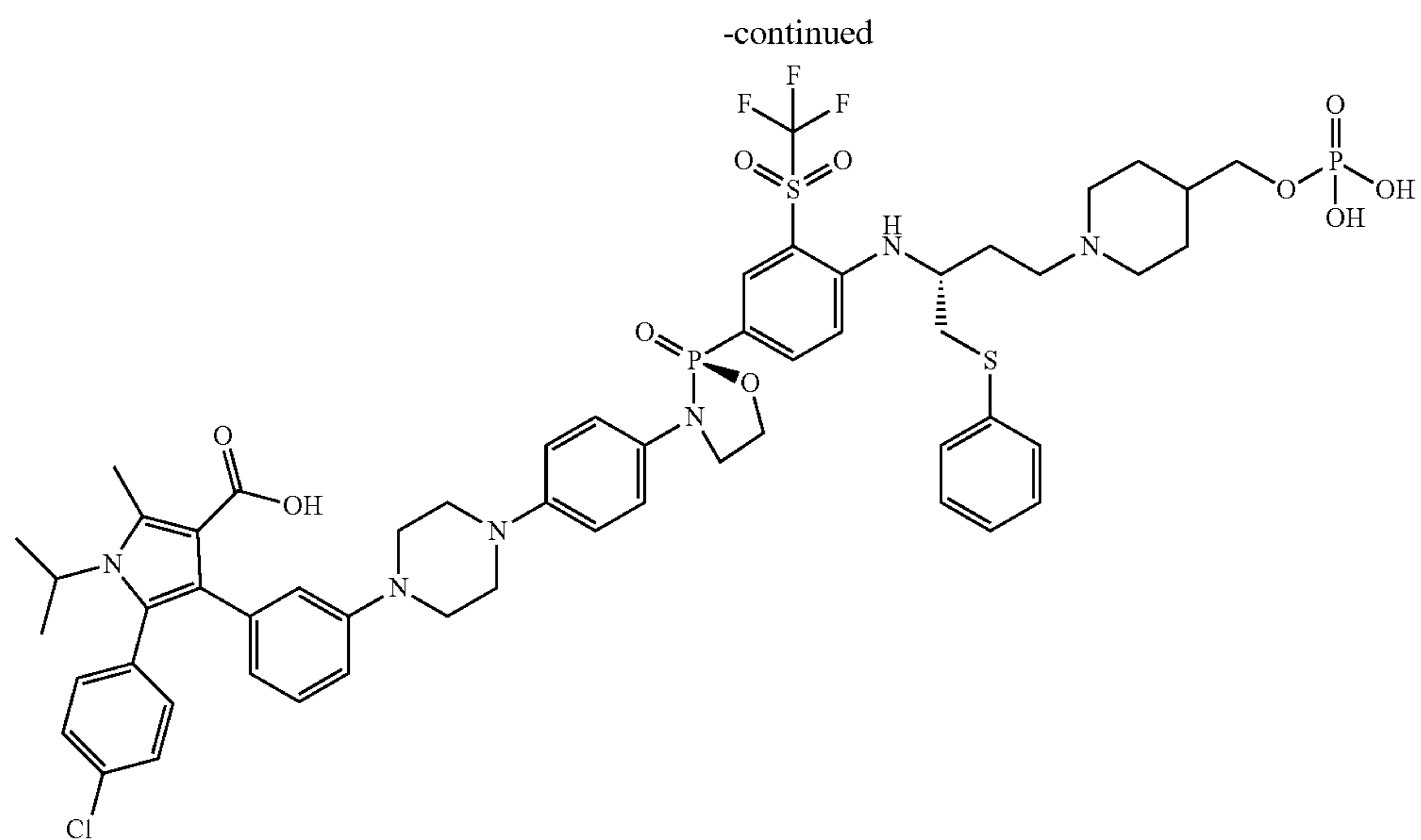
5-(4-chlorophenyl)-1-isopropyl-2-methyl-4-(3-(4-(4-((S)-2-oxido-2-(4-(((R)-1-(phenylthio)-4-(4-((phosphonooxy)methyl)piperidin-1-yl)butan-2-yl)amino)-3-((trifluoromethyl)sulfonyl)phenyl)-1,3,2-oxazaphospholidin-3-yl)phenyl)piperazin-1-yl)phenyl)-1H-pyrrole-3-carboxylic acid
