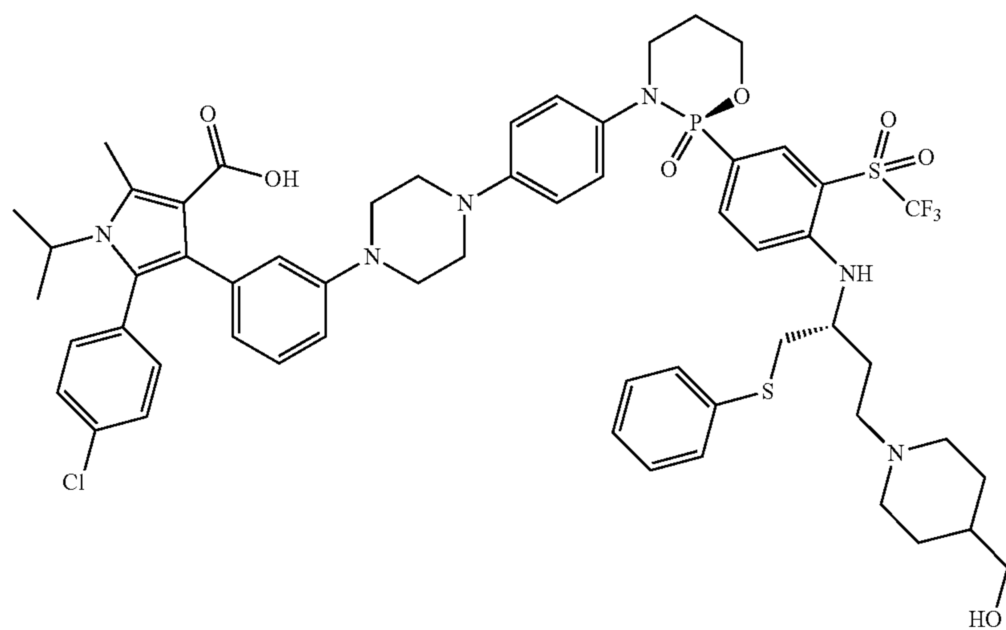
5-(4-chlorophenyl)-4-(3-(4-(4-((R)-2-(4-((R)-4-(4-(hydroxymethyl)piperidin-1-yl)-1-(phenylthio)butan-2-yl)amino)-3-((trifluoromethyl)sulfonyl)phenyl)-2-oxido-1,3,2-oxazaphosphinan-3-yl)phenyl)piperazin-1-yl)phenyl)-1-isopropyl-2-methyl-1H-pyrrole-3-carboxylic acid
