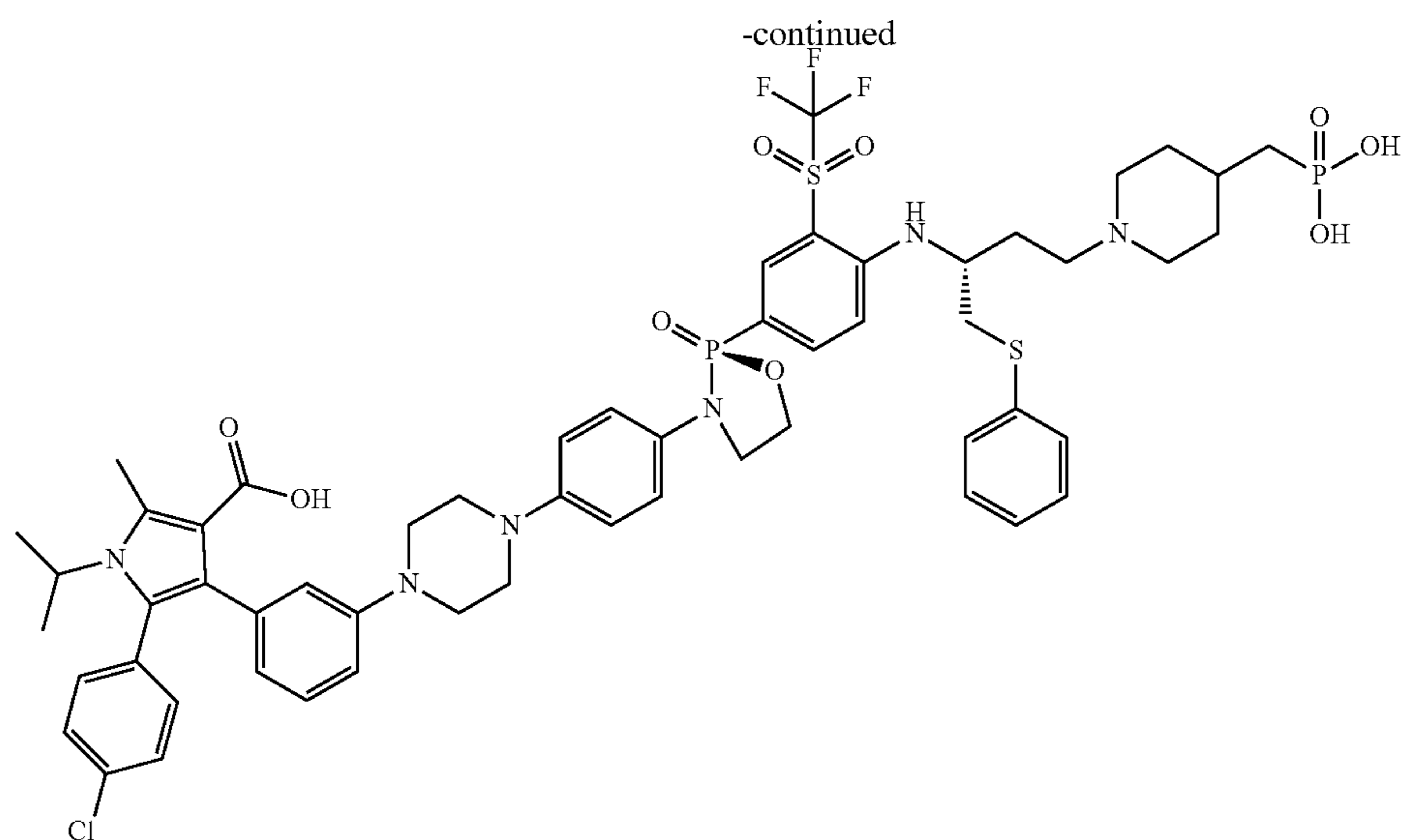
5-(4-chlorophenyl)-1-isopropyl-2-methyl-4-(3-(4-(4-((S)-2-oxido-2-(4-((R)-1-(phenylthio)-4-(4-(phosphonomethyl)piperidin-1-yl)butan-2-yl)amino)-3-((trifluoromethyl)sulfonyl)phenyl)-1,3,2-oxazaphospholidin-3-yl)phenyl)piperazin-1-yl)phenyl)-1H-pyrrole-3-carboxylic acid
