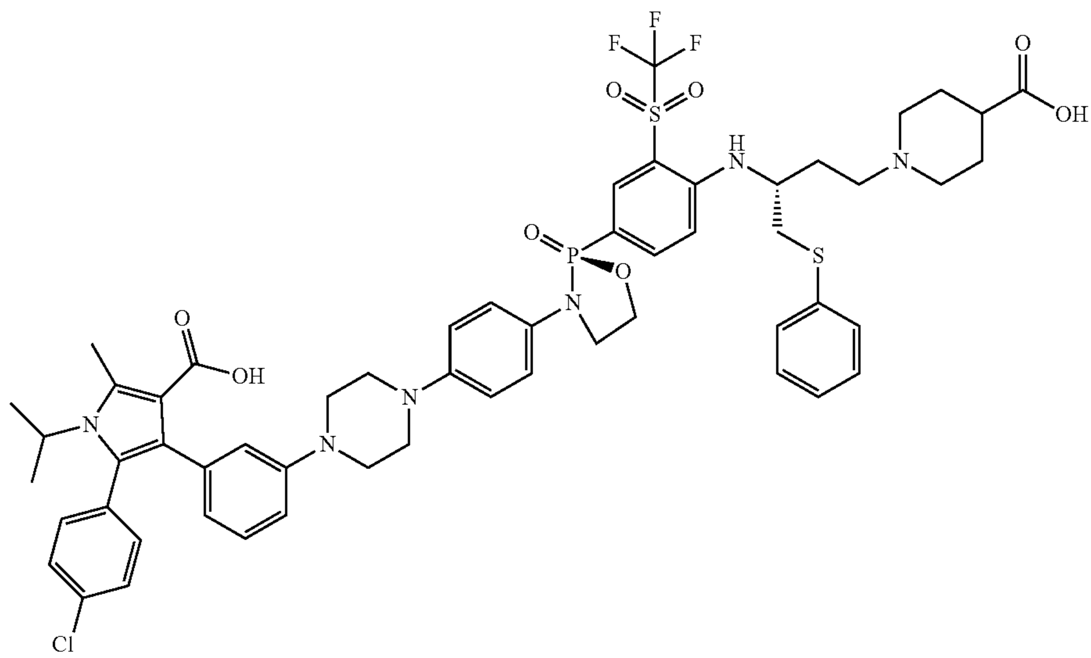
1-((R)-3-((4-((S)-3-(4-(4-(3-(4-carboxy-2-(4-chlorophenyl)-1-isopropyl-5-methyl-1H-pyrrol-3-yl)phenyl)piperazin-1-yl)phenyl)-2-oxido-1,3,2-oxazaphospholidin-2-yl)-2-((trifluoromethyl)sulfonyl)phenyl)amino)-4-(phenylthio)butyl)piperidine-4-carboxylic acid
