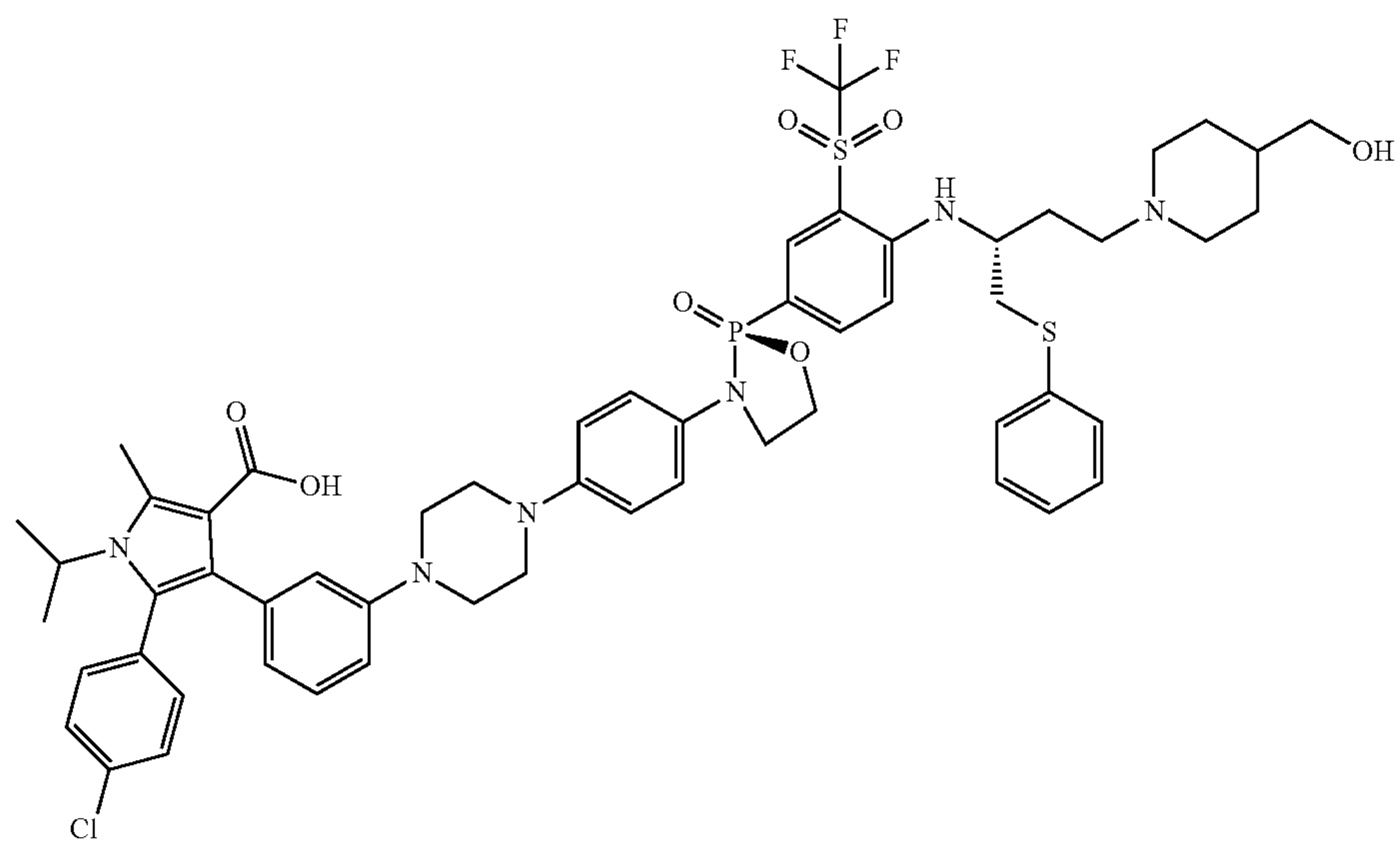
5-(4-chlorophenyl)-4-(3-(4-(4-((S)-2-(4-((R)-4-((R)-4-(4-hydroxypiperidin-1-yl)-1-(phenylthio)butan-2-yl)amino)-3-(trifluoromethyl)sulfonyl)phenyl)-2-oxido-1,3,2-oxazaphospholidin-3-yl)phenyl)piperazin-1-yl)phenyl)-1-isopropyl-2-methyl-1H-pyrrole-3-carboxylic acid
