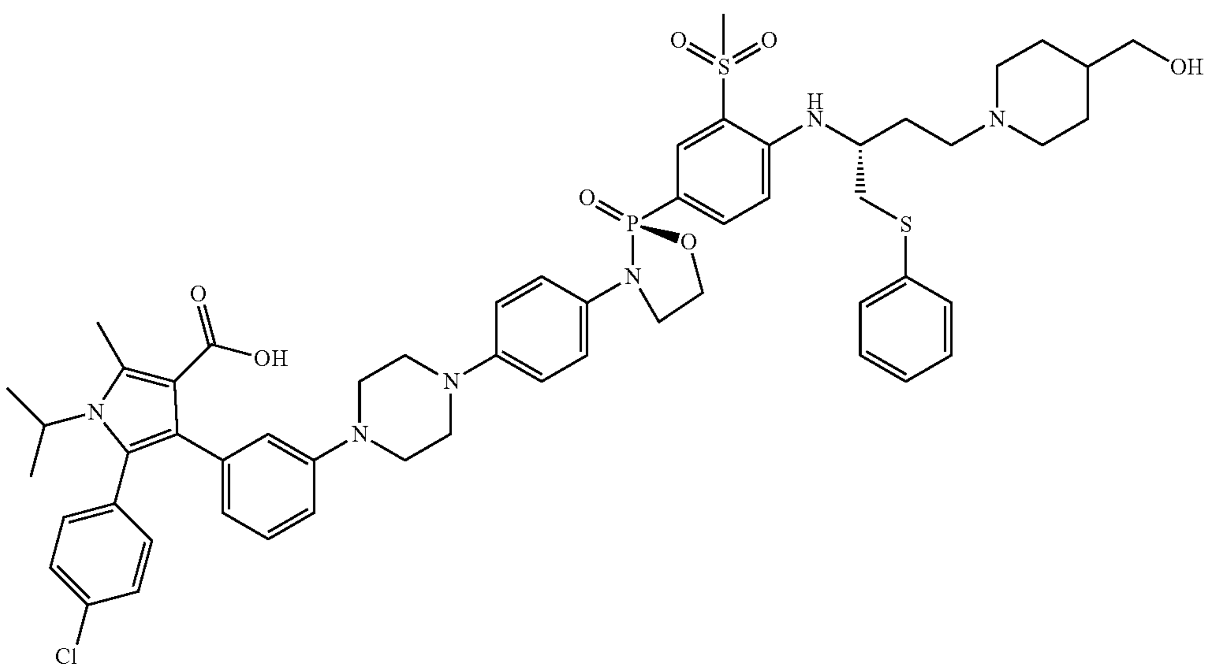
5-(4-chlorophenyl)-4-(3-(4-(4-((S)-2-(4-(((R)-4-(4-(hydroxymethyl)piperidin-1-yl)-1-(phenylthio)butan-2-yl)amino)-3-(methylsulfonyl)phenyl)-2-oxido-1,3,2-oxazaphospholidin-3-yl)phenyl)piperazin-1-yl)phenyl)-1-isopropyl-2-methyl-1H-pyrrole-3-carboxylic acid
