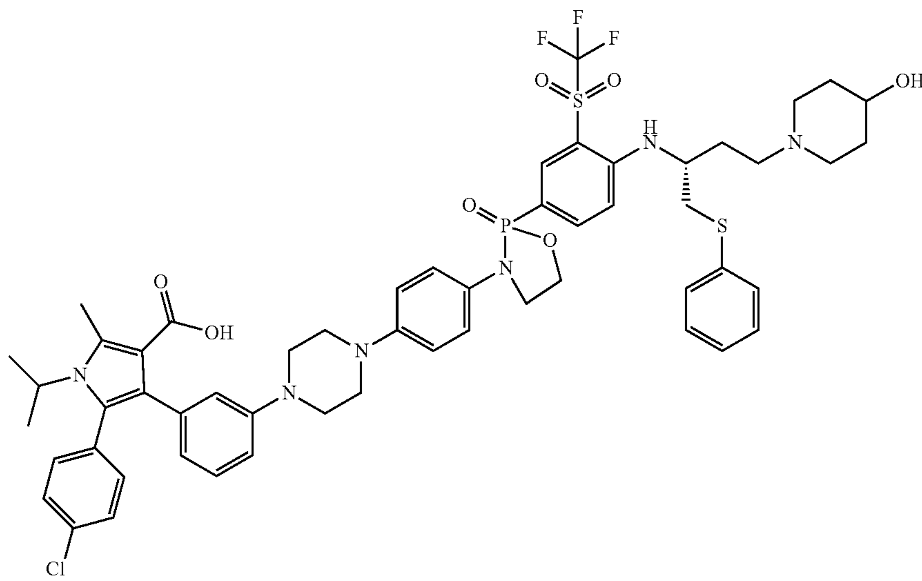
5-(4-chlorophenyl)-4-(3-(4-(4-(2-(4-((R)-4-(4-hydroxypiperidin-1-yl)-1-(phenylthio)butan-2-yl)amino-3-((trifluoromethyl)sulfonyl)phenyl)-2-oxido-1,3,2-oxazaphospholidin-3-yl)phenyl)piperazin-1-yl)phenyl)-1-isopropyl-2-methyl-1H-pyrrole-3-carboxylic acid
