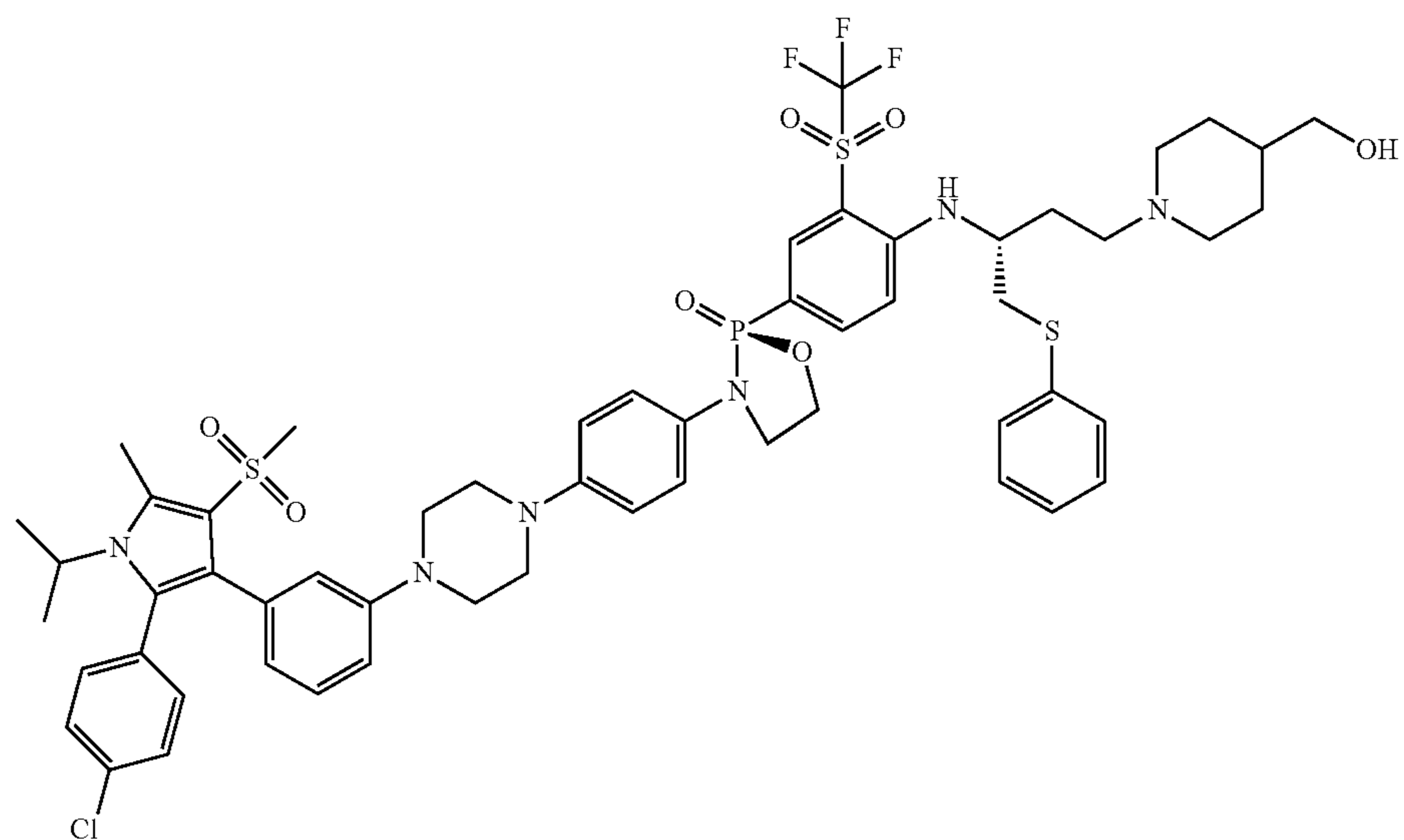
(S)-3-(4-(4-(3-(2-(4-chlorophenyl)-1-isopropyl-5-methyl-4-(methylsulfonyl)-1H-pyrrol-3-yl)phenyl)piperazin-1-yl)phenyl)-2-(4-(((R)-4-(4-(hydroxymethyl)piperidin-1-yl)-1-(phenylthio)butan-2-yl)amino)-3-((trifluoromethyl)sulfonyl)phenyl)-1,3,2-oxazaphospholidine 2-oxide
