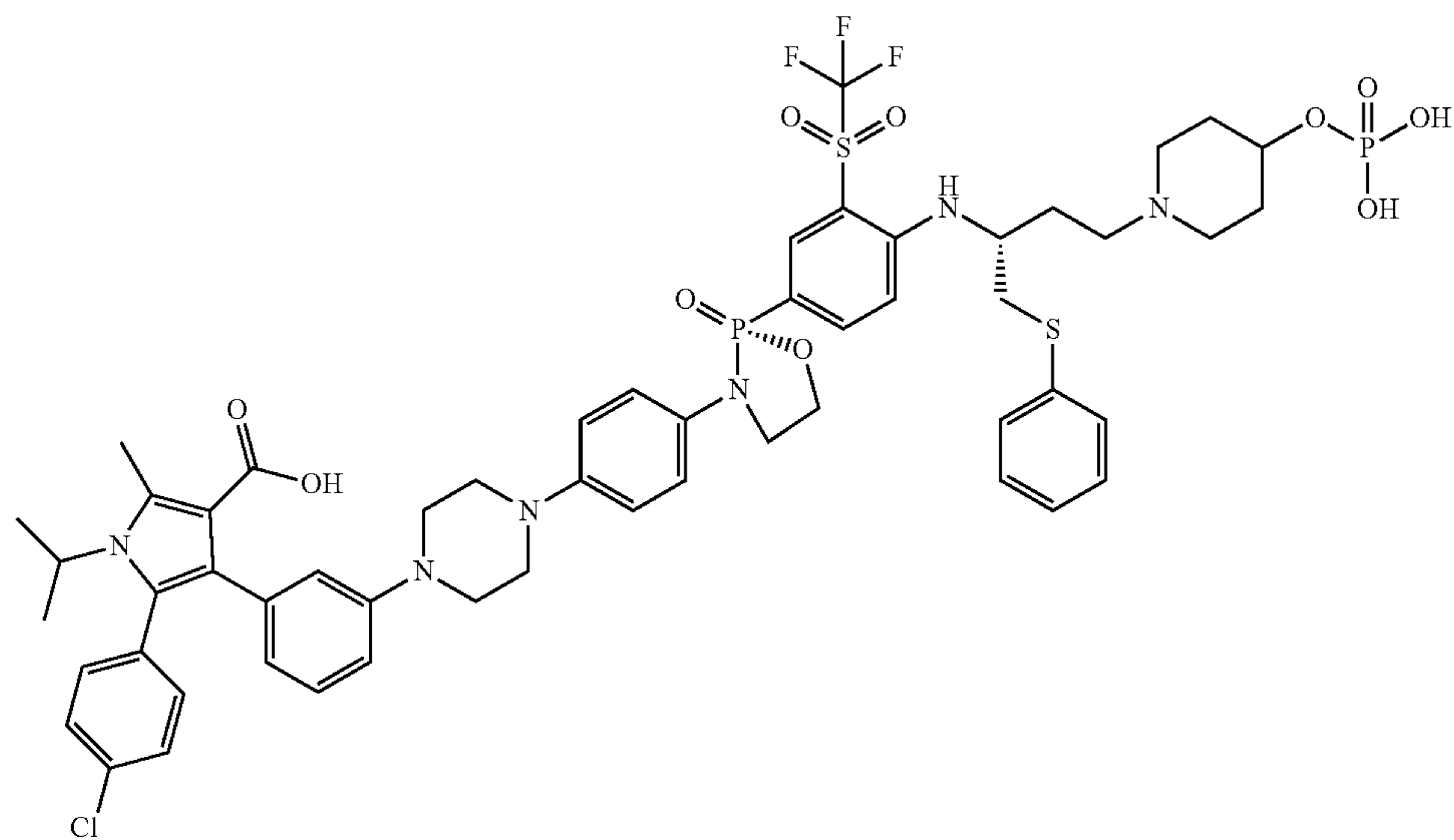
5-(4-chlorophenyl)-1-isopropyl-2-methyl-4-(3-(4-(4-(((R)-2-oxido-2-(4-(((R)-1-(phenylthio)-4-(4-(phosphonoxy)piperidin-1-yl)butan-2-yl)amino)-3-((trifluoromethyl)sulfonyl)phenyl)-1,3,2-oxazaphospholidin-3-yl)phenyl)piperazin-1-yl)phenyl)-1H-pyrrole-3-carboxylic acid
