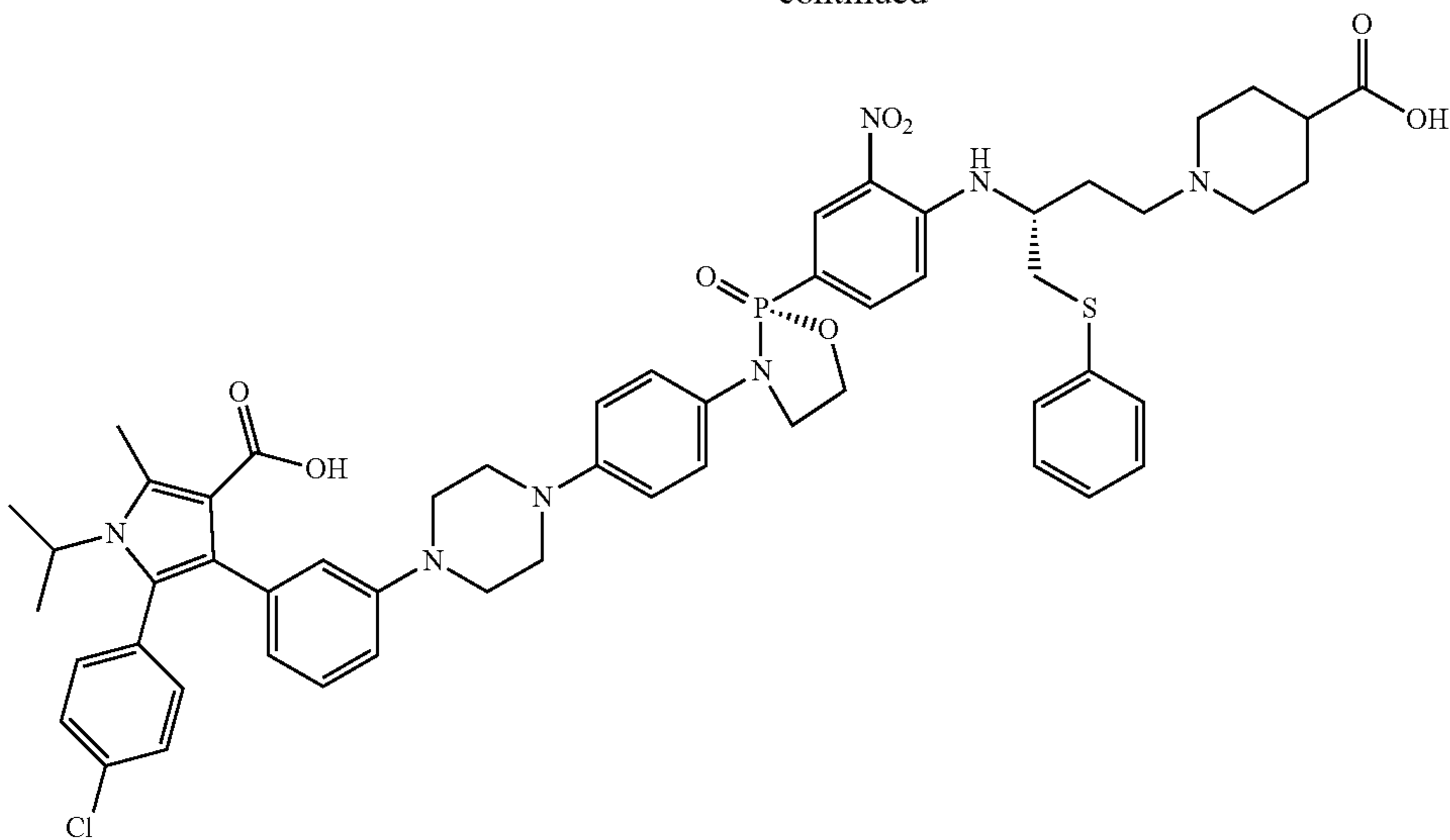
1-((R)-3-((4-((R)-3-(4-(4-(3-(4-carboxy-2-(4-chlorophenyl)-1-isopropyl-5-methyl-1H-pyrrol-3-yl)phenyl)piperazin-1-yl)phenyl)-2-oxido-1,3,2-oxazaphospholidin-2-yl)-1-nitrophenyl)amino)-4-(phenylthio)butyl)piperidine-4-carboxylic acid
