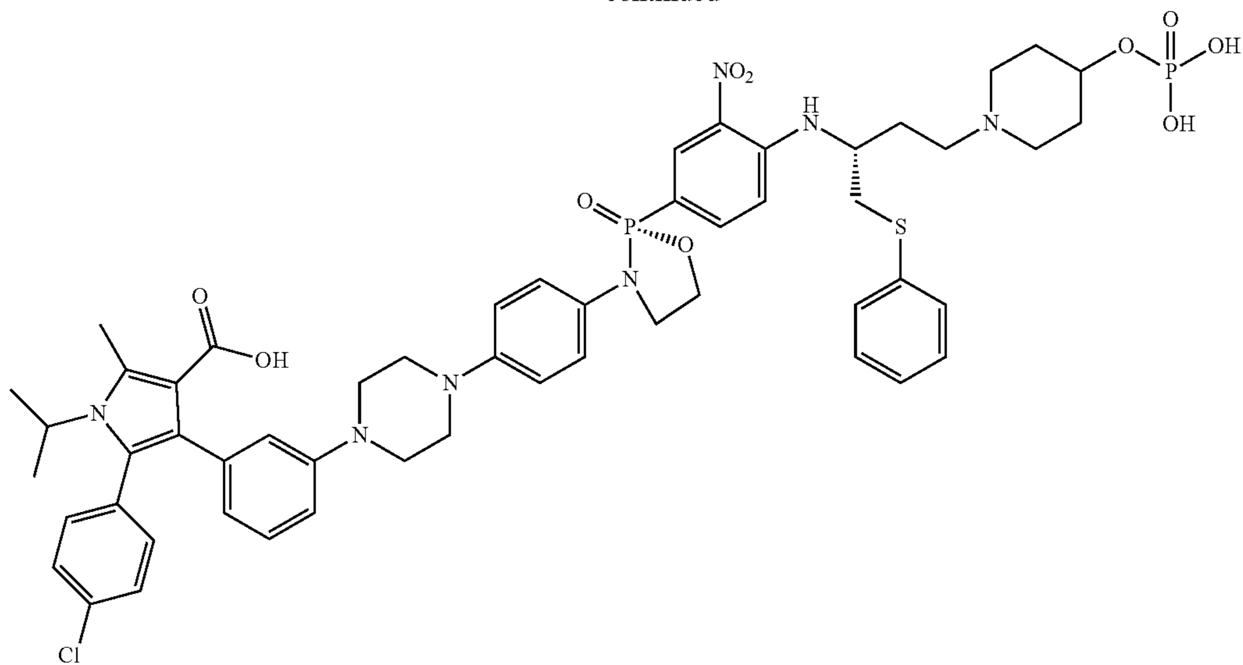
5-(4-chlorophenyl)-1-isopropyl-2-methyl-4-(3-(4-(4-((R)-2-(3-nitro-4-((R)-1-(phenylthio)-4-(4-(phosphonooxy)piperidin-1-yl)butan-2-yl)amino)phenyl)-2-oxido-1,3,2-oxazaphospholidin-3-yl)phenyl)piperazin-1-yl)phenyl)-1H-pyrrole-3-carboxylic acid
