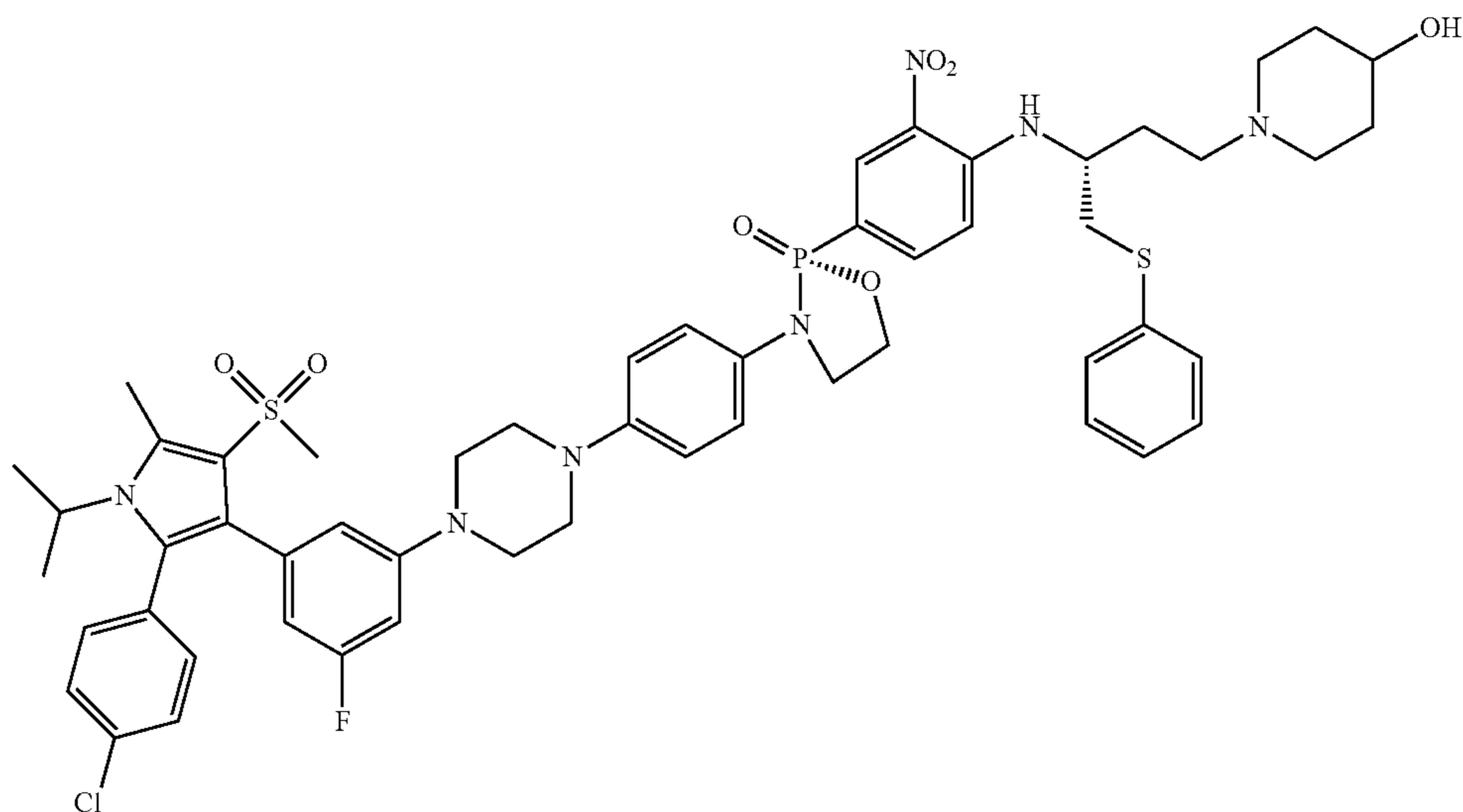
(R)-3-(4-(4-(3-(2-(4-chlorophenyl)-1-isopropyl-5-methyl-4-(methylsulfonyl)-1H-pyrrol-3-yl)-5-fluorophenyl)piperazin-1-yl)phenyl)-2-(4-(((R)-4-(4-(hydroxymethyl)piperidin-1-yl)-1-(phenylthio)butan-2-yl)amino)-3-nitrophenyl)-1,3,2-oxazaphospholidine 2-oxide
