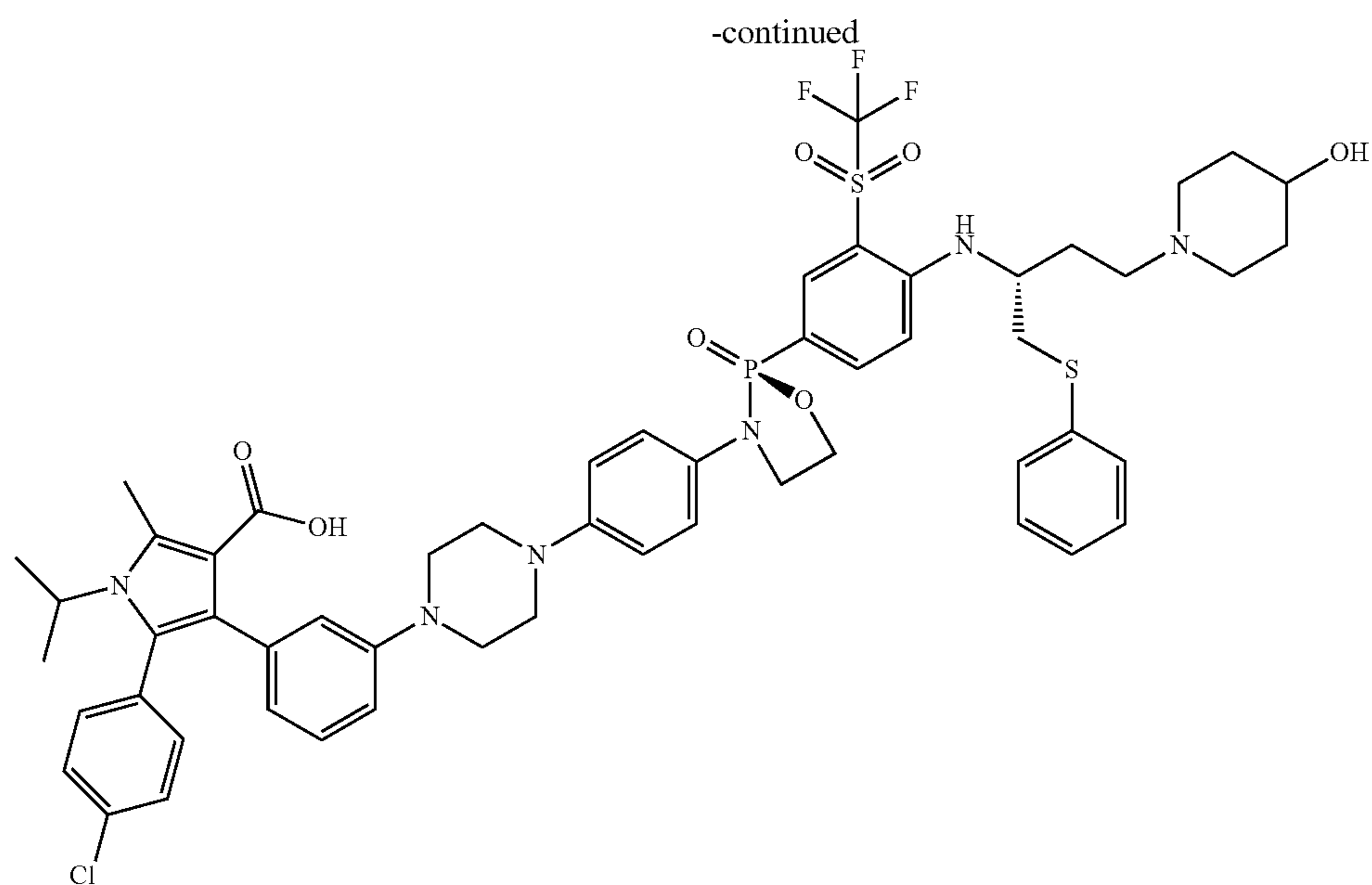
5-(4-chlorophenyl)-4-(3-(4-(4-((S)-2-(4-(((R)-4-(4-hydroxypiperidin-1-yl)-1-(phenylthio)butan-2-yl)amino)-3-((trifluoromethyl)sulfonyl)phenyl)-2-oxido-1,3,2-oxazaphospholidin-3-yl)phenyl)piperazin-1-yl)phenyl)-1-isopropyl-2-methyl-1H-pyrrole-3-carboxylic acid,
