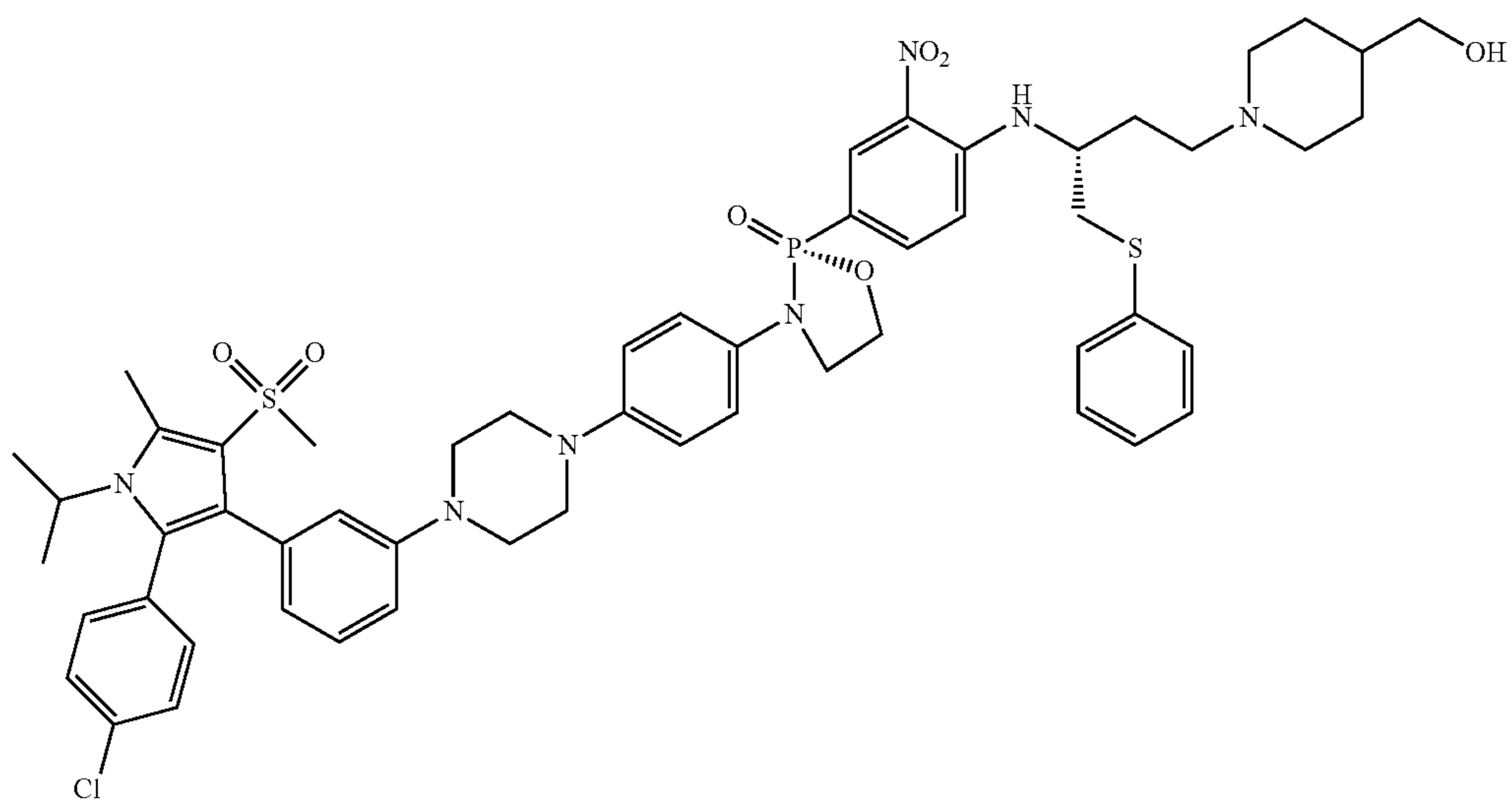
(R)-3-(4-(4-(3-(2-(4-chlorophenyl)-1-isopropyl-5-methyl-4-(methylsulfonyl)-1H-pyrrol-3-yl)phenyl)piperazin-1-yl)phenyl)-2-(4-(((R)-4-(4-(hydroxymethyl)pyridin-1-yl)-1-(phenylthio)butan-2-yl)amino)-3-nitrophenyl)-1,3,2-oxazaphospholidine 2-oxide
