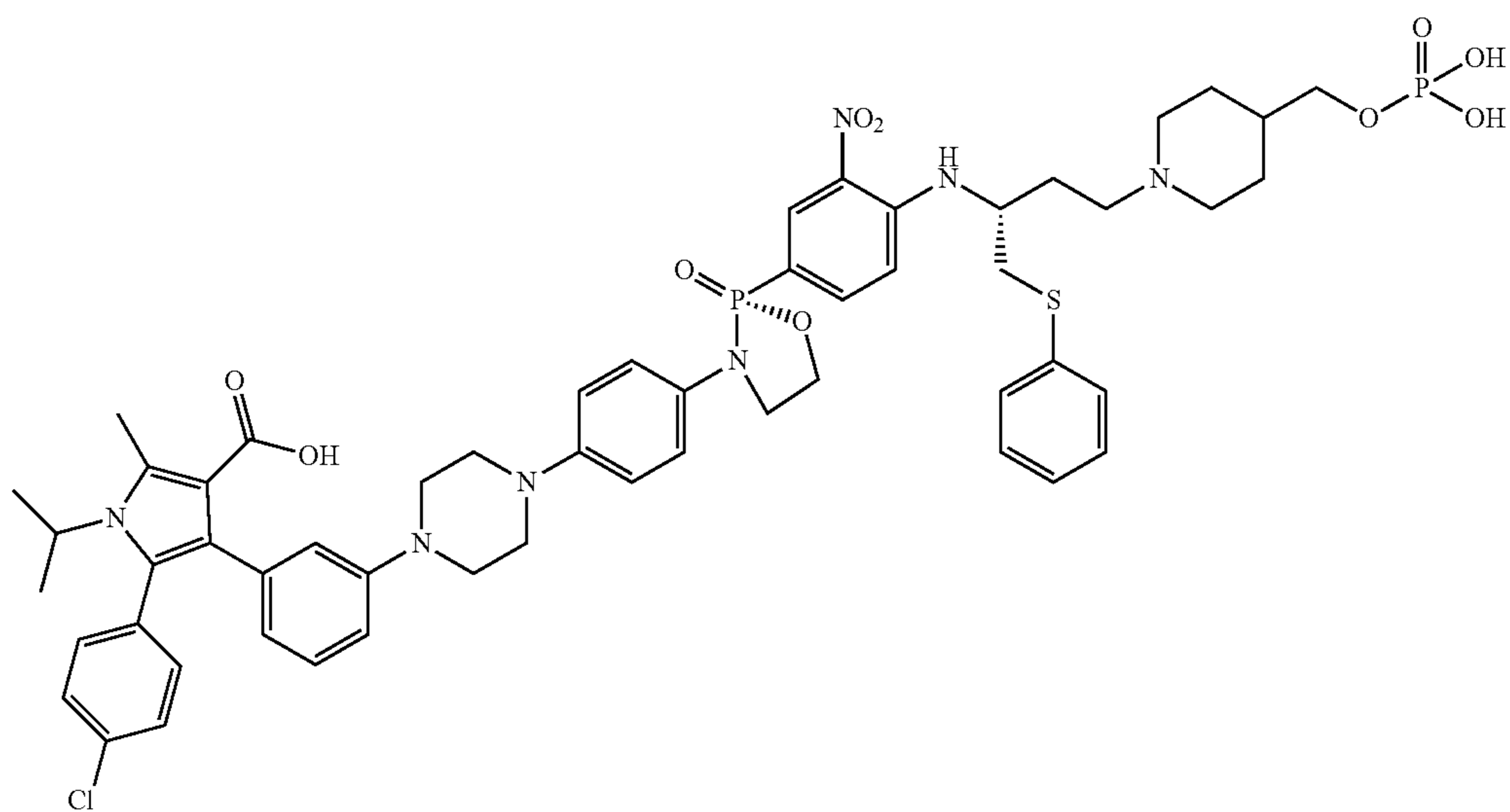
5-(4-chlorophenyl)-1-isopropyl-2-methyl-4-(3-(4-(4-((R)-2-(3-nitro-4-((R)-1-(phenylthio)-4-(4-((phosphonoxy)methyl)piperidin-1-yl)butan-2-yl)amino)phenyl)-2-oxido-1,3,2-oxazaphospholidin-3-yl)phenyl)piperazin-1-yl)phenyl)-1H-pyrrole-3-carboxylic acid
