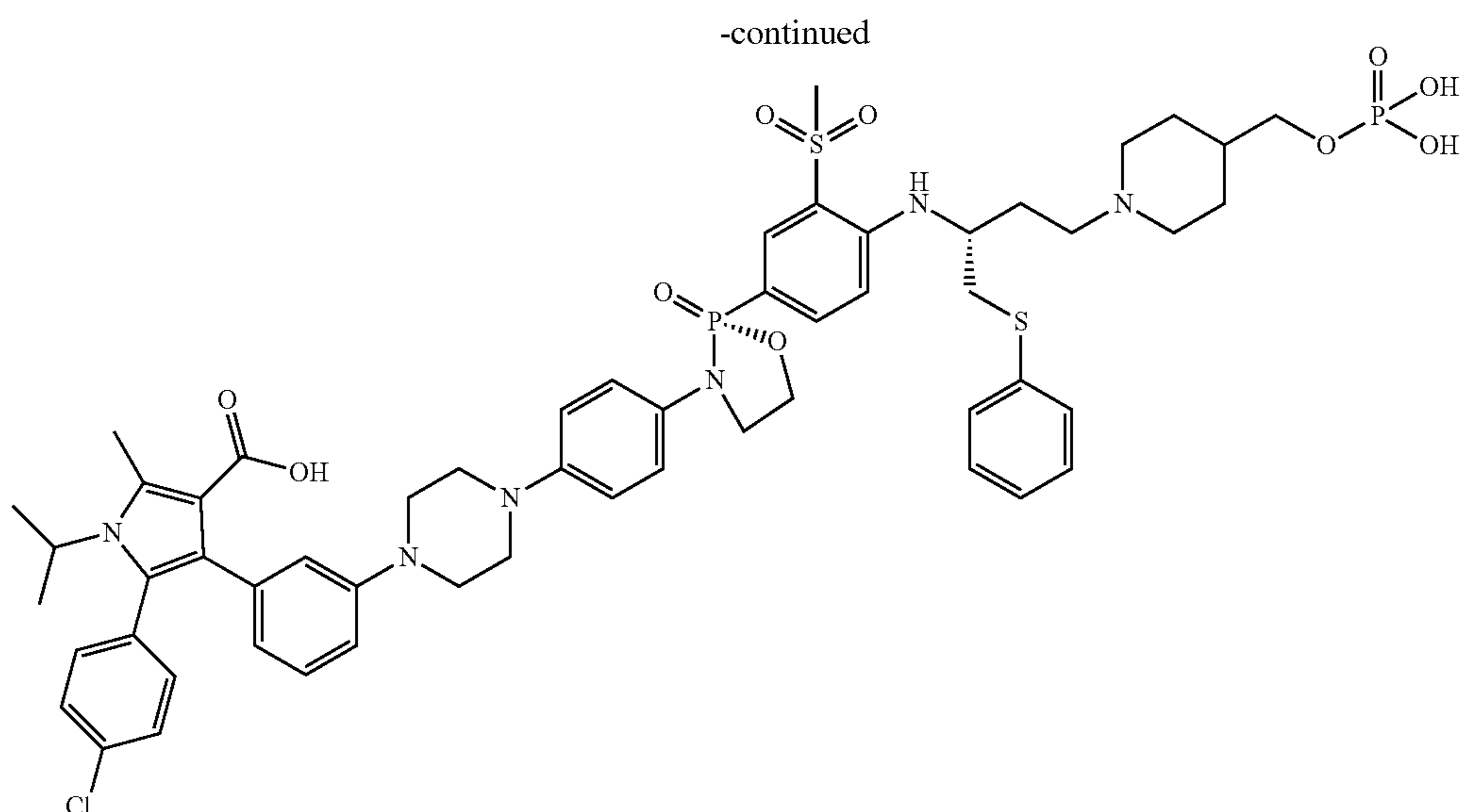
5-(4-chlorophenyl)-1-isopropyl-2-methyl-4-(3-(4-(4-((R)-2-(3-(methylsulfonyl)-4-(((R)-1-(phenylthio)-4-(4-((phosphonooxy)piperidin-1-yl)butan-2-yl)amino)phenyl)-2-oxido-1,3,2-oxazaphospholidin-3-yl)phenyl)piperazin-1-yl)phenyl)-1H-pyrrole-3-carboxylic acid
