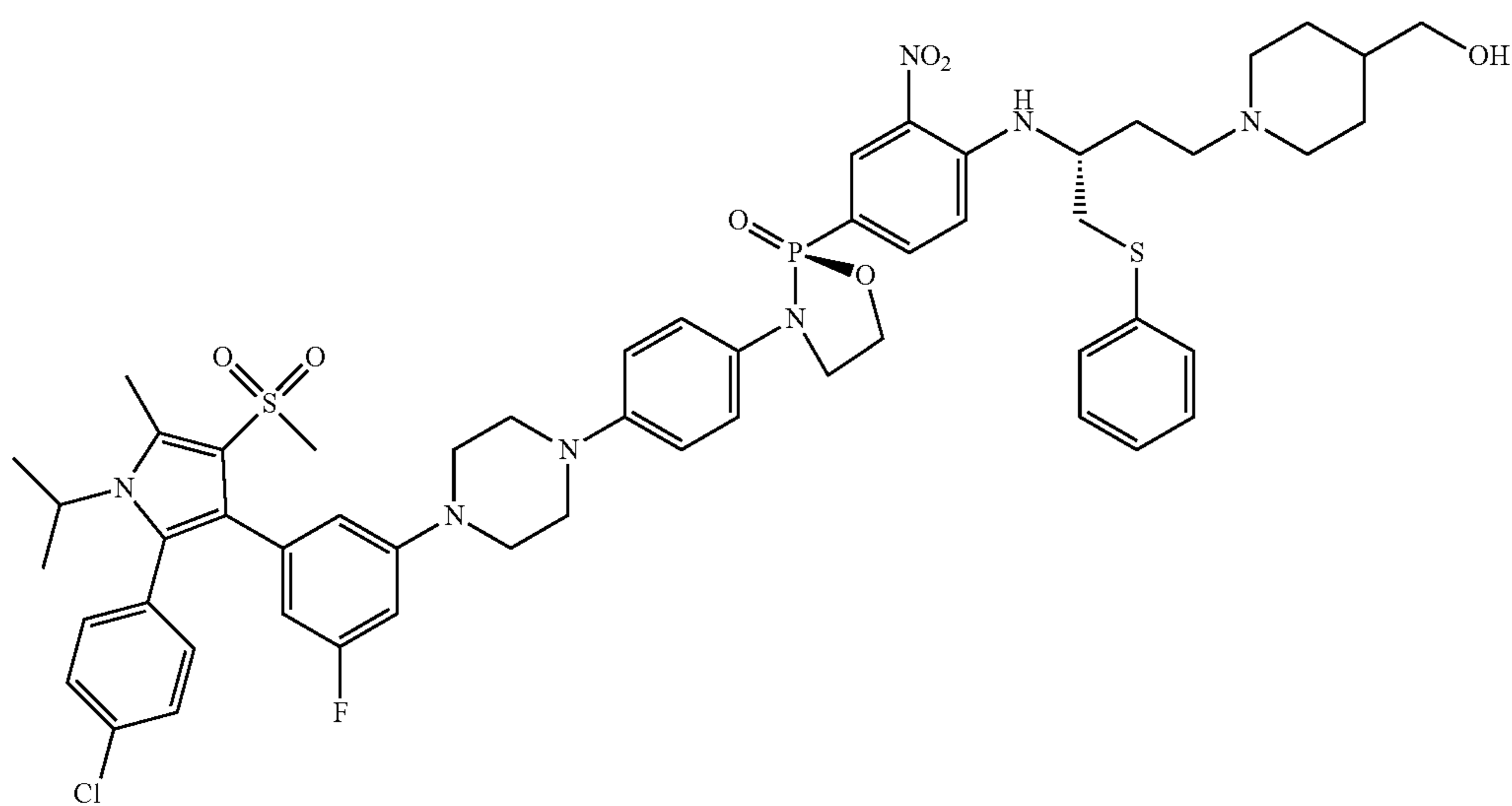
(S)-3-(4-(4-(3-(2-(4-chlorophenyl)-1-isopropyl-5-methyl-4-(methylsulfonyl)-1H-pyrrol-3-yl)-5-fluorophenyl)piperazin-1-yl)phenyl)-2-(4-(((S)-4-(4-(hydroxymethyl)piperidin-1-yl)-1-(phenylthio)butan-2-yl)amino)-3-nitrophenyl)-1,3,2-oxazaphospholidine 2-oxide
