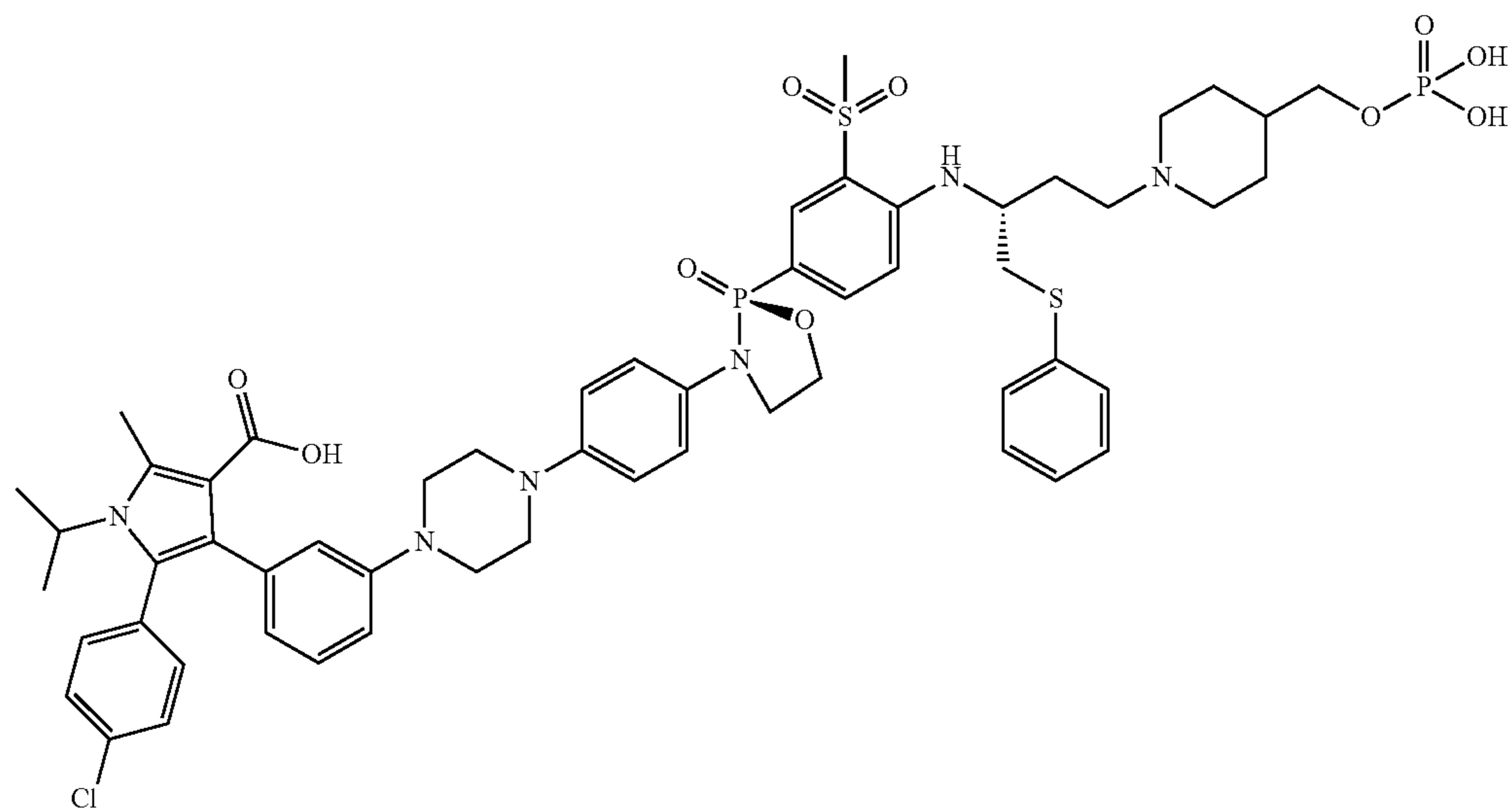
5-(4-chlorophenyl)-1-isopropyl-2-methyl-4-(3-(4-(4-((S)-2-(3-(methylsulfonyl)-4-(((R)-1-(phenylthio)-4-(4-(phosphonooxy)piperidin-1-yl)butan-2-yl)amino)phenyl)-2-oxido-1,3,2-oxazaphospholidin-3-yl)phenyl)piperazin-1-yl)phenyl)-1H-pyrrole-3-carboxylic acid
