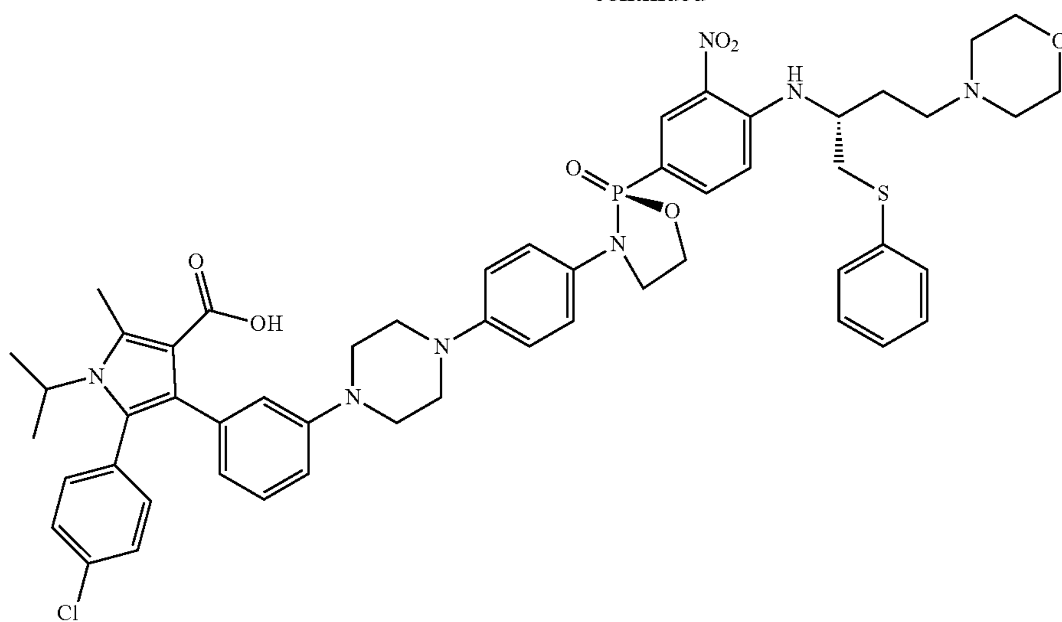
5-(4-chlorophenyl)-1-isopropyl-2-methyl-4-(3-(4-(4-((S)-2-(4-((R)-4-morpholino-1-(phenylthio)butan-2-yl)amino)-3-nitrophenyl)-2-oxido-1,3,2-oxazaphospholidin-3-yl)phenyl)piperazin-1-yl)phenyl)-1H-pyrrole-3-carboxylic acid
