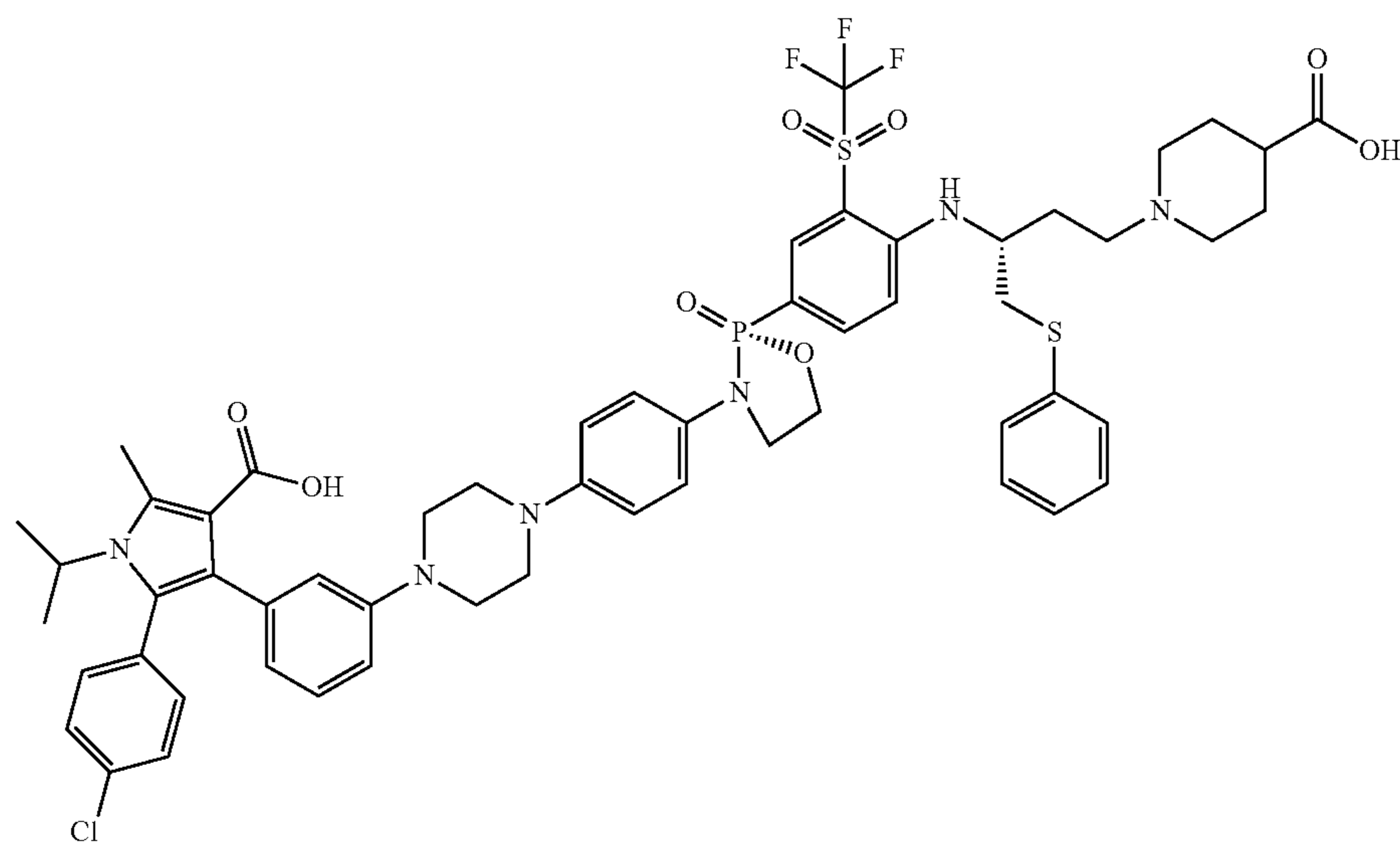
1-((R)-3-((4-((R)-3-(4-(4-(3-(4-carboxy-2-(4-chlorophenyl)-1-isopropyl-5-methyl-1H-pyrrol-3-yl)phenyl)piperazin-1-yl)phenyl)-2-oxido-1,3,2-oxazaphospholidin-2-yl)-2-((trifluoromethyl)sulfonyl)phenyl)amino)-4-(phenylthio)butyl)piperidine-4-carboxylic acid
