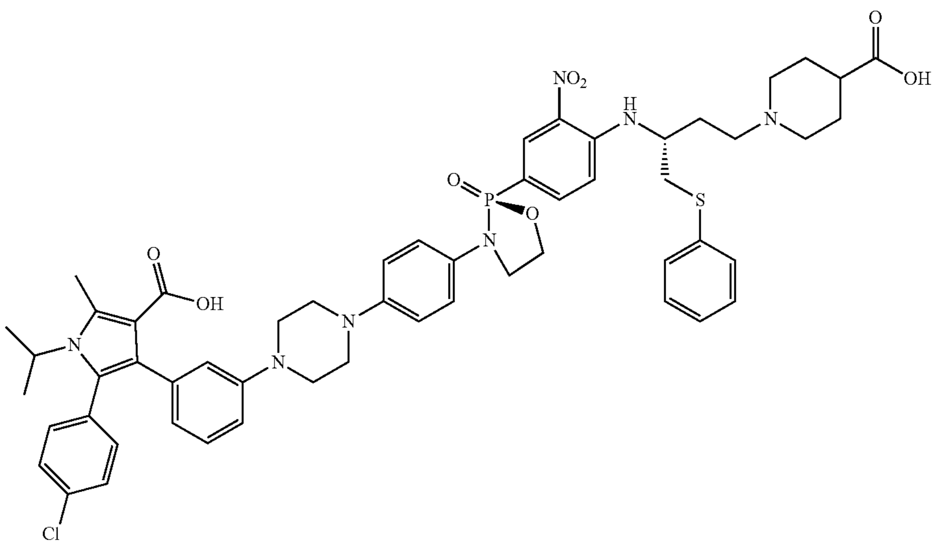
1-((S)-3-((4-((R)-3-(4-(4-(3-(4-carboxy-2-(4-chlorophenyl)-1-isopropyl-5-methyl-1H-pyrrol-3-yl)phenyl)piperazin-1-yl)phenyl)-2-oxido-1,3,2-oxazaphospholidin-2-yl)-1-nitrophenyl)amino)-4-(phenylthio)butyl)piperidine-4-carboxylic acid
