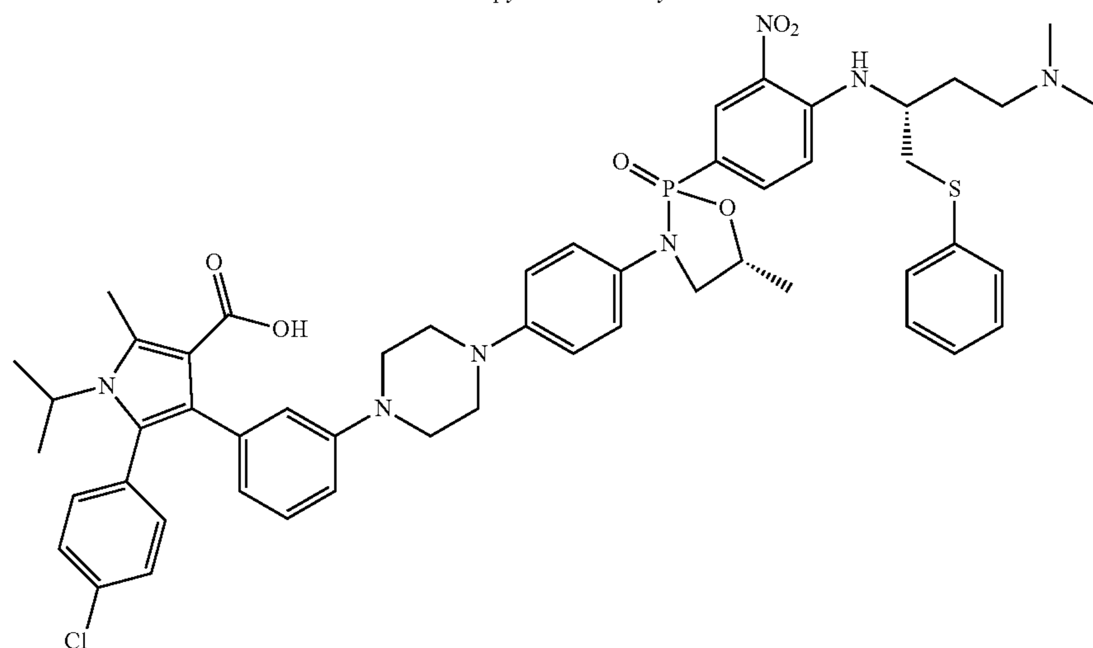
5-(4-chlorophenyl)-4-(3-(4-(4-(2-(4-(((R)-4-(4-hydroxypiperidin-1-yl)-1-(phenylthio)butan-2-yl)amino)-3-nitrophenyl)-2-oxido-1,3,2-oxazaphospholidin-3-yl)phenyl)piperazin-1-yl)phenyl)-1-isopropyl-2-methyl-1H-pyrrole-3-carboxylic acid
