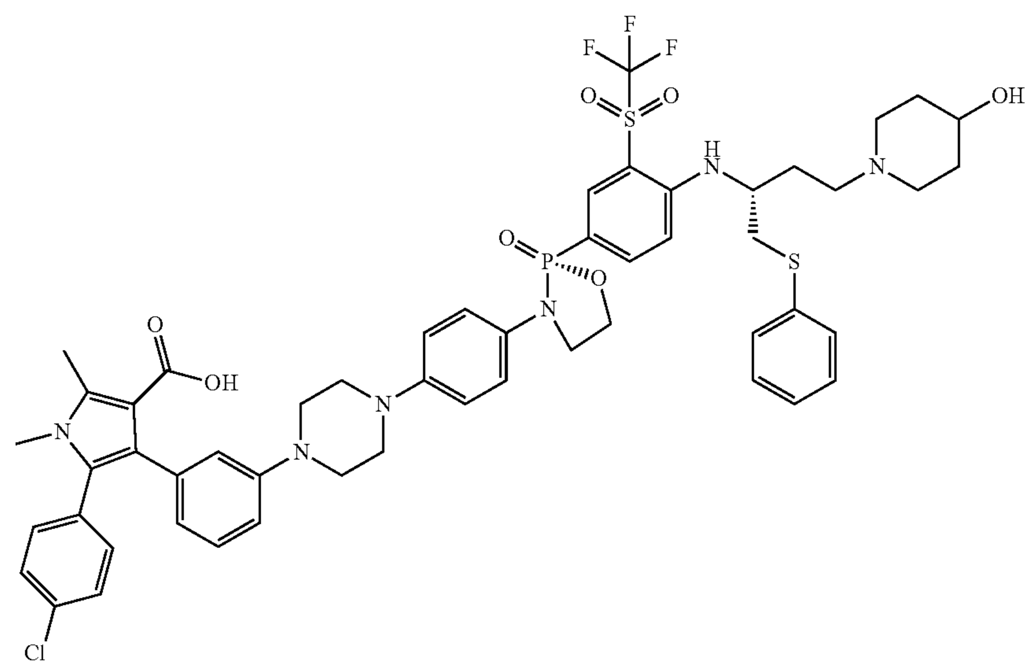
5-(4-chlorophenyl)-4-(3-(4-(4-((R)-2-(4-(((R)-4-(4-hydroxypiperidin-1-yl)-1-(phenylthio)butan-2-yl)amino)-3-((trifluoromethyl)sulfonyl)phenyl)-2-oxido-1,3,2-oxazaphospholidin-3-yl)phenyl)piperazin-1-yl)phenyl)-1,2-dimethyl-1H-pyrrole-3-carboxylic acid
