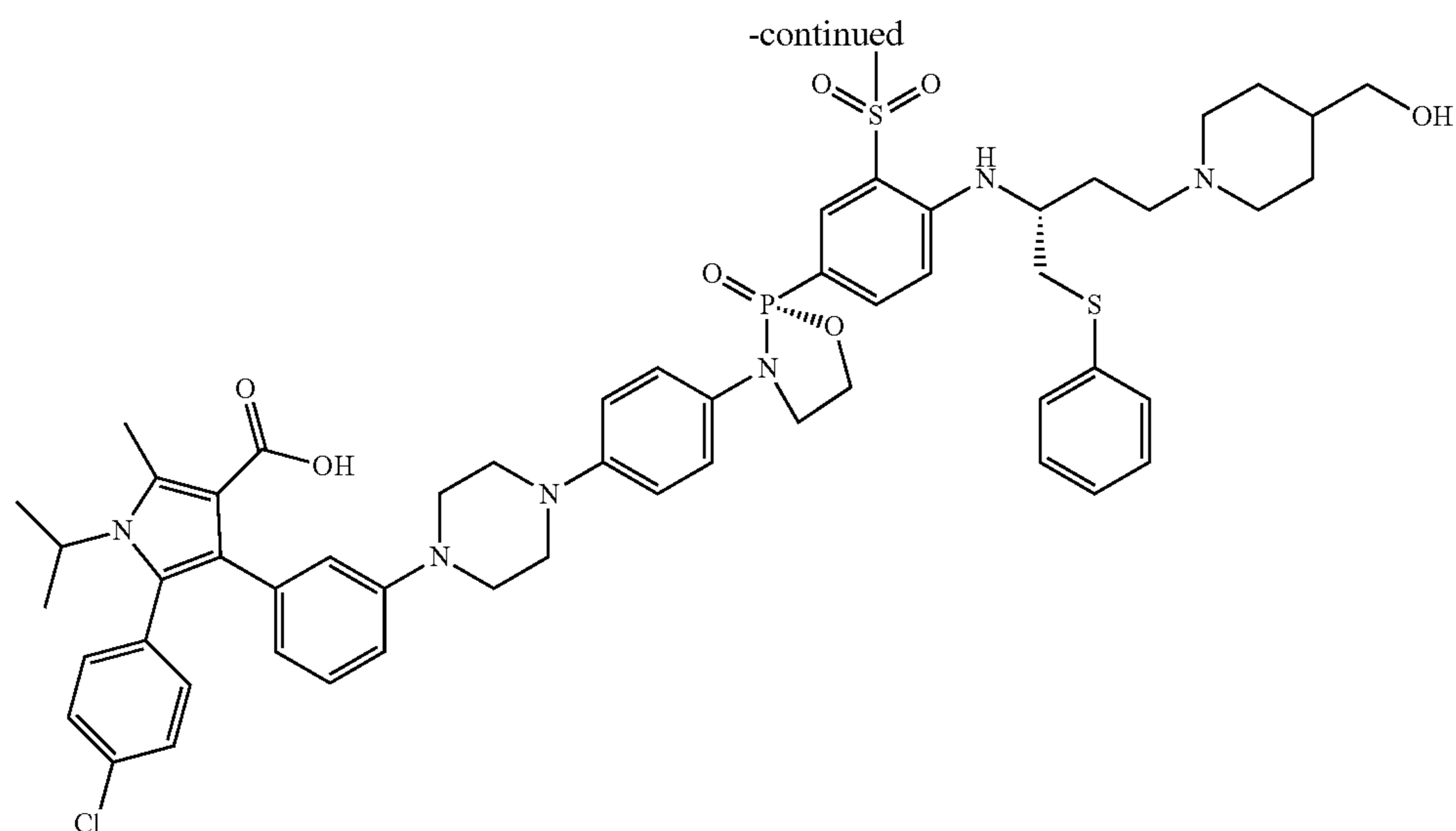
5-(4-chlorophenyl)-4-(3-(4-(4-((R)-2-(4-(((R)-4-(4-(hydroxymethyl)piperidin-1-yl)-1-(phenylthio)butan-2-yl)amino)-3-(methylsulfonyl)phenyl)-2-oxido-1,3,2-oxazaphospholidin-3-yl)phenyl)piperazin-1-yl)phenyl)-1-isopropyl-2-methyl-1H-pyrrole-3-carboxylic acid
