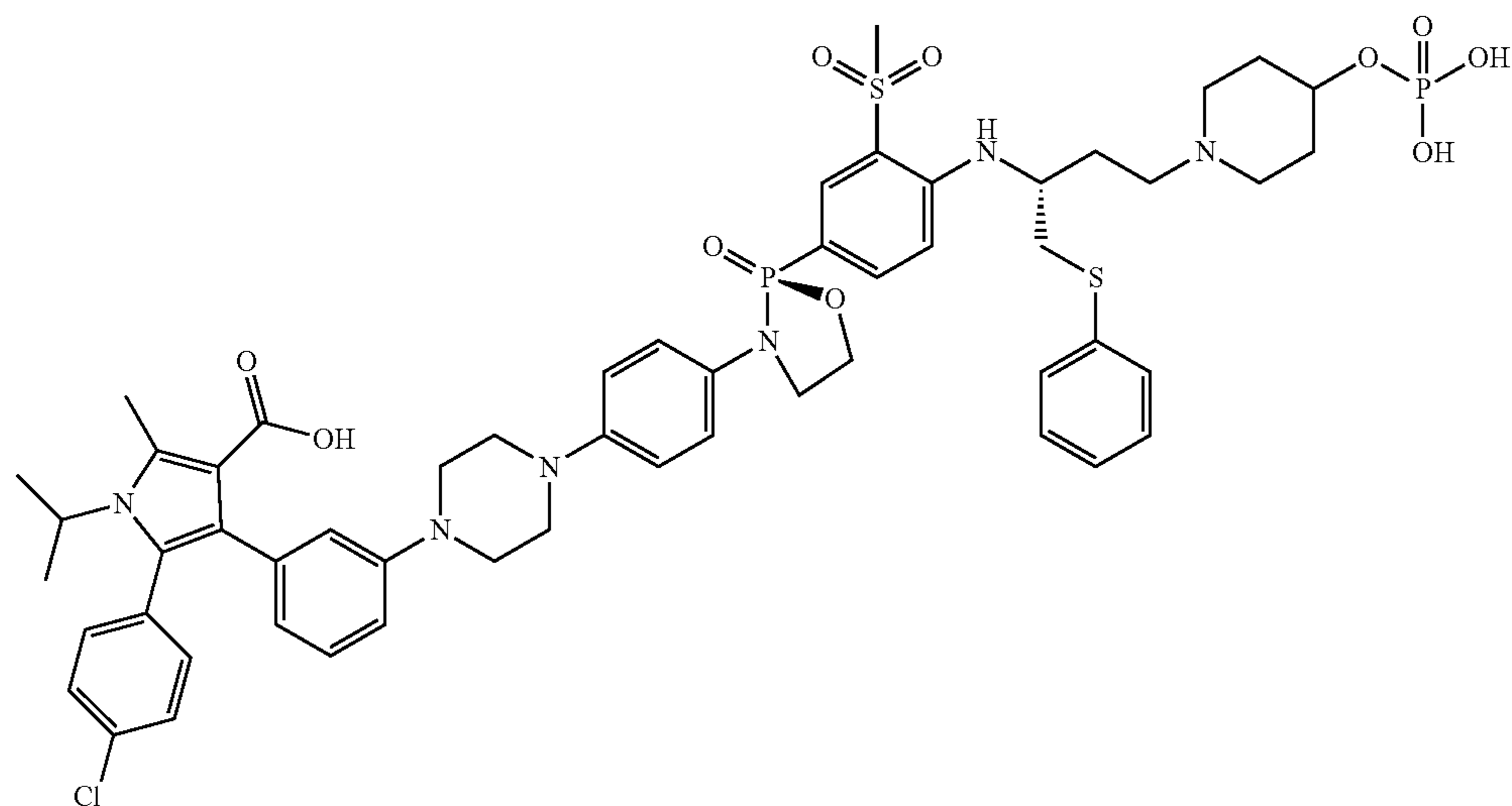
5-(4-chlorophenyl)-1-isopropyl-2-methyl-4-(3-(4-(4-((S)-2-(3-(methylsulfonyl)-4-((R)-1-(phenylthio)-4-(4-(phosphonoxy)piperidin-1-yl)butan-2-yl)amino)phenyl)-2-oxido-1,3,2-oxazaphospholidin-3-yl)phenyl)piperazin-1-yl)phenyl)-1H-pyrrole-3-carboxylic acid
