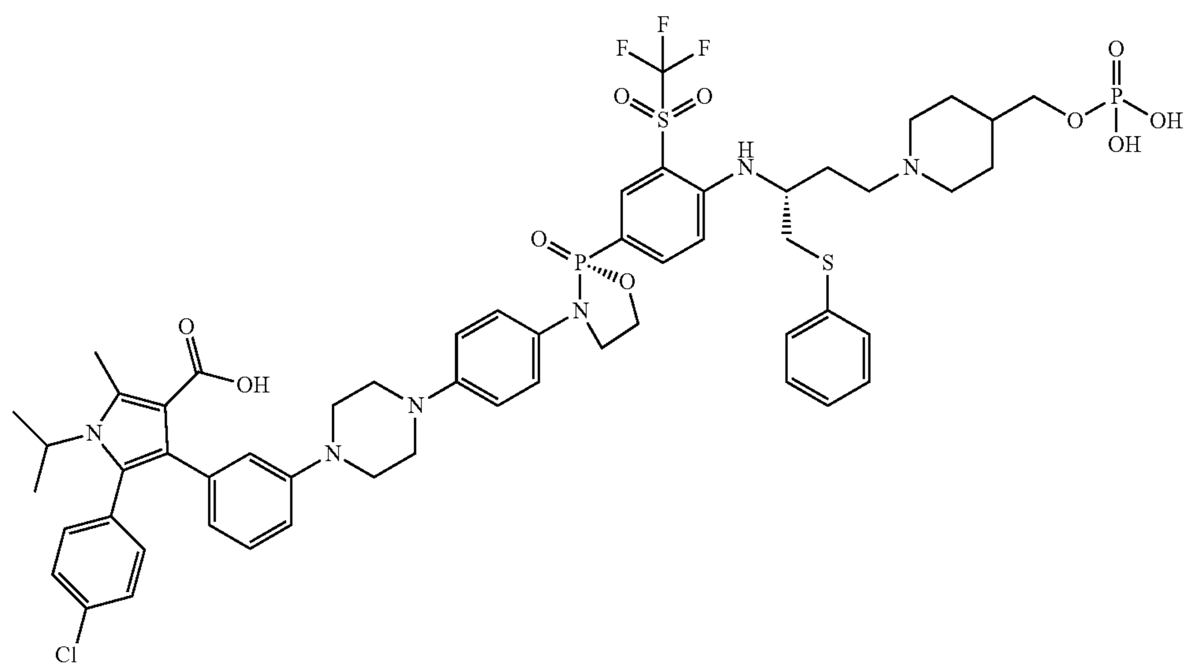
5-(4-chlorophenyl)-1-isopropyl-2-methyl-4-(3-(4-(4-((R)-2-oxido-2-(4-(((R)-1-(phenylthio)-4-(4-(phosphonoxy)methyl)piperidin-1-yl)butan-2-yl)amino)-3-((trifluoromethyl)sulfonyl)phenyl)-1,3,2-oxazaphospholidin-3-yl)phenyl)piperazin-1-yl)phenyl)-1H-pyrrole-3-carboxylic acid
