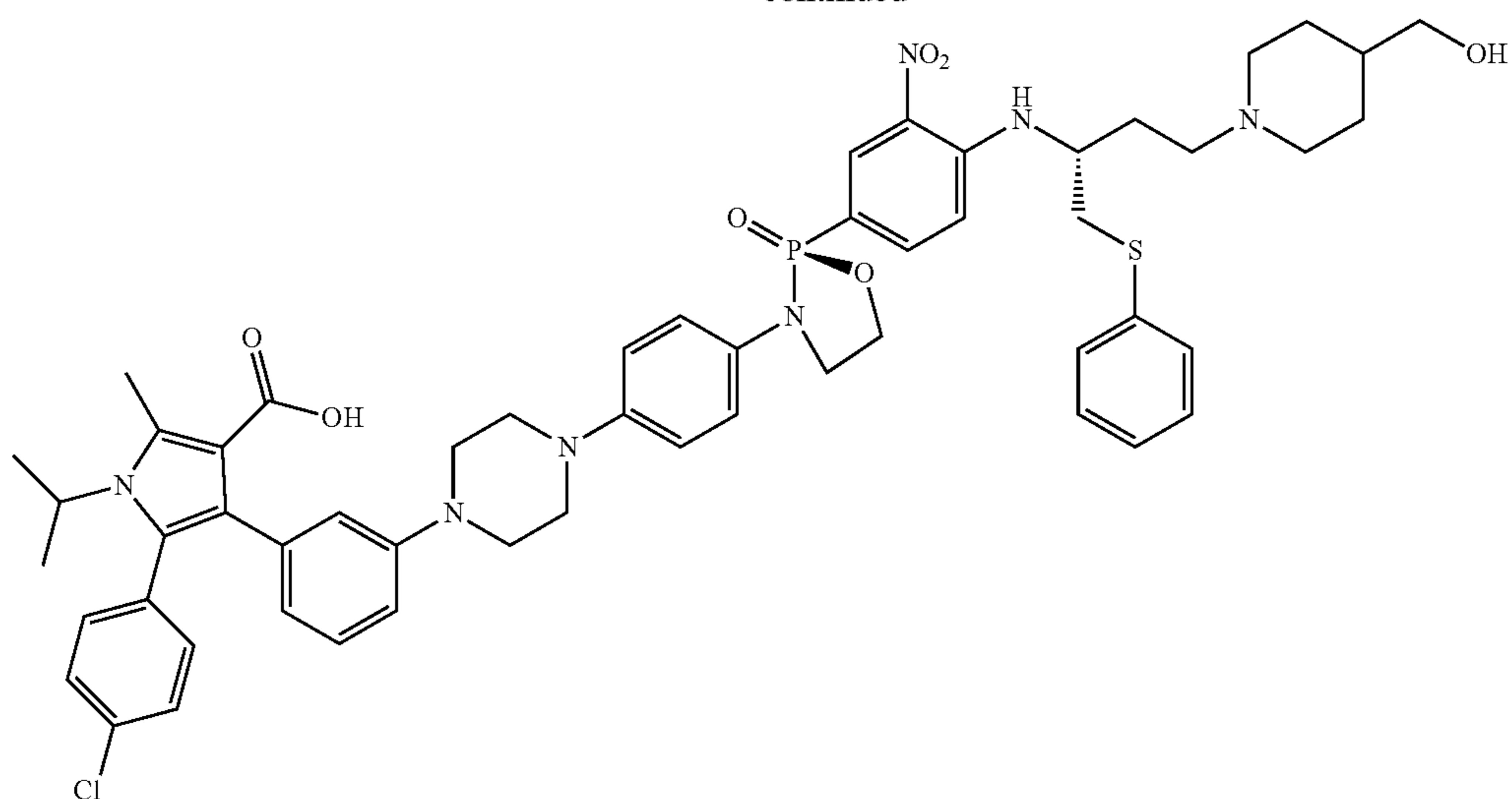
5-(4-chlorophenyl)-4-(3-(4-(4-((S)-2-(4-(((R)-4-(4-hydroxymethyl)piperidin-1-yl)-1-(phenylthio)butan-2-yl)amino)-3-nitrophenyl)-2-oxido-1,3,2-oxazaphospholidin-3-yl)phenyl)piperazin-1-yl)phenyl)-1-isopropyl-2-methyl-1H-pyrrole-3-carboxylic acid
