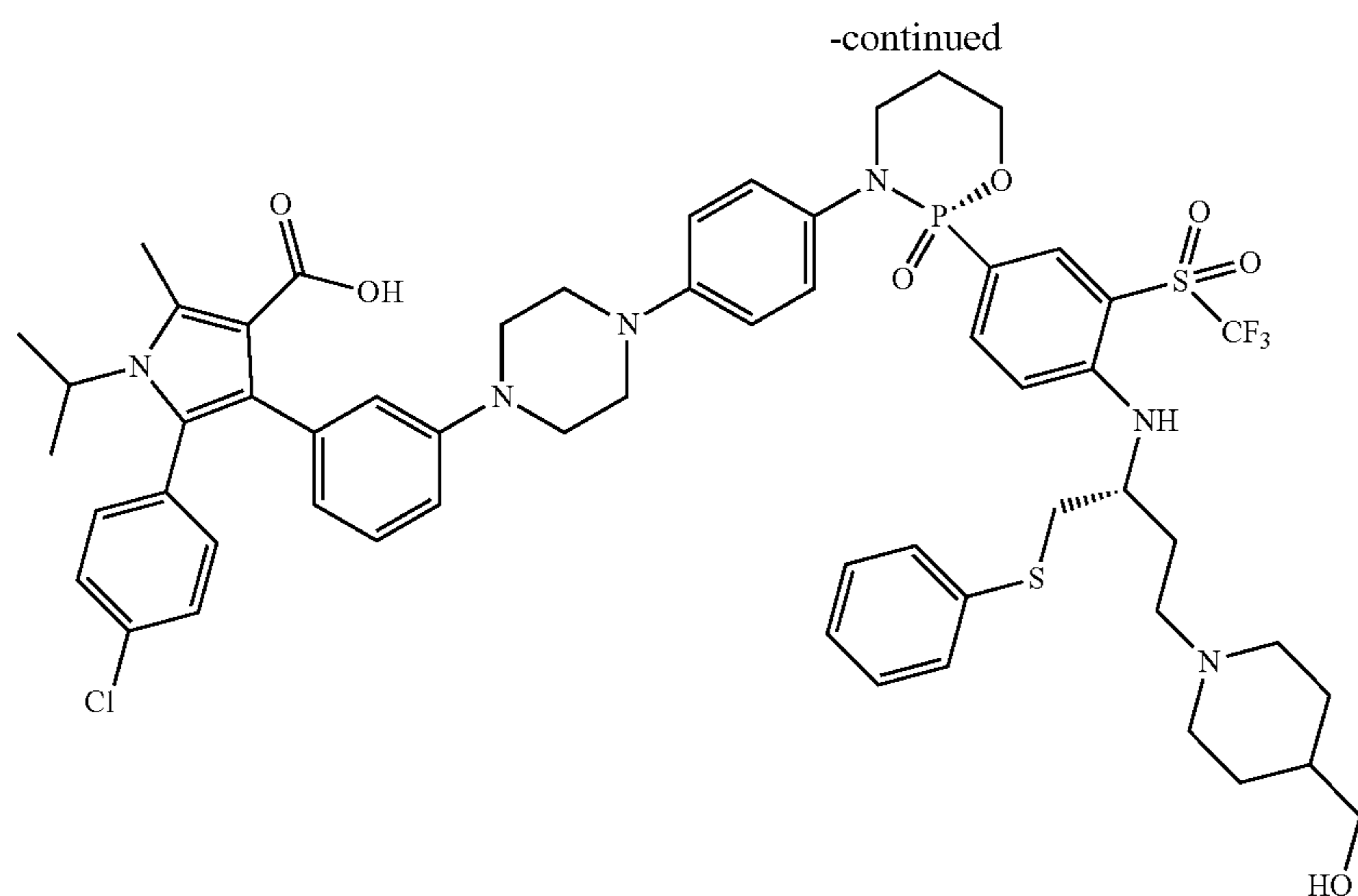
5-(4-chlorophenyl)-4-(3-(4-(4-((S)-2-(4-((R)-4-(4-(hydroxymethyl)piperidin-1-yl)-1-(phenylthio)butan-2-yl)amino)-3-((trifluoromethyl)sulfonyl)phenyl)-2-oxido-1,3,2-oxazaphosphinan-3-yl)phenyl)piperazin-1-yl)phenyl)-1-isopropyl-2-methyl-1H-pyrrole-3-carboxylic acid
