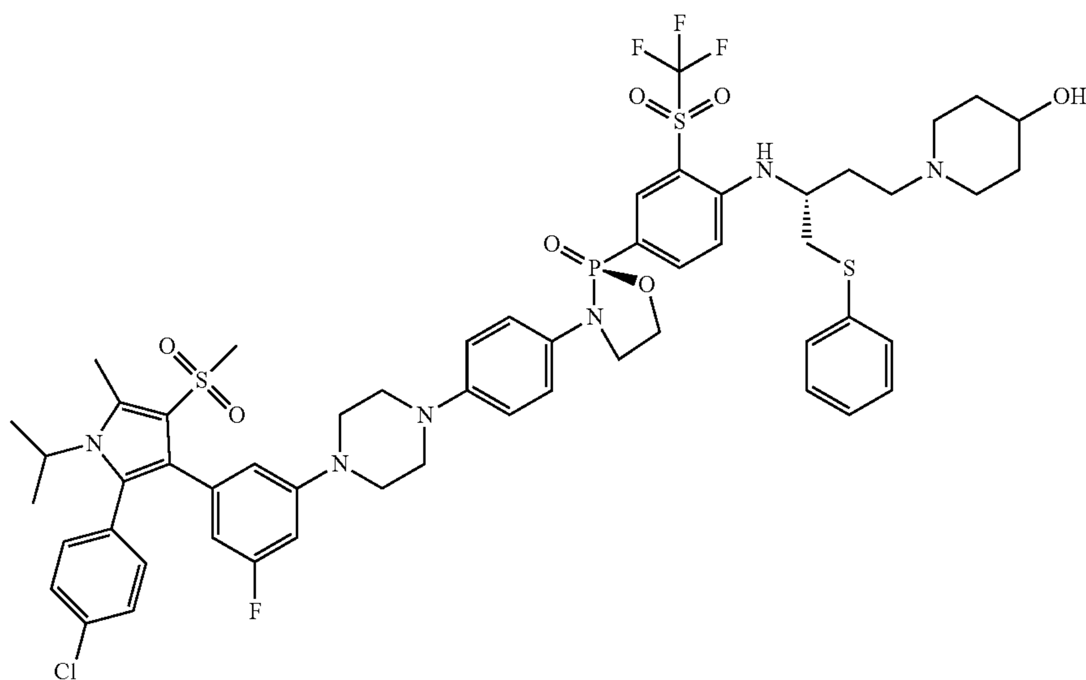
(S)-3-(4-(4-(3-(2-(4-chlorophenyl)-1-isopropyl-5-methyl-4-(methylsulfonyl)-1H-pyrrol-3-yl)-5-fluorophenyl)piperazin-1-yl)phenyl)-2-(4-(((R)-4-(4-(hydroxypiperidin-1-yl)-1-(phenylthio)butan-2-yl)amino)-3-(trifluoromethyl)sulfonyl)phenyl)-1,3,2-oxazaphospholidine 2-oxide
