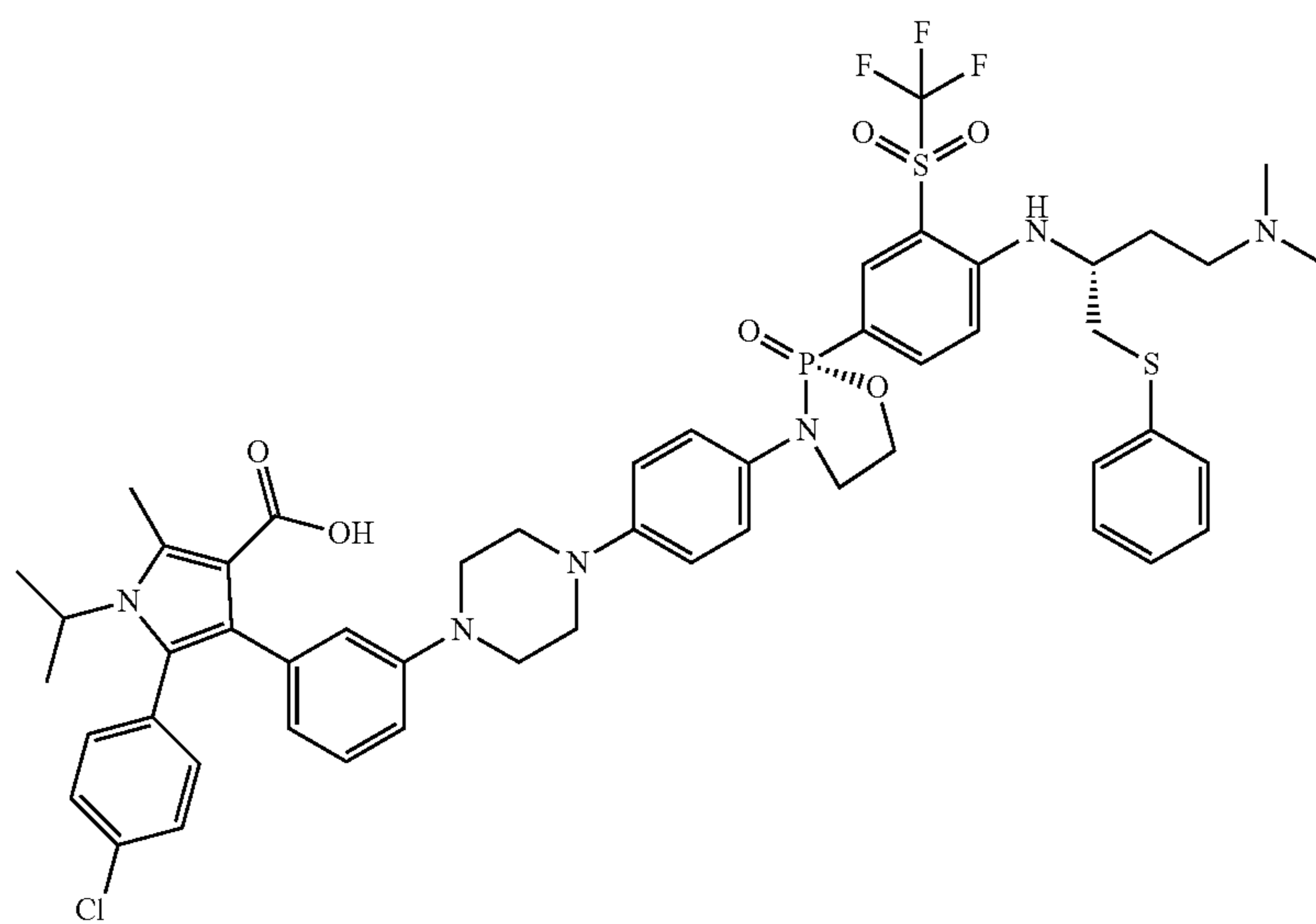
5-(4-chlorophenyl)-4-(3-(4-(4-((R)-2-(4-(((R)-4-(dimethylamino)-1-(phenylthio)butan-2-yl)amino)-3-((trifluoromethyl)sulfonyl)phenyl)-2-oxido-1,3,2-oxazaphospholidin-3-yl)phenyl)piperazin-1-yl)phenyl)-1-isopropyl-2-methyl-1H-pyrrole-3-carboxylic acid
