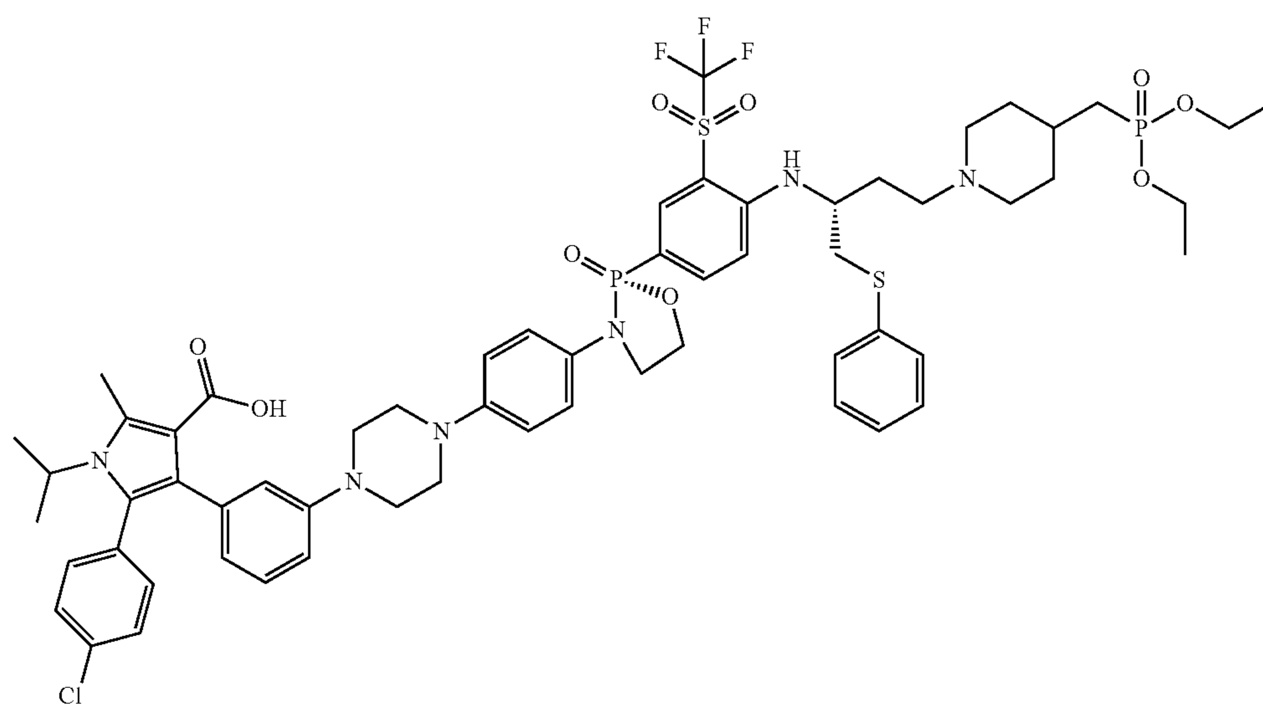
5-(4-chlorophenyl)-4-(3-(4-(4-((R)-2-(4-(((R)-4-(4-((diethoxyphosphoryl)methyl)piperidin-1-yl)-1-(phenylthio)butan-2-yl)amino)-3-((trifluoromethyl)sulfonyl)phenyl)-2-oxido-1,3,2-oxazaphospholidin-3-yl)phenyl)piperazin-1-yl)phenyl)-1-isopropyl-2-methyl-1H-pyrrole-3-carboxylic acid
