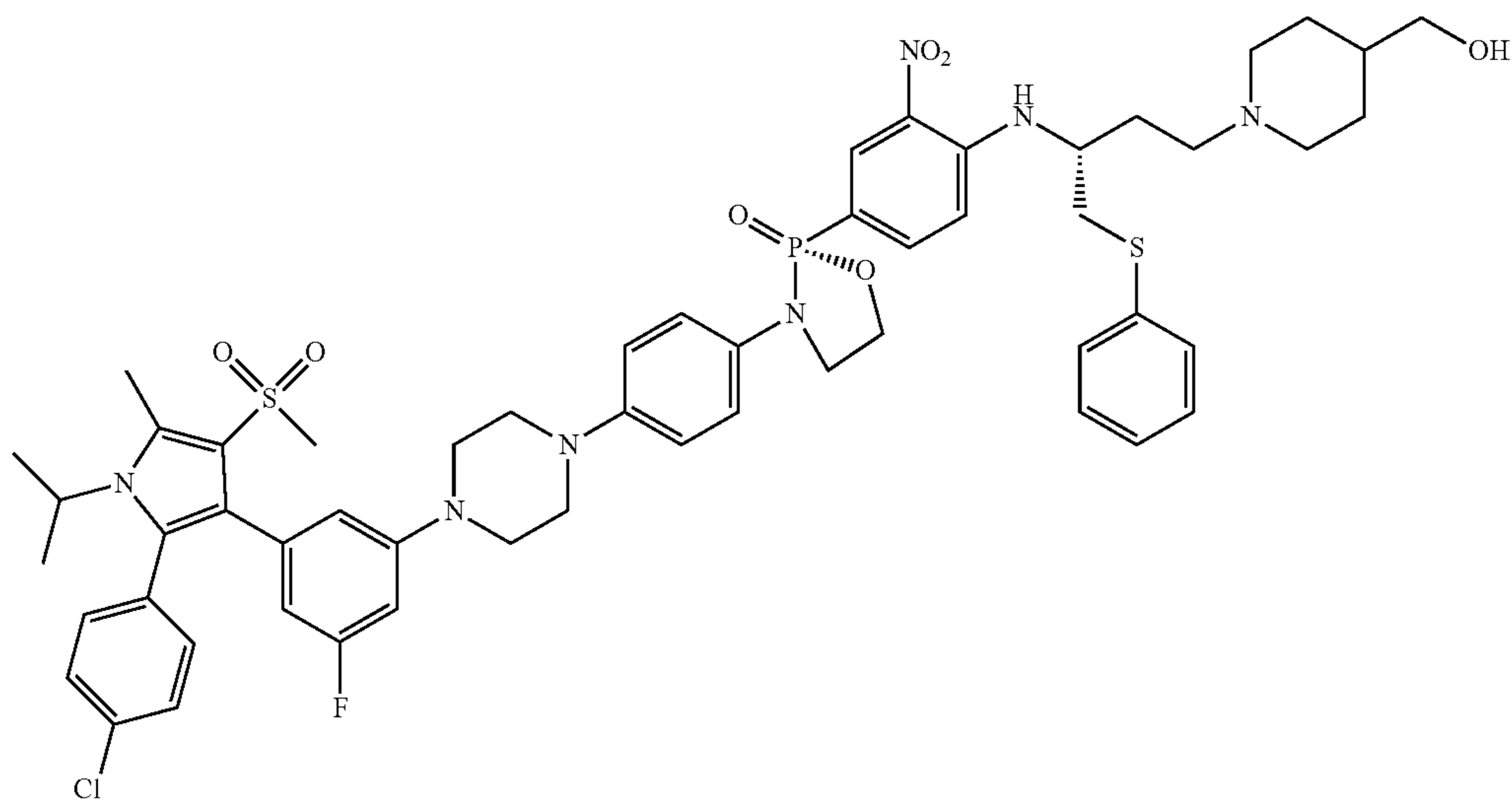
(R)-3-(4-(4-(3-(2-(4-chlorophenyl)-1-isopropyl-5-methyl-4-(methylsulfonyl)-1H-pyrrol-3-yl)-5-fluorophenyl)piperazin-1-yl)phenyl)-2-(4-(((R)-4-(4-(hydroxymethyl)piperidin-1-yl)-1-(phenylthio)butan-2-yl)amino)-3-nitrophenyl)-1,3,2-oxazaphospholidine 2-oxide
