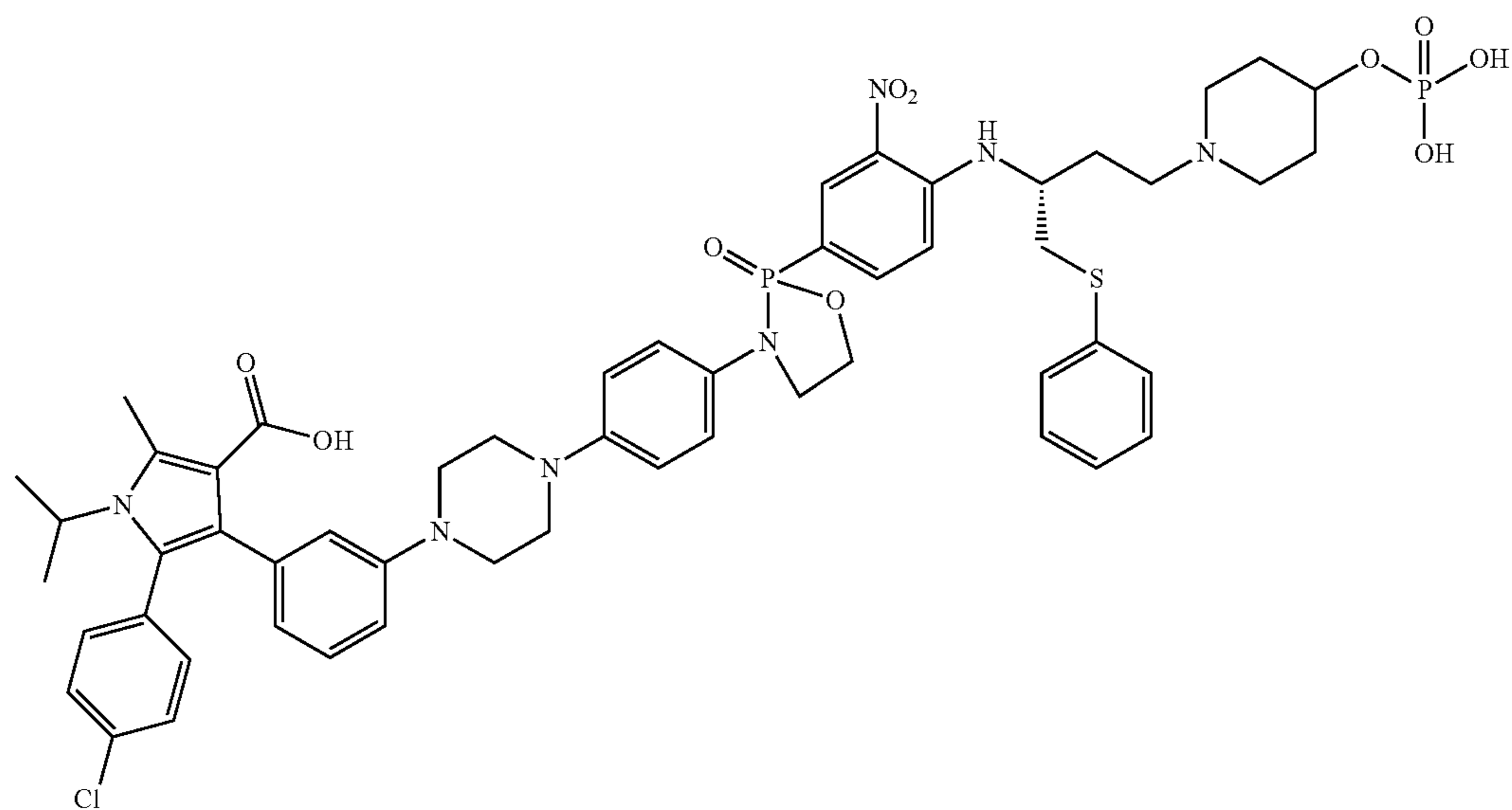
5-(4-chlorophenyl)-1-isopropyl-2-methyl-4-(3-(4-(4-(2-(3-nitro-4-(((R)-1-(phenylthio)-4-(4-(phosphonoxy)piperidin-1-yl)butan-2-yl)amino)phenyl)-2-oxido-1,3,2-oxazaphospholidin-3-yl)phenyl)piperazin-1-yl)phenyl)-1H-pyrrole-3-carboxylic acid
