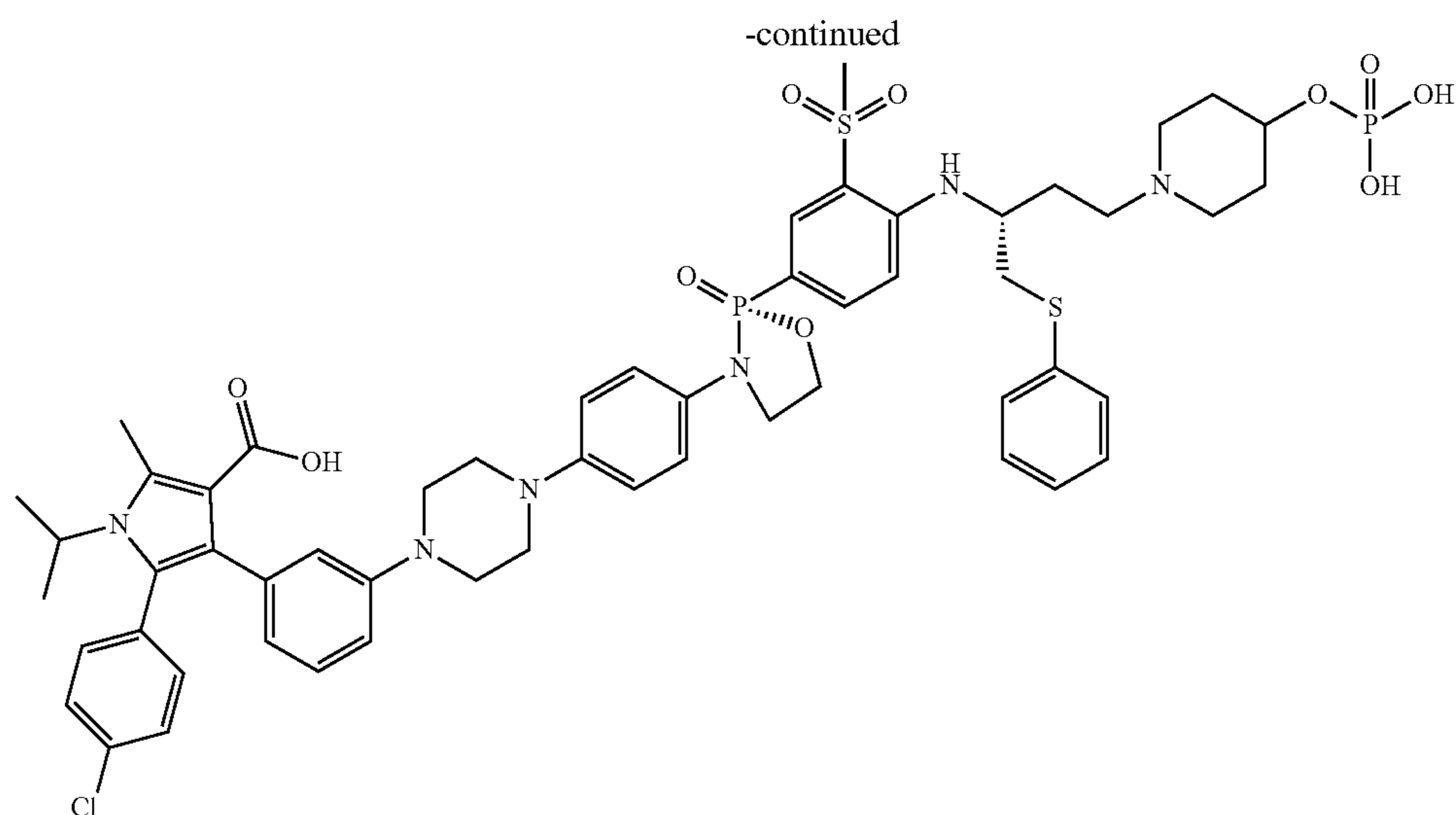
5-(4-chlorophenyl)-1-isopropyl-2-methyl-4-(3-(4-(4-((R)-2-(3-(methylsulfonyl)-4-(((R)-1-(phenylthio)-4-(4-(phosphonooxy)piperidin-1-yl)butan-2-yl)amino)phenyl)-2-oxido-1,3,2-oxazaphospholidin-3-yl)phenyl)piperazin-1-yl)phenyl)-1H-pyrrole-3-carboxylic acid
