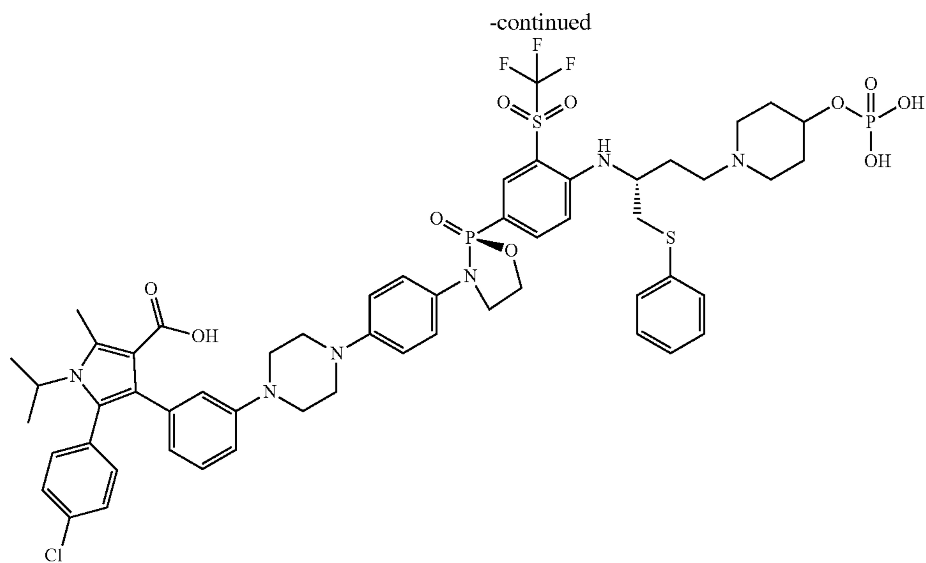
5-(4-chlorophenyl)-1-isopropyl-2-methyl-4-(3-(4-(4-((S)-2-oxido-2-(4-(((R)-1-(phenylthio)-4-(4-(phosphonoxy)piperidin-1-yl)butan-2-yl)amino)-3-((trifluoromethyl)sulfonyl)phenyl)-1,3,2-oxazaphospholidin-3-yl)phenyl)piperazin-1-yl)phenyl)-1H-pyrrole-3-carboxylic acid
