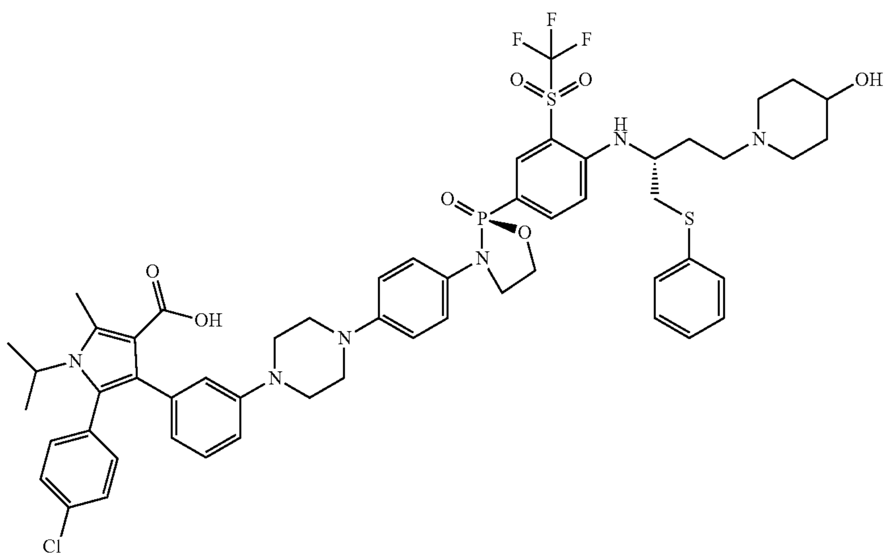
5-(4-chlorophenyl)-4-(3-(4-(4-((S)-2-(4-((R)-4-((R)-4-(4-hydroxypiperidin-1-yl)-1-(phenylthio)butan-2-yl)amino)-3-((trifluoromethyl)sulfonyl)phenyl)-2-oxido-1,3,2-oxazaphospholidin-3-yl)phenyl)piperazin-1-yl)phenyl)-1-isopropyl-2-methyl-1H-pyrrole-3-carboxylic acid
