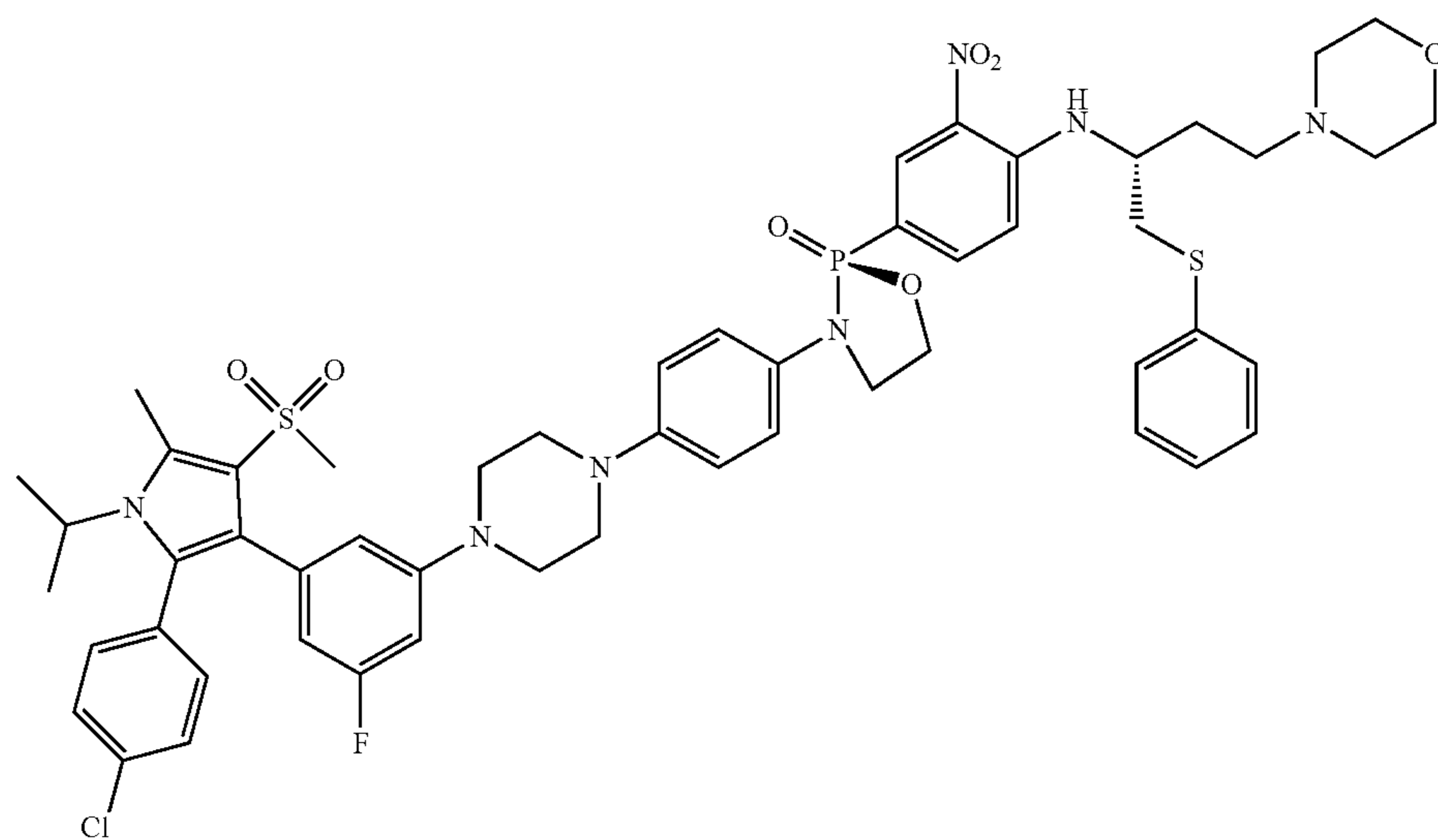
(S)-3-(4-(4-(3-(2-(4-chlorophenyl)-1-isopropyl-5-methyl-4-(methylsulfonyl)-1H-pyrrol-3-yl)-5-fluorophenyl)piperazin-1-yl)phenyl)-2-(4-(((R)-4-morpholino-1-(phenylthio)butan-2-yl)amino)-3-nitrophenyl)-1,3,2-oxazaphospholidine 2-oxide
