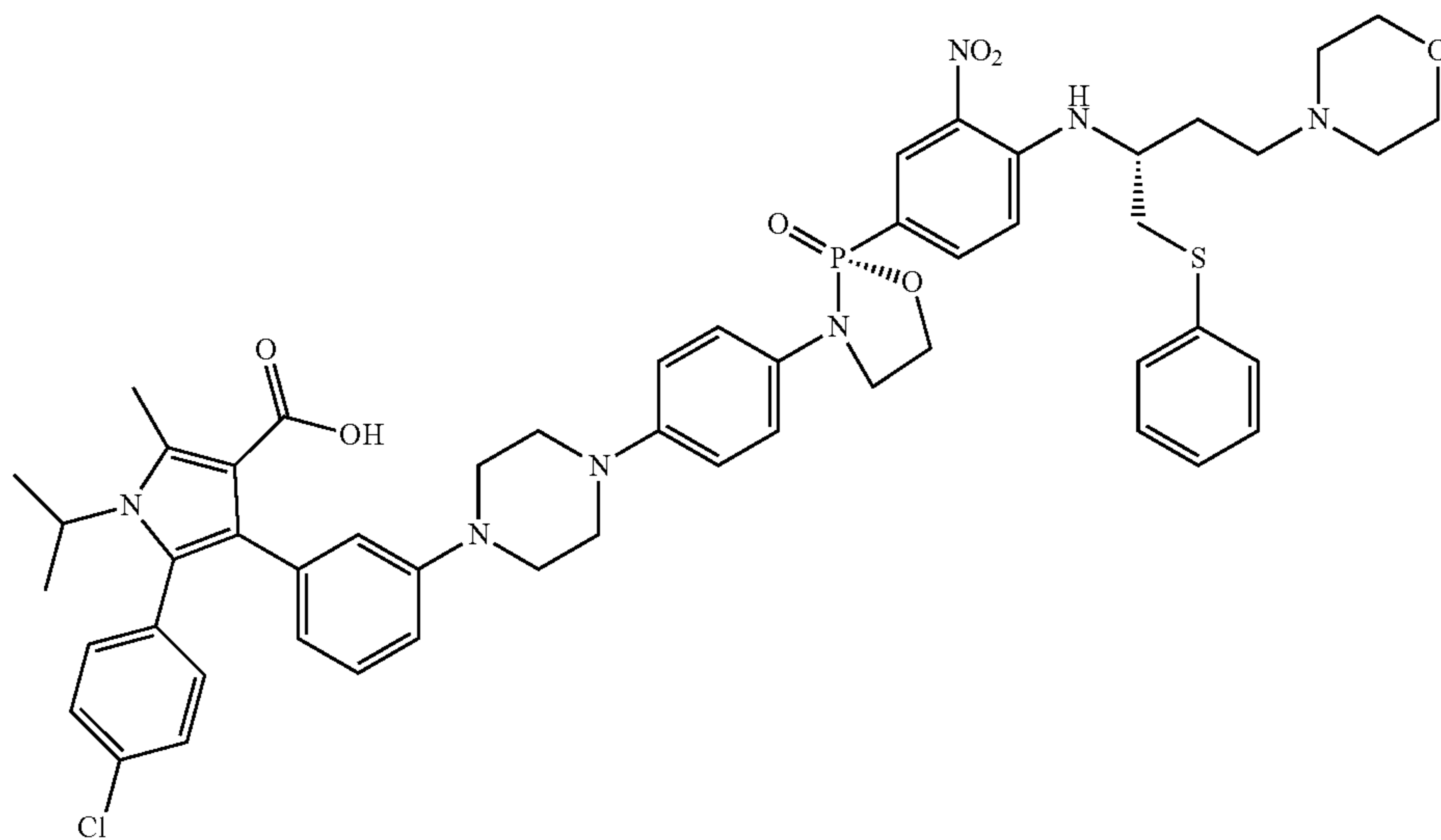
5-(4-chlorophenyl)-1-isopropyl-2-methyl-4-(3-(4-(4-((R)-2-(4-((R)-4-morpholino-1-(phenylthio)butan-2-yl)amino)-3-nitrophenyl)-2-oxido-1,3,2-oxazaphospholidin-3-yl)phenyl)piperazin-1-yl)phenyl)-1H-pyrrole-3-carboxylic acid
