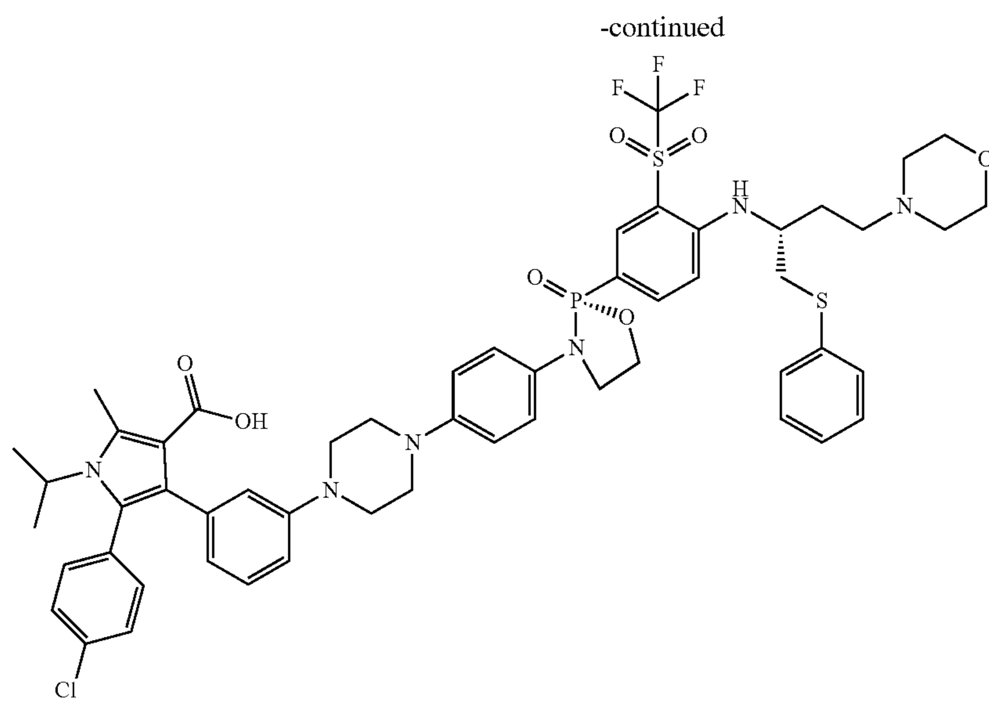
5-(4-chlorophenyl)-1-isopropyl-2-methyl-4-(3-(4-(4-((R)-2-(4-(((R)-4-morpholino-1-(phenylthio)butan-2-yl)amino)-3-((trifluoromethyl)sulfonyl)phenyl)-2-oxido-1,3,2-oxazaphospholidin-3-yl)phenyl)piperazin-1-yl)phenyl)-1H-pyrrole-3-carboxylic acid
