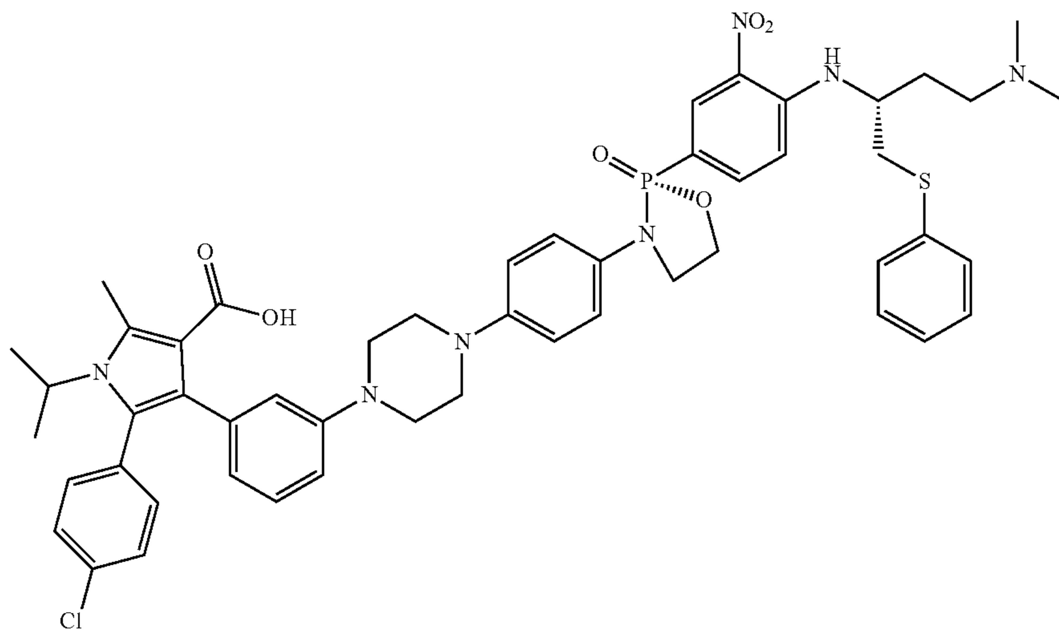
5-(4-chlorophenyl)-4-(3-(4-(4-((R)-2-(4-(((R)-4-(dimethylamino)-1-(phenylthio)butan-2-yl)amino)-3-nitrophenyl)-2-oxido-1,3,2-oxazaphospholidin-3-yl)phenyl)piperazin-1-yl)phenyl)-1-isopropyl-2-methyl-1H-pyrrole-3-carboxylic acid
