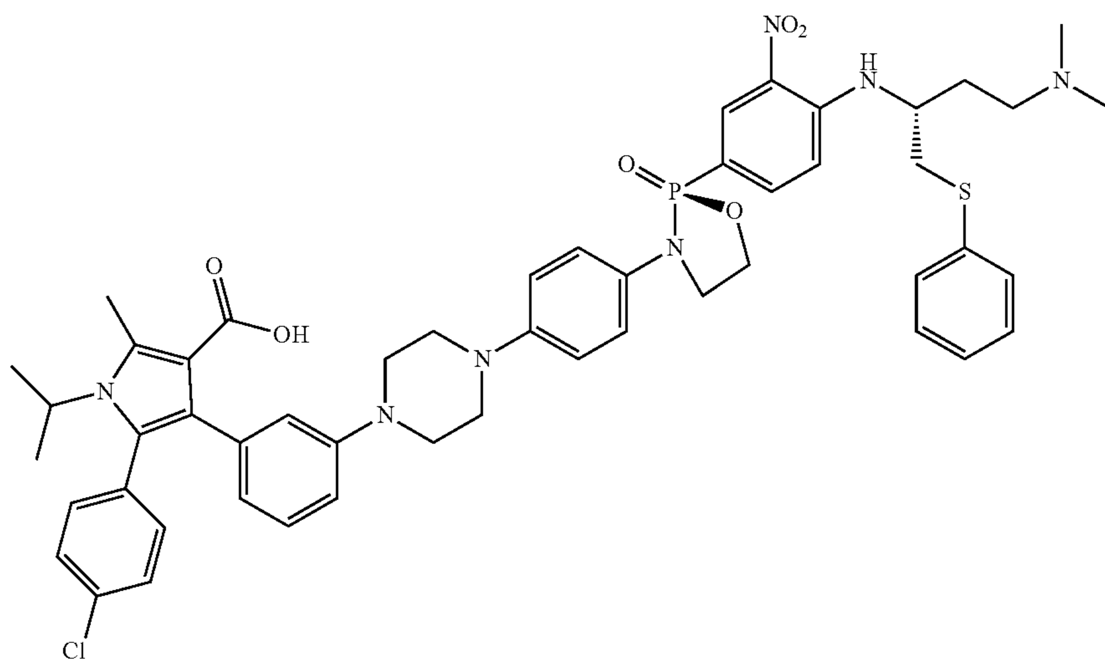
5-(4-chlorophenyl)-4-(3-(4-(4-((S)-2-((S)-2-(4-(((R)-4-(dimethylamino)-1-(phenylthio)butan-2-yl)amino)-3-nitrophenyl)-2-oxido-1,3,2-oxazaphospholidin-3-yl)phenyl)piperazin-1-yl)phenyl)-1-isopropyl-2-methyl-1H-pyrrole-3-carboxylic acid
