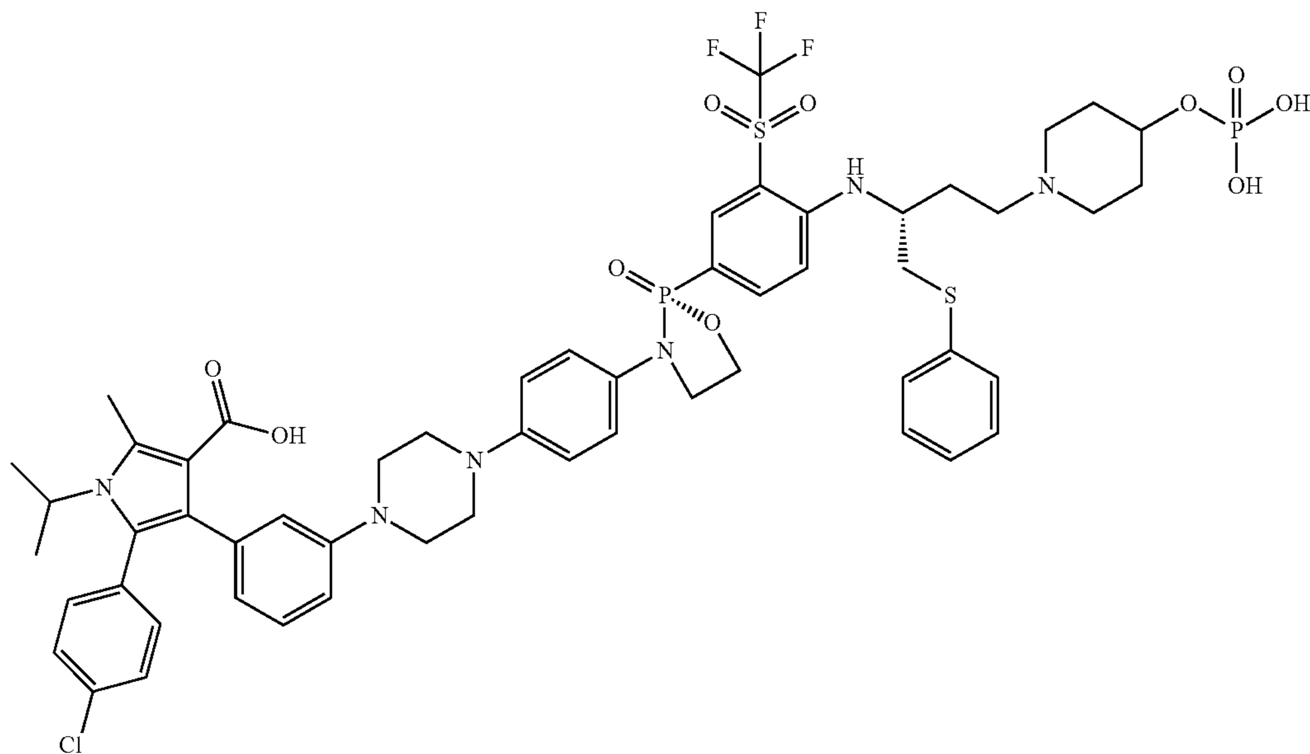
5-(4-chlorophenyl)-1-isopropyl-2-methyl-4-(3-(4-(4-((R)-2-oxido-2-(4-(((R)-1-(phenylthio)-4-(4-(phosphonoxy)piperidin-1-yl)butan-2-yl)amino)-3-((trifluoromethyl)sulfonyl)phenyl)-1,3,2-oxazaphospholidin-3-yl)phenyl)piperazin-1-yl)phenyl)-1H-pyrrole-3-carboxylic acid,
