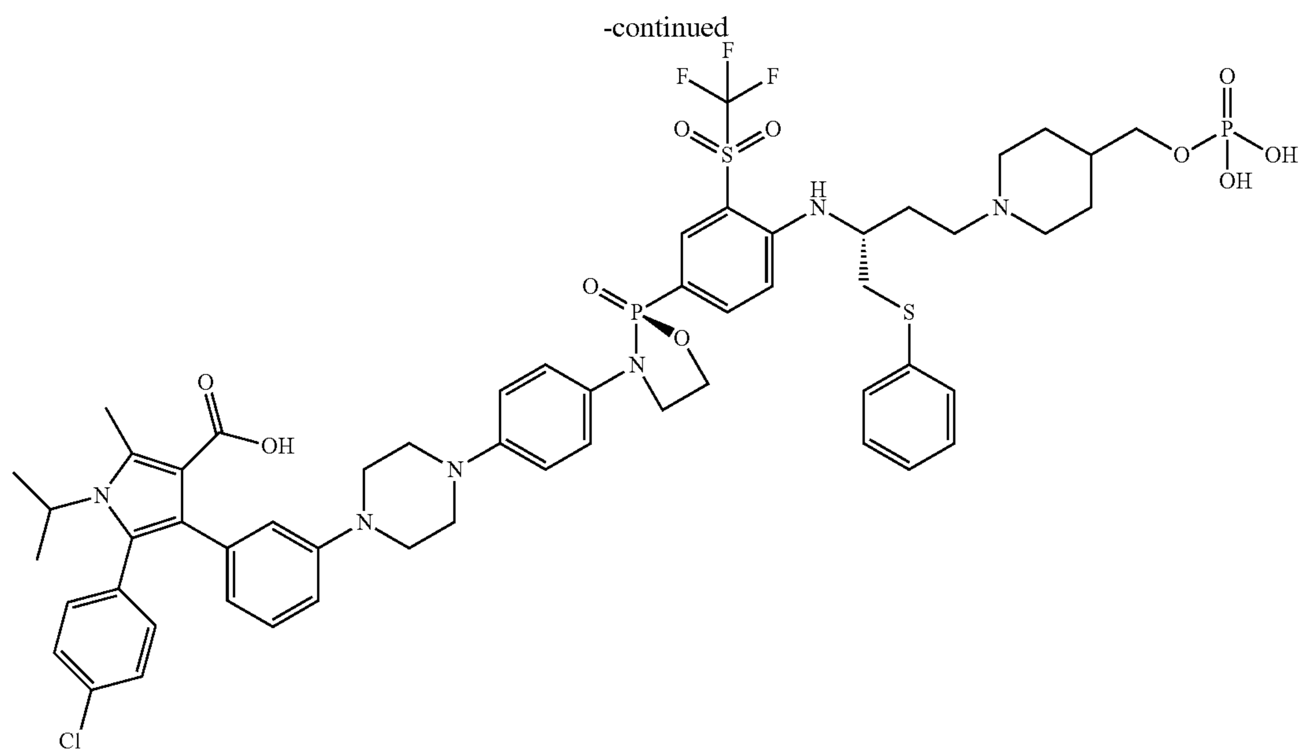
5-(4-chlorophenyl)-1-isopropyl-2-methyl-4-(3-(4-(4-((S)-2-oxido-2-(4-(((R)-1-(phenylthio)-4-(4-(phosphonooxy)methyl)piperidin-1-yl)butan-2-yl)amino-3-(trifluoromethyl)sulfonyl)phenyl)-1,3,2-oxazaphospholidin-3-yl)phenyl)piperazin-1-yl)phenyl)-1H-pyrrole-3-carboxylic acid,
