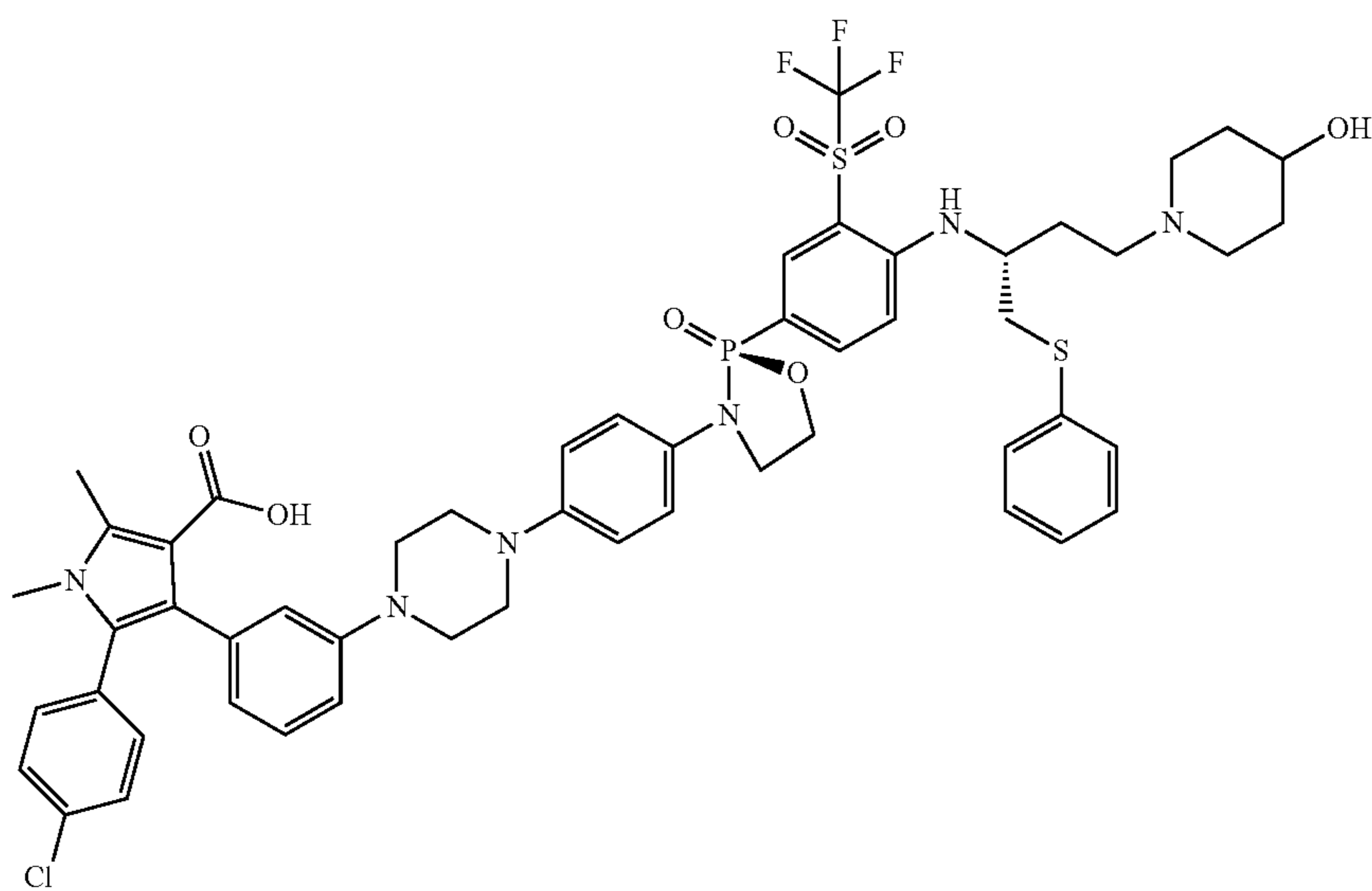
5-(4-chlorophenyl)-1-ethyl-4-(3-(4-(4-((S)-2-(4-((R)-4-(4-hydroxypiperidin-1-yl)-1-(phenylthio)butan-2-yl)amino)-3-((trifluoromethyl)sulfonyl)phenyl)-2-oxido-1,3,2-oxazaphospholidin-3-yl)phenyl)piperazin-1-yl)phenyl)-2-dimethyl-1H-pyrrole-3-carboxylic acid
