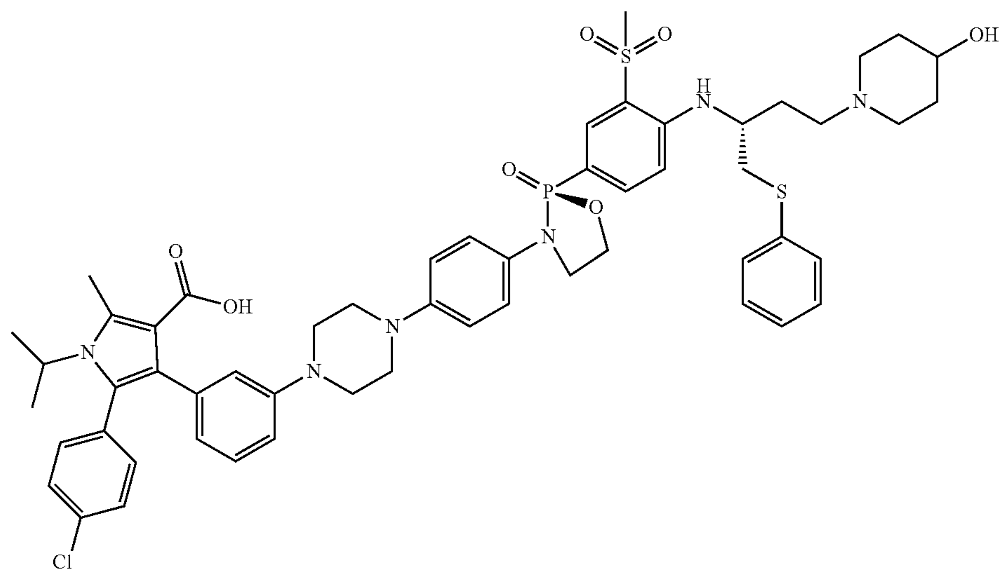
5-(4-chlorophenyl)-4-(3-(4-(4-((S)-2-(4-(((R)-4-(4-(hydroxypiperidin-1-yl)-1-(phenylthio)butan-2-yl)amino)-3-(methylsulfonyl)phenyl)-2-oxido-1,3,2-oxazaphospholidin-3-yl)phenyl)piperazin-1-yl)phenyl)-1-isopropyl-2-methyl-1H-pyrrole-3-carboxylic acid
