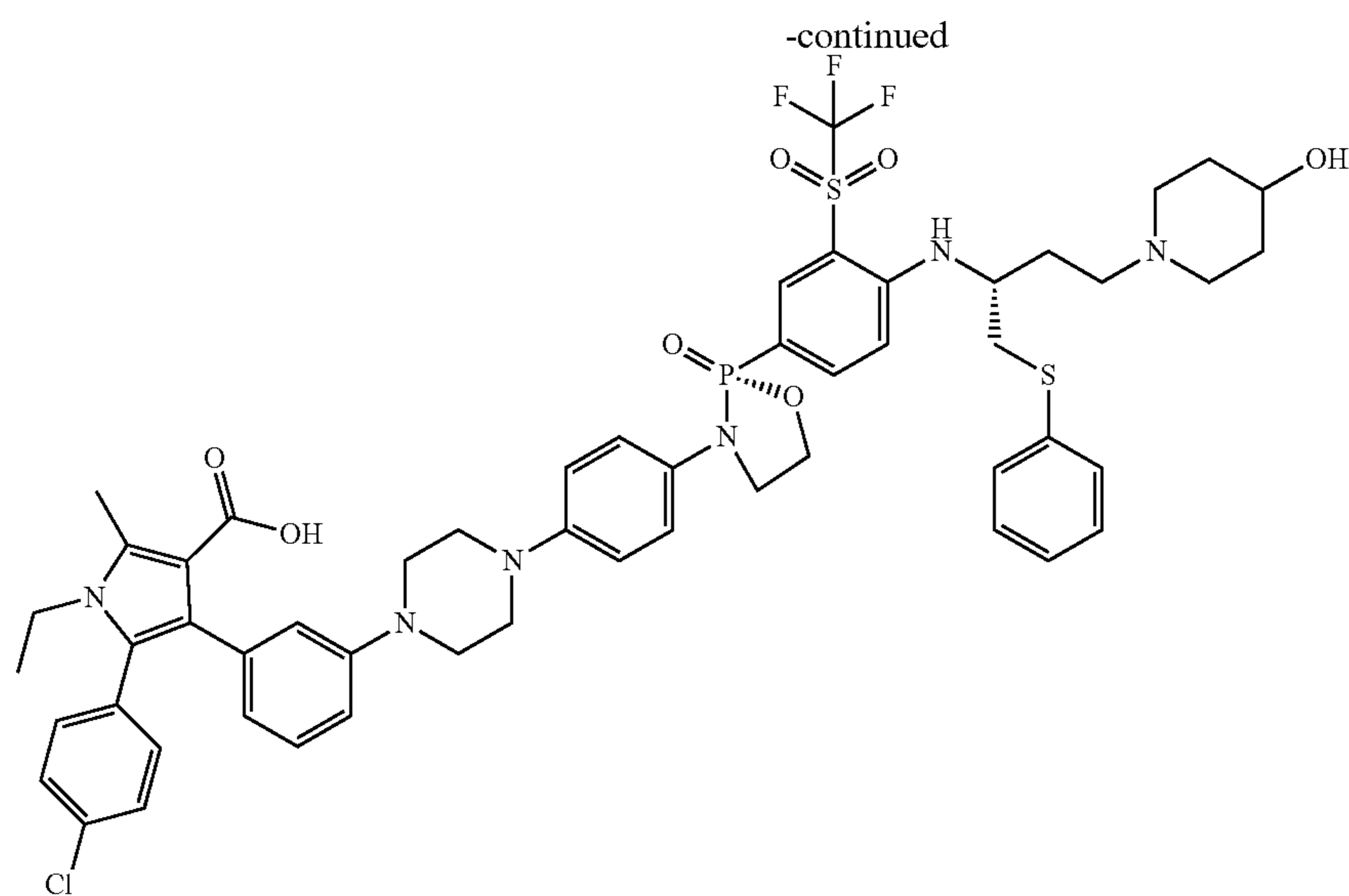
5-(4-chlorophenyl)-1-ethyl-4-(3-(4-(4-((R)-2-(4-((R)-4-(4-hydroxypiperidin-1-yl)-1-(phenylthio)butan-2-yl)amino)-3-((trifluoromethyl)sulfonyl)phenyl)-2-oxido-1,3,2-oxazaphospholidin-3-yl)phenyl)piperazin-1-yl)phenyl)-2-methyl-1H-pyrrole-3-carboxylic acid
