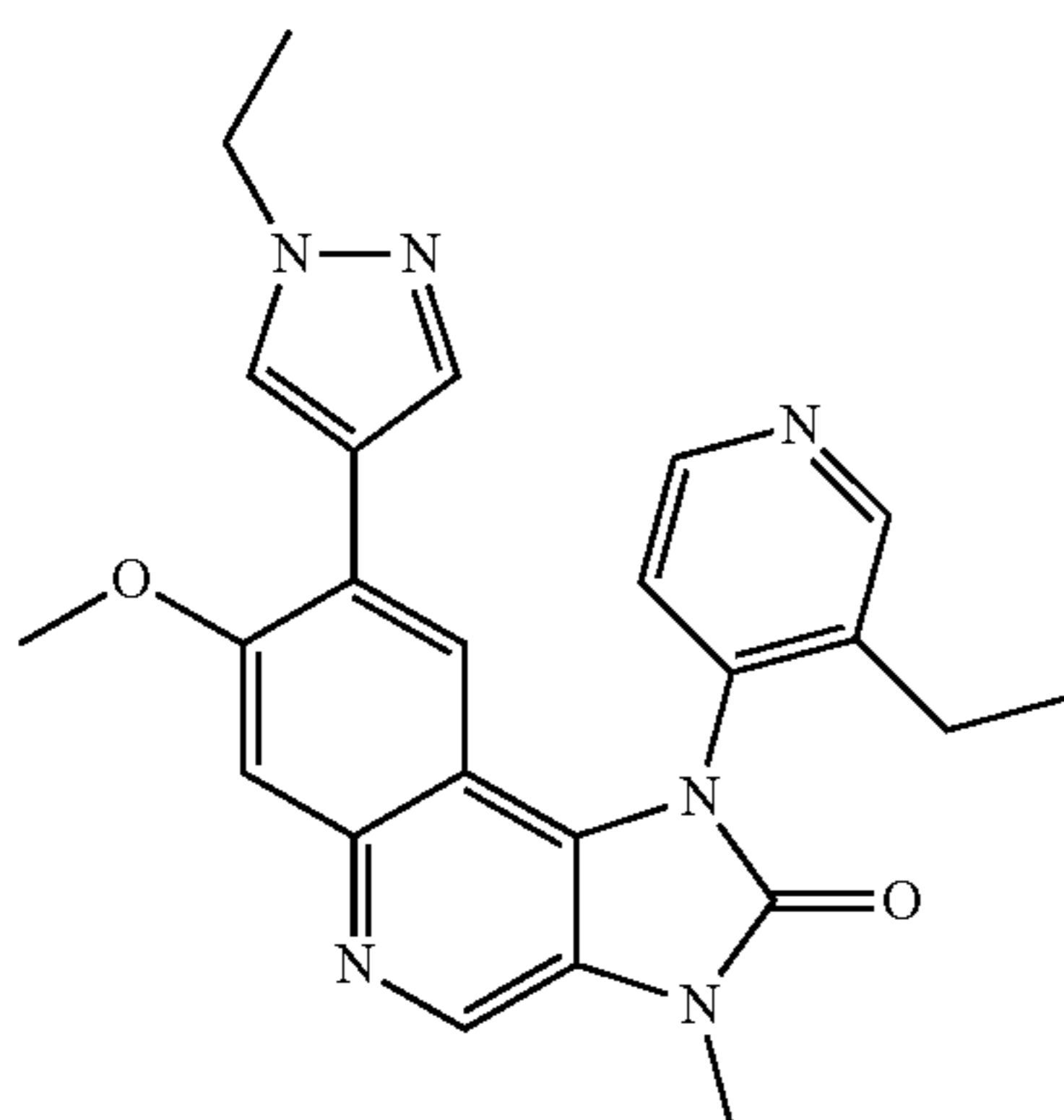
8-(1-Ethyl-1H-pyrazol-4-yl)-1-(3-ethylpyridin-4-yl)-7-methoxy-3-methyl-1,3-dihydroimidazo[4,5-c]quinolin-2-one
