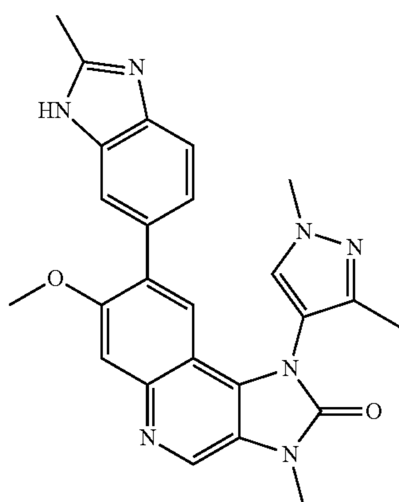
1-(1,3-Dimethyl-1H-pyrazol-4-yl)-7-methoxy-3-methyl-8-(2-methyl-3H-benzimidazol-5-yl)-1,3-dihydroimidazo[4,5-c]quinolin-2-one
