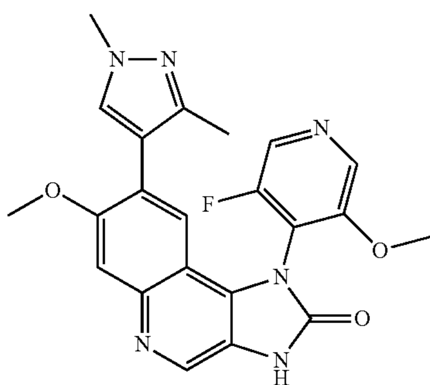
8-(1,3-Dimethyl-1H-pyrazol-4-yl)-1-(3-fluoro-5-methoxy-pyridin-4-yl)-7-methoxy-1,3-dihydroimidazo[4,5-c]quinolin-2-one
