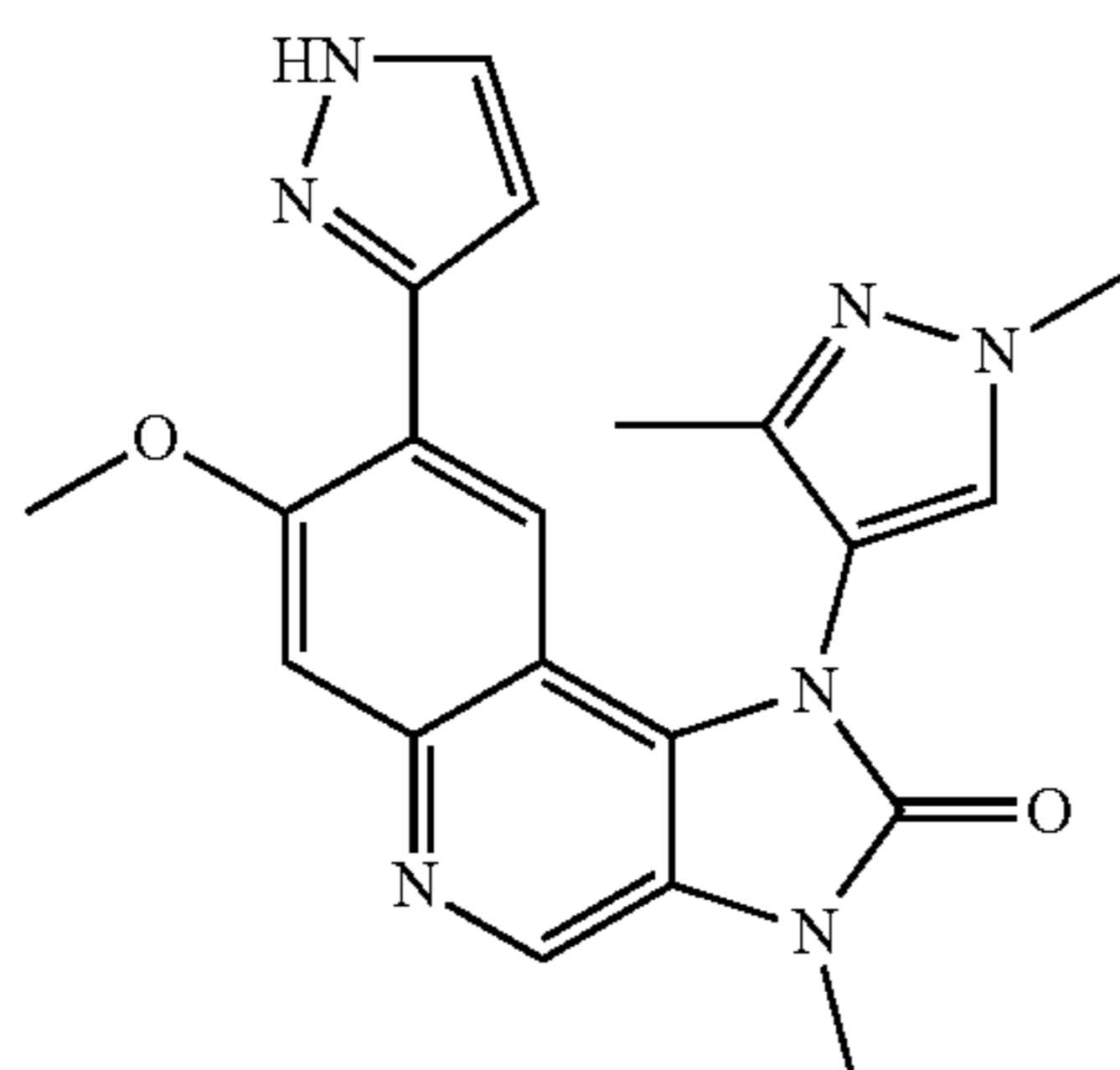
1-(1,3-Dimethyl-1H-pyrazol-4-yl)-7-methoxy-3-methyl-8-(1H-pyrazol-3-yl)-1,3-dihydroimidazo[4,5-c]quinolin-2-one
