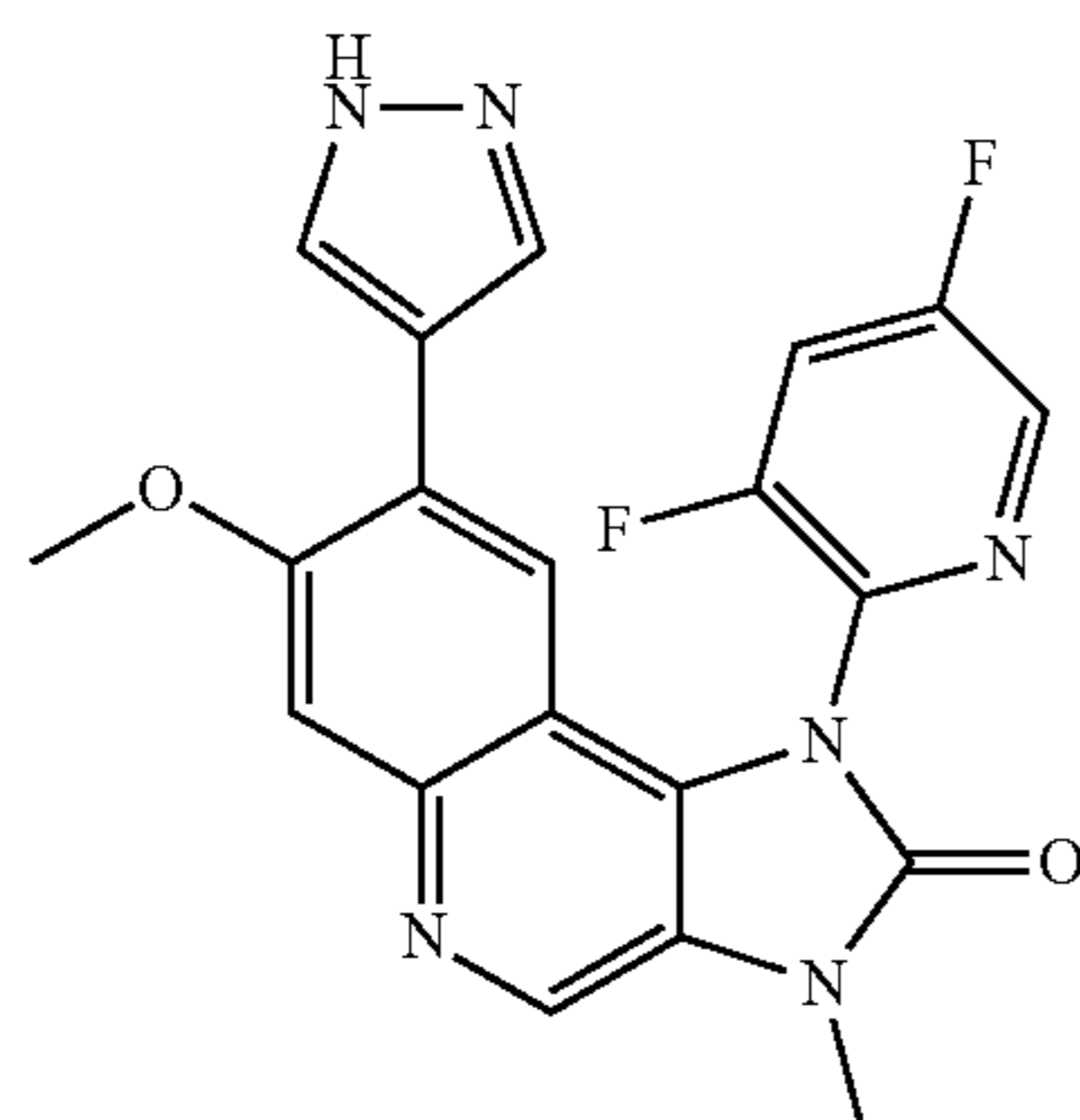
1-(3,5-Difluoropyridin-2-yl)-7-methoxy-3-methyl-8-(1H-pyrazol-4-yl)-1,3-dihydroimidazo[4,5-c]quinolin-2-one
