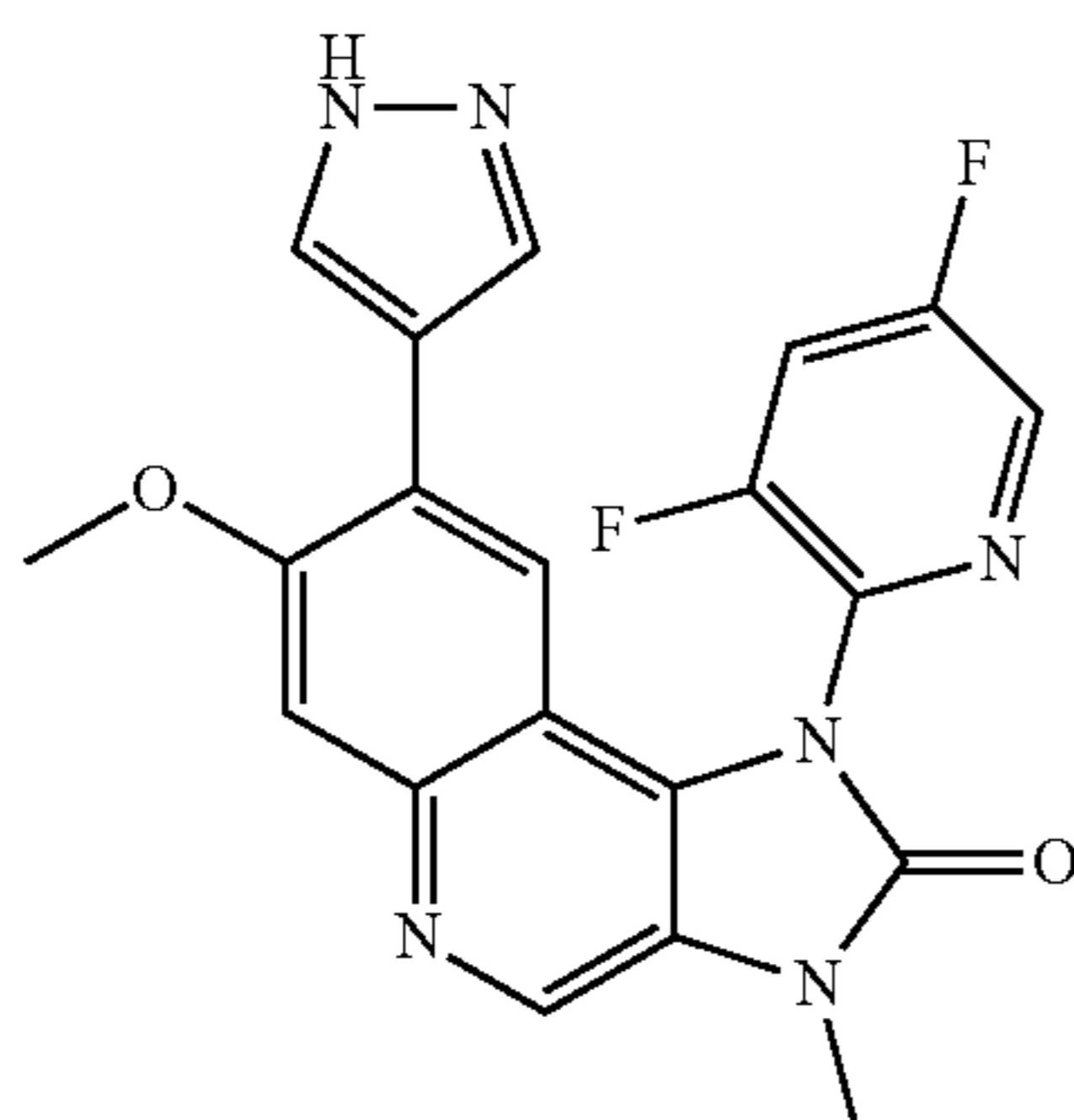
1-(3,5-Difluoropyridin-2-yl)-7-methoxy-3-methyl-8-(1H-pyrazol-4-yl)-1,3-dihydroimidazo[4,5-c]quinolin-2-one
