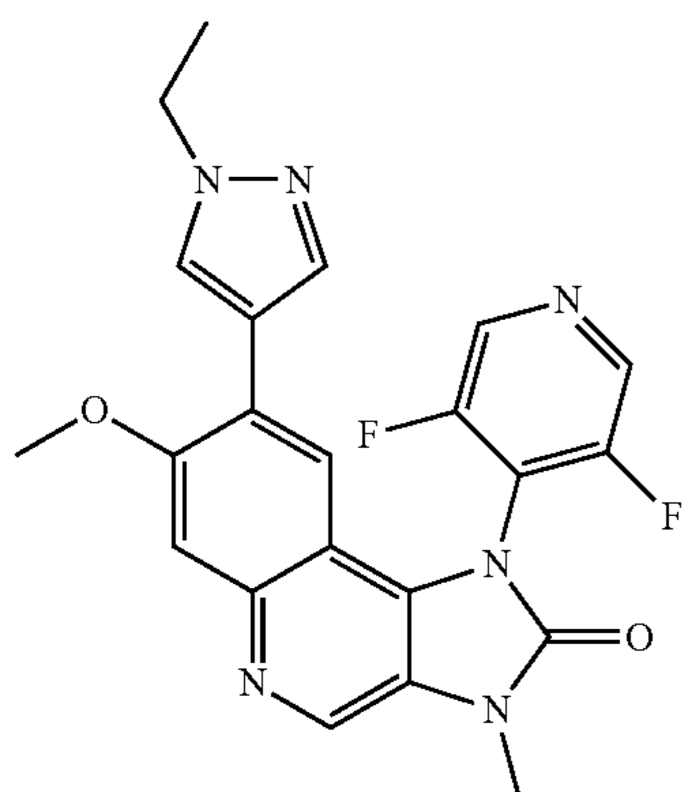
1-(3,5-Difluoropyridin-4-yl)-8-(1-ethyl-1H-pyrazol-4-yl)-7-methoxy-3-methyl-1,3-dihydroimidazo[4,5-c]quinolin-2-one
