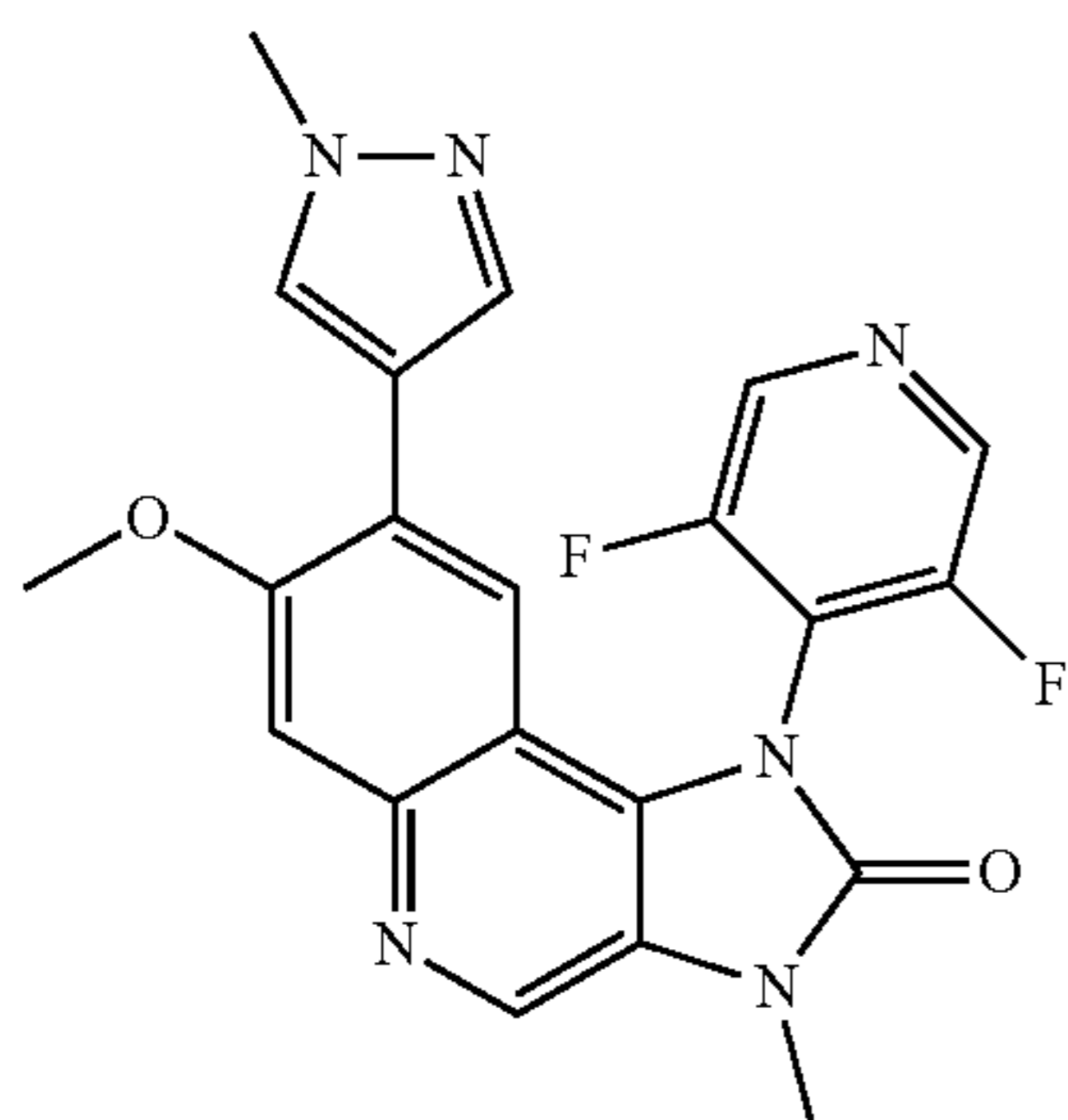
1-(3,5-Difluoropyridin-4-yl)-7-methoxy-3-methyl-8-(1-methyl-1H-pyrazol-4-yl)-1,3-dihydroimidazo[4,5-c]quinolin-2-one
