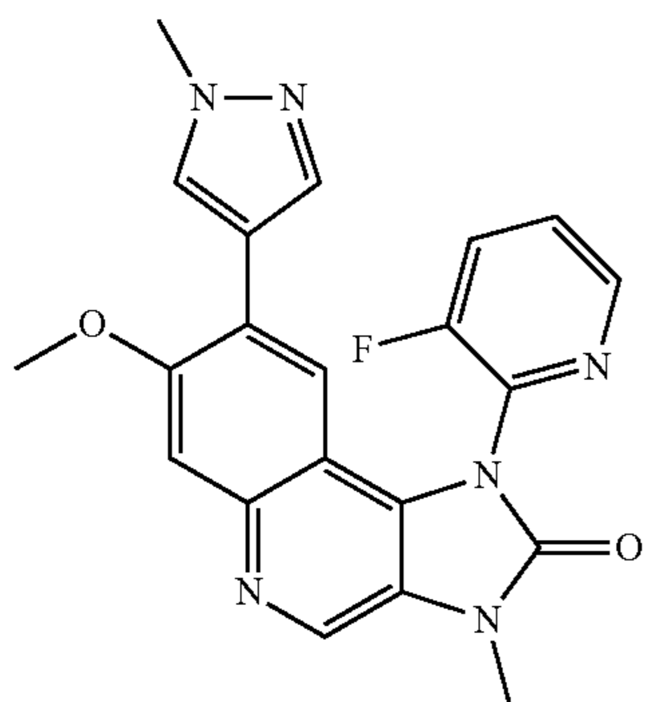
1-(3-Fluoropyridin-2-yl)-7-methoxy-3-methyl-8-(1-methyl-1H-pyrazol-4-yl)-1,3-dihydroimidazo[4,5-c]quinolin-2-one
