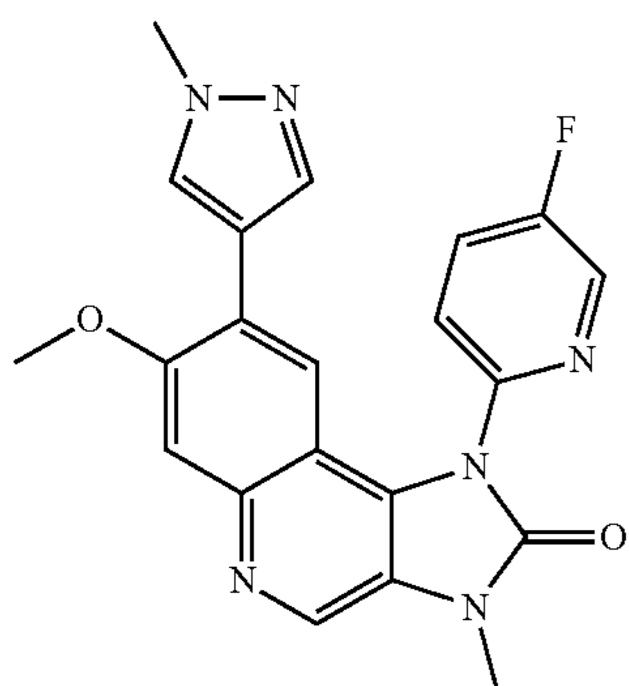
1-(5-Fluoropyridin-2-yl)-7-methoxy-3-methyl-8-(1-methyl-1H-pyrazol-4-yl)-1,3-dihydroimidazo[4,5-c]quinolin-2-one
