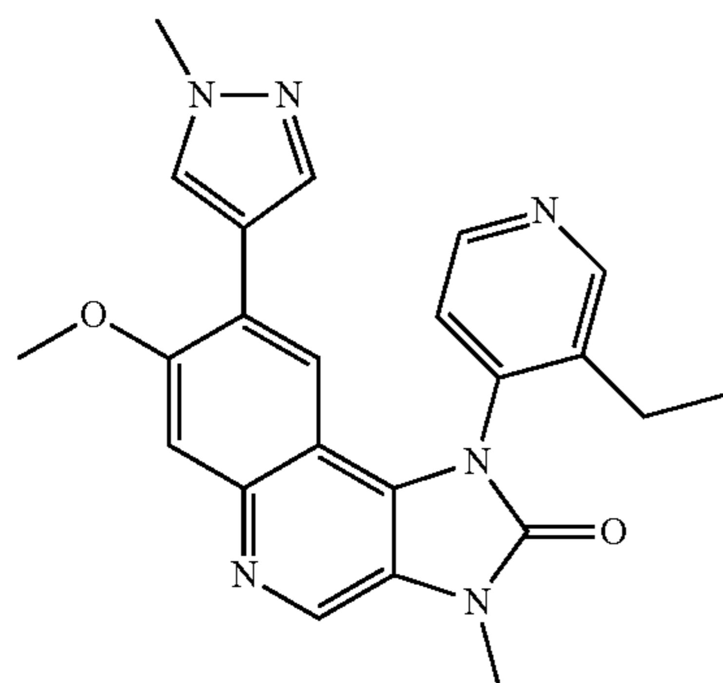
1-(3-Ethylpyridin-4-yl)-7-methoxy-3-methyl-8-(1-methyl-1H-pyrazol-4-yl)-1,3-dihydroimidazo[4,5-c]quinolin-2-one
