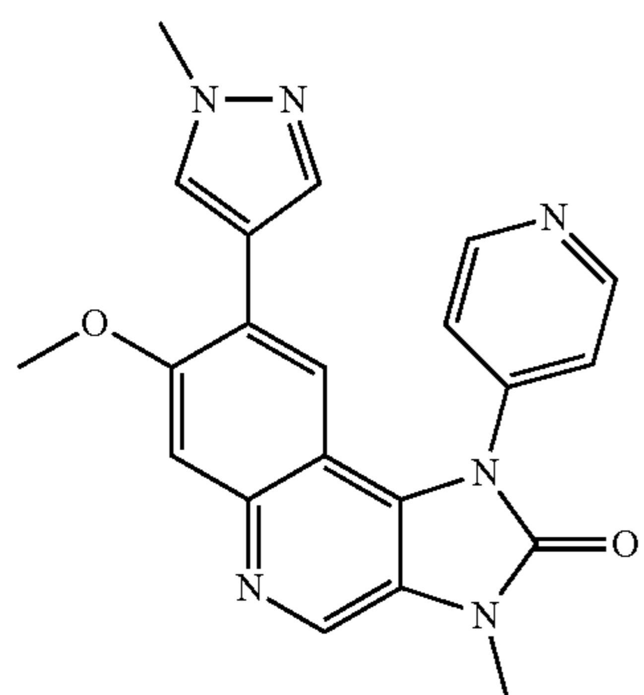
7-Methoxy-3-methyl-8-(1-methyl-1H-pyrazol-4-yl)-1-pyridin-4-yl-1,3-dihydroimidazo[4,5-c]quinolin-2-one
