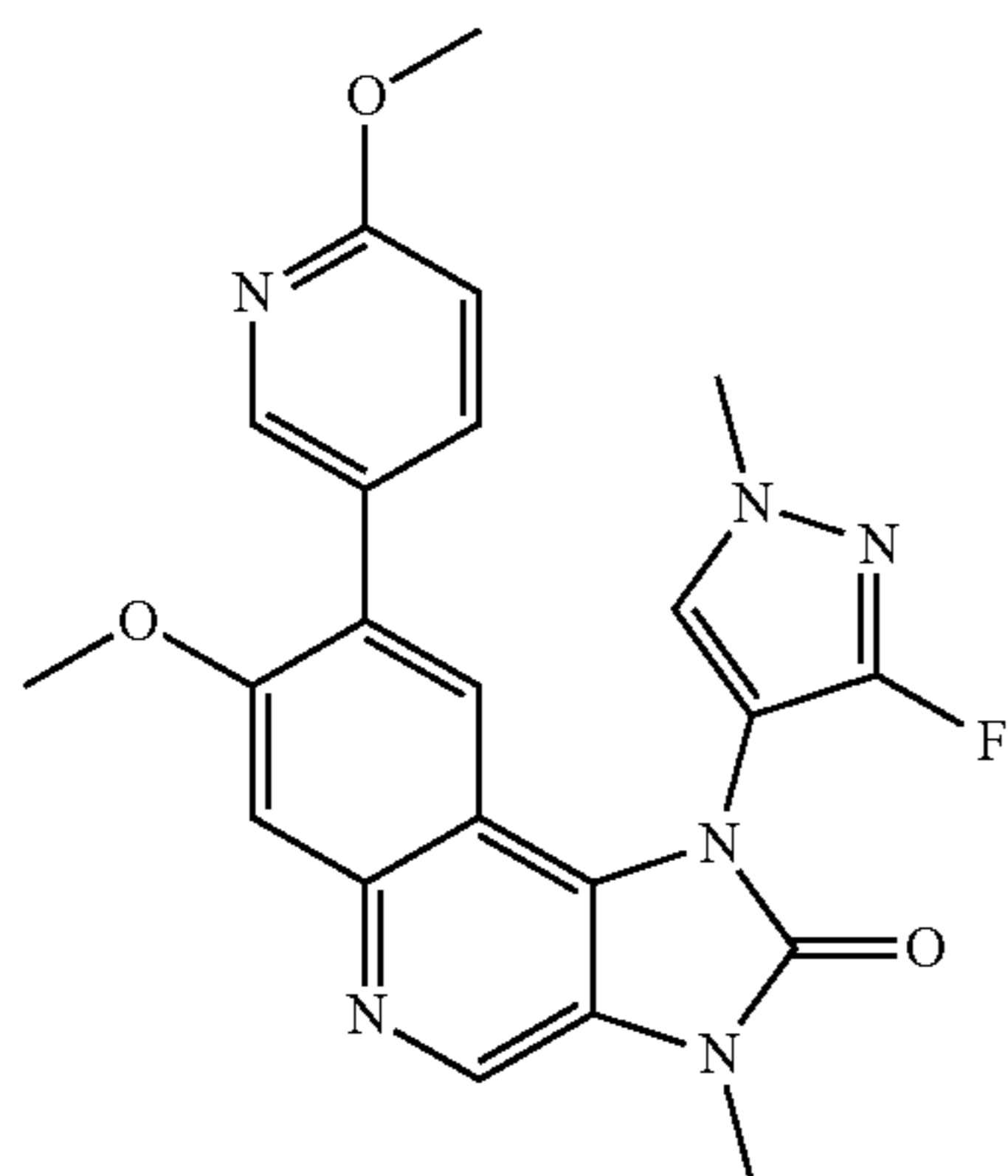
1-(3-Fluoro-1-methyl-1H-pyrazol-4-yl)-7-methoxy-8-(6-methoxypyridin-3-yl)-3-methyl-1,3-dihydroimidazo[4,5-c]quinolin-2-one
