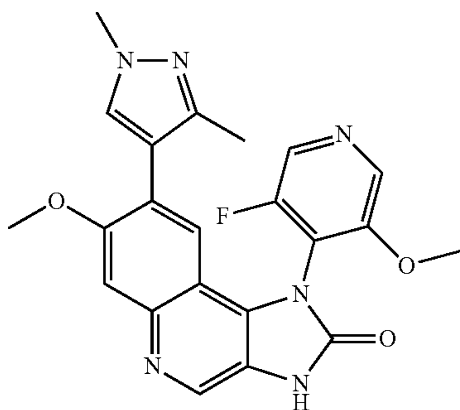
8-(1,3-Dimethyl-1H-pyrazol-4-yl)-1-(3-fluoro-5-methoxy-pyridin-4-yl)-7-methoxy-1,3-dihydroimidazo[4,5-c]quinolin-2-one
