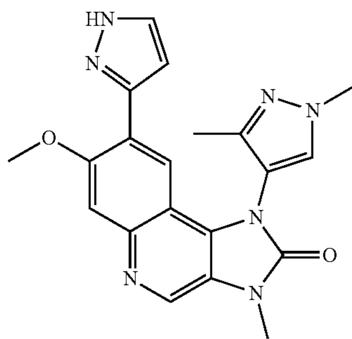
1-(1,3-Dimethyl-1H-pyrazol-4-yl)-7-methoxy-3-methyl-8-(1H-pyrazol-3-yl)-1,3-dihydroimidazo[4,5-c]quinolin-2-one
