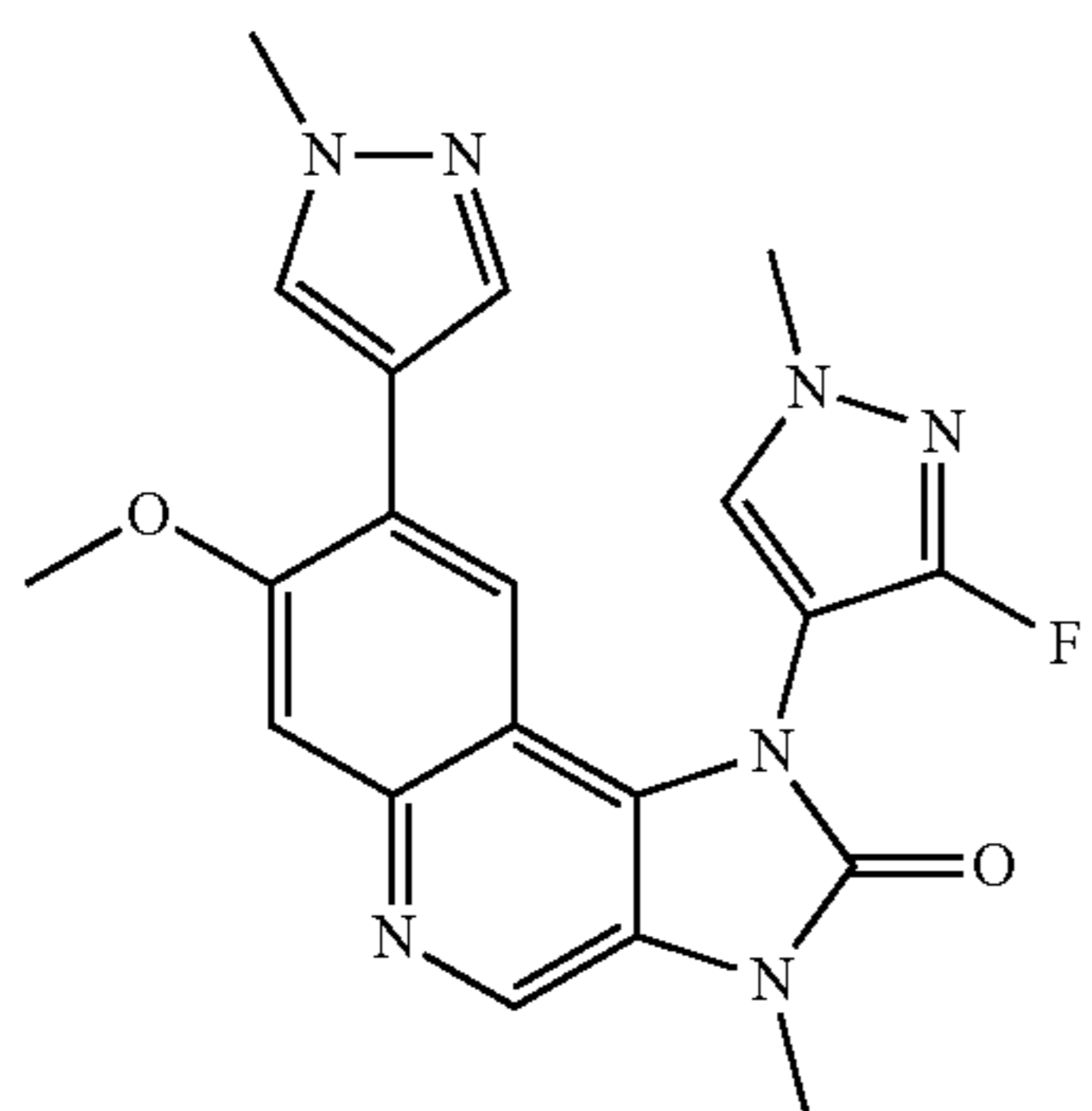
1-(3-Fluoro-1-methyl-1H-pyrazol-4-yl)-7-methoxy-3-methyl-8-(1-methyl-1H-pyrazol-4-yl)-1,3-dihydroimidazo[4,5-c]quinolin-2-one
