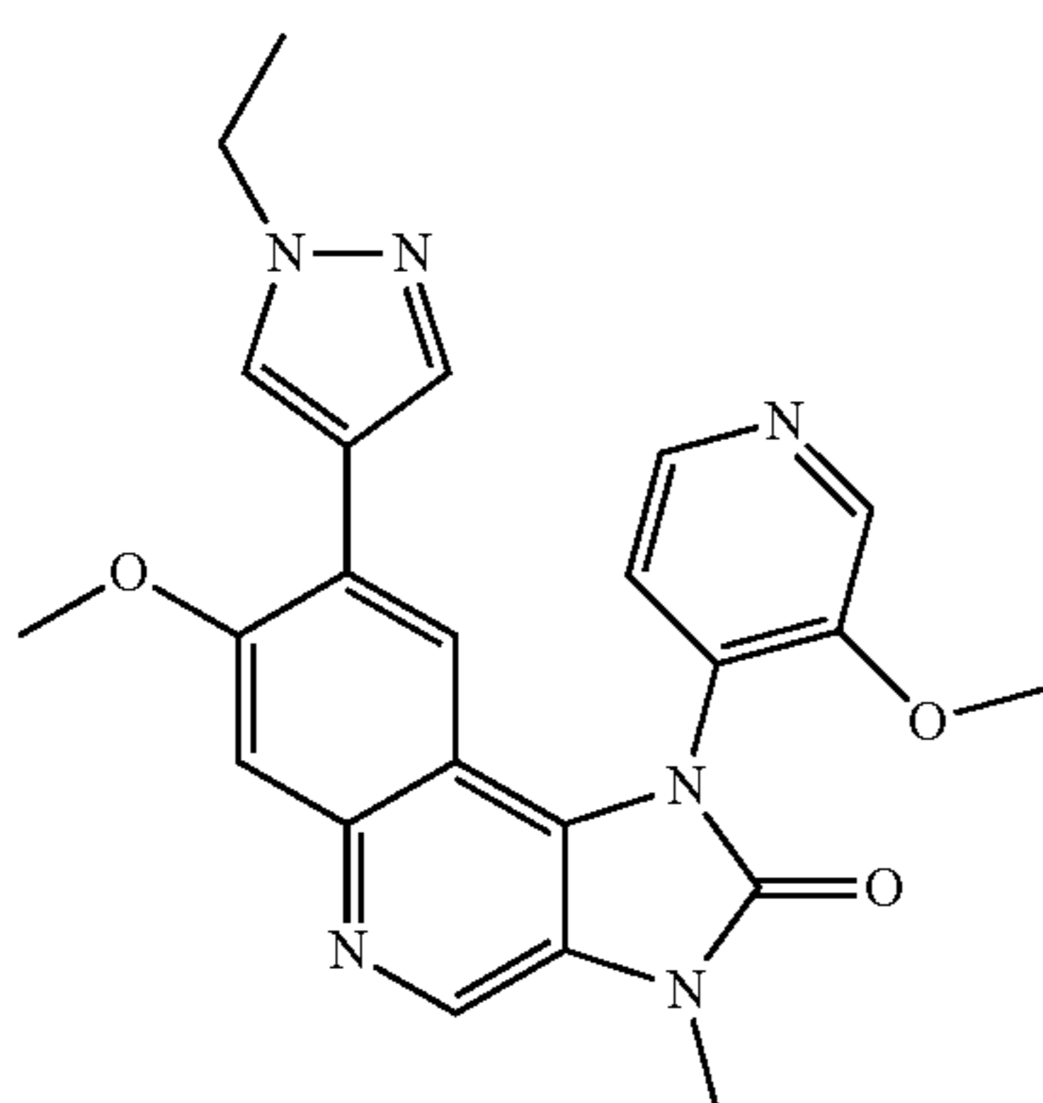
8-(1-Ethyl-1H-pyrazol-4-yl)-7-methoxy-1-(3-methoxypyridin-4-yl)-3-methyl-1,3-dihydroimidazo[4,5-c]quinolin-2-one
