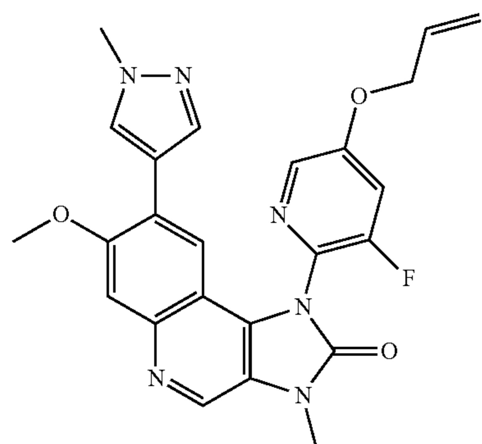
1-(5-Allyloxy-3-fluoropyridin-2-yl)-7-methoxy-3-methyl-8-(1-methyl-1H-pyrazol-4-yl)-1,3-dihydroimidazo[4,5-c]quinolin-2-one
