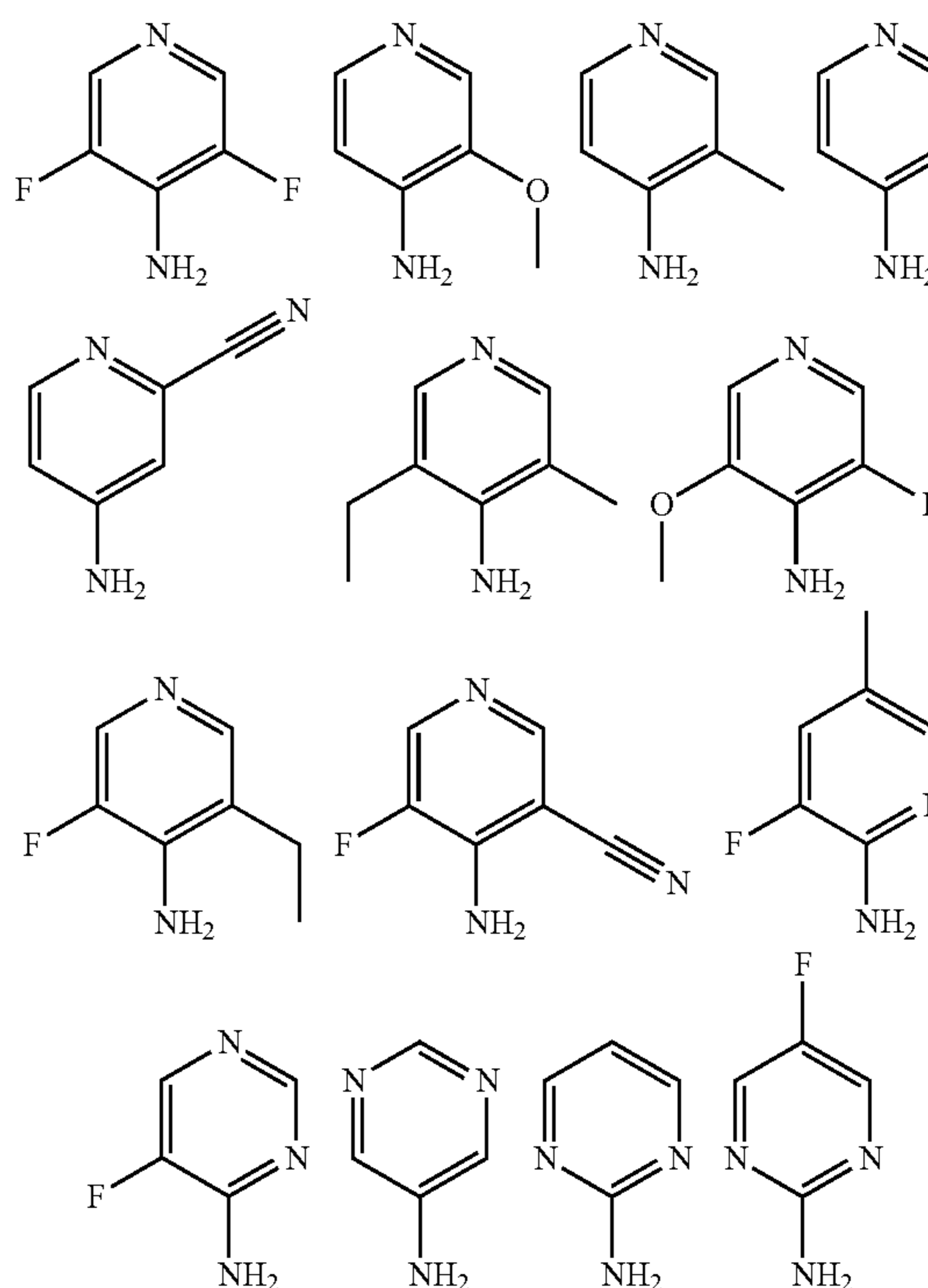
Schems 4 Amine derivatives, boronic acid esters or analogues
