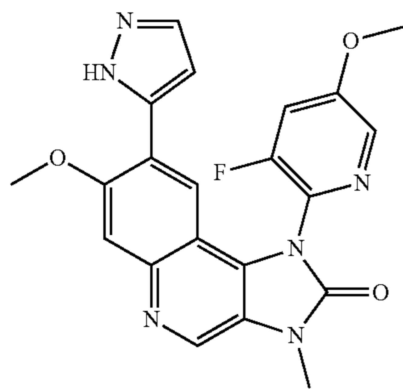
1-(3-Fluoro-5-methoxypyridin-2-yl)-7-methoxy-3-methyl-8-(2H-pyrazol-3-yl)-1,3-dihydroimidazo[4,5-c]quinolin-2-one
