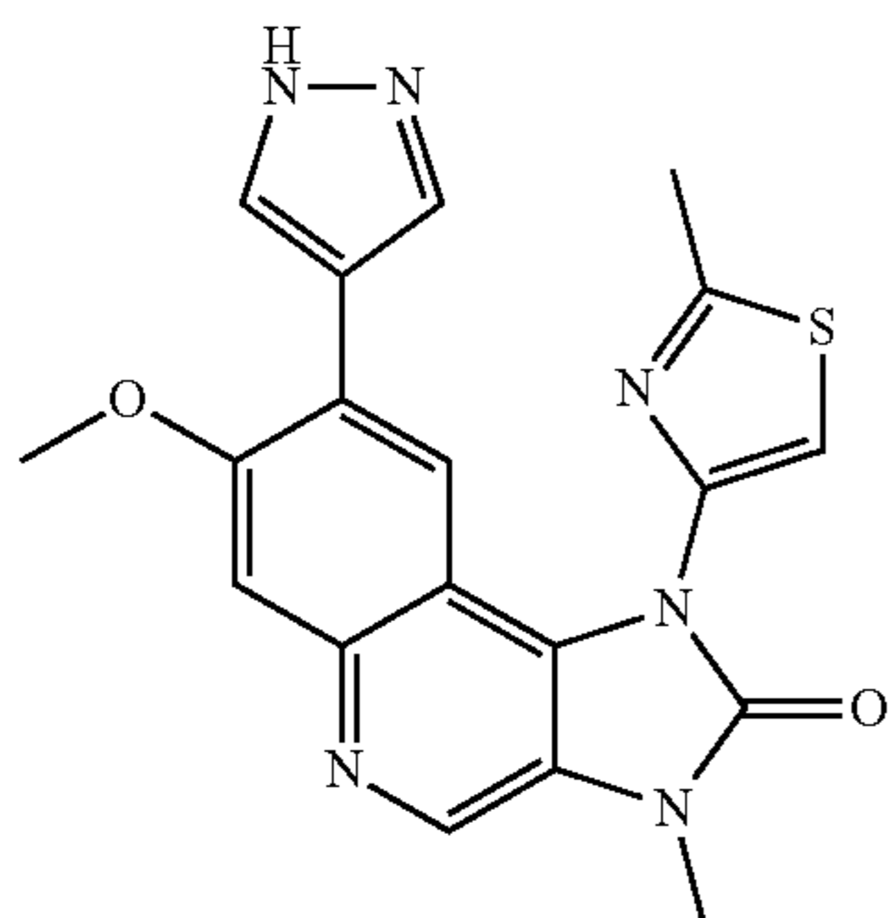
7-Methoxy-3-methyl-1-(2-methylthiazol-4-yl)-8-(1H-pyrazol-4-yl)-1,3-dihydroimidazo[4,5-c]quinolin-2-one
