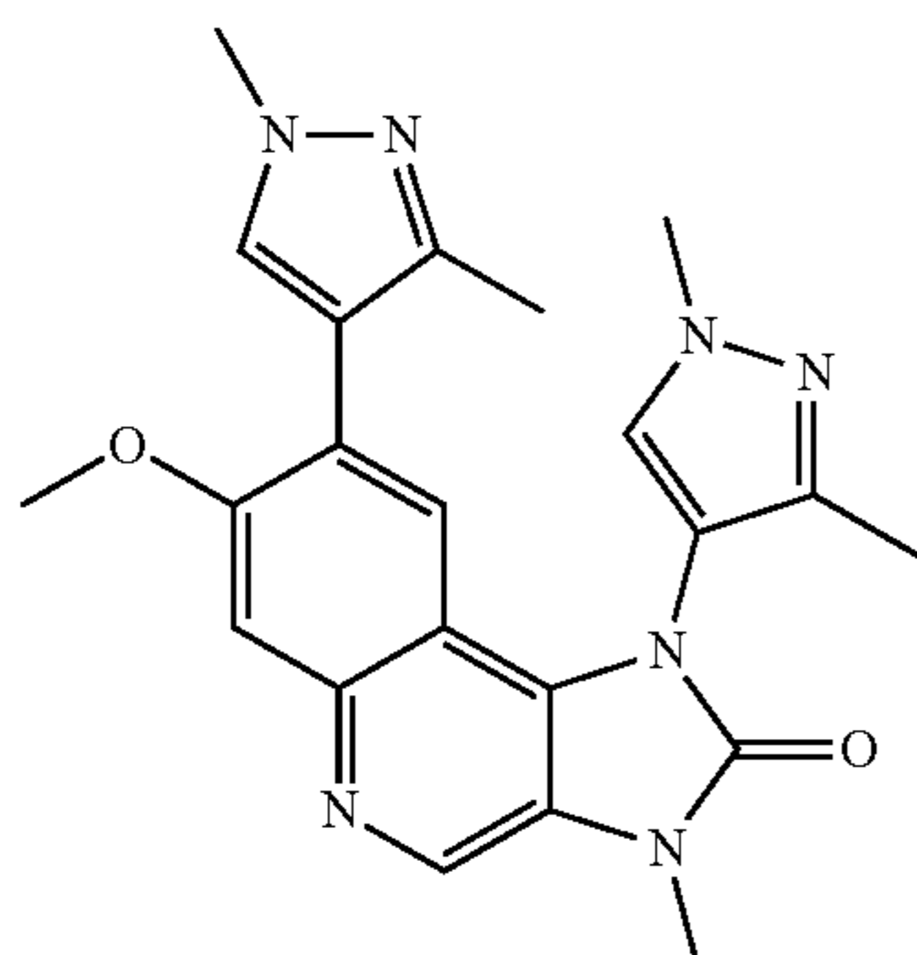
1,8-Bis(1,3-dimethyl-1H-pyrazol-4-yl)-7-methoxy-3-methyl-1,3-dihydroimidazo[4,5-c]quinolin-2-one
