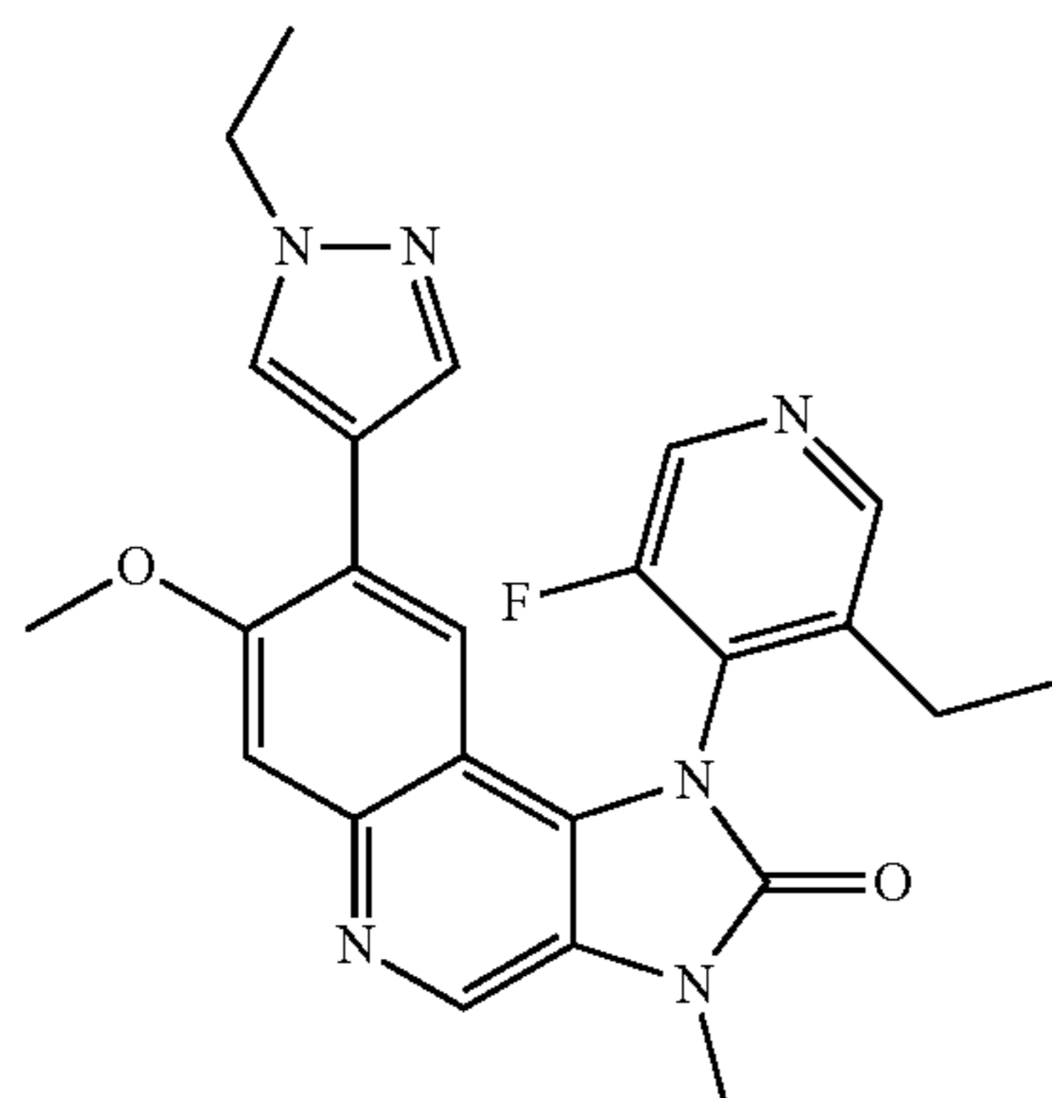
1-(3-Ethyl-5-fluoropyridin-4-yl)-8-(1-ethyl-1H-pyrazol-4-yl)-7-methoxy-3-methyl-1,3-dihydroimidazo[4,5-c]quinolin-2-one
