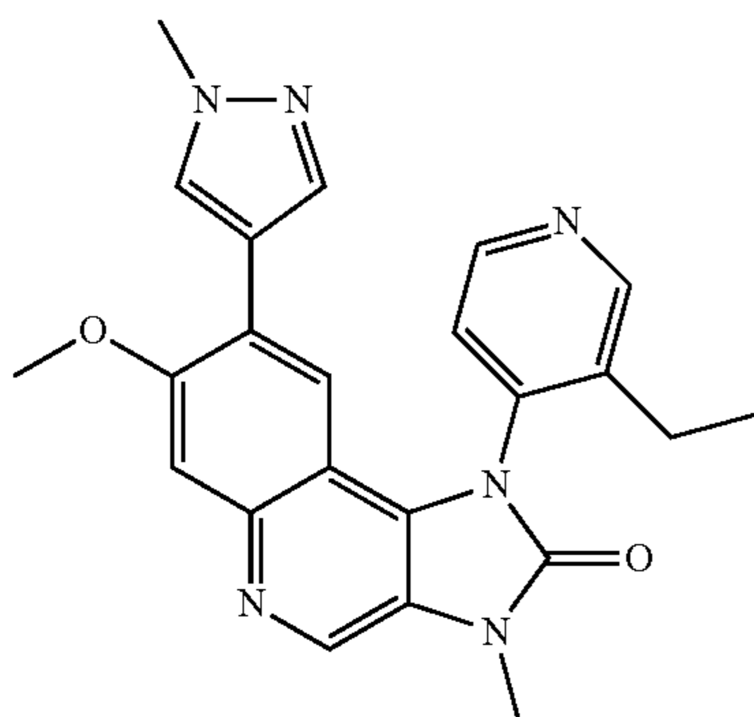
1-(3-Ethylpyridin-4-yl)-7-methoxy-3-methyl-8-(1-methyl-1H-pyrazol-4-yl)-1,3-dihydroimidazo[4,5-c]quinolin-2-one
