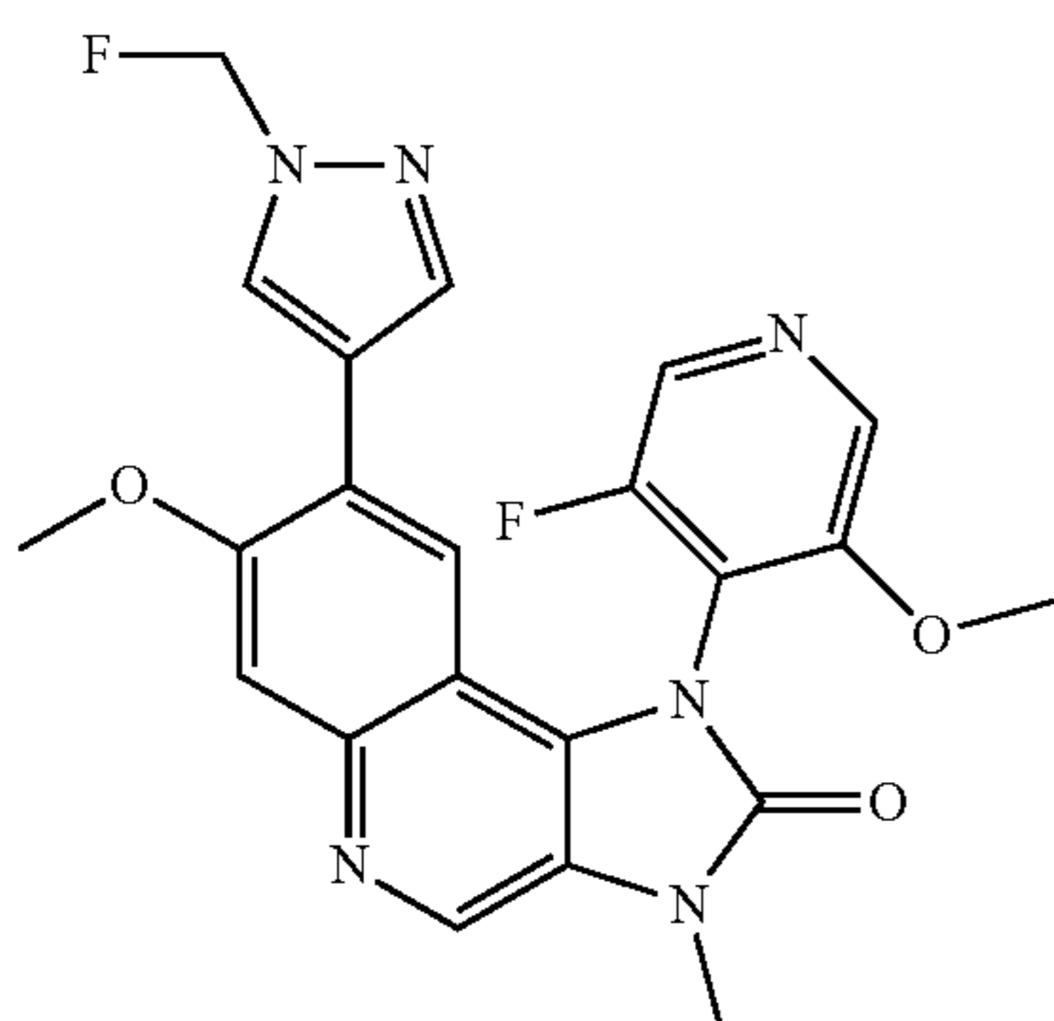
1-(3-Fluoro-5-methoxypyridin-4-yl)-8-(1-fluoromethyl-1H-pyrazol-4-yl)-7-methoxy-3-methyl-1,3-dihydroimidazo[4,5-c]quinolin-2-one
