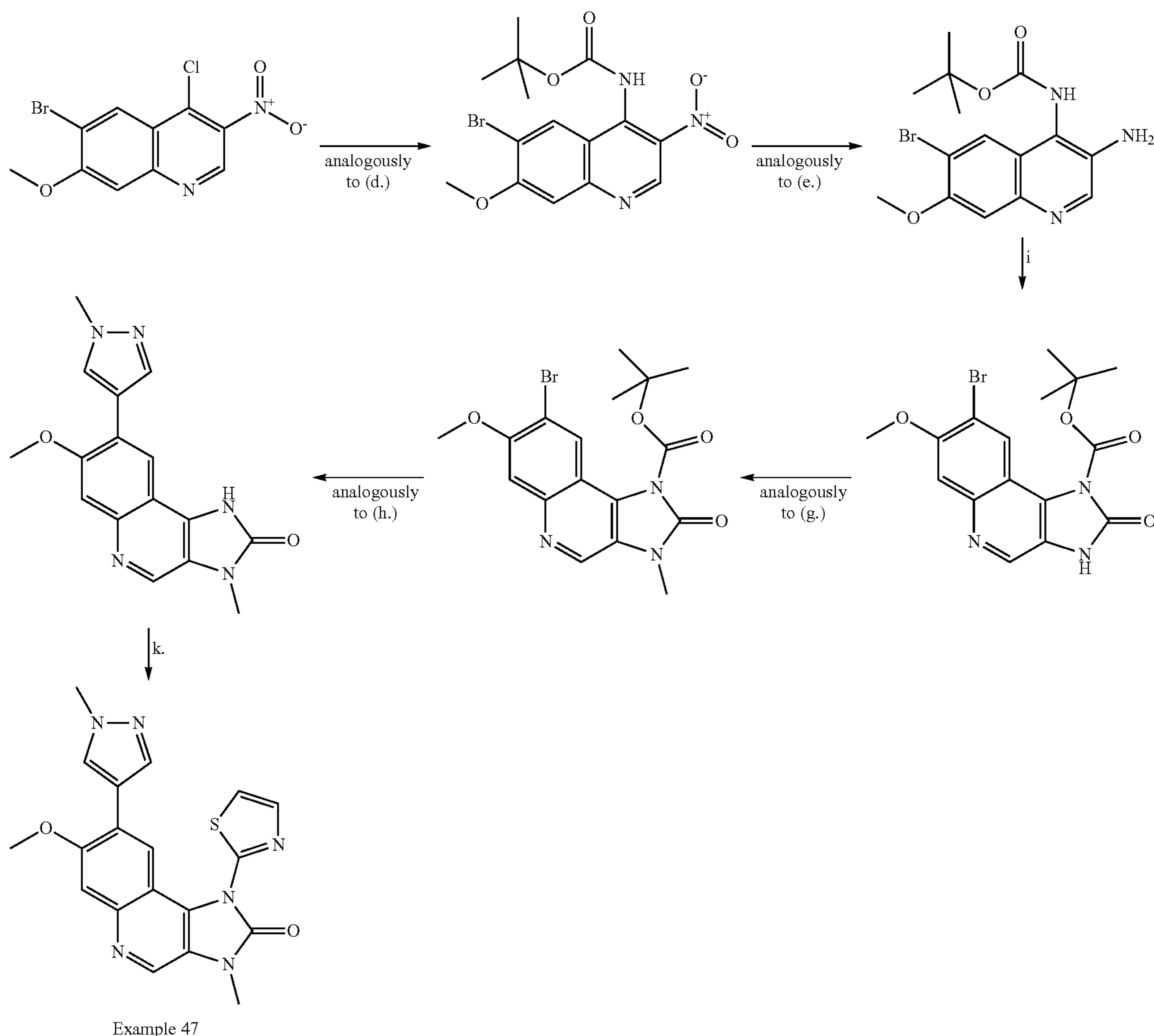
Scheme 2 Synthesis of Compound Example 47
