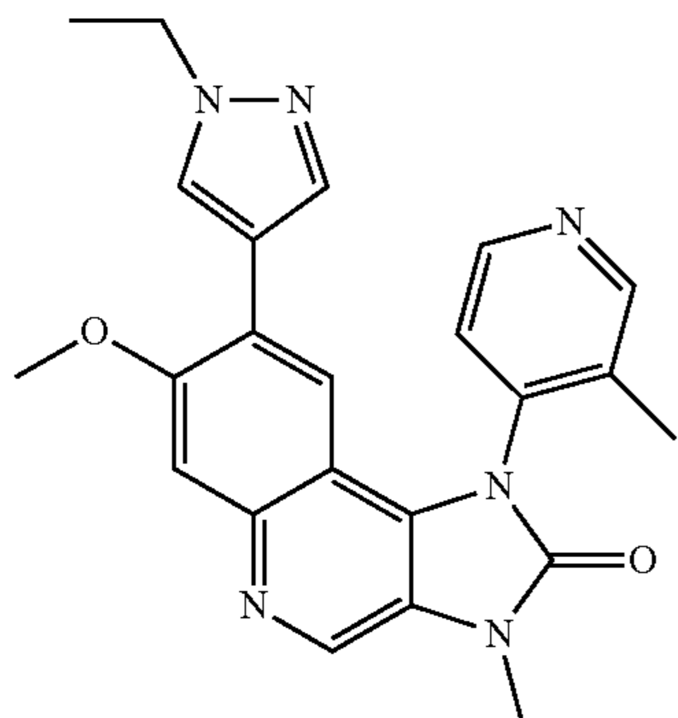
8-(1-Ethyl-1H-pyrazol-4-yl)-7-methoxy-3-methyl-1-(3-methylpyridin-4-yl)-1,3-dihydroimidazo[4,5-c]quinolin-2-one
