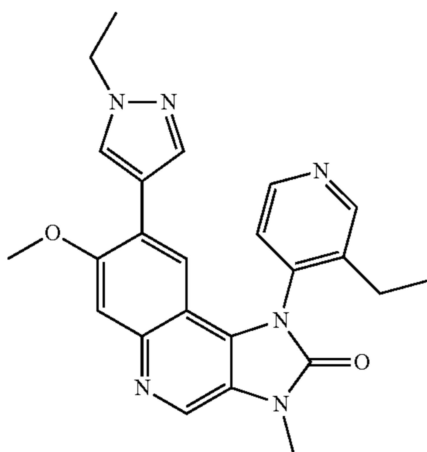
8-(1-Ethyl-1H-pyrazol-4-yl)-1-(3-ethylpyridin-4-yl)-7-methoxy-3-methyl-1,3-dihydroimidazo[4,5-c]quinolin-2-one
