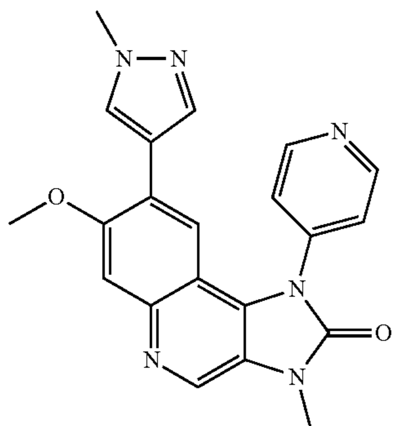
7-Methoxy-3-methyl-8-(1-methyl-1H-pyrazol-4-yl)-1-pyridin-4-yl-1,3-dihydroimidazo[4,5-c]quinolin-2-one
