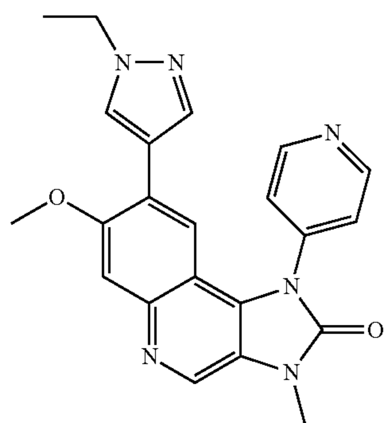
8-(1-Ethyl-1H-pyrazol-4-yl)-7-methoxy-3-methyl-1-pyridin-4-yl-1,3-dihydroimidazo[4,5-c]quinolin-2-one
