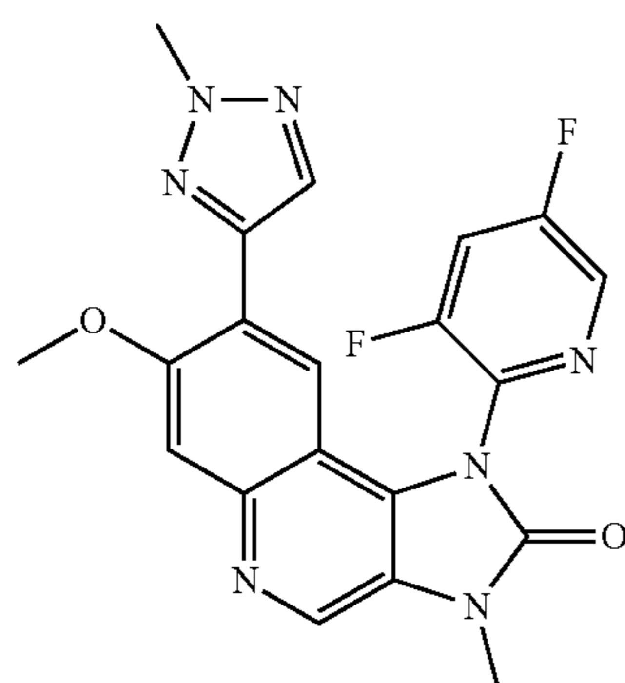
1-(3,5-Difluoropyridin-2-yl)-7-methoxy-3-methyl-8-(2-methyl-2H-1,2,3-triazol-4-yl)-1,3-dihydroimidazo[4,5-c]quinolin-2-one
