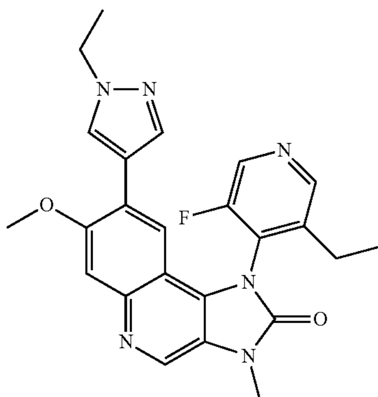
1-(3-Ethyl-5-fluoropyridin-4-yl)-8-(1-ethyl-1H-pyrazol-4-yl)-7-methoxy-3-methyl-1,3-dihydroimidazo[4,5-c]quinolin-2-one
