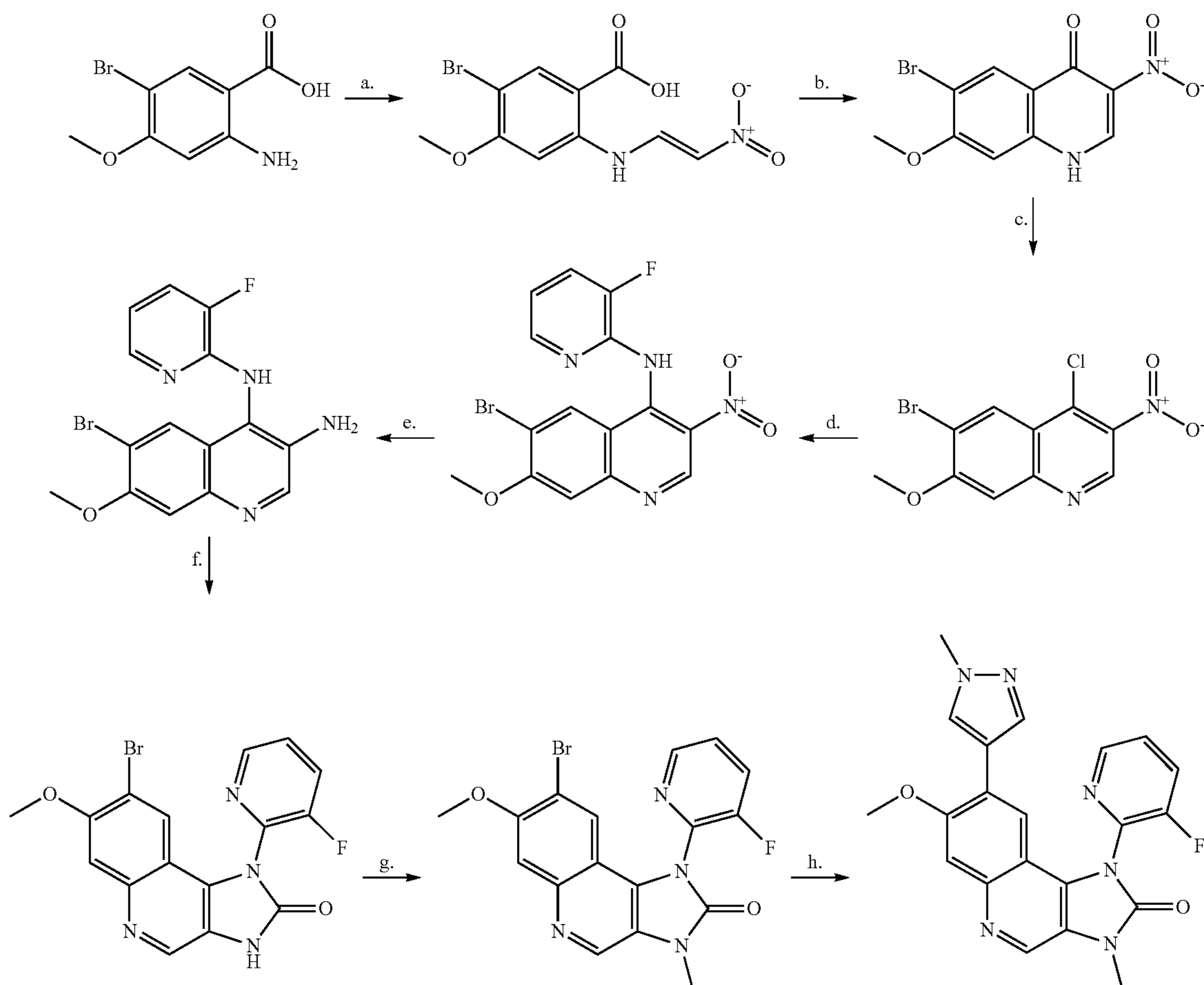
Scheme 1 Synthesis of Compound Example 14
