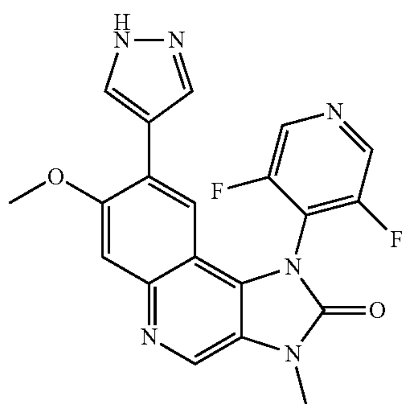
1-(3,5-Difluoropyridin-4-yl)-7-methoxy-3-methyl-8-(1H-pyrazol-4-yl)-1,3-dihydroimidazo[4,5-c]quinolin-2-one
