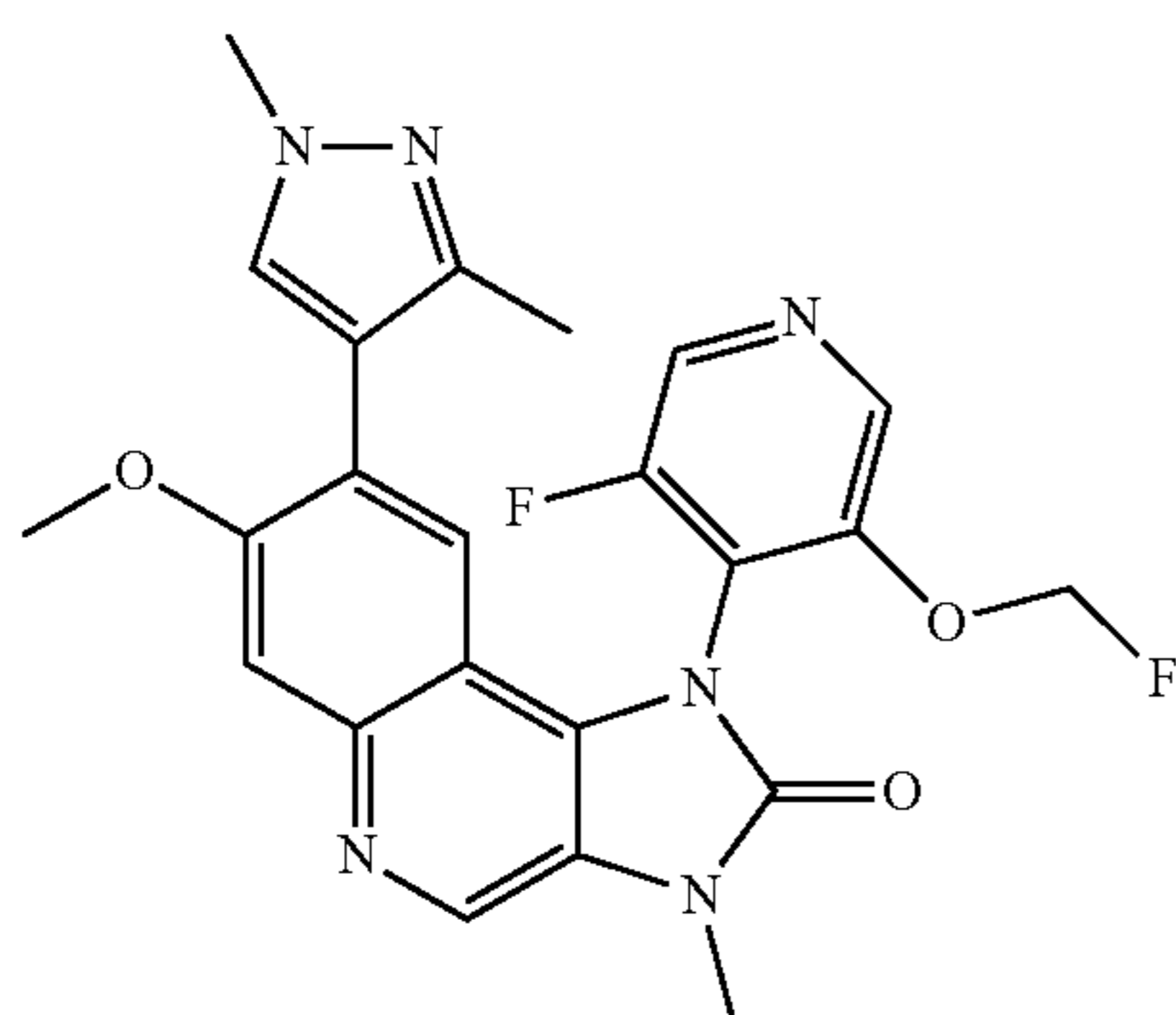
8-(1,3-Dimethyl-1H-pyrazol-4-yl)-1-(3-fluoro-5-fluoromethoxy)pyridin-4-yl)-7-methoxy-3-methyl-1,3-dihydroimidazo[4,5-c]quinolin-2-one
