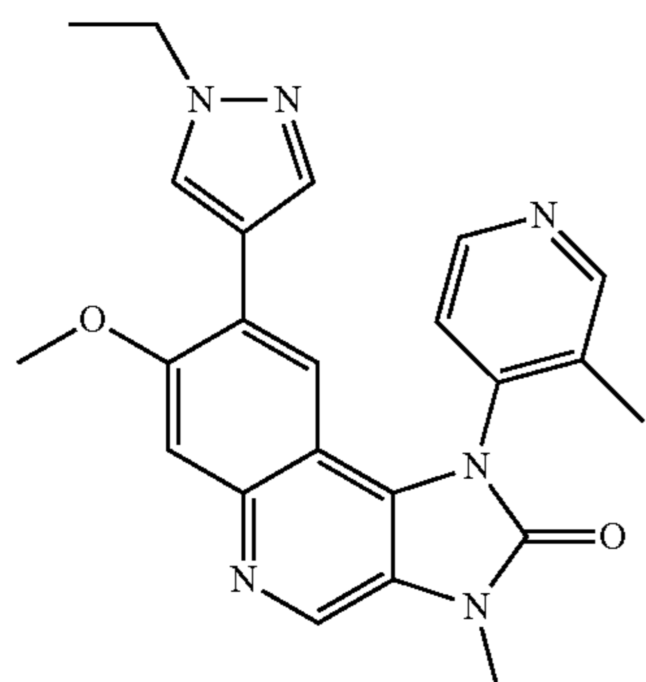
8-(1-Ethyl-1H-pyrazol-4-yl)-7-methoxy-3-methyl-1-(3-methylpyridin-4-yl)-1,3-dihydroimidazo[4,5-c]quinolin-2-one
