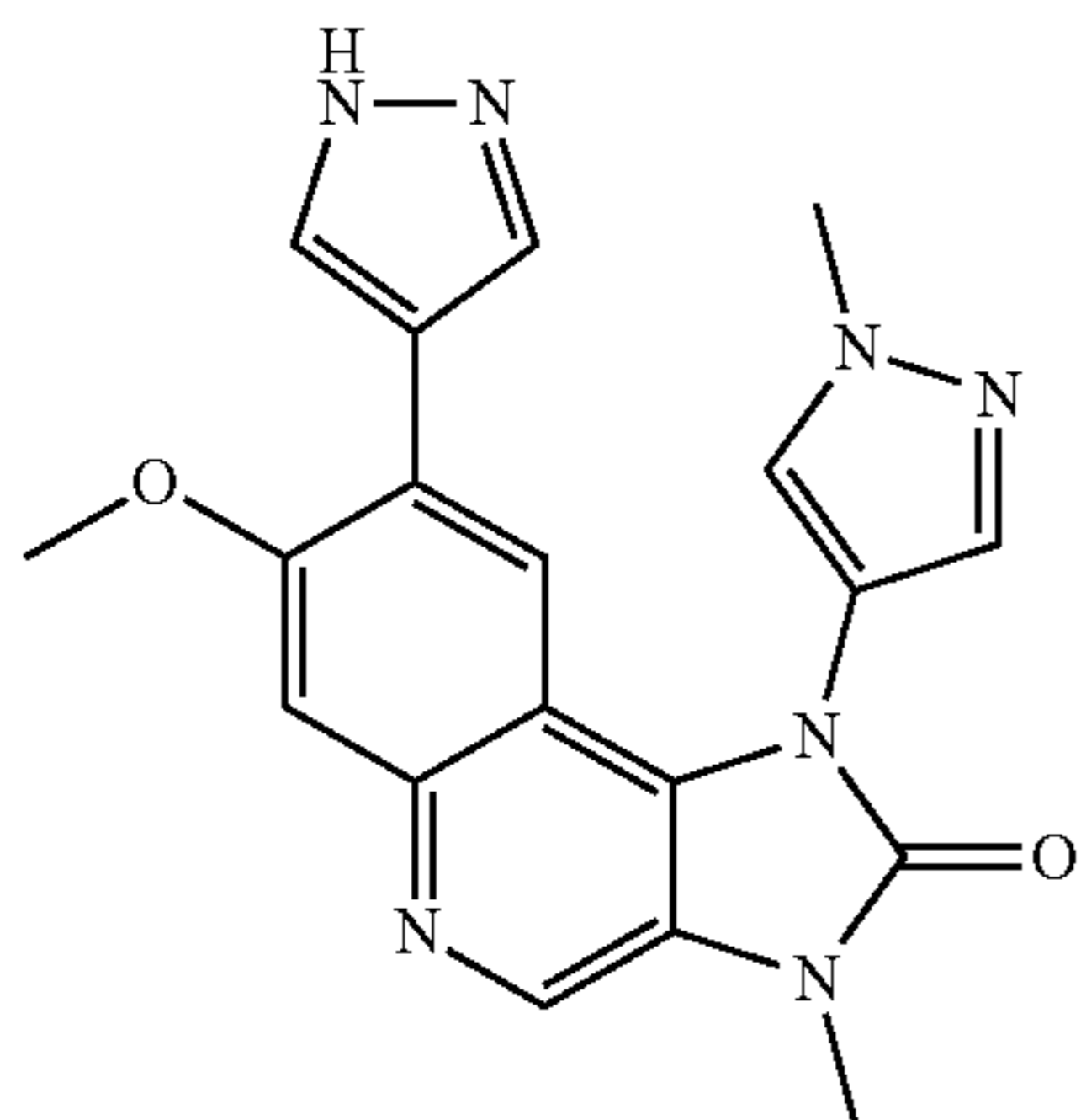
7-Methoxy-3-methyl-1-(1-methyl-1H-pyrazol-4-yl)-8-(1H-pyrazol-4-yl)-1,3-dihydroimidazo[4,5-c]quinolin-2-one
