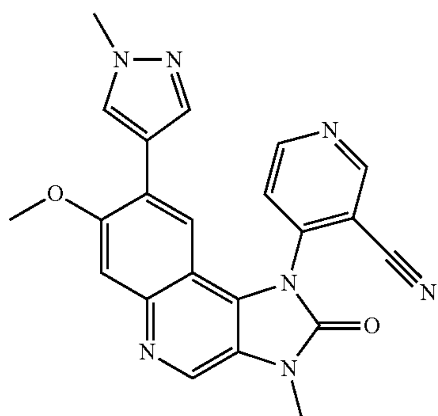
4-[7-Methoxy-3-methyl-8-(1-methyl-1H-pyrazol-4-yl)-2-oxo-2,3-dihydroimidazo[4,5-c]quinolin-1-yl]nicotinonitrile
