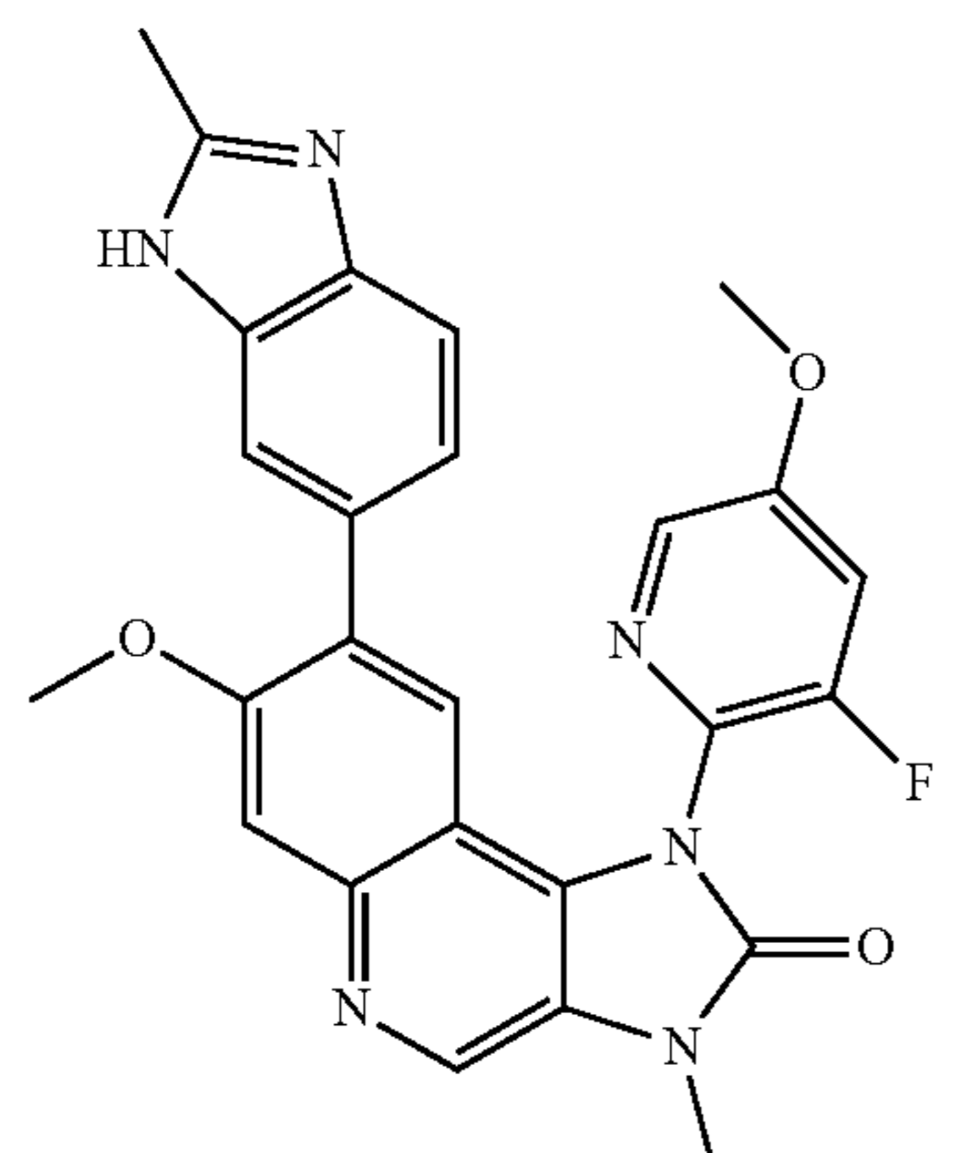
1-(3-Fluoro-5-methoxy-pyridin-2-yl)-7-methoxy-3-methyl-8-(2-methyl-3H-benzimidazol-5-yl)-1,3-dihydroimidazo[4,5-c]quinolin-2-one
