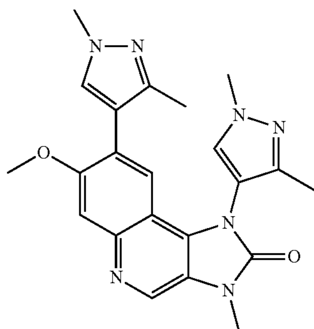
1,8-Bis(1,3-dimethyl-1H-pyrazol-4-yl)-7-methoxy-3-methyl-1,3-dihydroimidazo[4,5-c]quinolin-2-one
