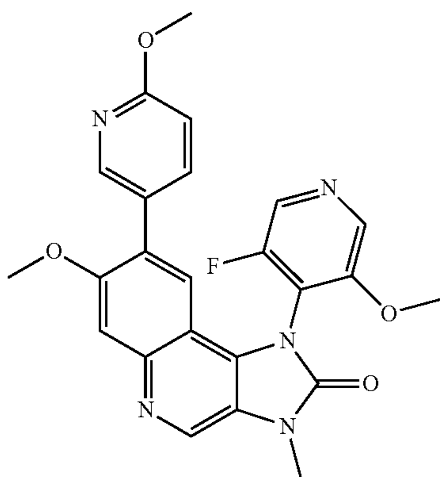
1-(3-Fluoro-5-methoxypyridin-4-yl)-7-methoxy-8-(6-methoxypyridin-3-yl)-3-methyl-1,3-dihydroimidazo[4,5-c]quinolin-2-one
