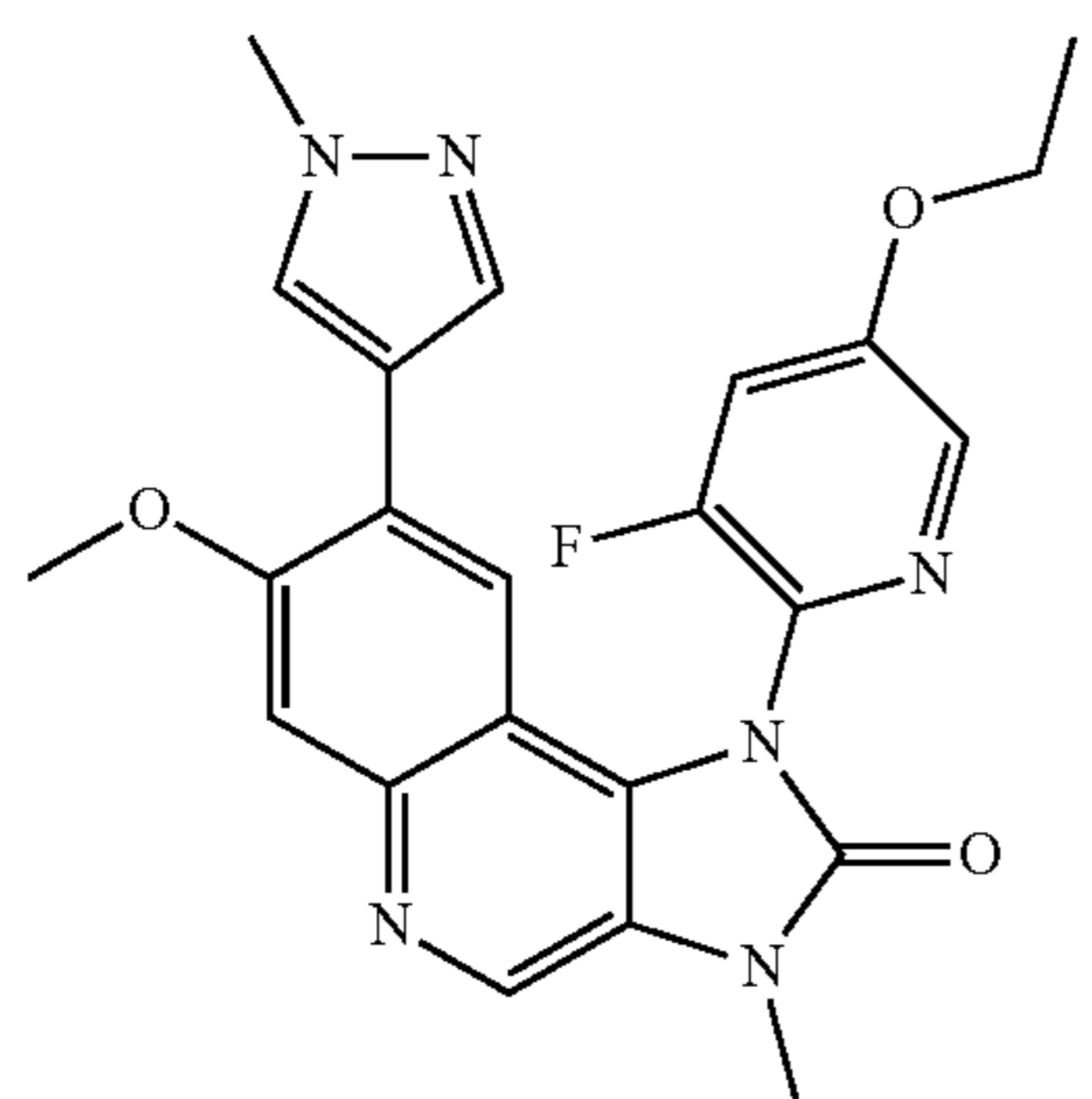
1-(5-Ethoxy-3-fluoropyridin-2-yl)-7-methoxy-3-methyl-8-(1-methyl-1H-pyrazol-4-yl)-1,3-dihydroimidazo[4,5-c]quinolin-2-one
