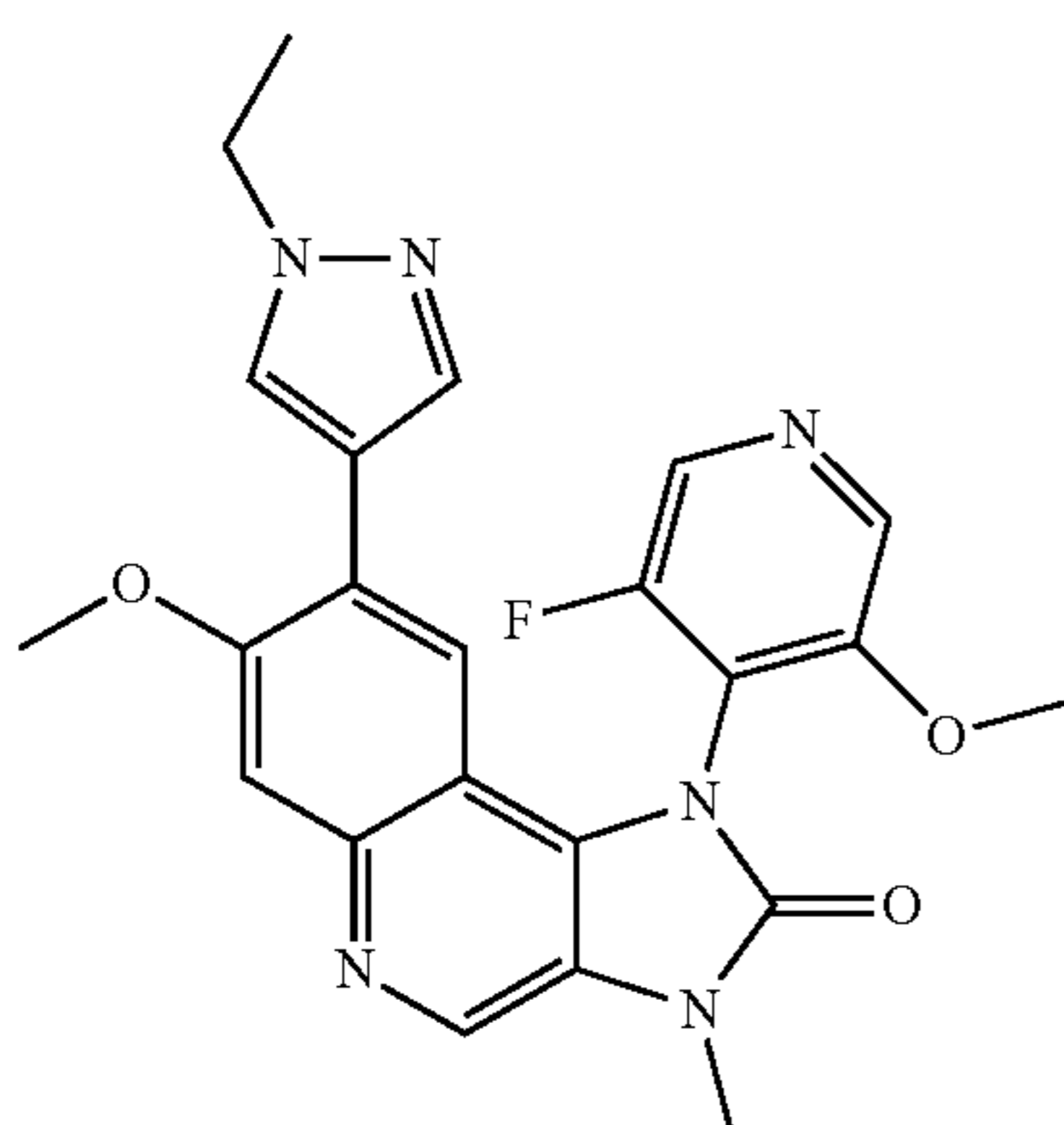
8-(1-Ethyl-1H-pyrazol-4-yl)-1-(3-fluoro-5-methoxypyridin-4-yl)-7-methoxy-3-methyl-1,3-dihydroimidazo[4,5-c]quinolin-2-one
