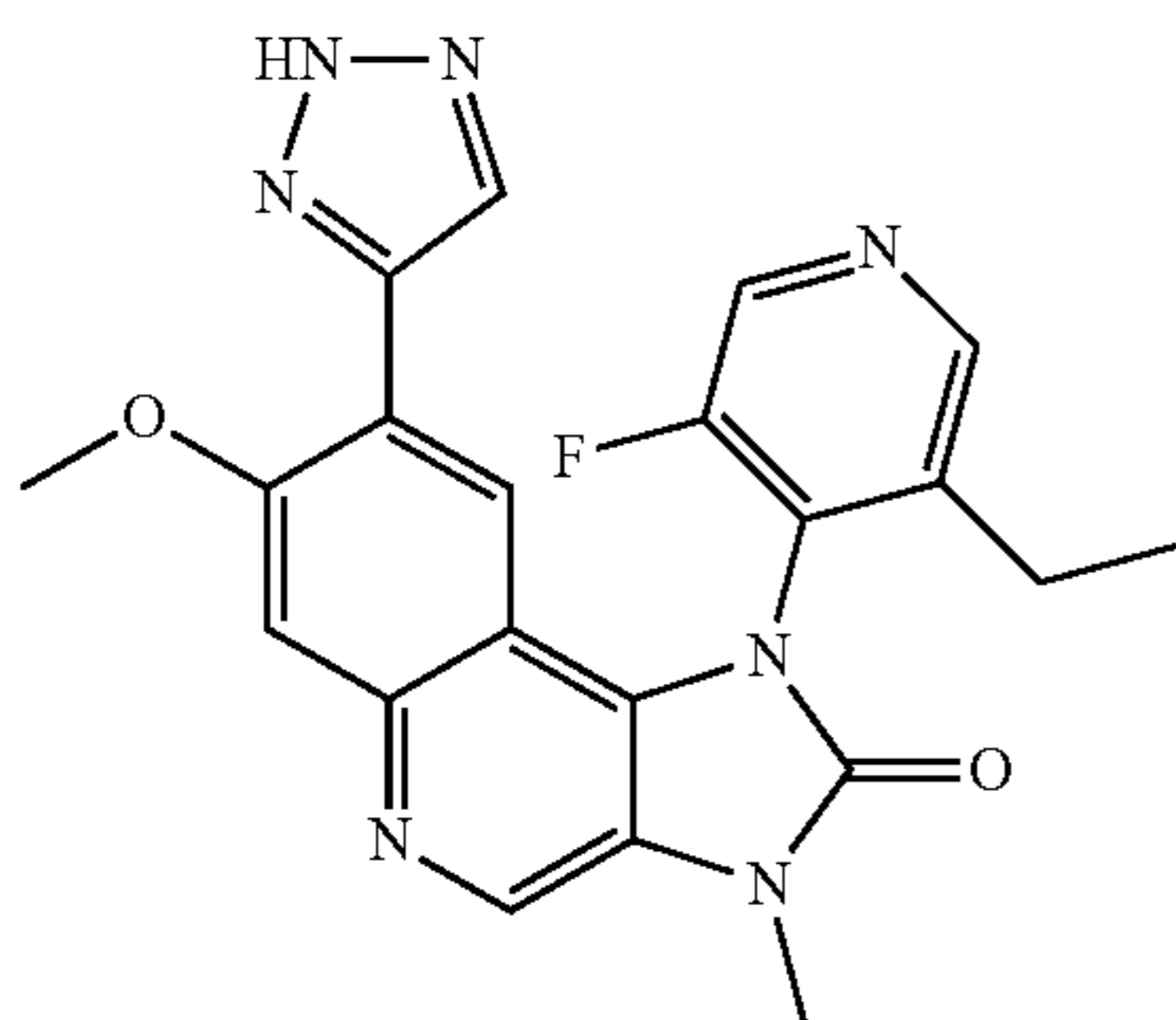
1-(3-Ethyl-5-fluoropyridin-4-yl)-7-methoxy-3-methyl-8-(2H-1,2,3-triazol-4-yl)-1,3-dihydroimidazo[4,5-c]quinolin-2-one
