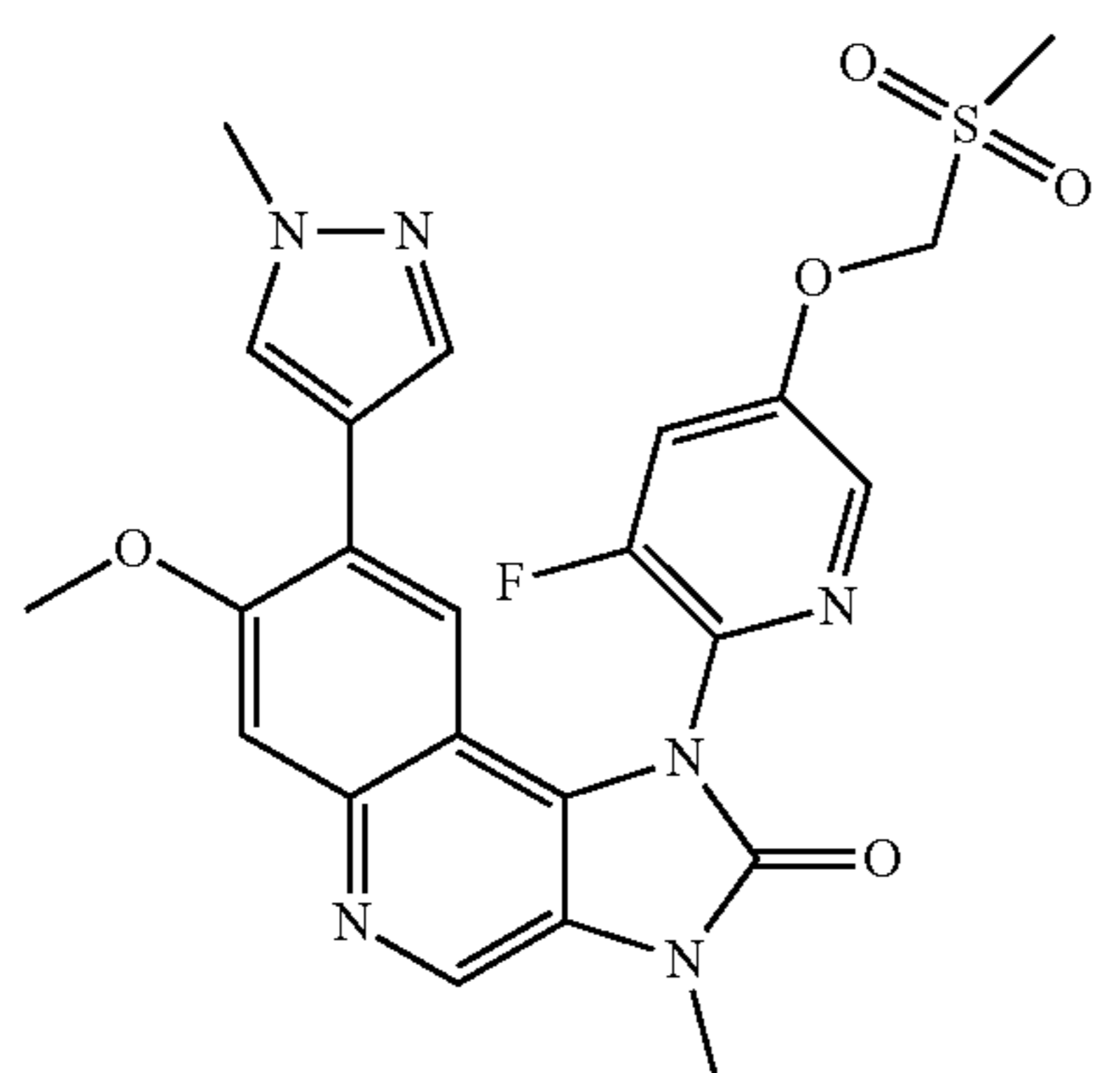
1-(3-Fluoro-5-methylsulfonylmethoxy)pyridin-2-yl)-7-methoxy-3-methyl-8-(1-methyl-1H-pyrazol-4-yl)-1,3-dihydroimidazo[4,5-c]quinolin-2-one
