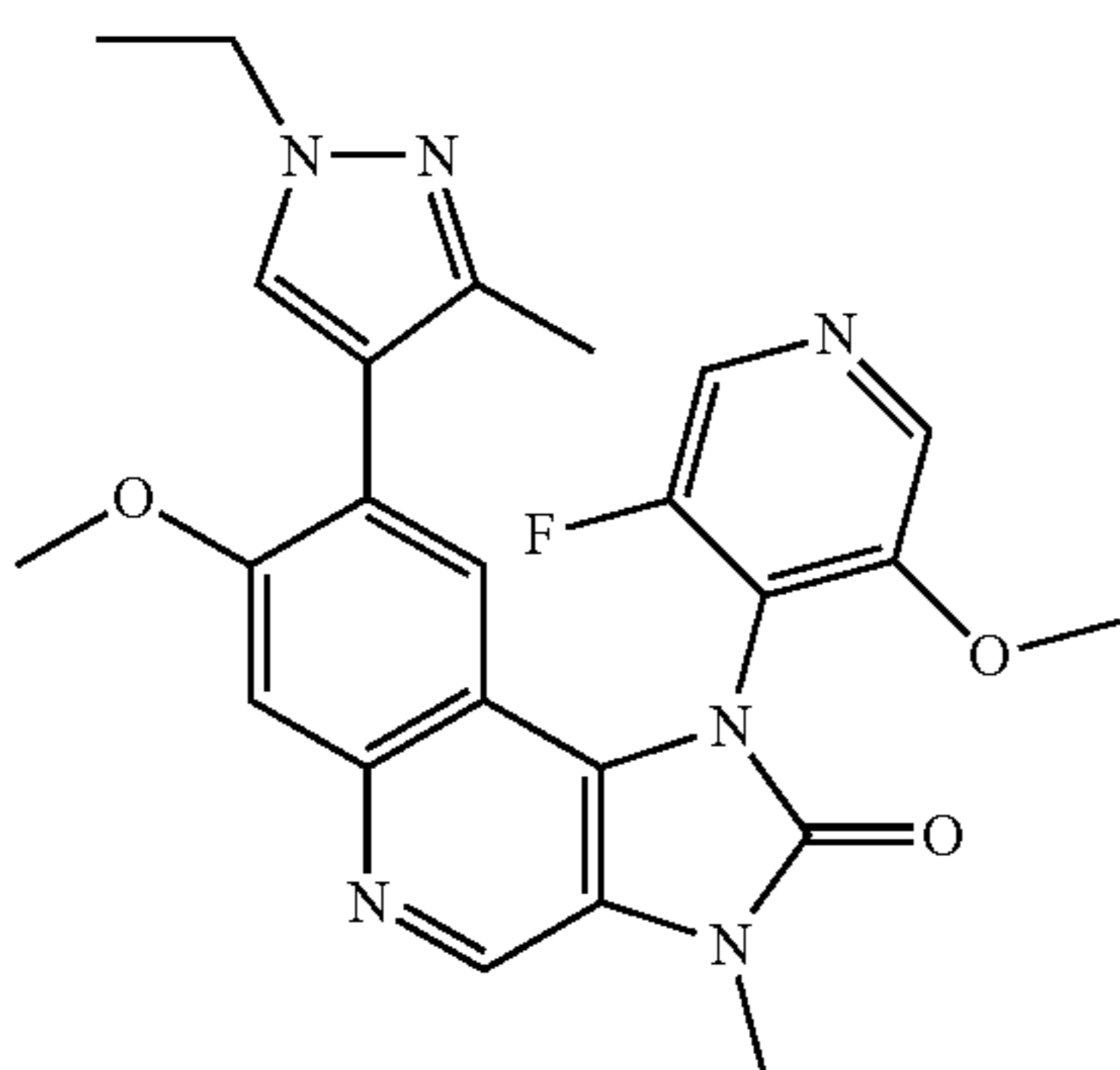
8-(1-Ethyl-3-methyl-1H-pyrazol-4-yl)-1-(3-fluoro-5-methoxy-pyridin-4-yl)-7-methoxy-3-methyl-1,3-dihydroimidazo[4,5-c]quinolin-2-one
