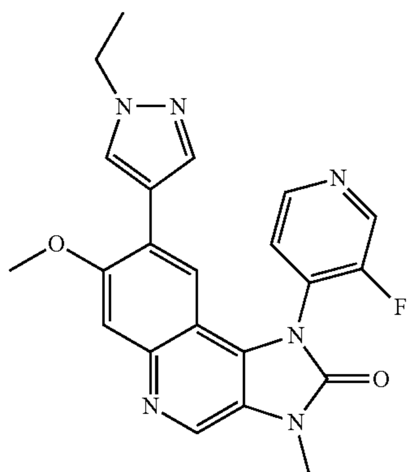
8-(1-Ethyl-1H-pyrazol-4-yl)-1-(3-fluoropyridin-4-yl)-7-methoxy-3-methyl-1,3-dihydroimidazo[4,5-c]quinolin-2-one
