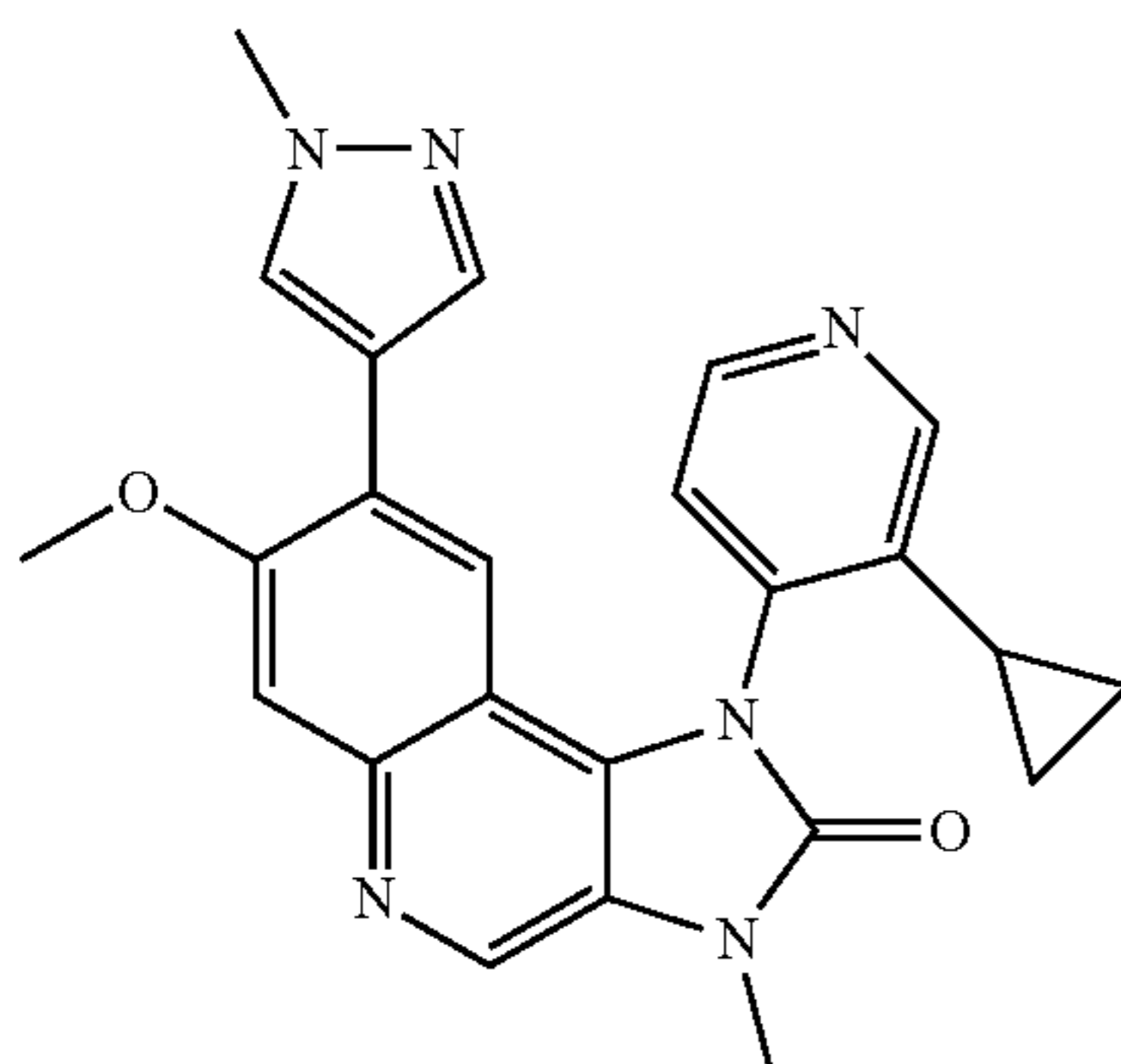
1-(3-Cyclopropylpyridin-4-yl)-7-methoxy-3-methyl-8-(1-methyl-1H-pyrazol-4-yl)-1,3-dihydroimidazo[4,5-c]quinolin-2-one
