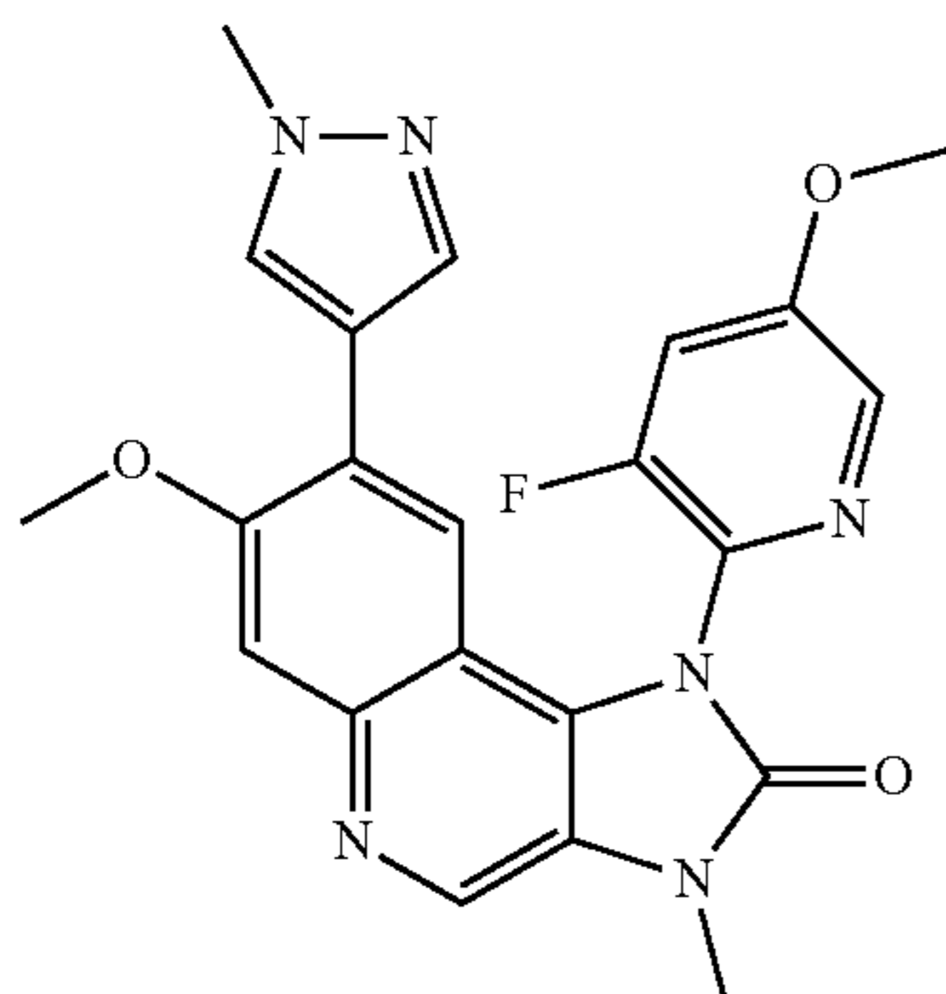
1-(3-Fluoro-5-methoxypyridin-2-yl)-7-methoxy-3-methyl-8-(1-methyl-1H-pyrazol-4-yl)-1,3-dihydroimidazo[4,5-c]quinolin-2-one
