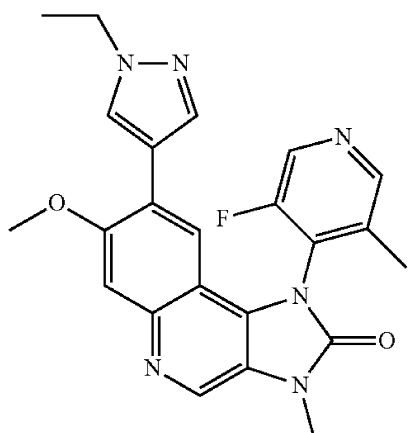
8-(1-Ethyl-1H-pyrazol-4-yl)-1-(3-fluoro-5-methylpyridin-4-yl)-7-methoxy-3-methyl-1,3-dihydroimidazo[4,5-c]quinolin-2-one
