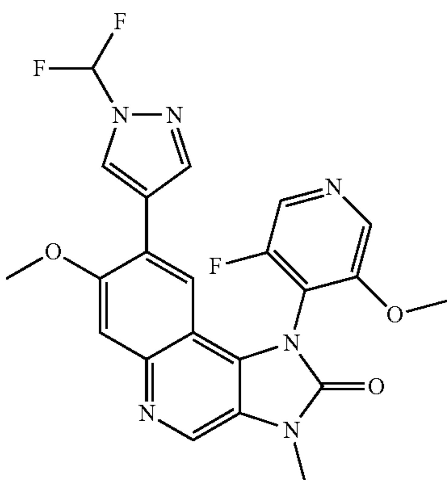
8-(1-Difluoromethyl-1H-pyrazol-4-yl)-1-(3-fluoro-5-methoxy-pyridin-4-yl)-7-methoxy-3-methyl-1,3-dihydroimidazo[4,5-c]quinolin-2-one
