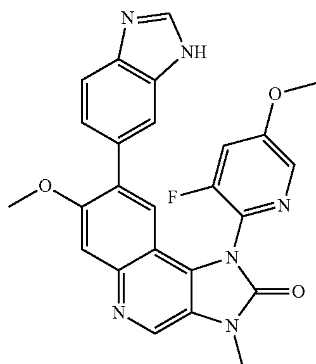
8-(3H-Benzimidazol-5-yl)-1-(3-fluoro-5-methoxypyridin-2-yl)-7-methoxy-3-methyl-1,3-dihydroimidazo[4,5-c]quinolin-2-one
