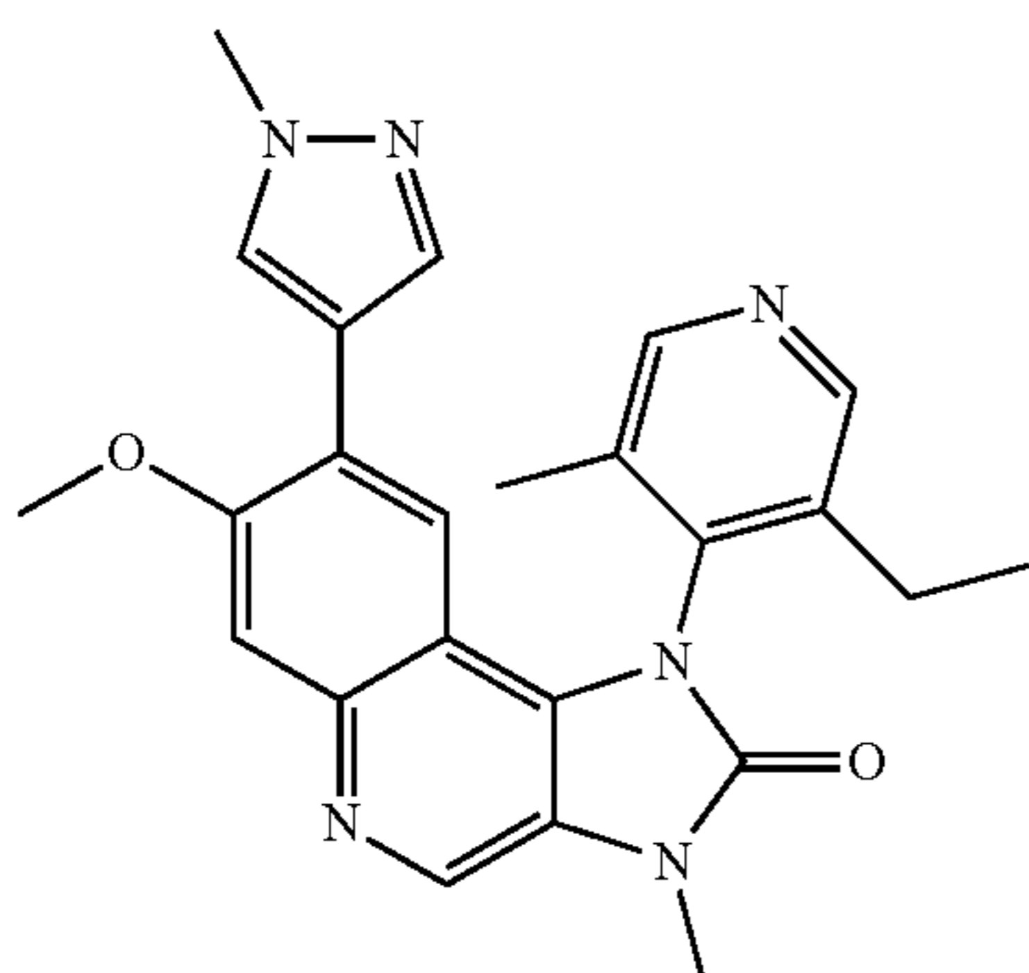
1-(3-Ethyl-5-methylpyridin-4-yl)-7-methoxy-3-methyl-8-(1-methyl-1H-pyrazol-4-yl)-1,3-dihydroimidazo[4,5-c]quinolin-2-one
