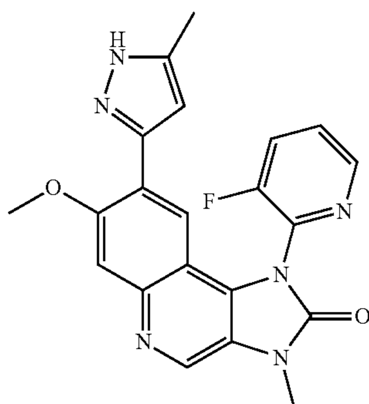
1-(3-Fluoropyridin-2-yl)-7-methoxy-3-methyl-8-(5-methyl-1H-pyrazol-3-yl)-1,3-dihydroimidazo[4,5-c]quinolin-2-one
