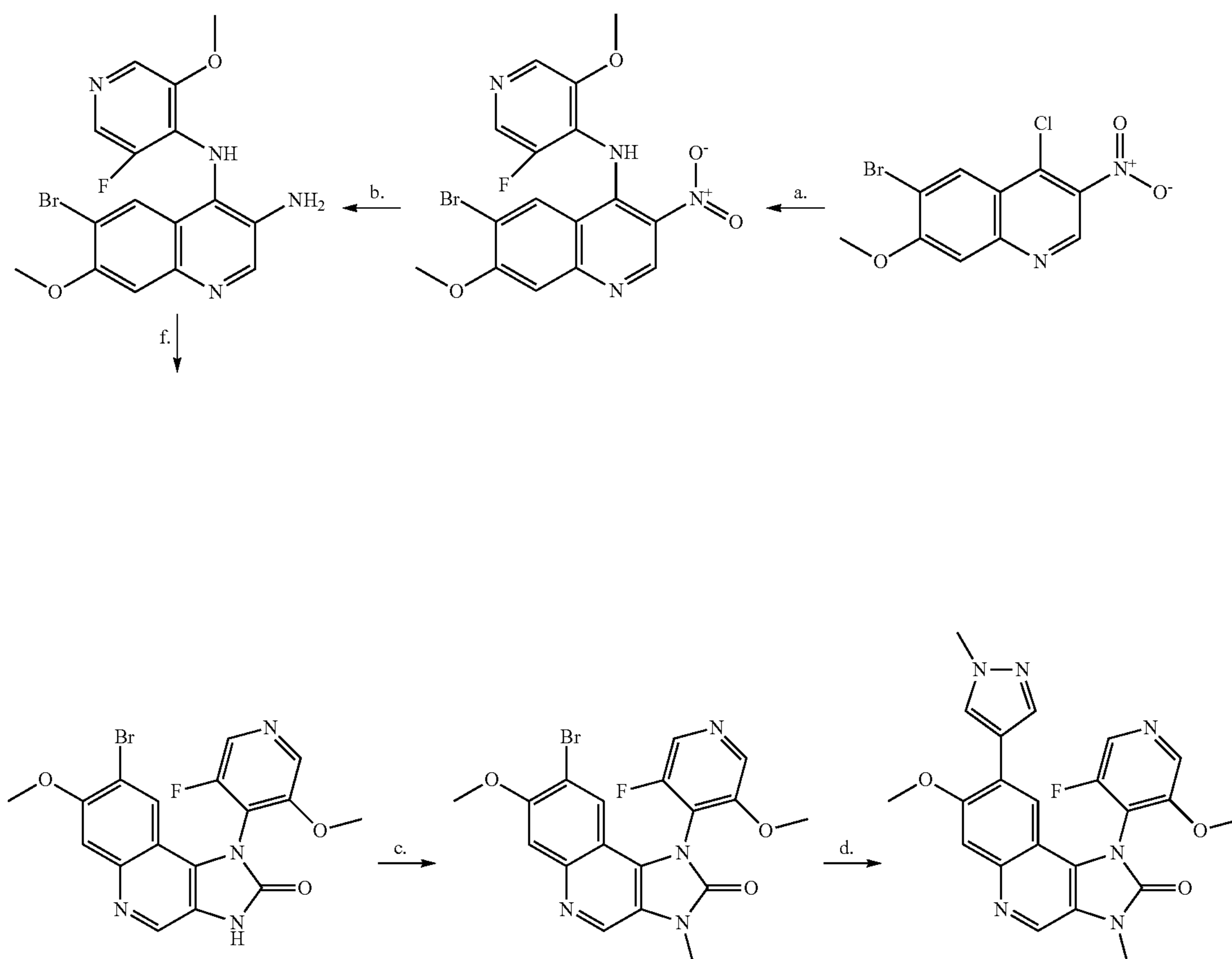
Scheme 3 Synthesis of Compound Example 4
