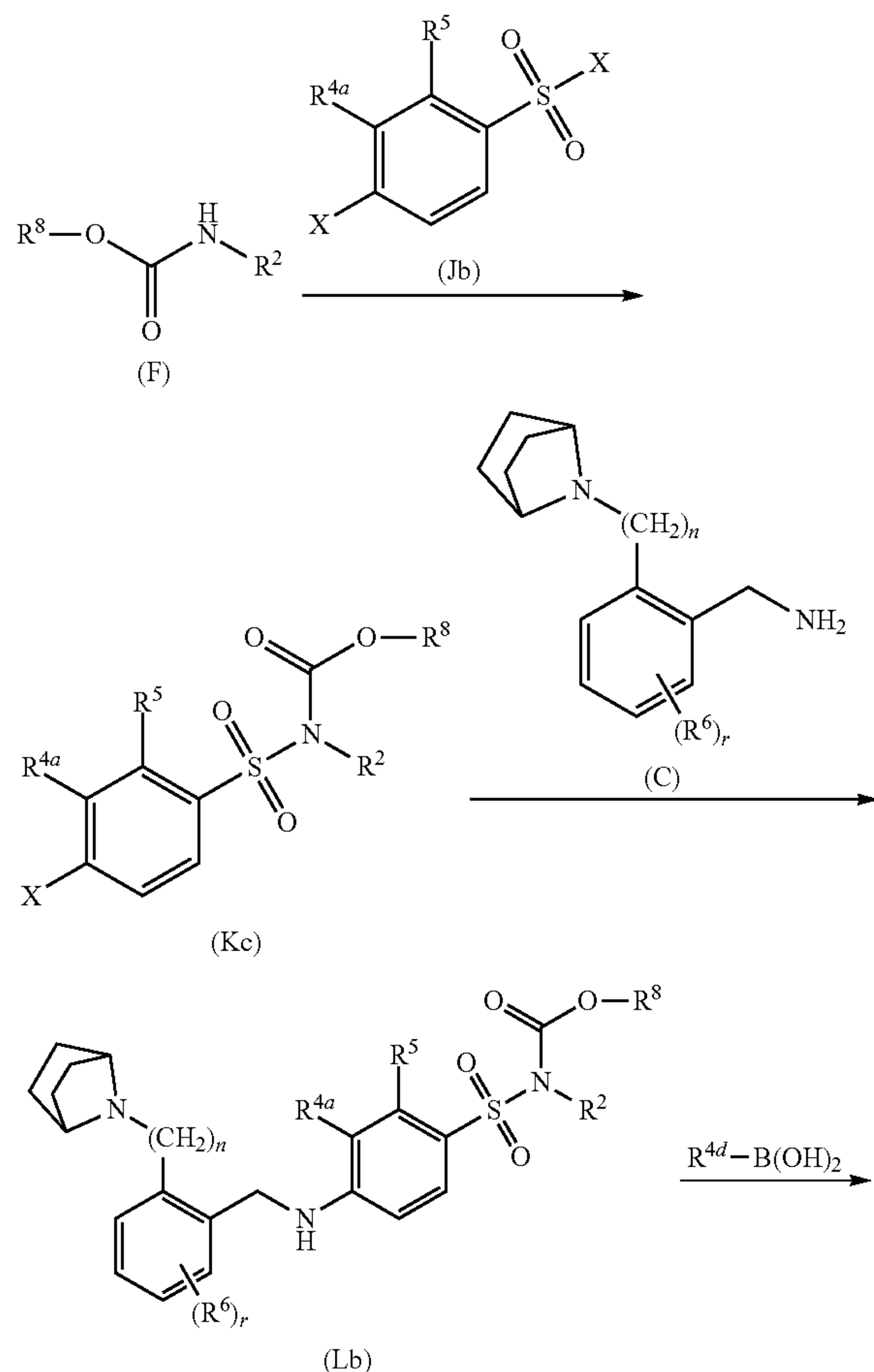
REACTION SCHEME 5
