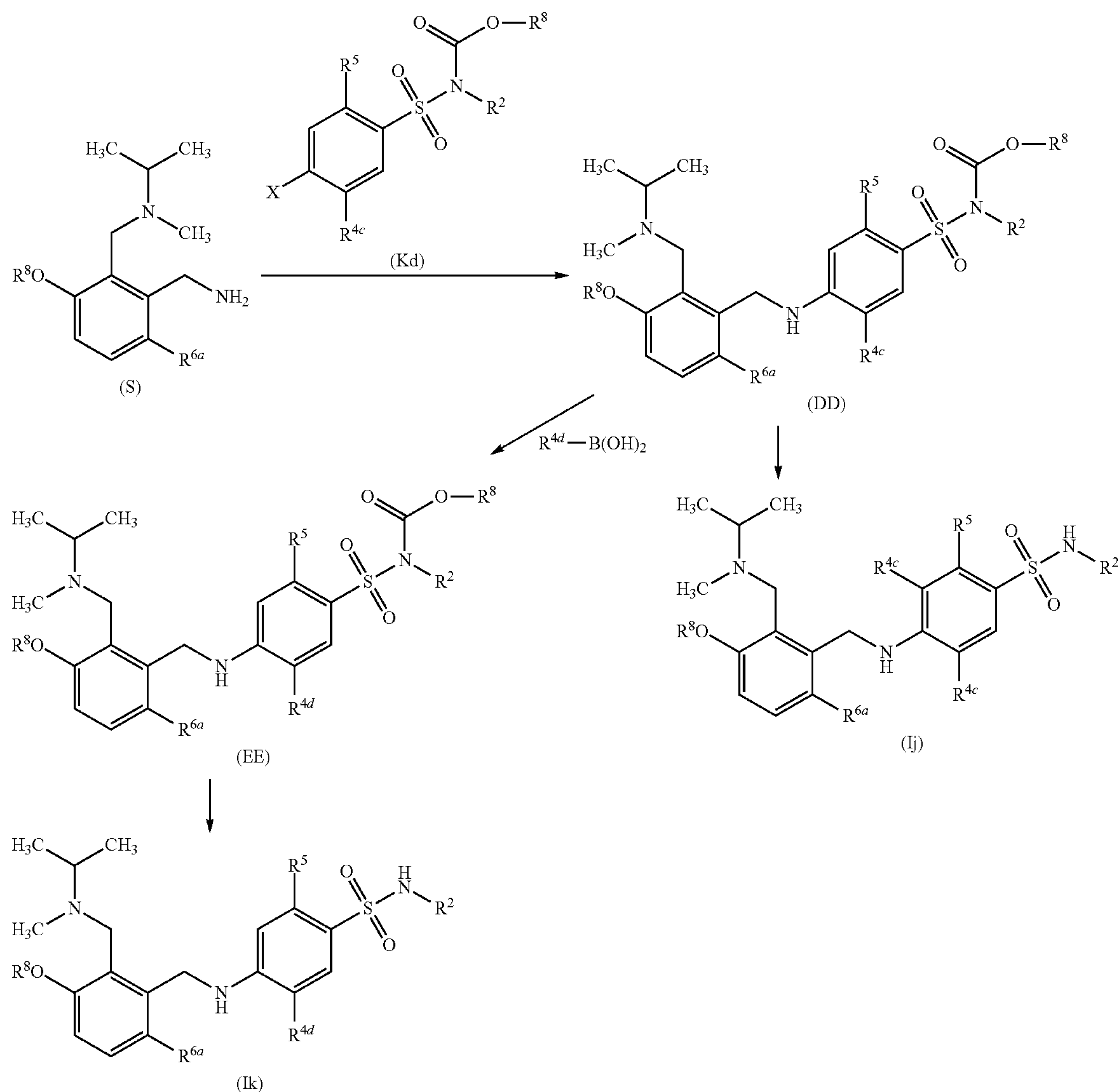
REACTION SCHEME 9
