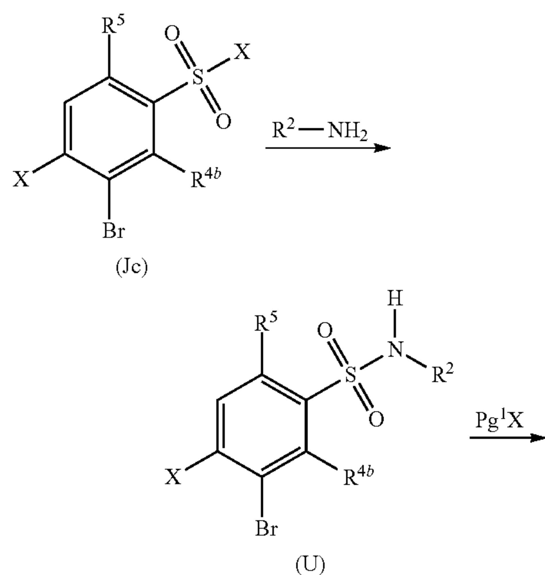
REACTION SCHEME 4
