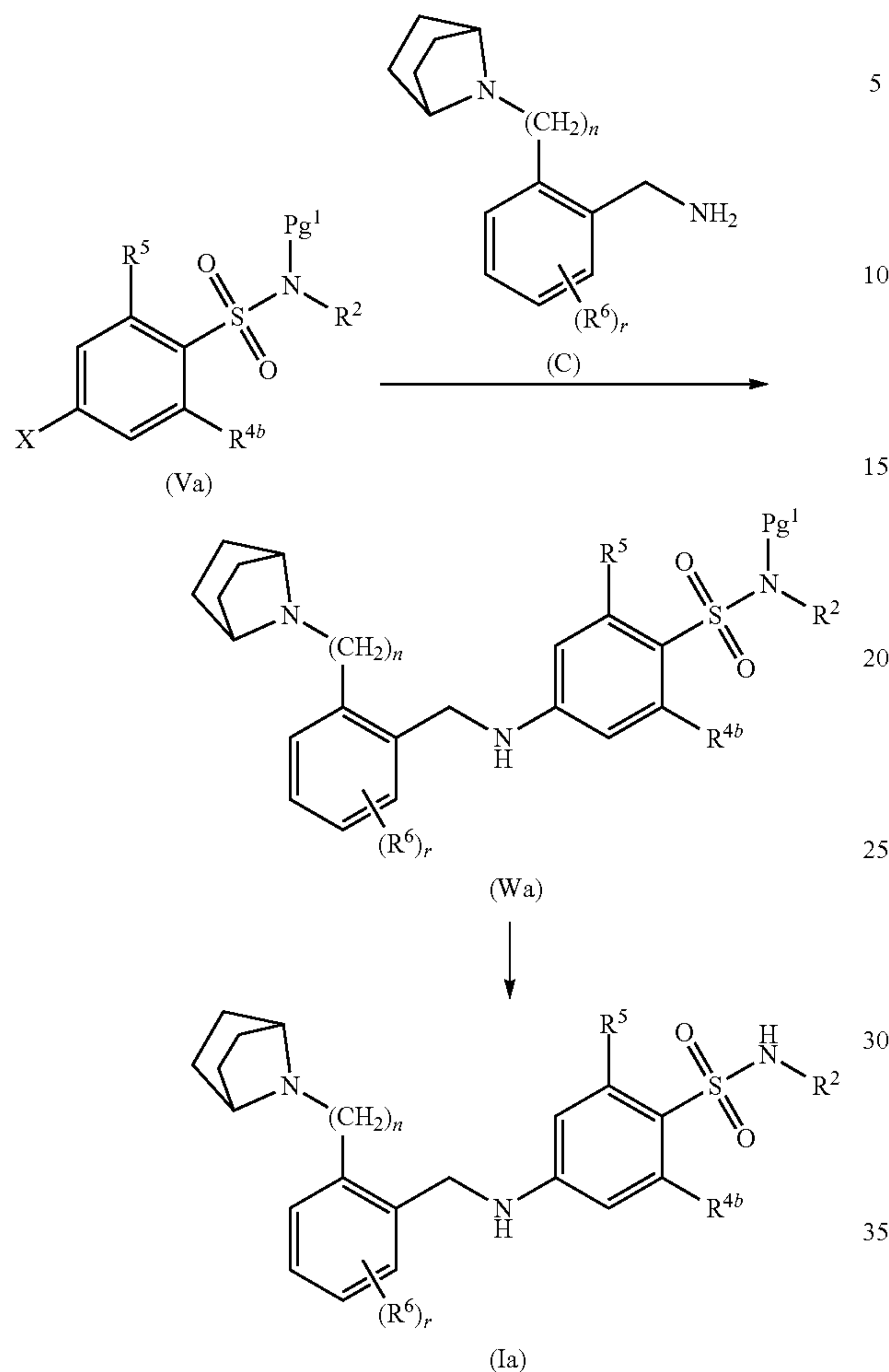
REACTION SCHEME 6
