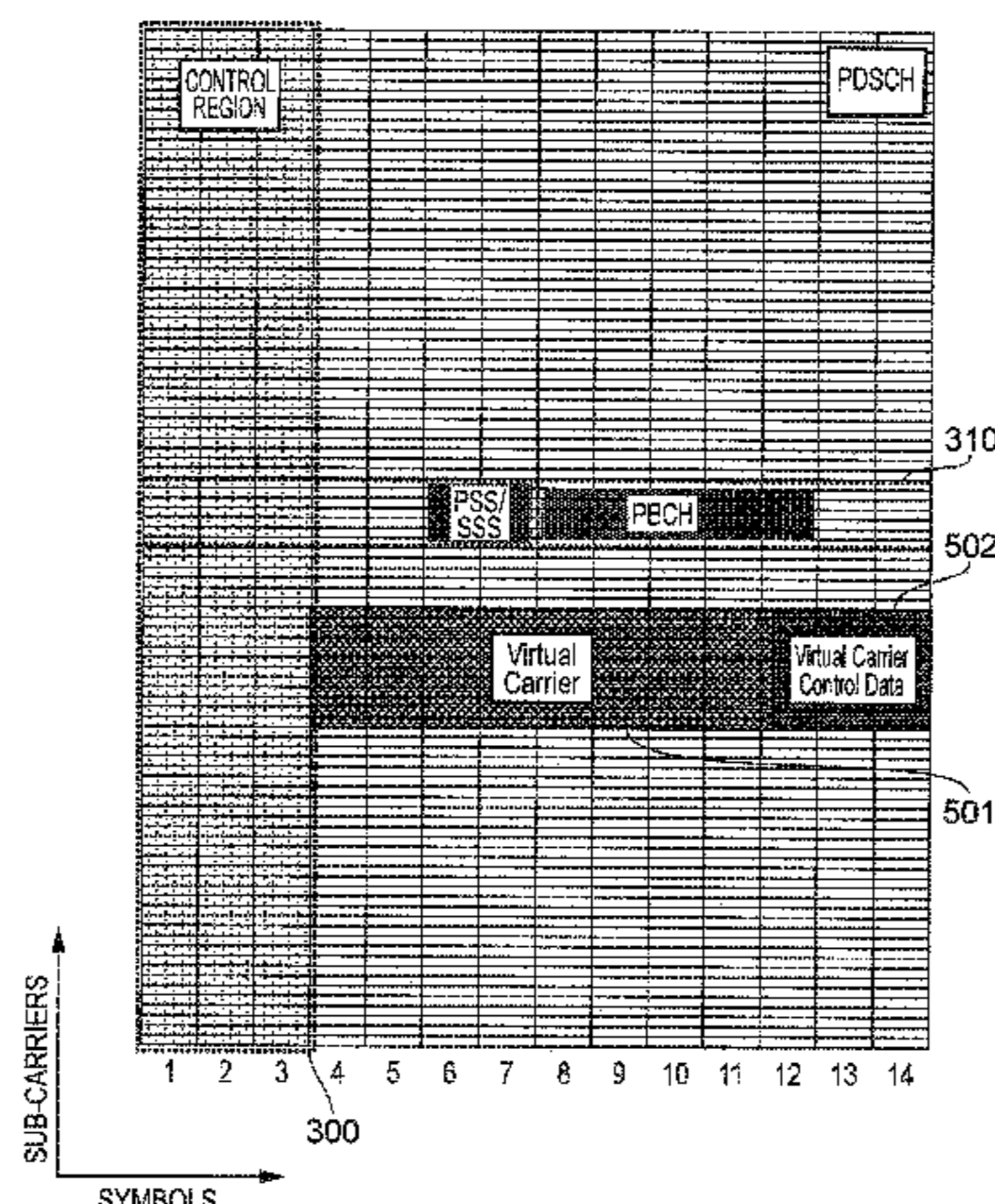
DOWNLINK SUB-FRAME WITH VIRTUAL CARRIER
