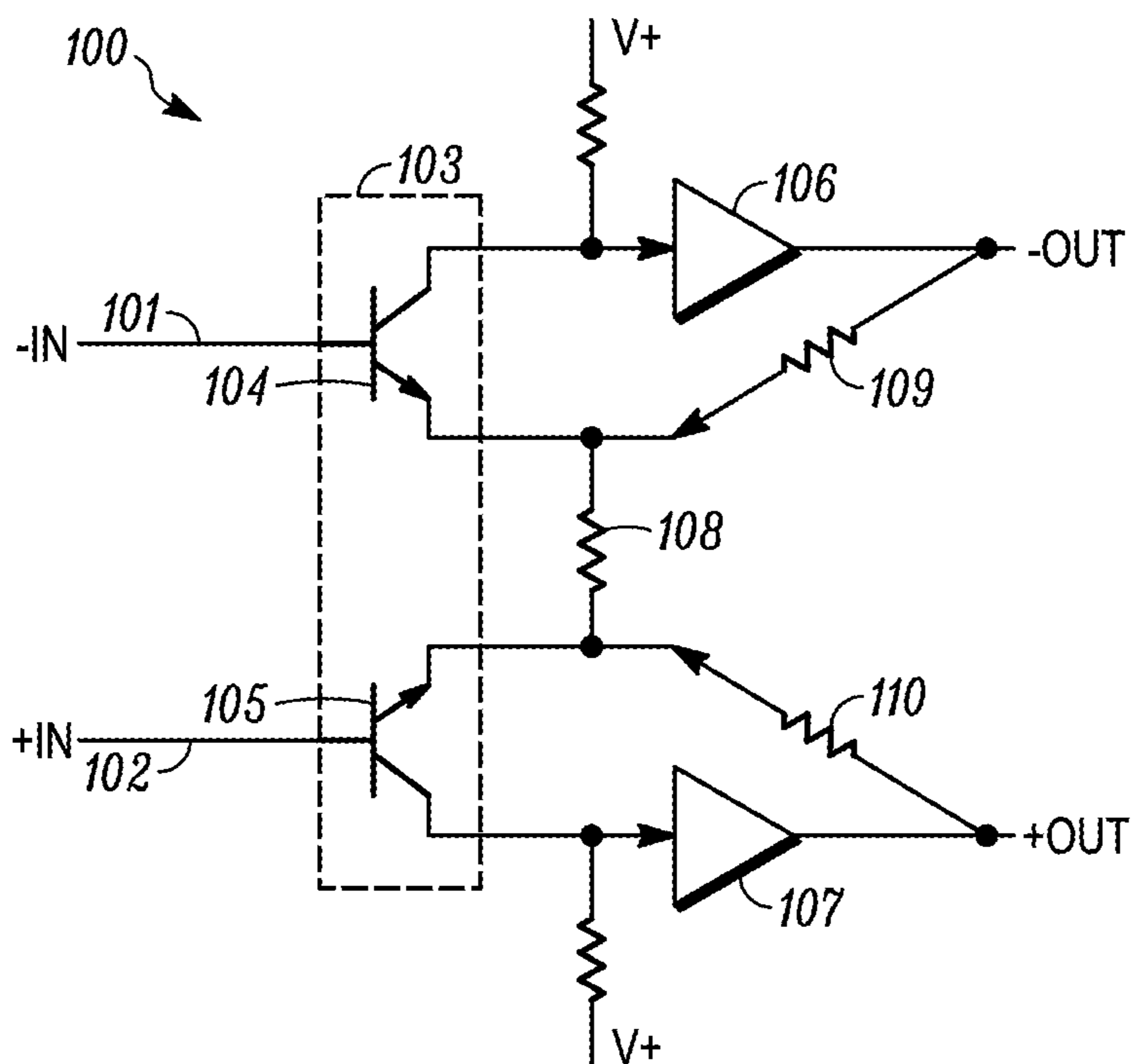
FIG. 1 (Prior Art)
