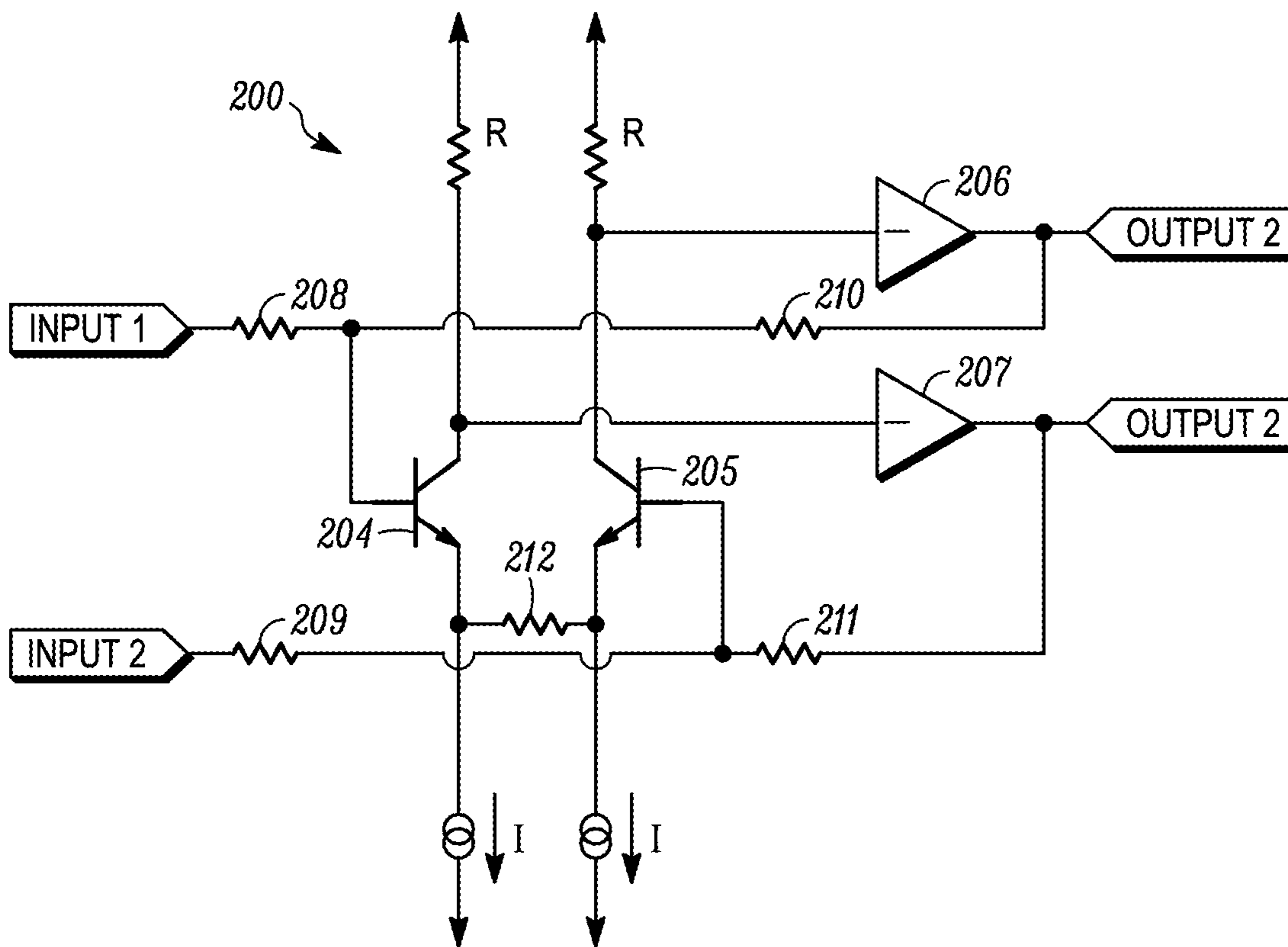
FIG. 2 (Prior Art)
