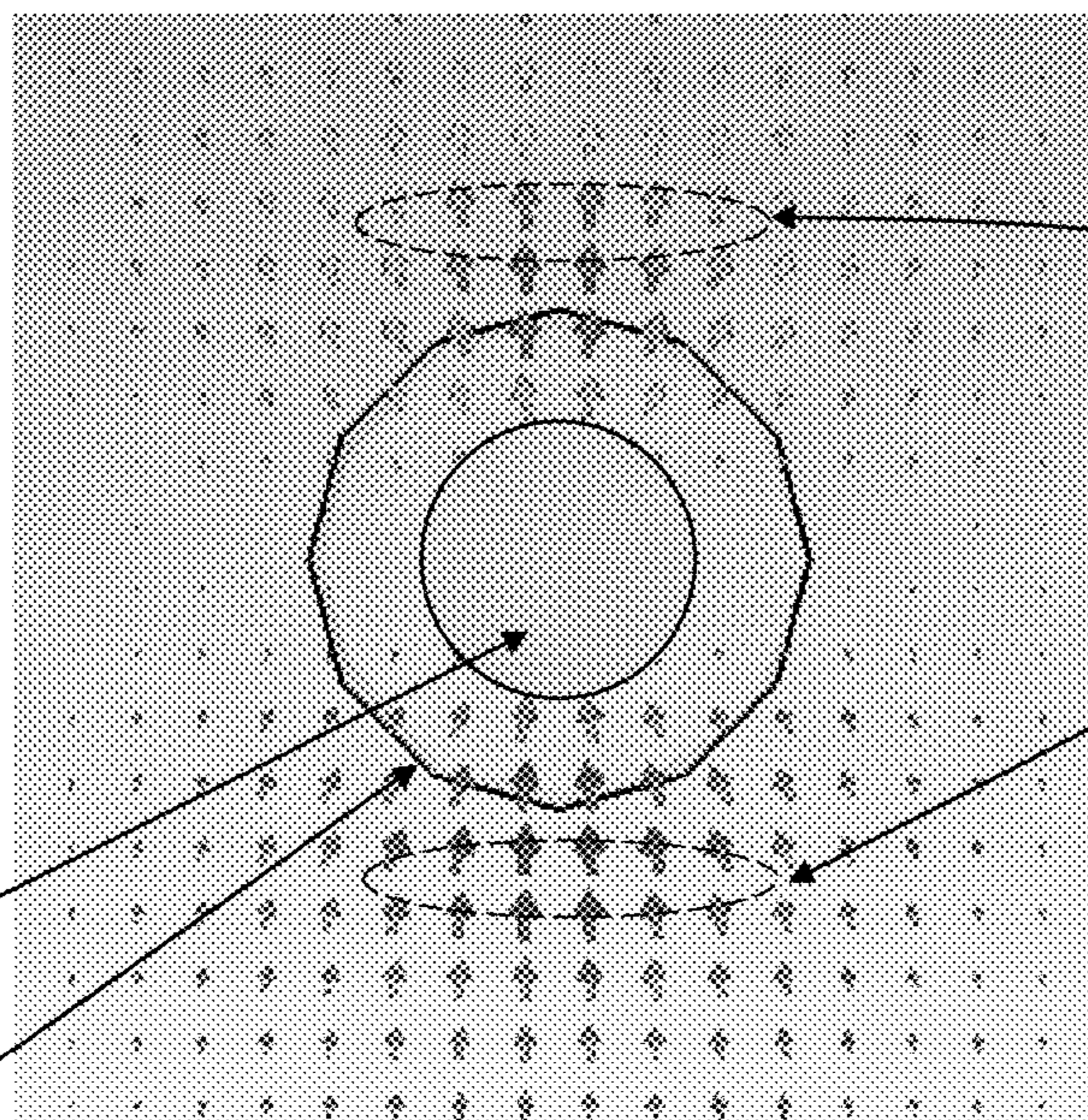
2141 FIG. 21L HE Wave Mode (Large Mode Size)
