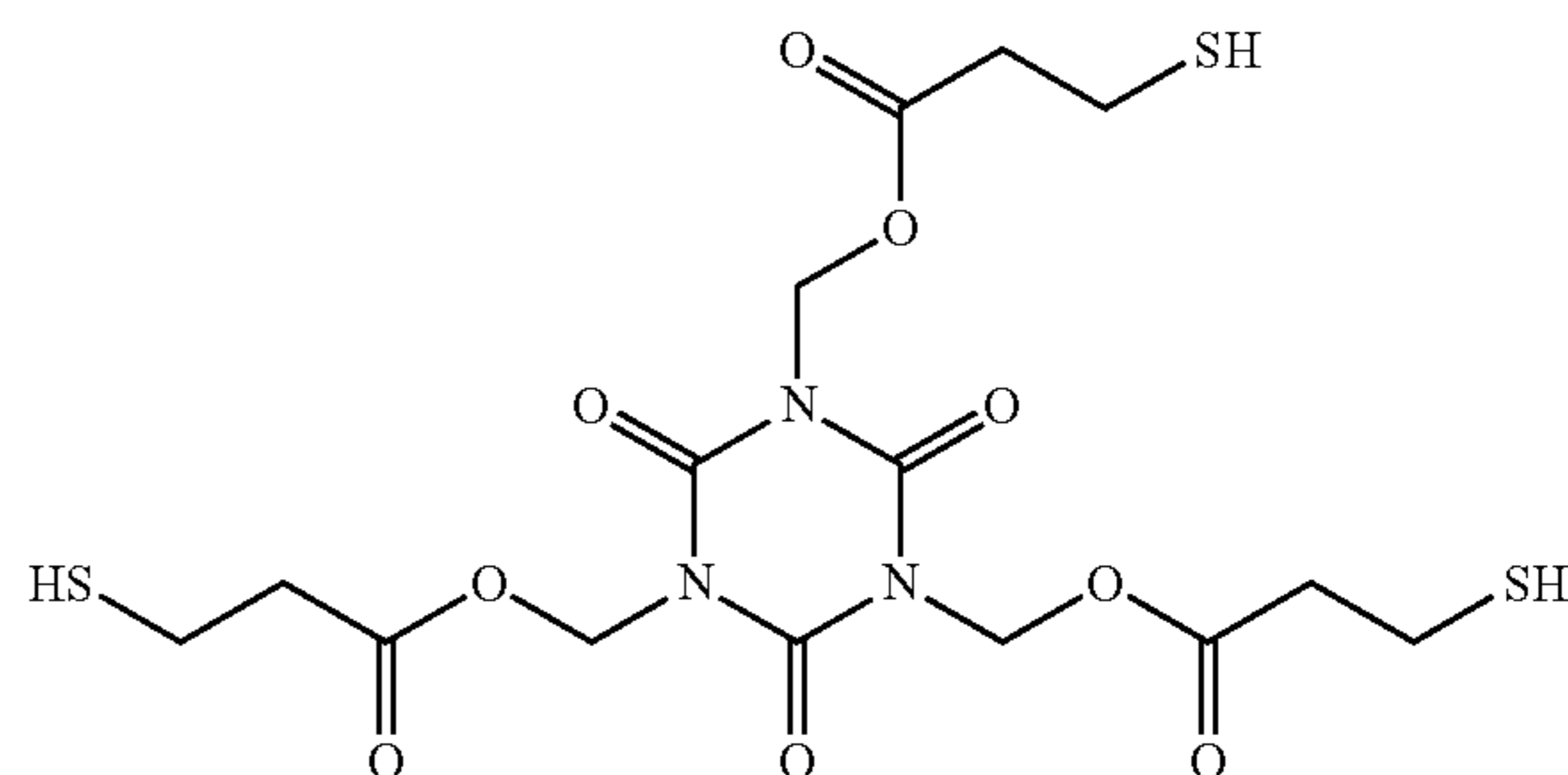
Chemical Formula 1-5
