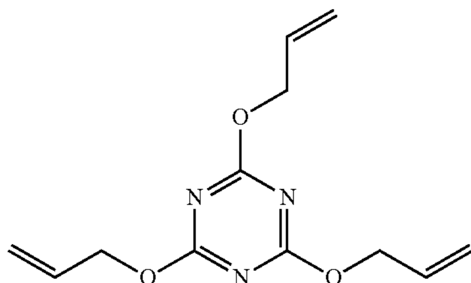
Chemical Formula 2-3
