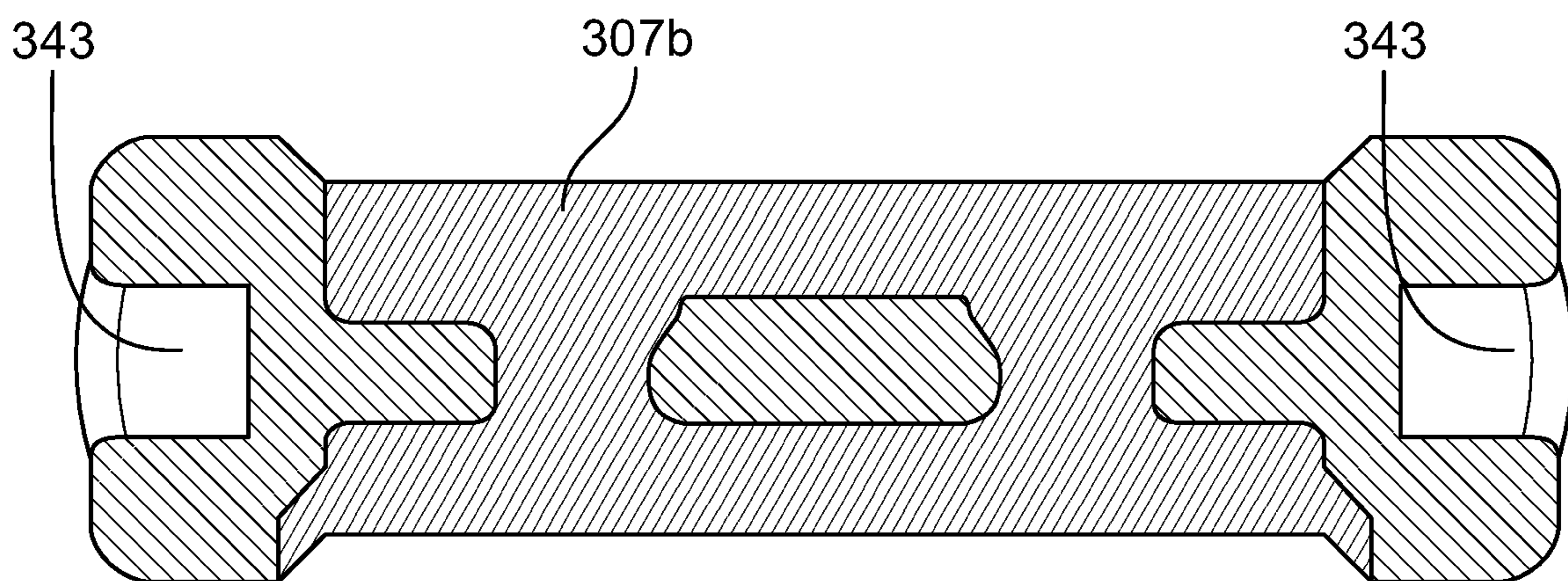
SECTION F-F
