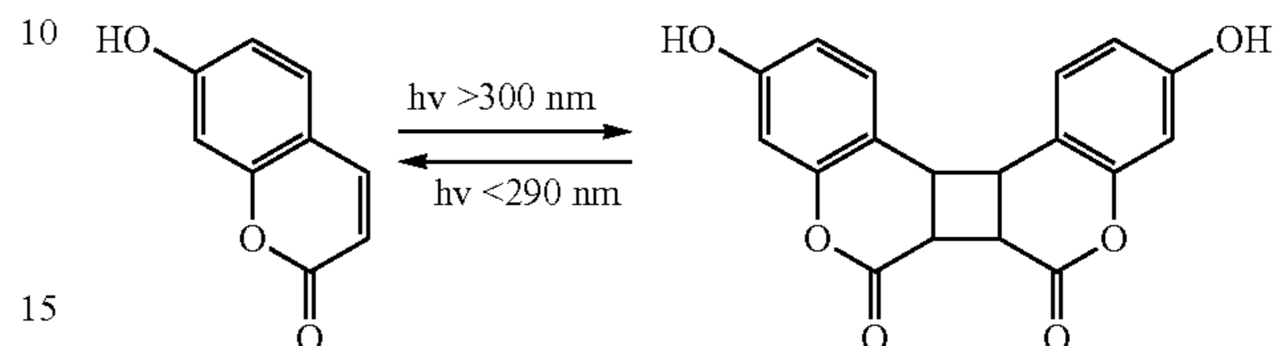
Scheme 2-Reversibility of coumarin substituent.
