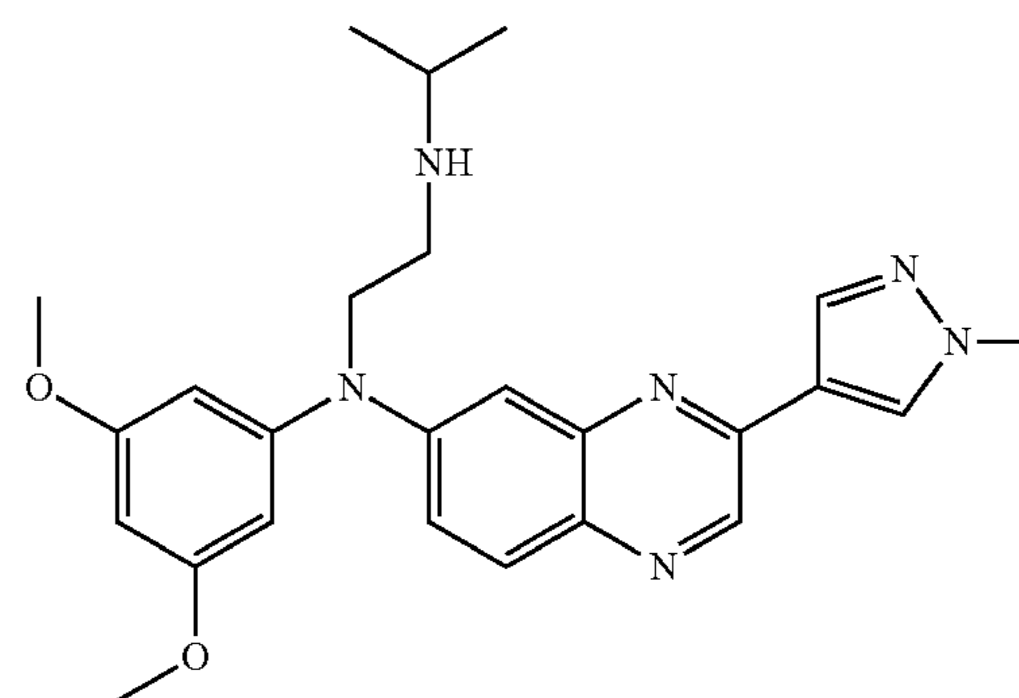
compound A
