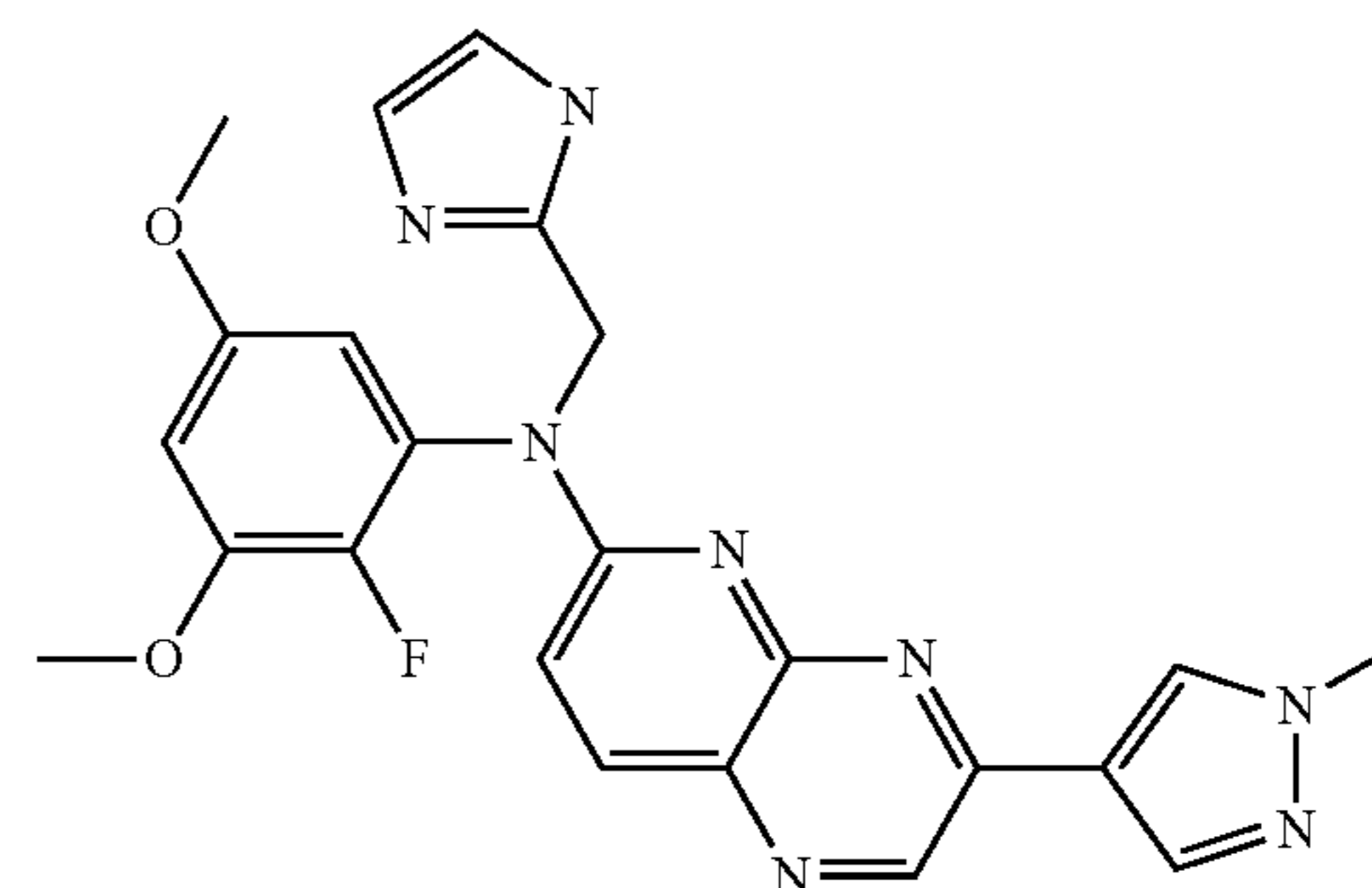
compound B
