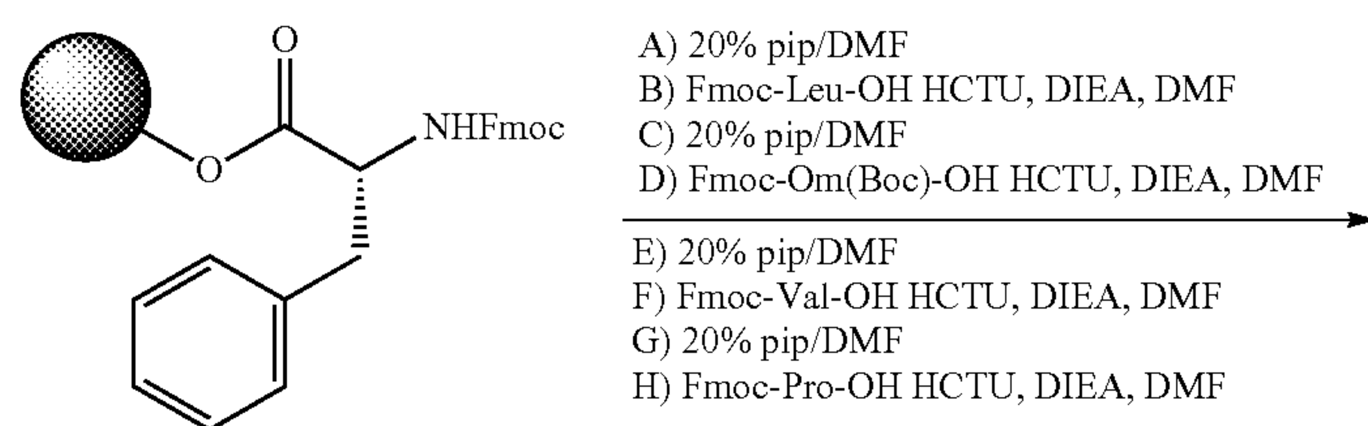
Scheme 3 Solid-Phase Synthesis of the Linear Peptides
