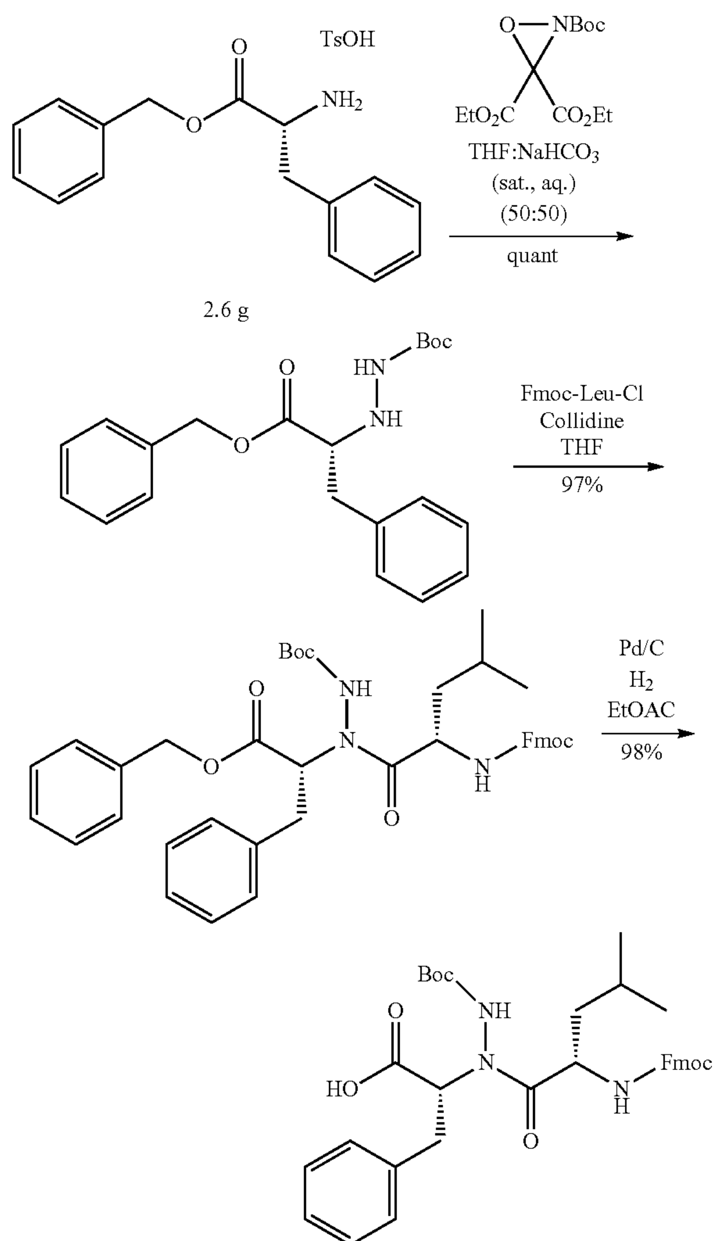
Scheme 1 Synthesis of Dipeptides
