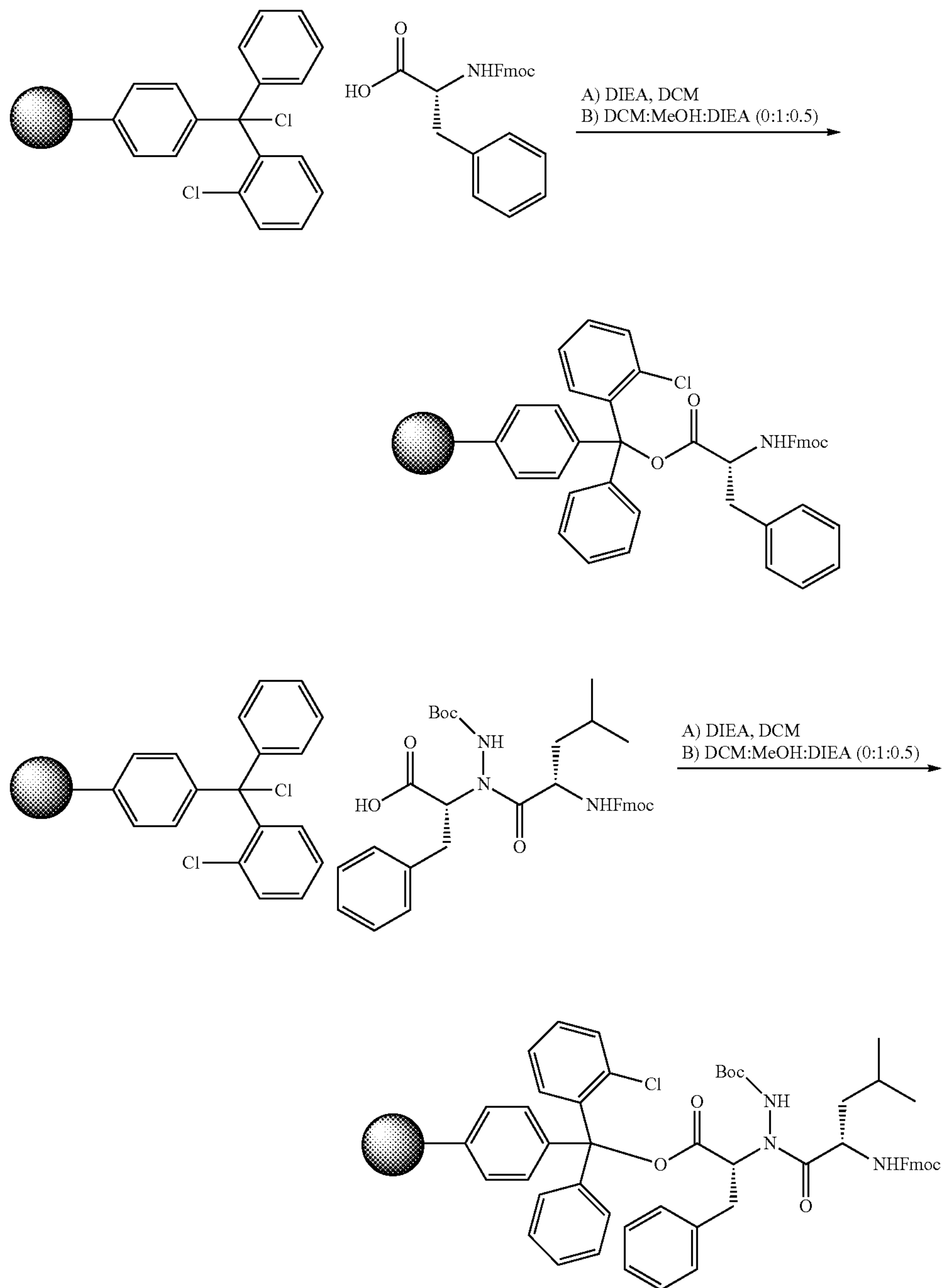
Scheme 2 Loading the 2-Chlorotrityl Chloride Resin
