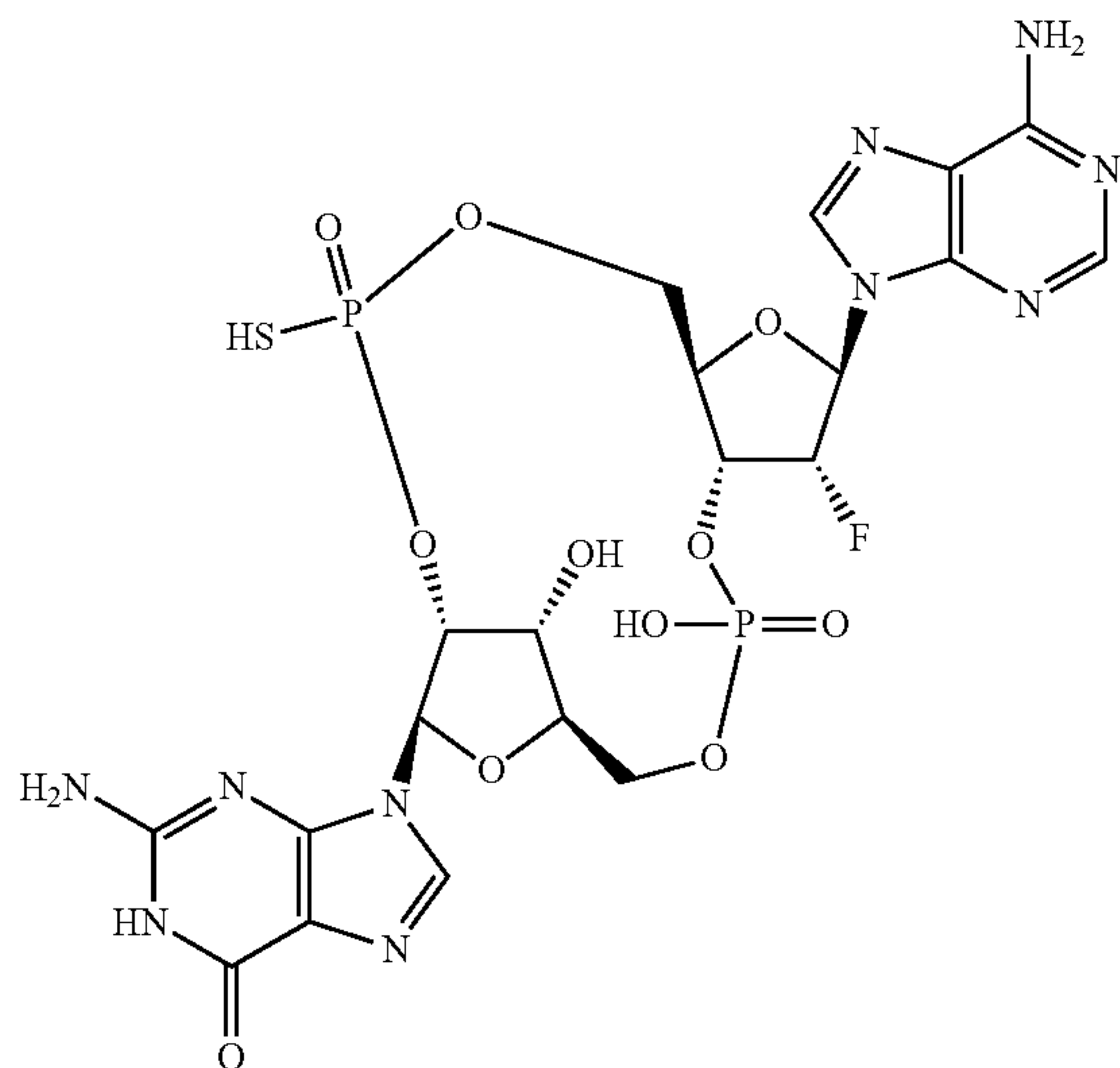
28a-Isomer 1 &amp; 28b-Isomer 2
