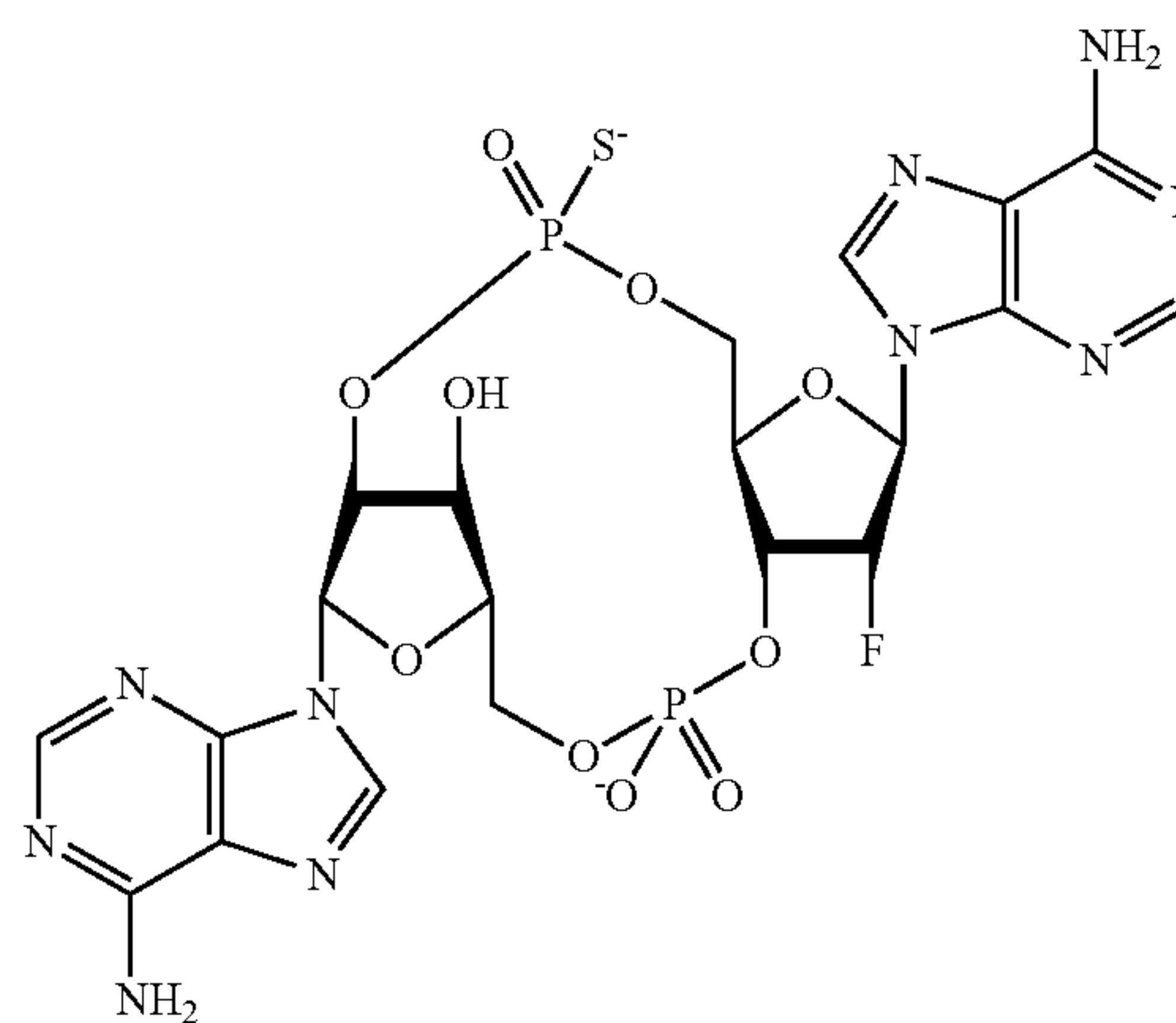
2a - Isomer 1 2b - Isomer 2
