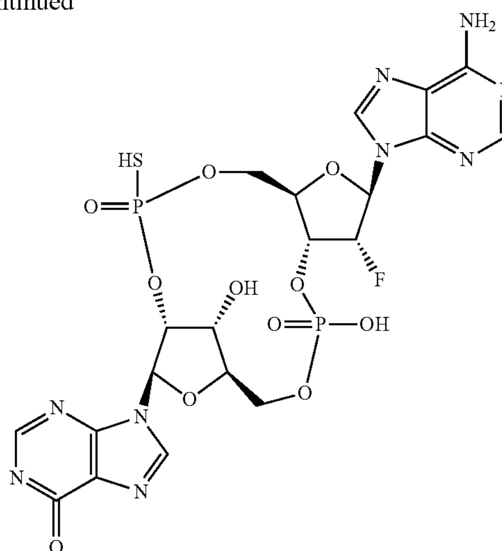
2a-Isomer 1 &amp; 2b-Isomer 2
