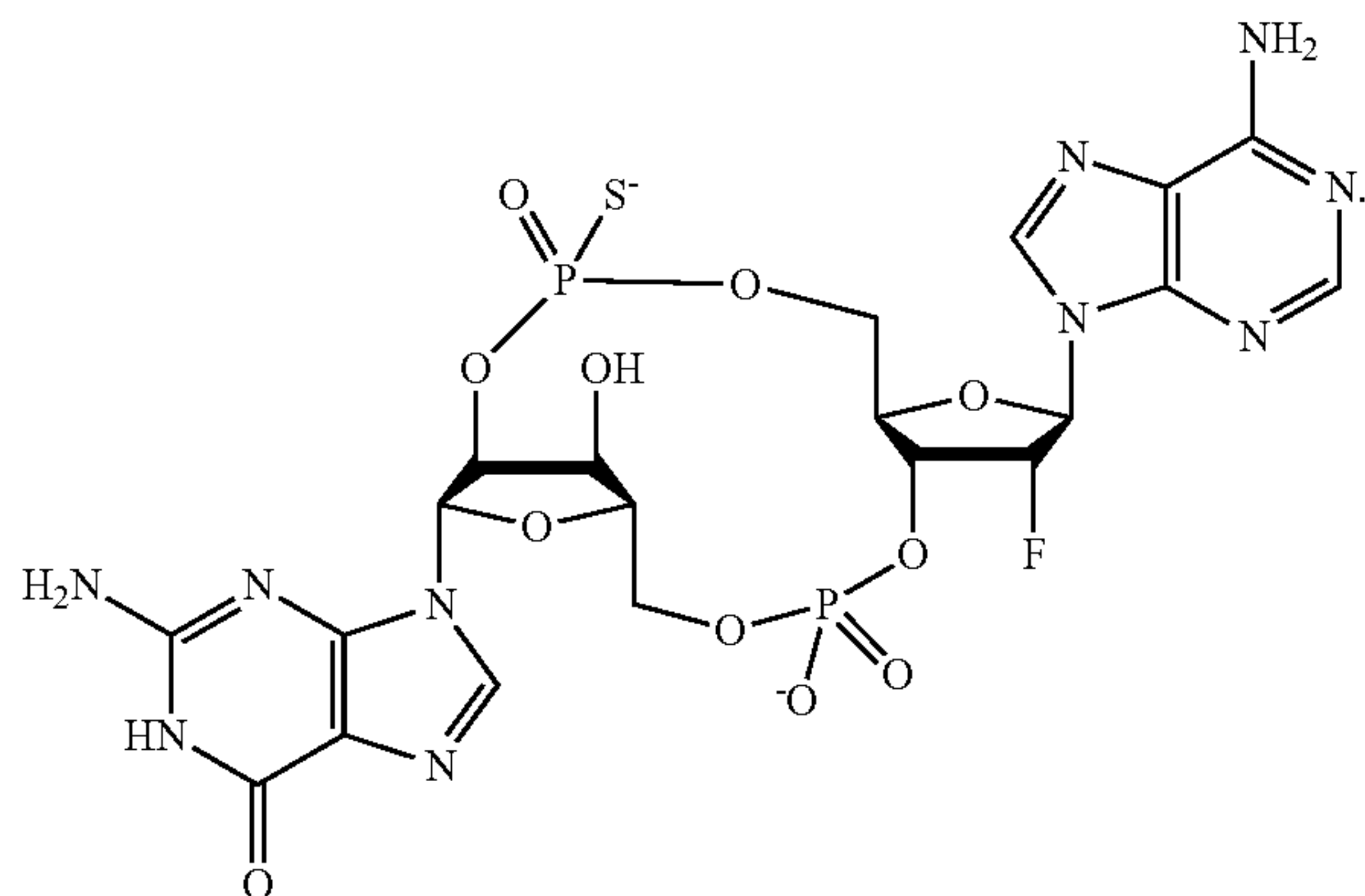
Compound 28
