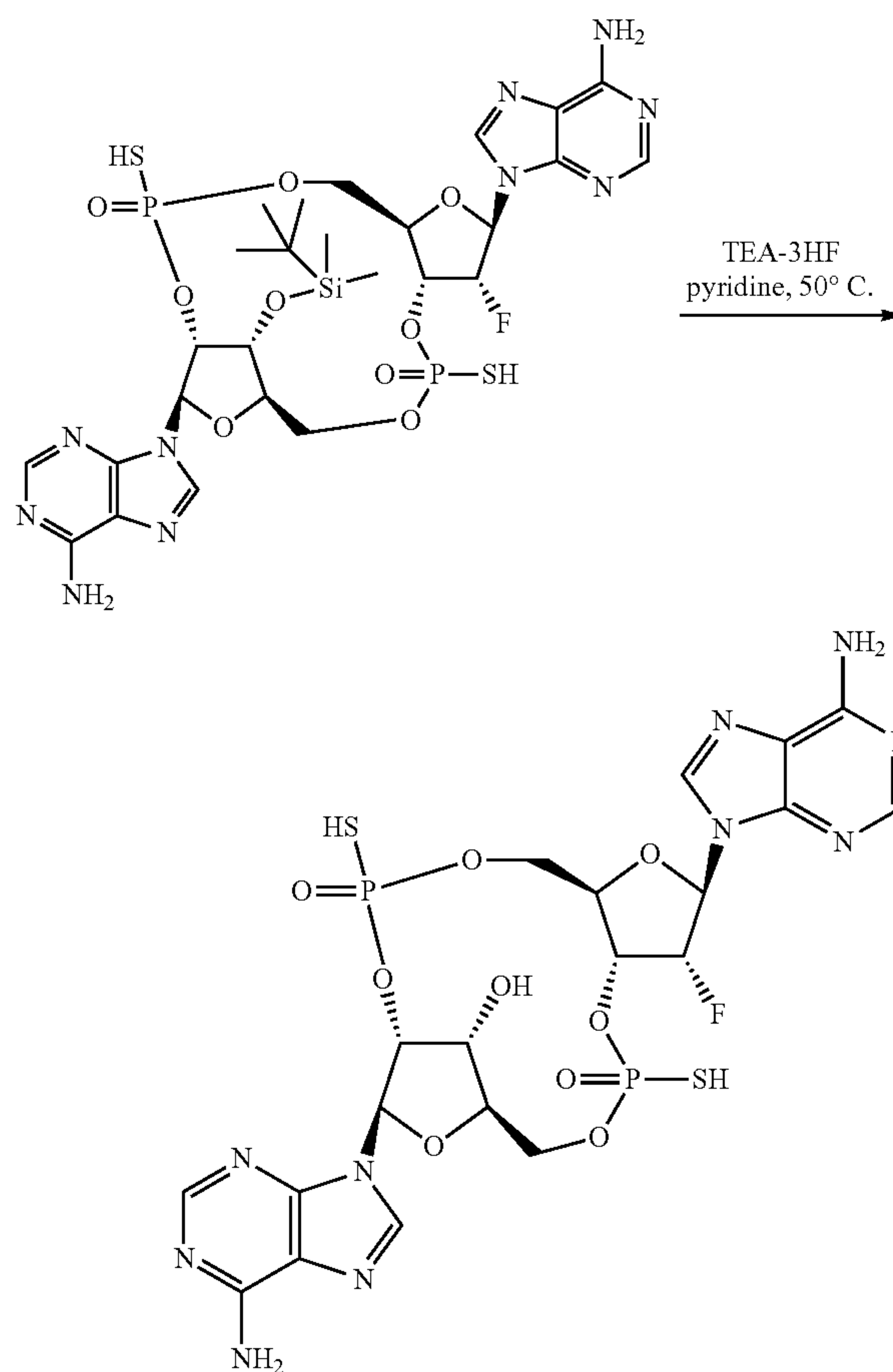
1a-Isomer 1 &amp; 1b-Isomer 2
