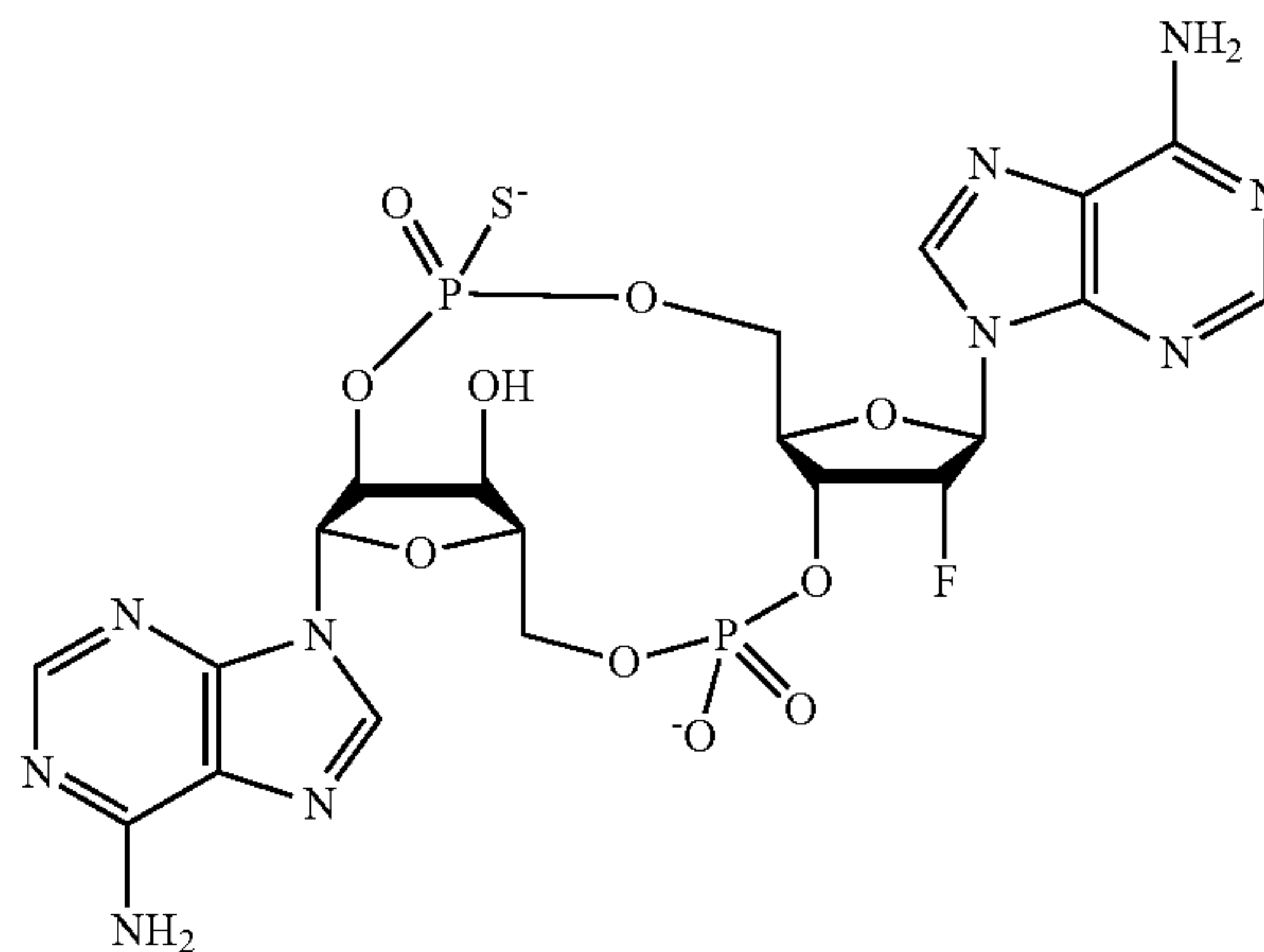
Compound 2
