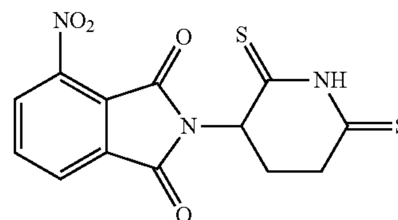
9: C 13 H 9 N 3 O 4 S 2 MW 335.36
