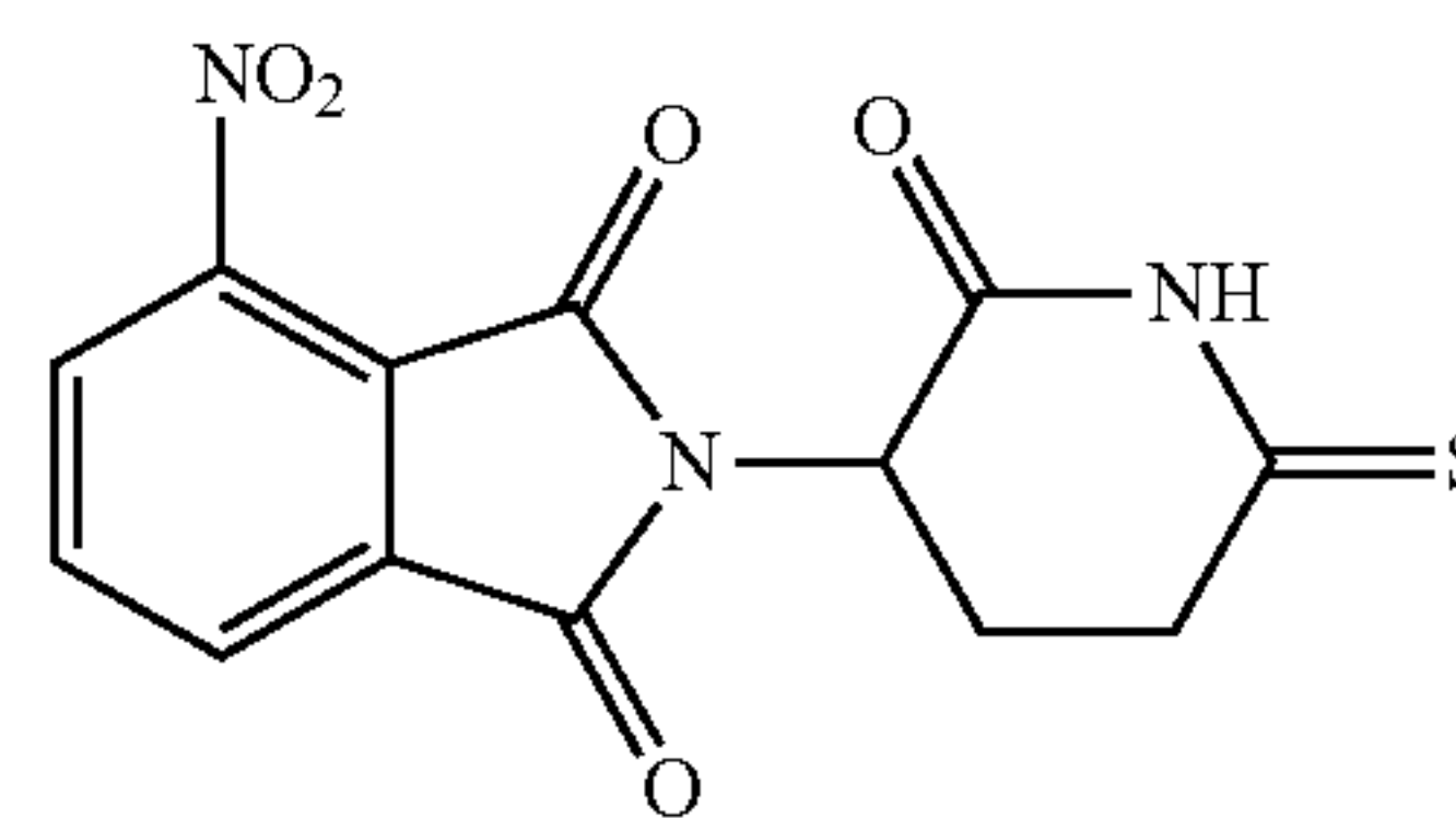
7: C 13 H 9 N 3 O 5 S MW 319.29
