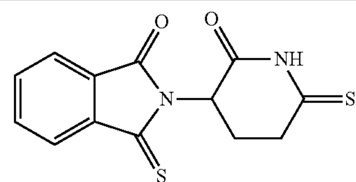
2: C 13 H 10 N 2 O 2 S 2 MW 290.36
