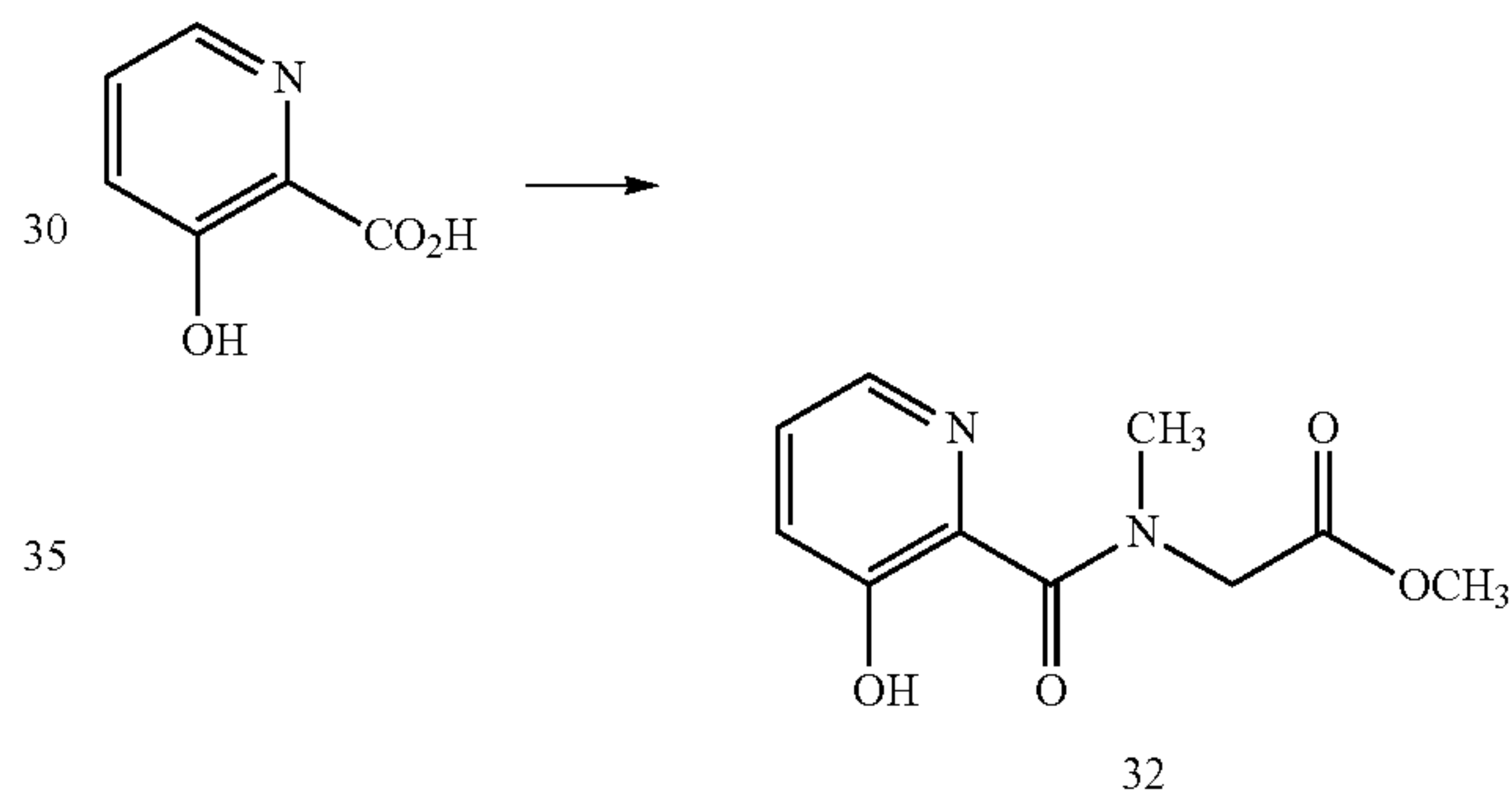
Scheme XIX
