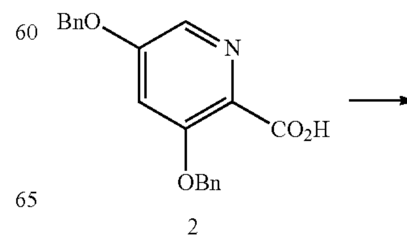
Scheme IX
