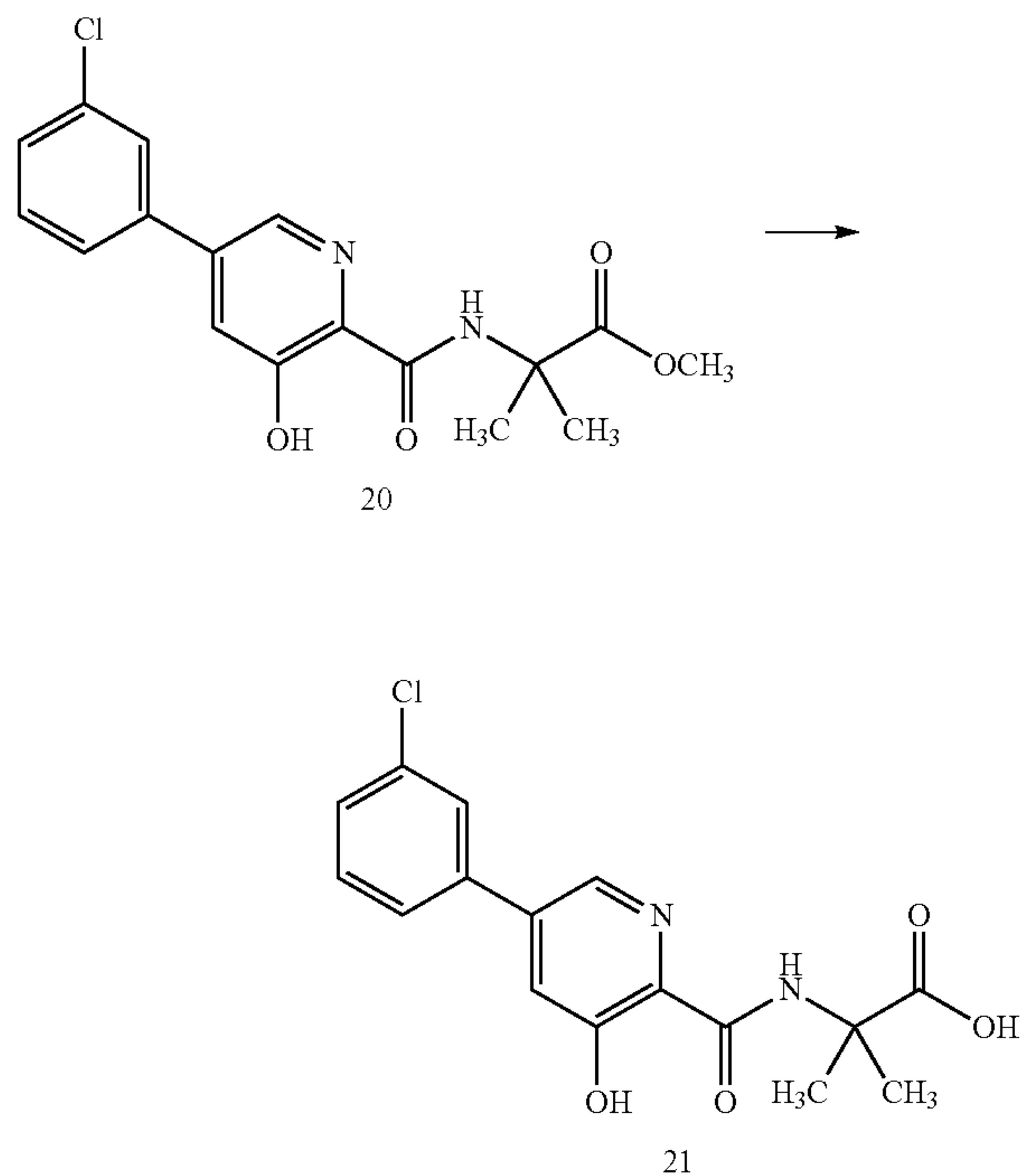
Scheme X
