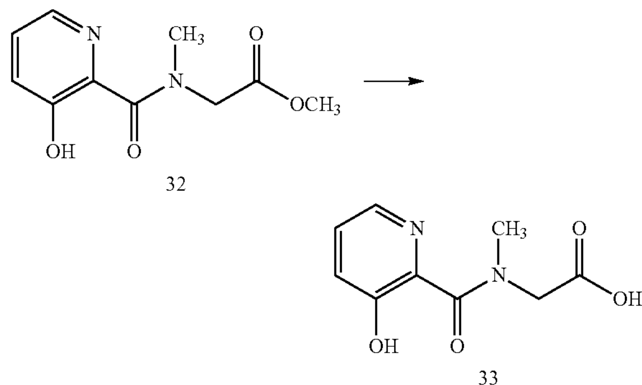
Scheme XX
