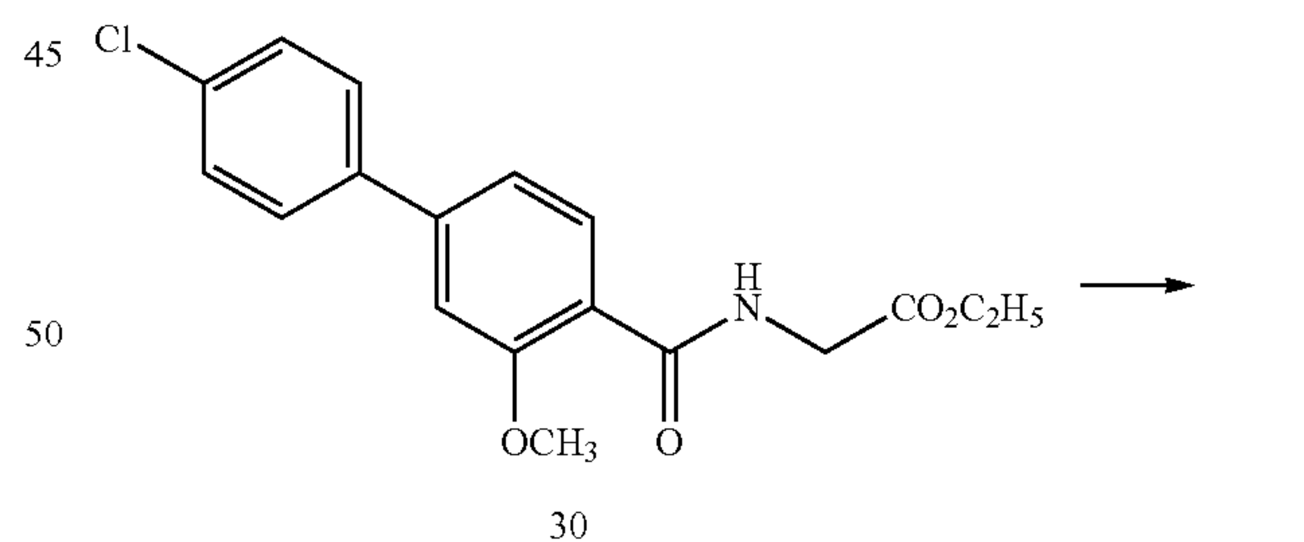
Scheme XVIII
