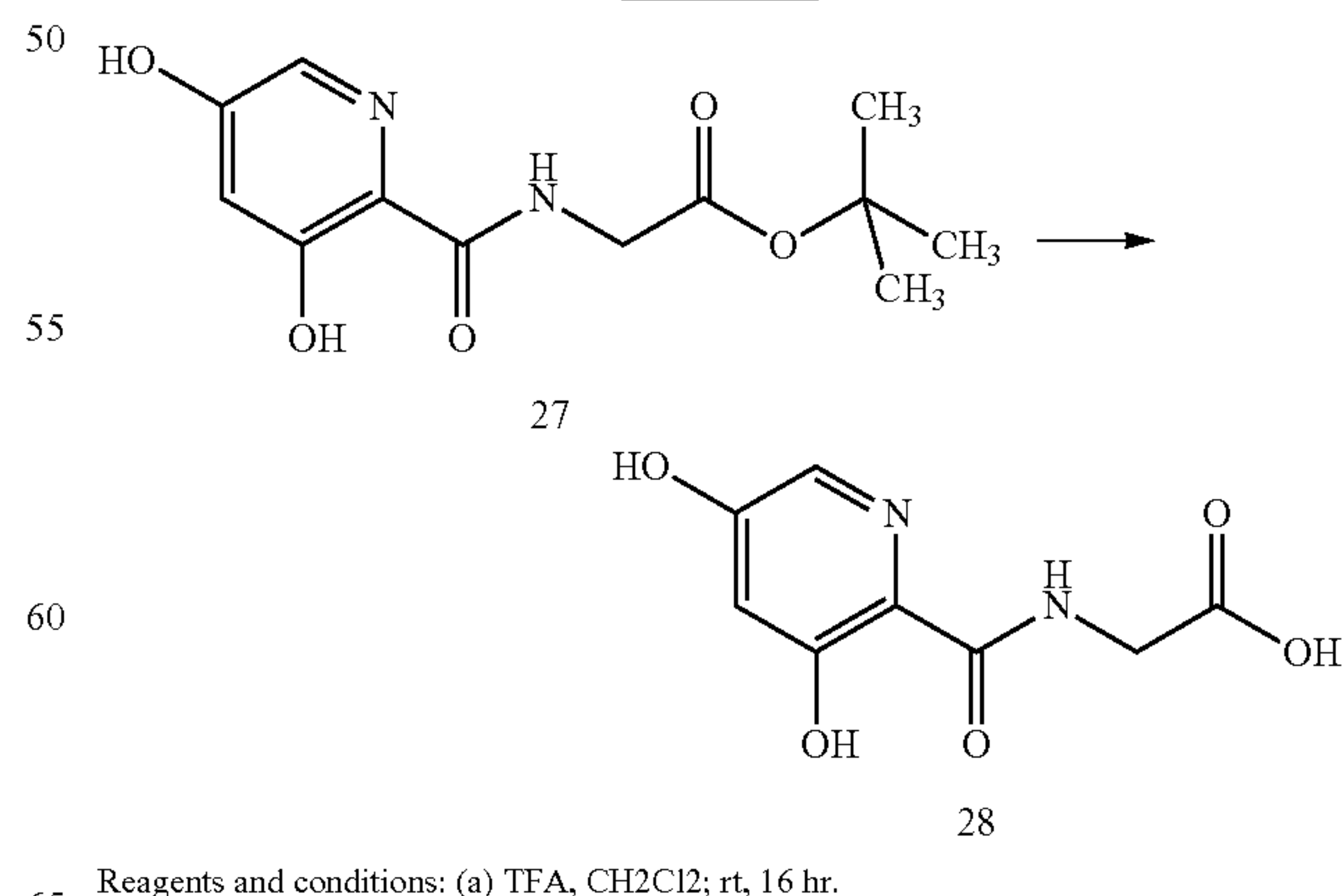
Scheme XV
