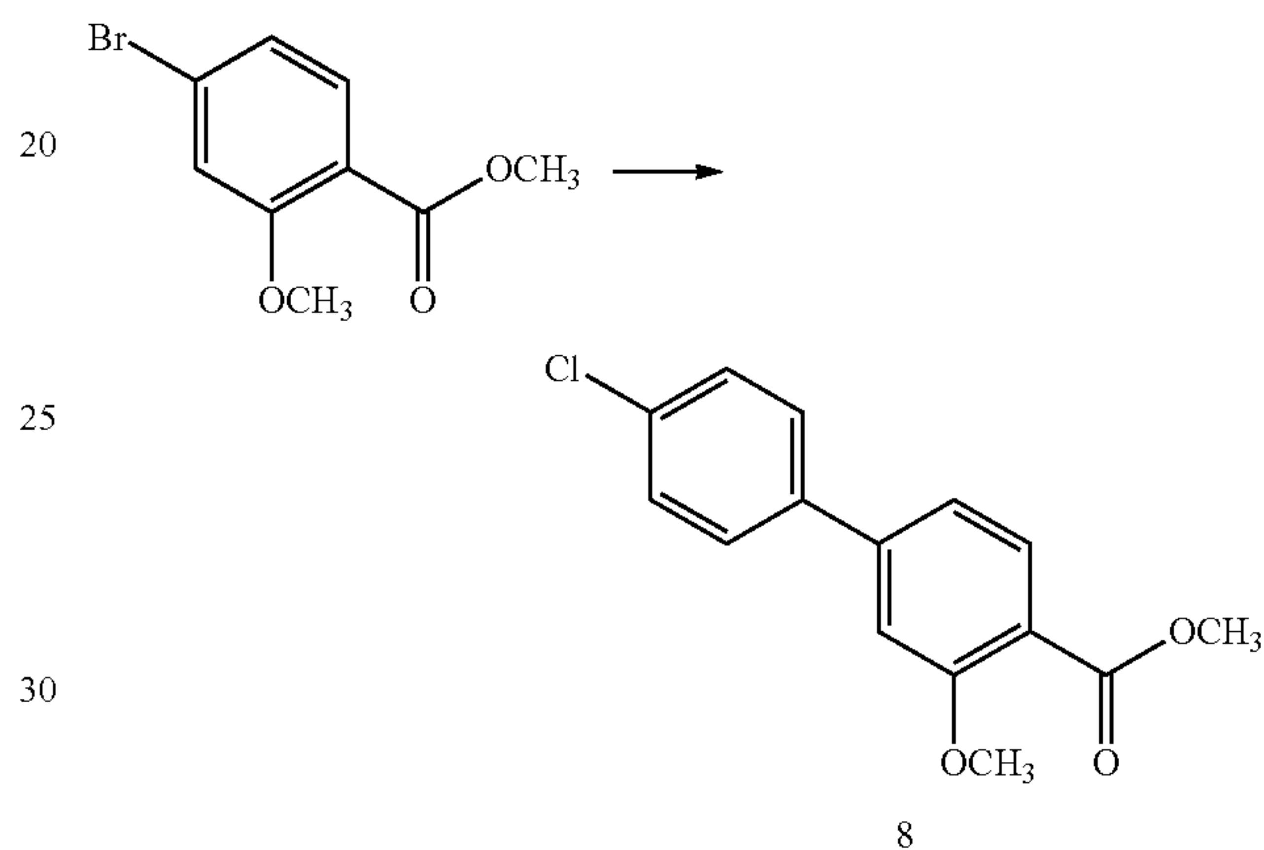
Scheme V
