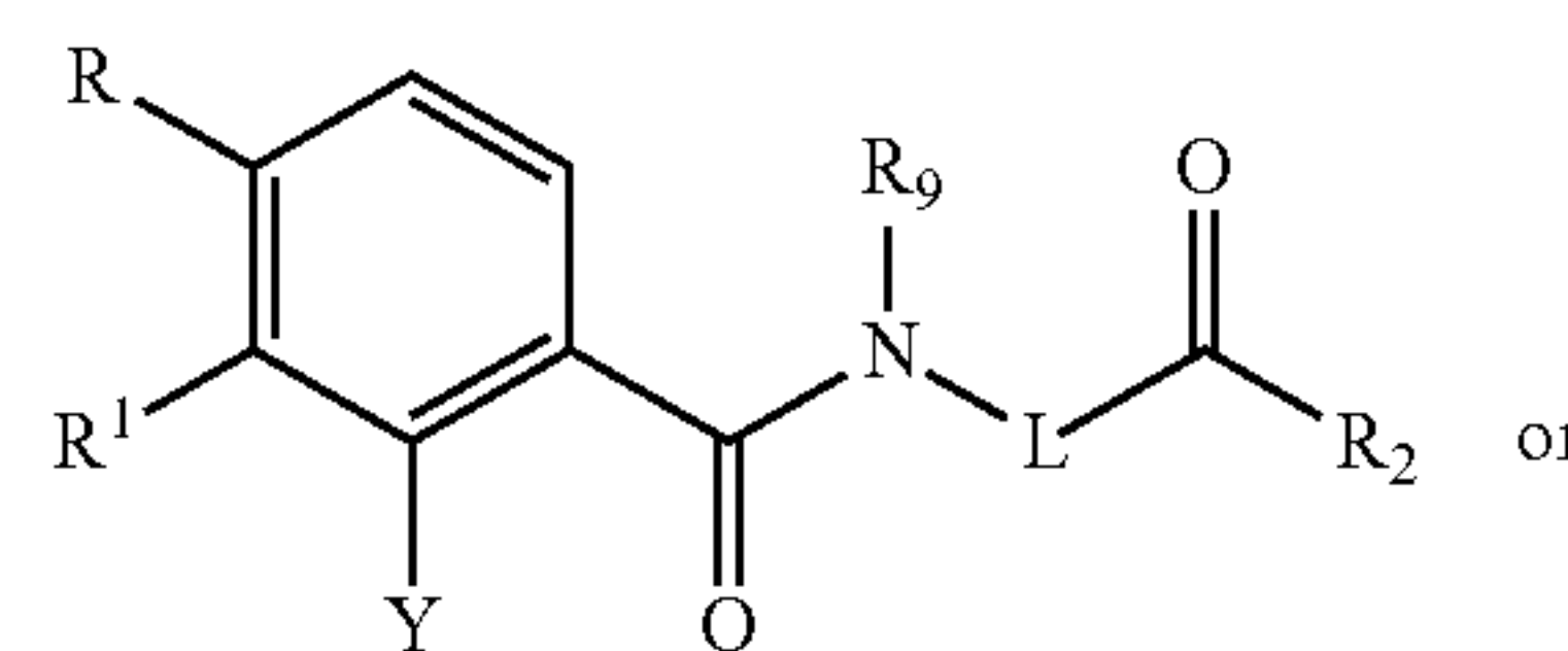
arylamide
