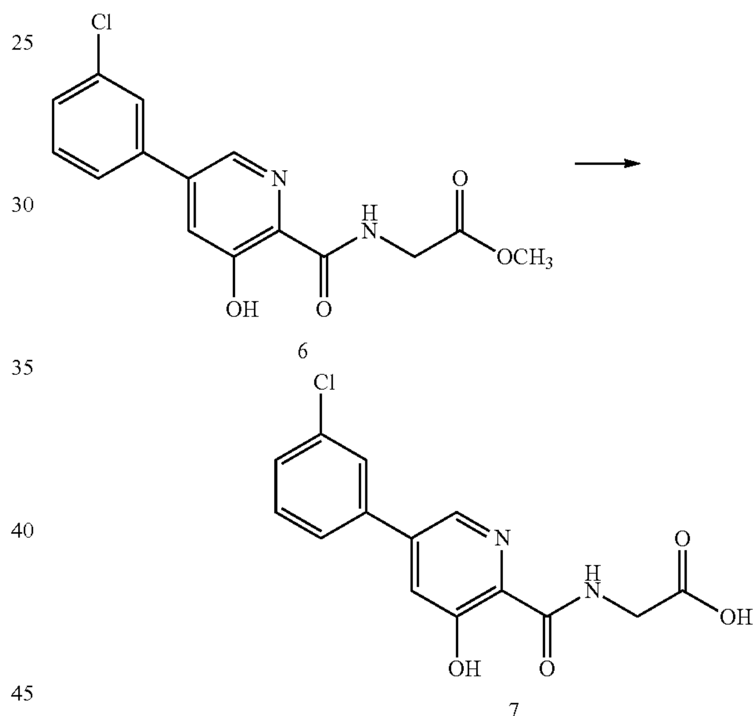
Scheme II
