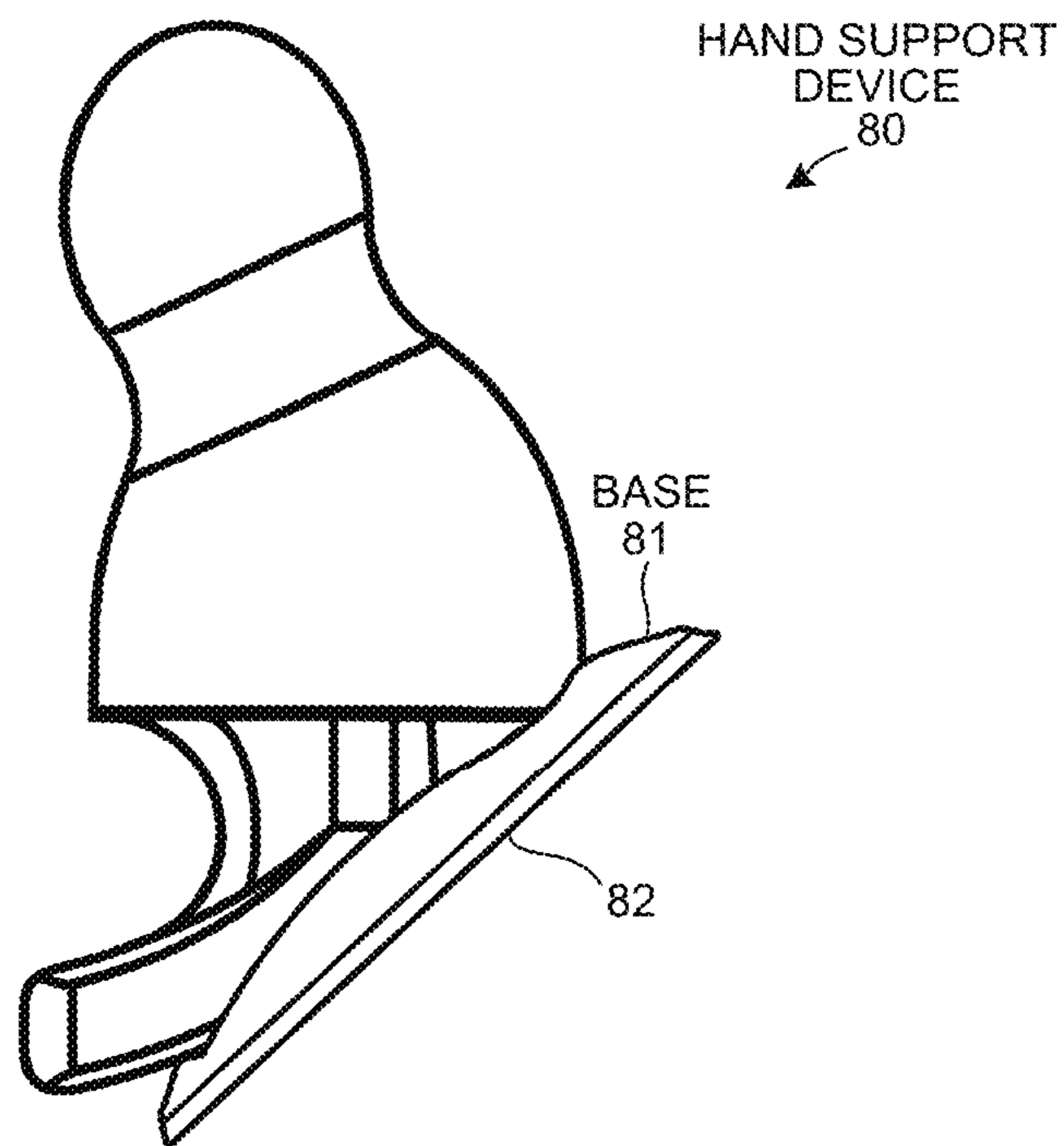
SIDE VIEW OF HAND SUPPORT DEVICE (THIRD EMBODIMENT) FIG. 18
