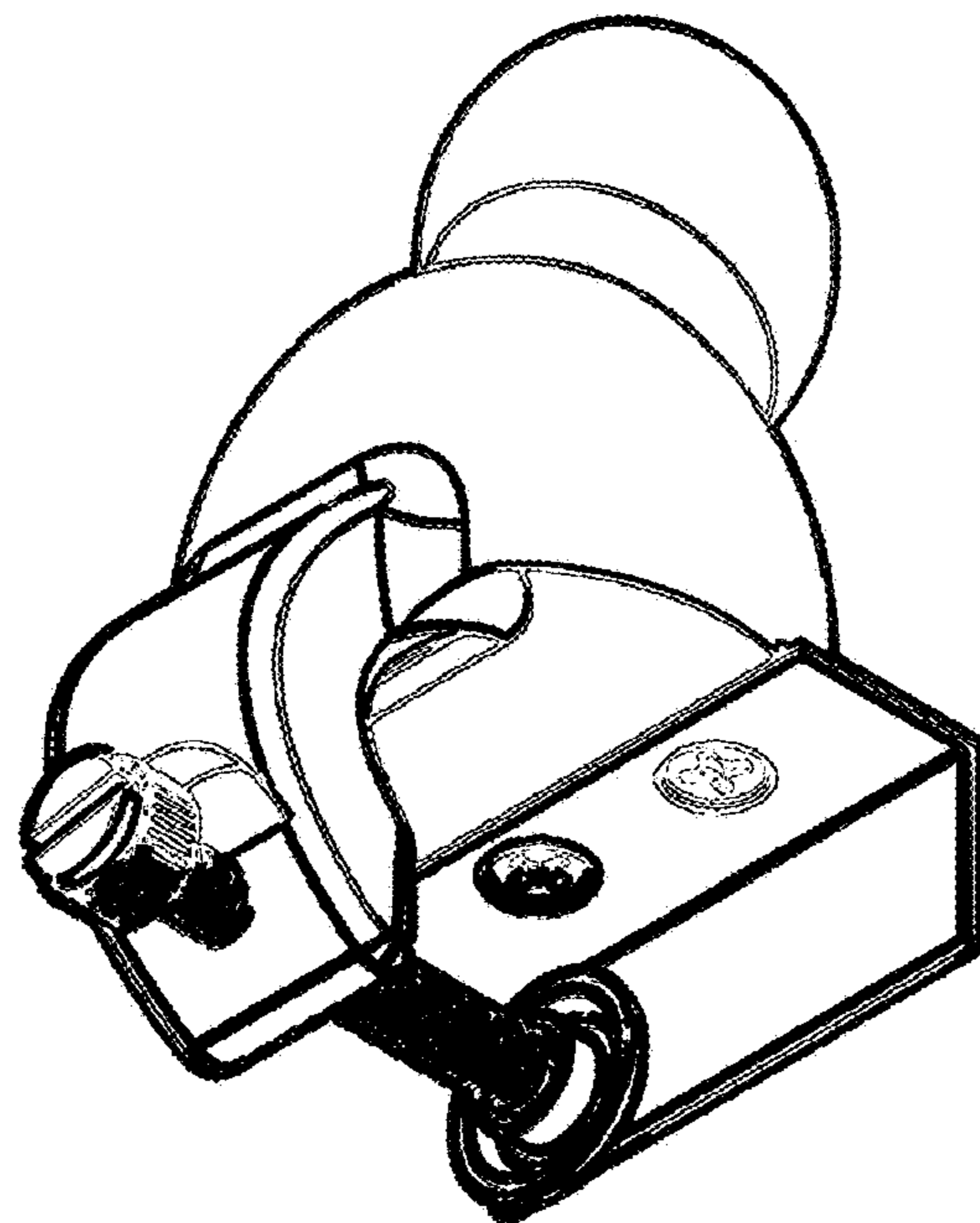
PERSPECTIVE VIEW OF HAND SUPPORT DEVICE FIG. 3
