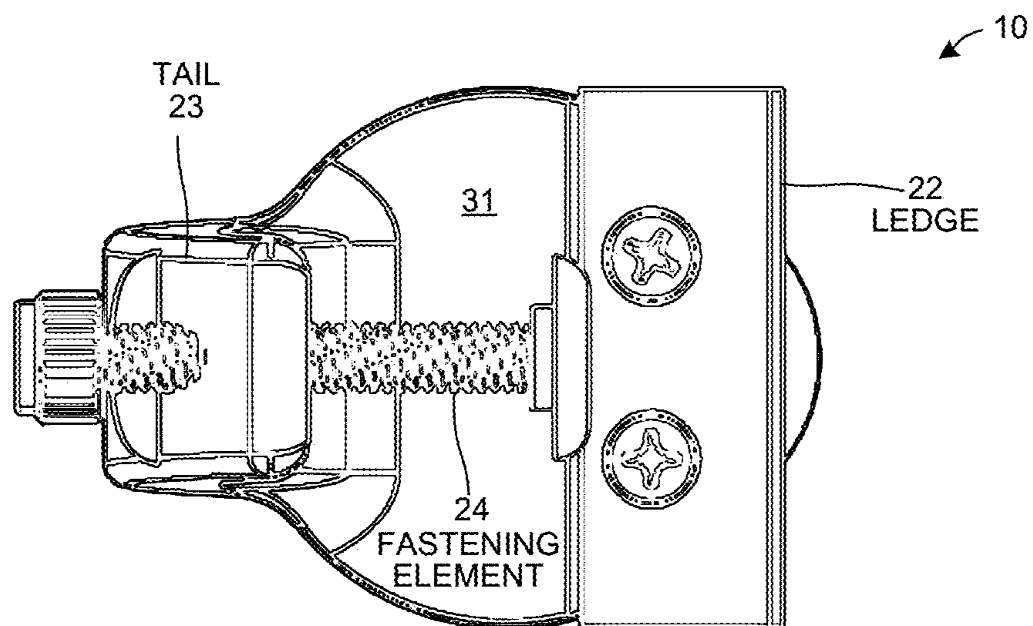
BOTTOM VIEW OF HAND SUPPORT DEVICE FIG. 7
