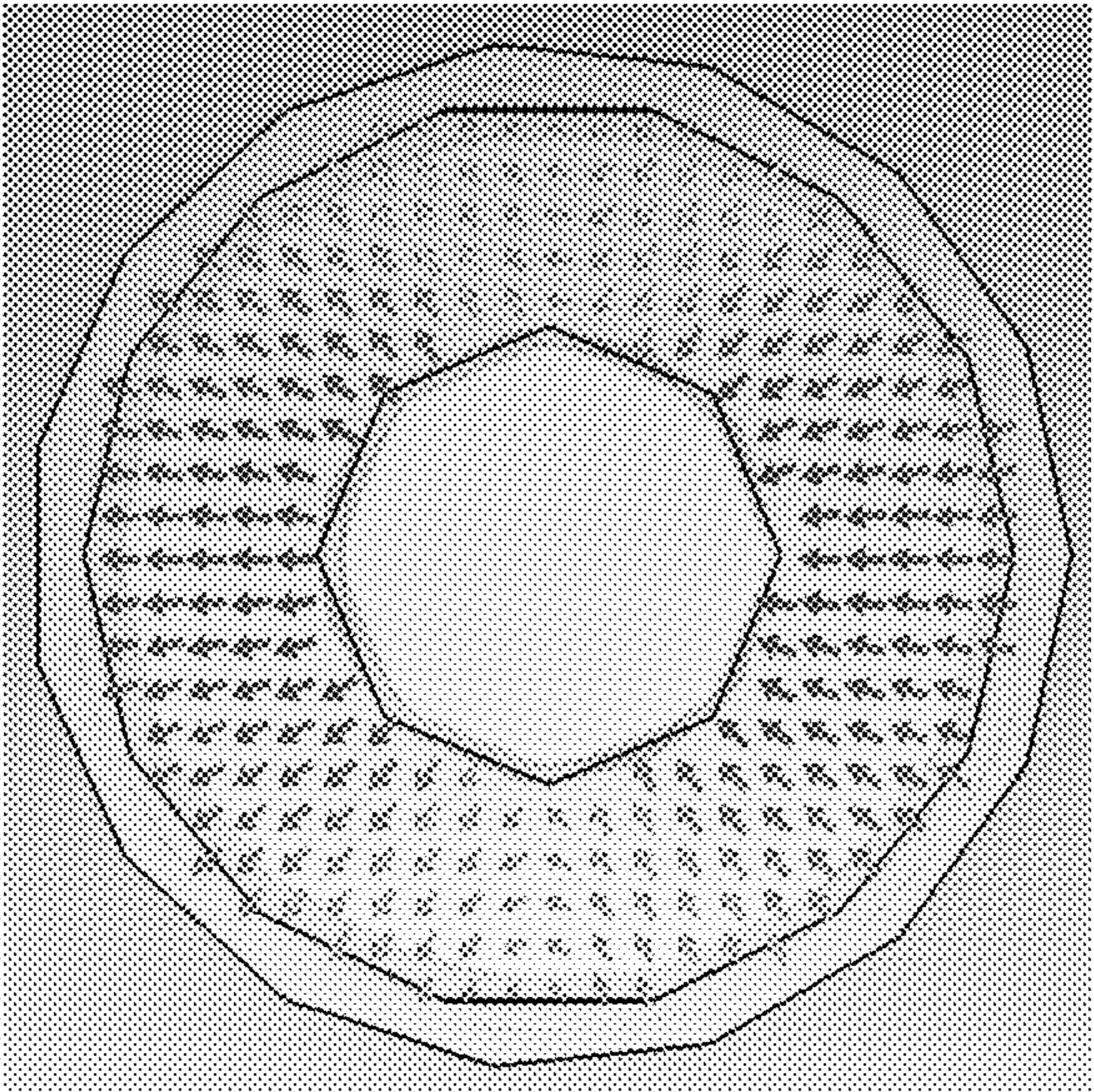
HE11, Vertical Polarization
