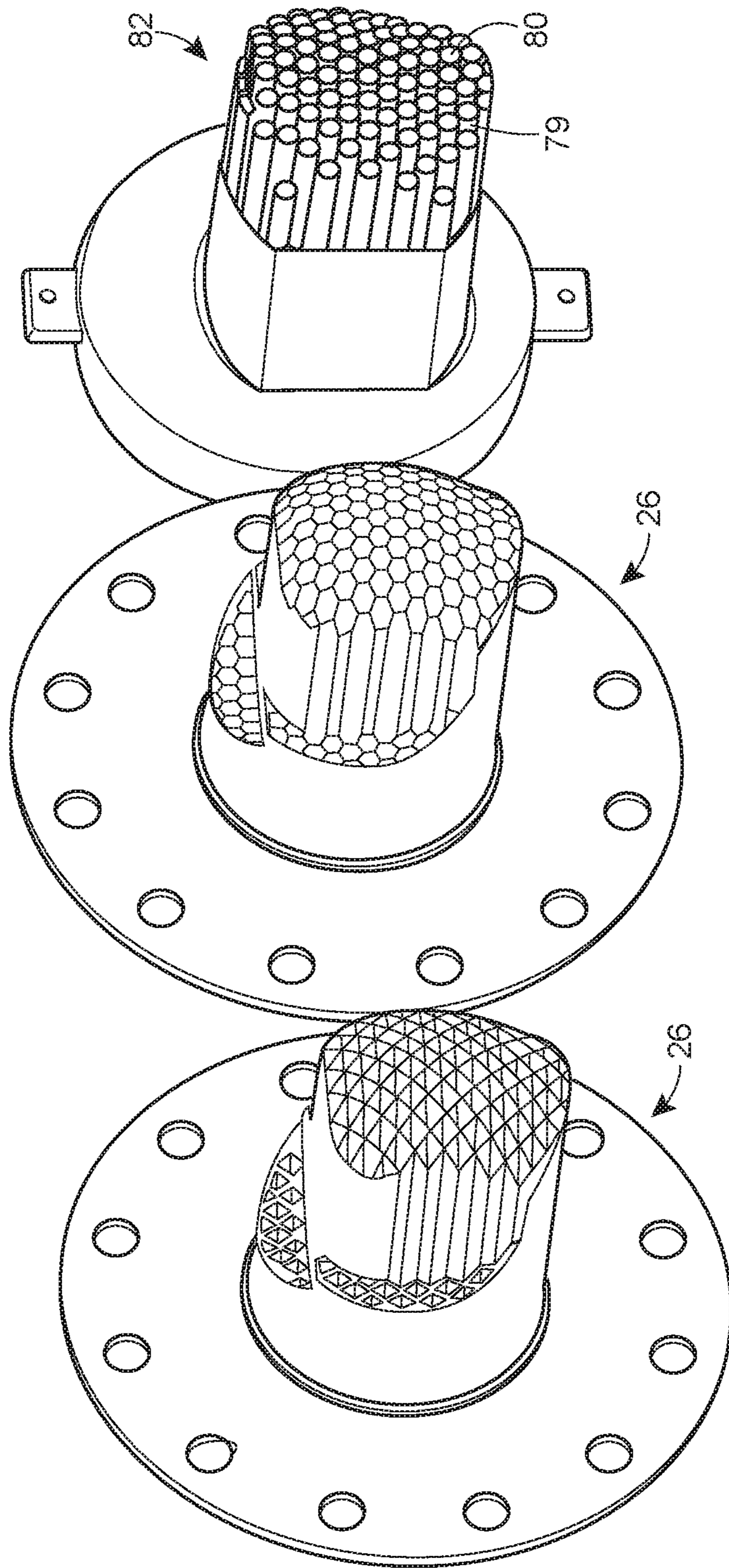
FIG. 13C (PRIOR ART)
