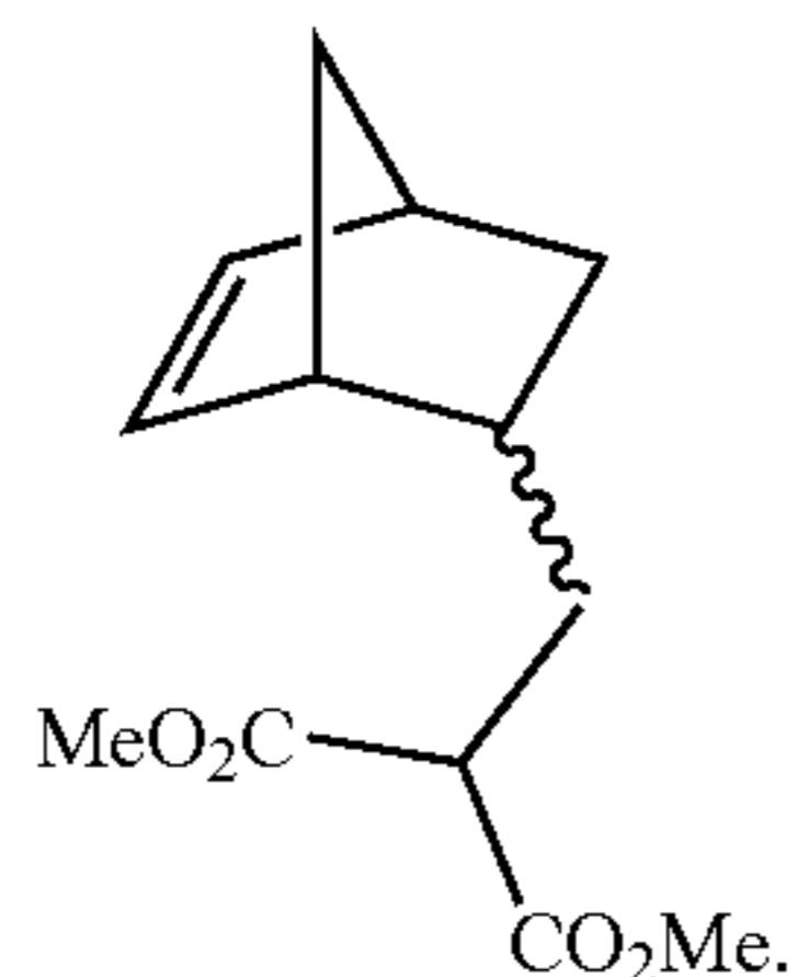
dimethyl 2-((bicyclo[2.2.1]hept-5-en-2-yl)methyl)malonate
