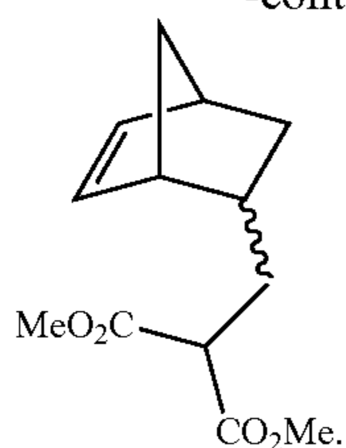
dimethyl 2-((bicyclo[2.2.1]hept-5-en-2-yl)methyl)malonate
