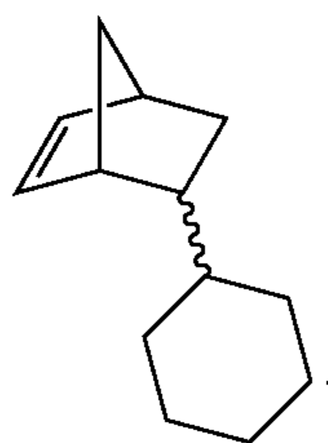
5-cyclohexylbicyclo[2.2.1]hept-2-ene (NBCyHex)
