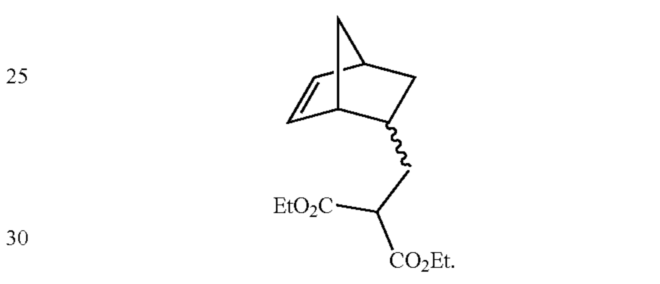
diethyl 2-((bicyclo[2.2.1]hept-5-en-2-yl)methyl)malonate
