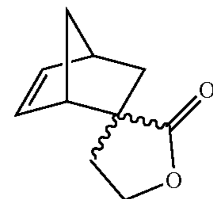
4',5'-dihydro-2'H-spiro[bicyclo[2.2.1]heptane-2,3'-furan]-5-en-2'-one or spiro lactone NB (NBSL)
