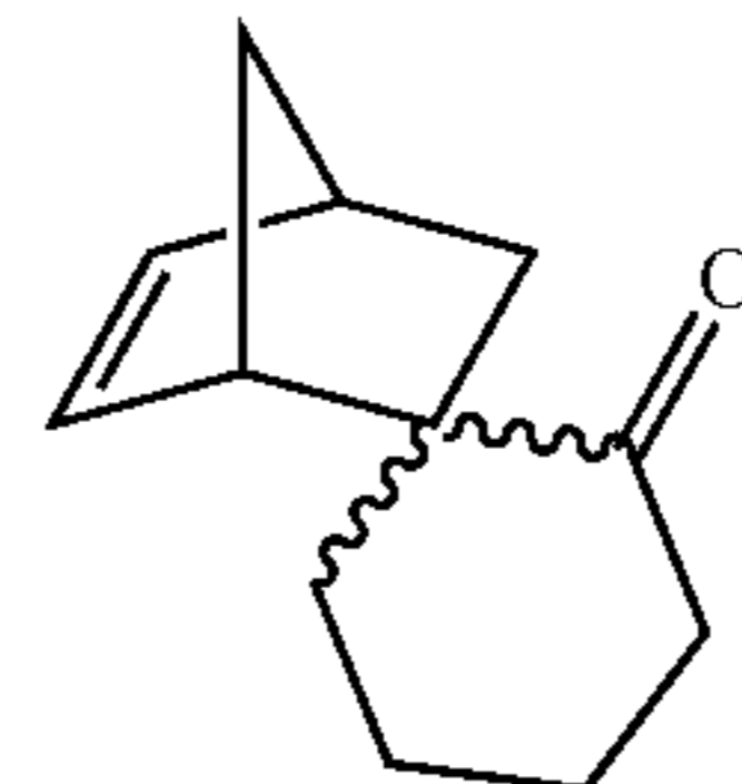
spiro[bicyclo[2.2.1]heptane-2,3'-piperidin]-5-en-2'-one
