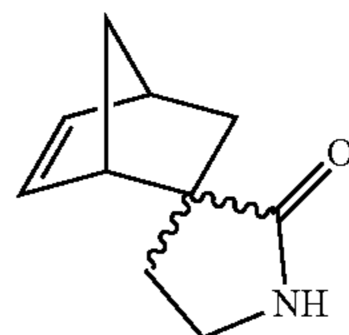
spiro[bicyclo[2.2.1]heptane-2,3'-pyrrolidin]-5-en-2'-one
