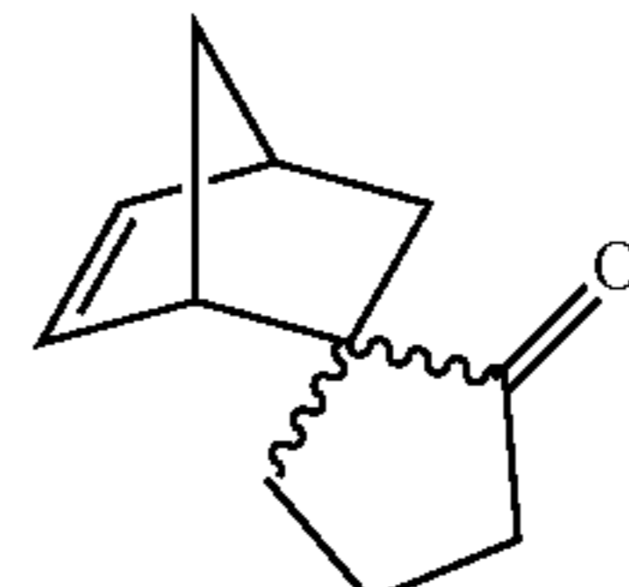
spiro[bicyclo[2.2.1]heptane-2,1'-cyclopentan]-5-en-2'-one
