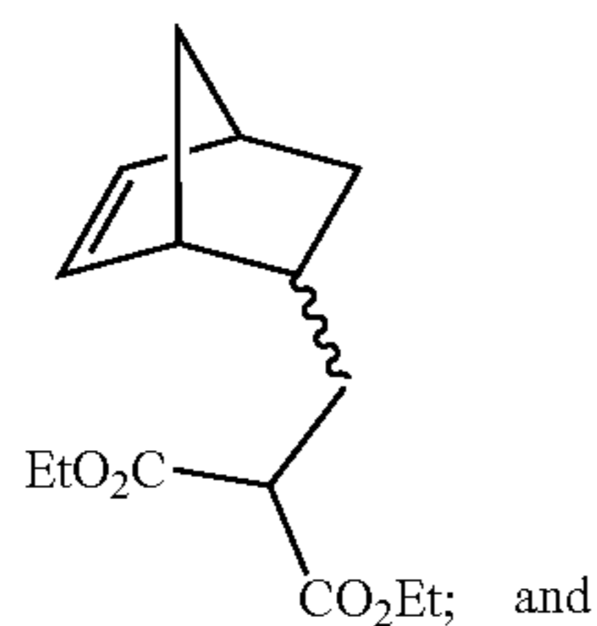
diethyl 2-((bicyclo[2.2.1]hept-5-en-2-yl)methyl)malonate
