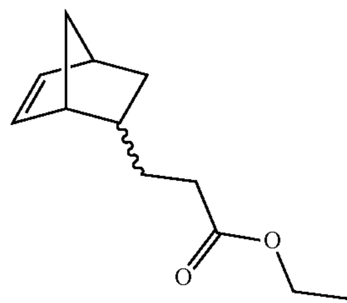
ethyl 3-(bicyclo[2.2.1]hept-5-ene-2-yl)propanoate (EPEsNB)
