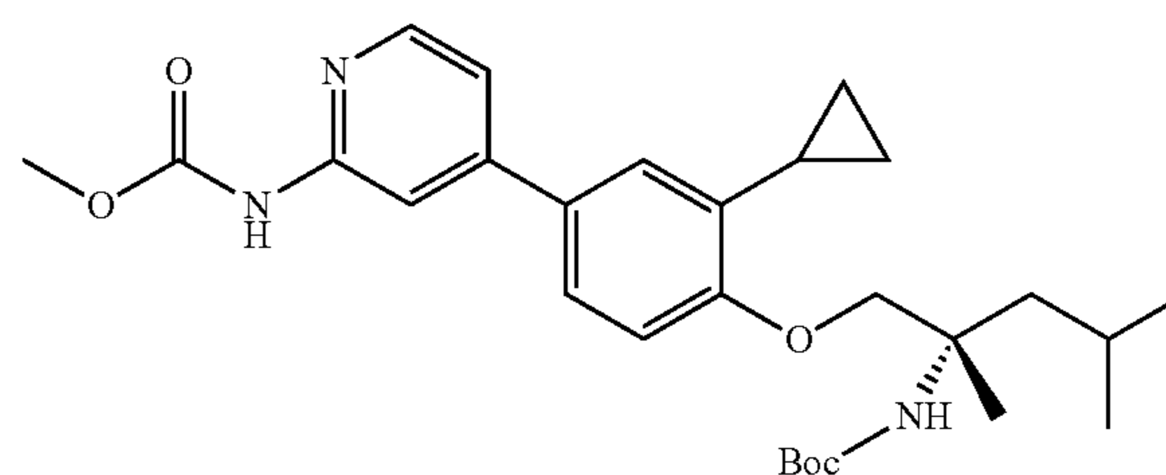
Part C: (S)-methyl (4-(4-((2-Boc-amino-2,4-dimethylpentyl)oxy)-3-cyclopropylphenyl)pyridin-2-yl)carbamate
