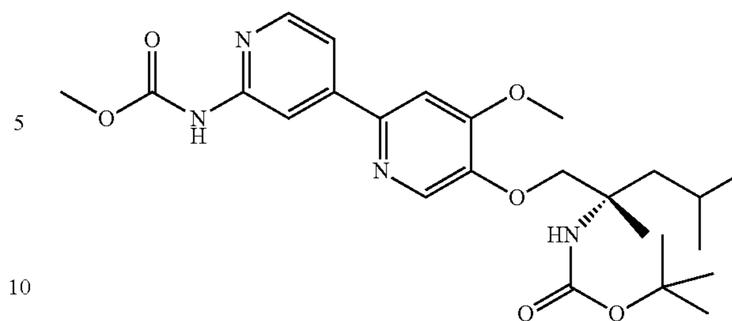
Part C: Boc protected (S)-methyl (5-((2-amino-2,4-dimethylpentyl)oxy)-4-methoxy-[2,4'-bipyridin]-2'-yl)carbamate
