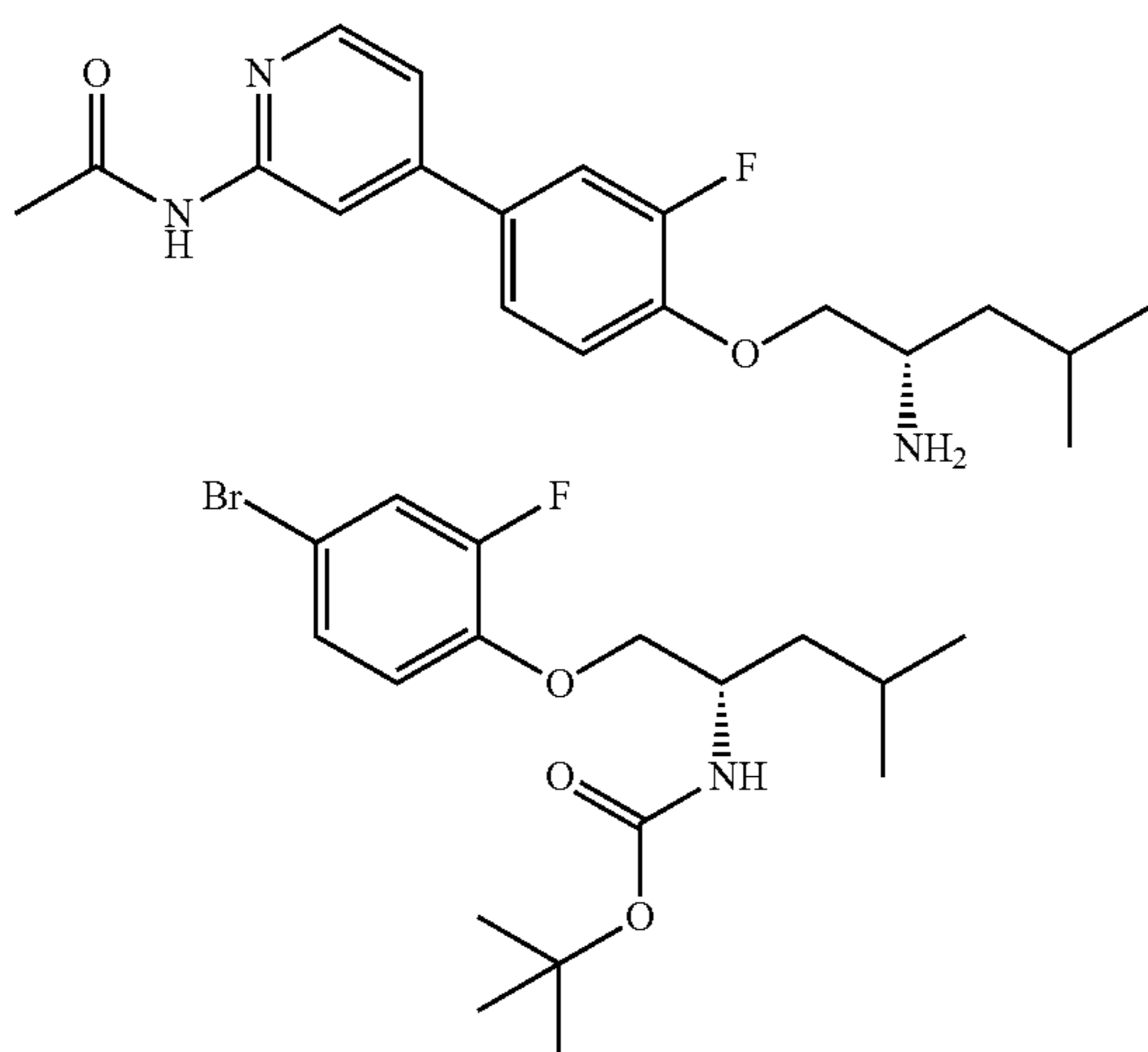
Part 2A: (S)-tert-butyl (1-(4-bromo-2-fluorophenoxy)-4-methylpentan-2-yl)carbamate
