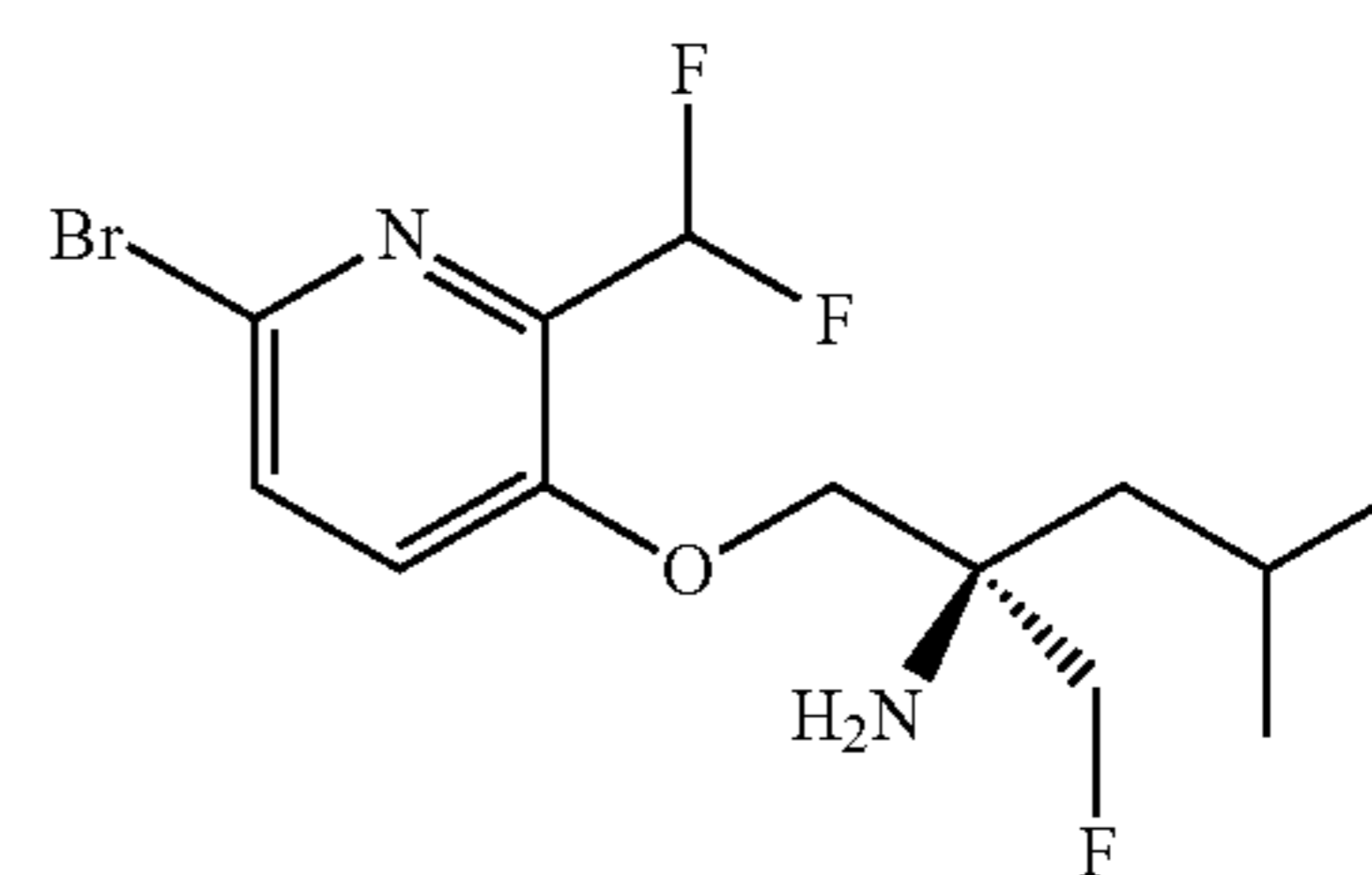
Part C: (R)-1-((6-bromo-2-(difluoromethyl)pyridin-3-yl)oxy)-2-(fluoromethyl)-4-methylpentan-2-amine
