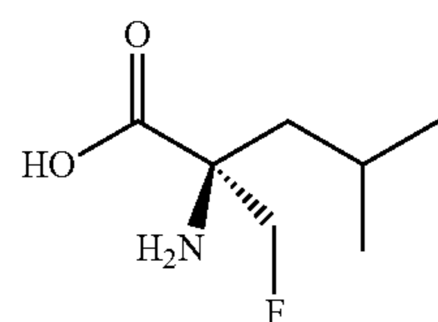
Part A: (R)-2-amino-2-(fluoromethyl)-4-methylpentanoic acid
