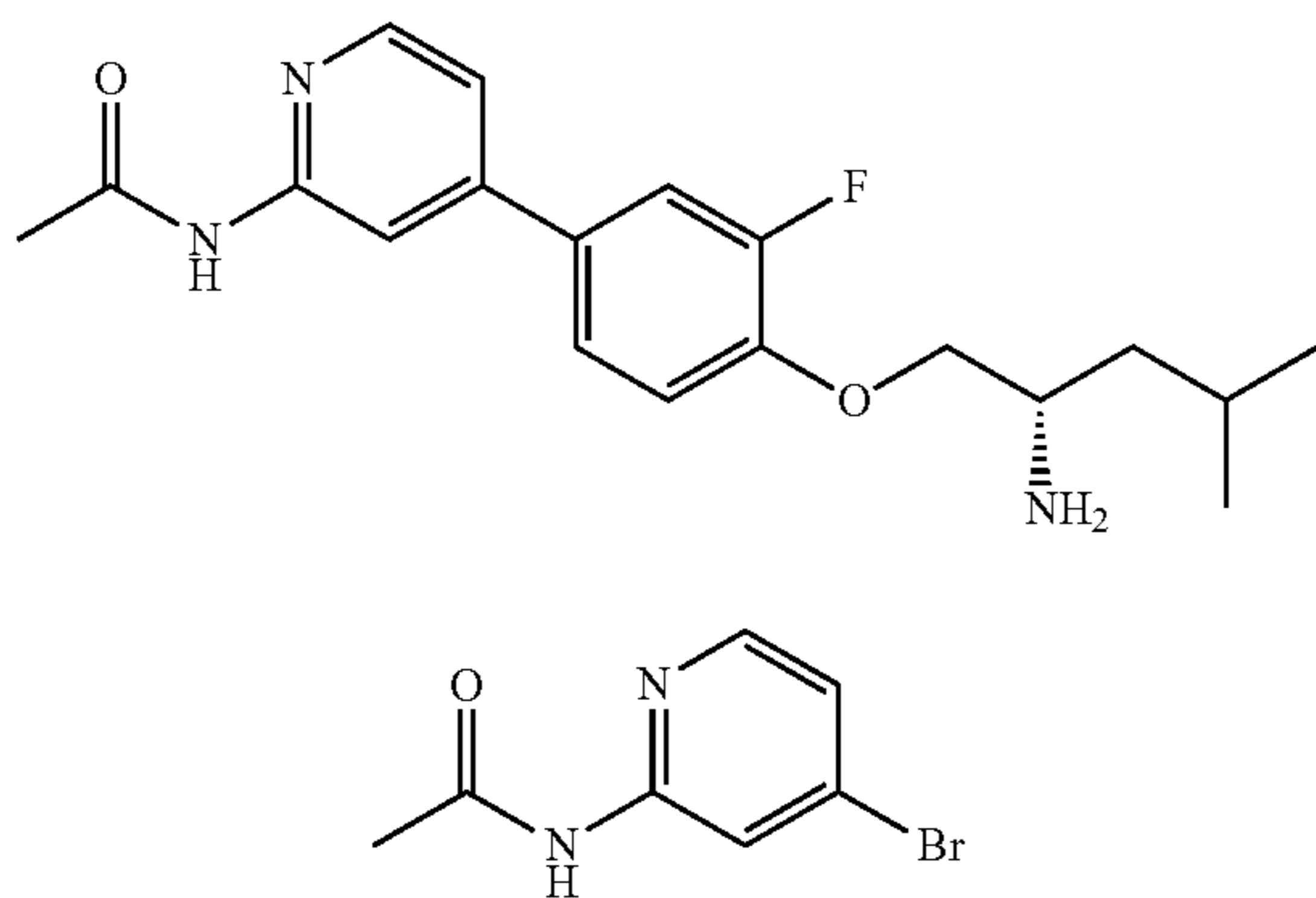
Part A: N-(4-bromopyridin-2-yl)acetamide
