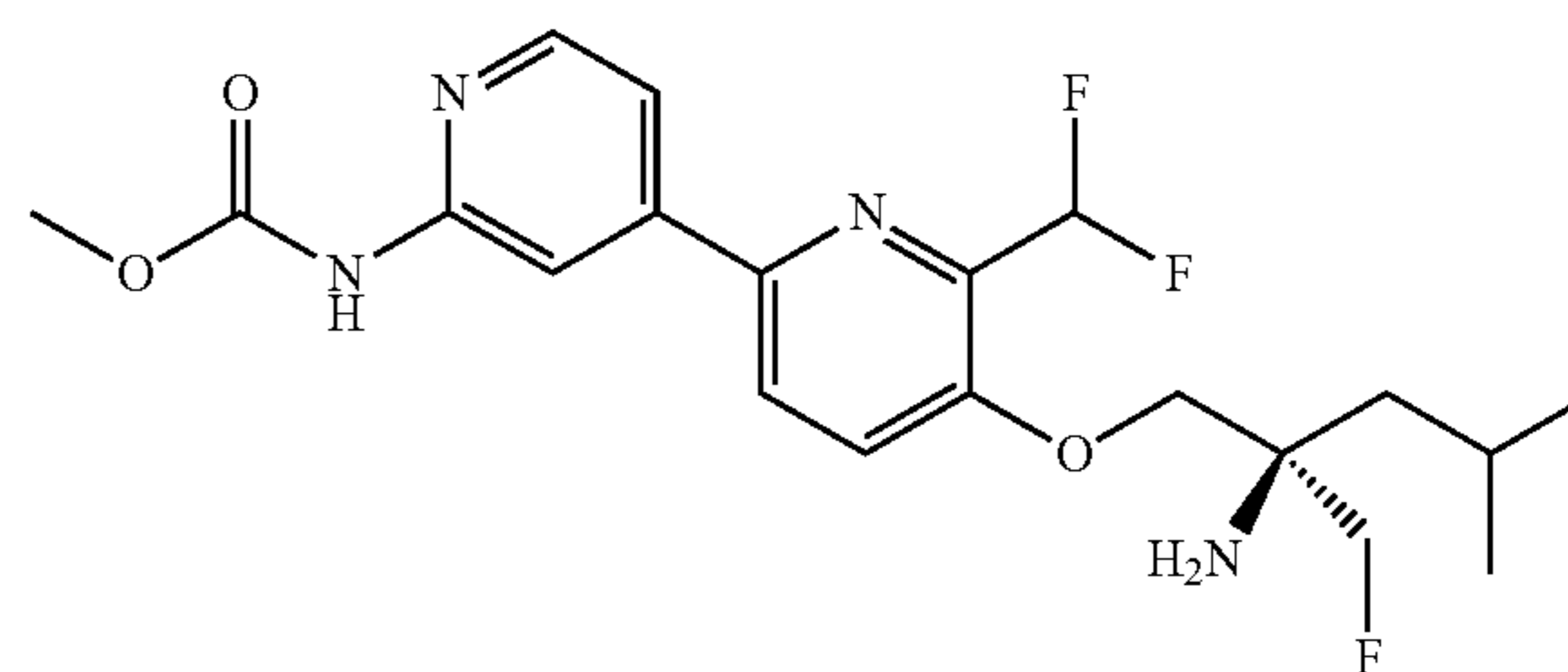
Part D: (R)-methyl (5-((2-amino-2-(fluoromethyl)-4-methylpentyl)oxy)-6-(difluoromethyl)-[2,4'-bipyridin]-2'-yl) carbamate
