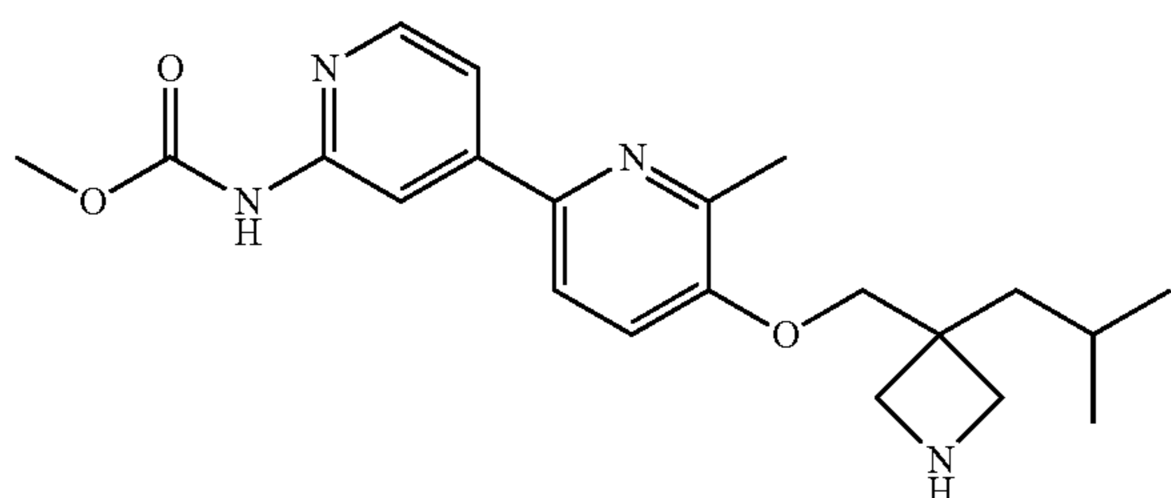
Part D: methyl (5-((3-isobutylazetidin-3-yl)methoxy)-6-methyl-[2,4'-bipyridin]-2'-yl)carbamate
