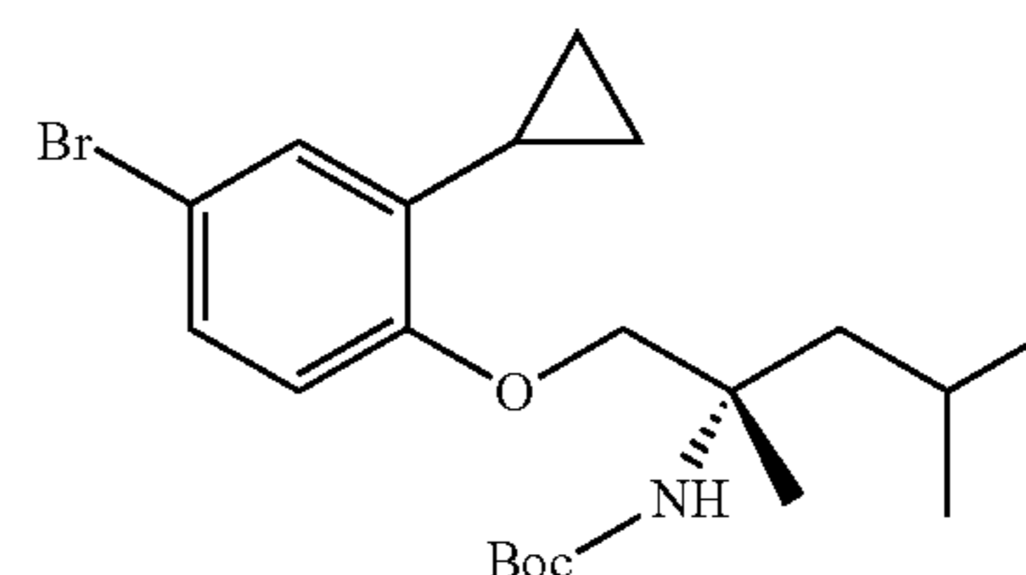
Part B: (S)-tert-butyl (1-(4-bromo-2-cyclopropylphenoxy)-2,4-dimethylpentan-2-yl)carbamate
