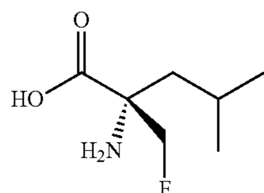
Part C: (S)-2-amino-2-(fluoromethyl)-4-methylpentanoic acid
