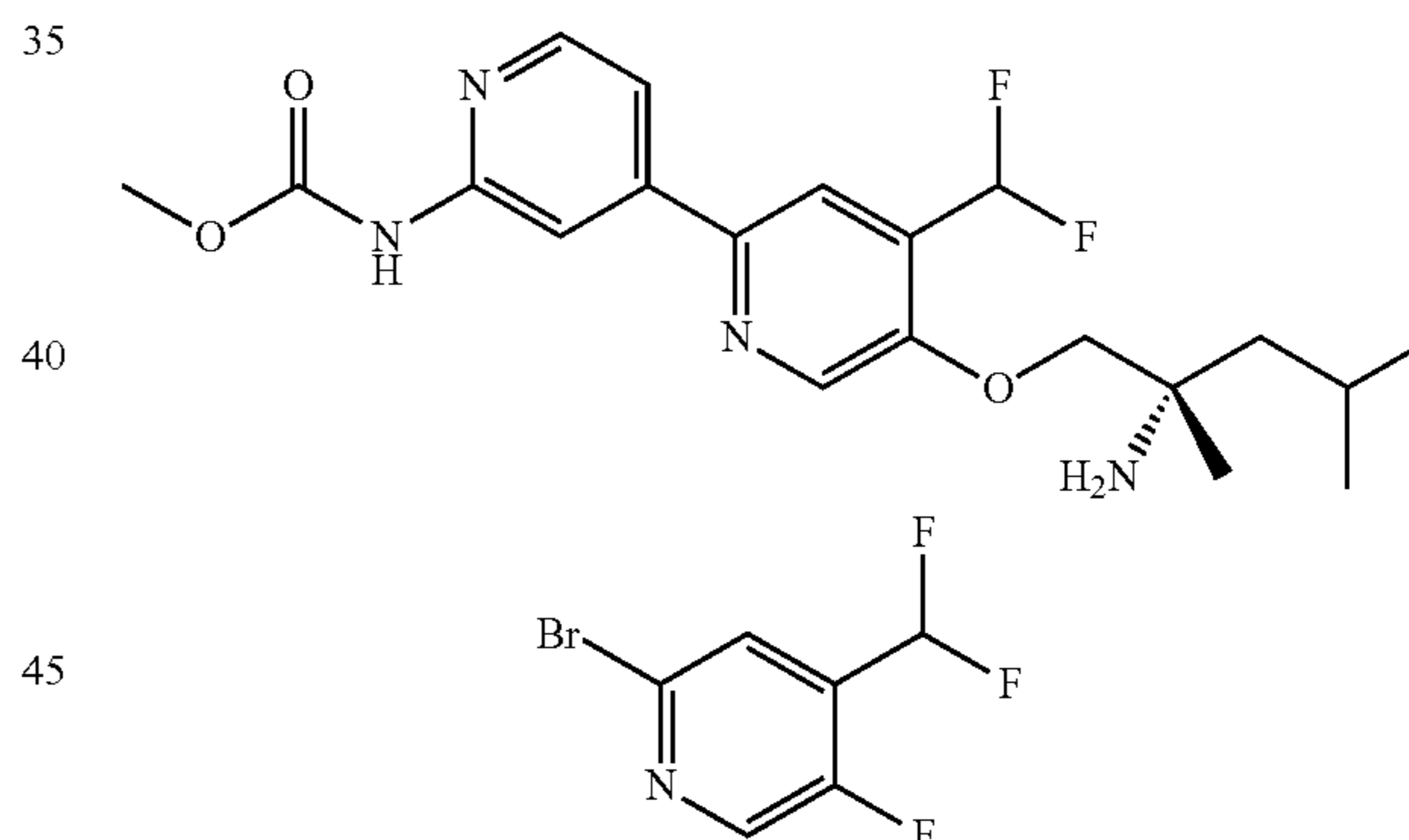
Part A: 2-bromo-4-(difluoromethyl)-5-fluoropyridine
