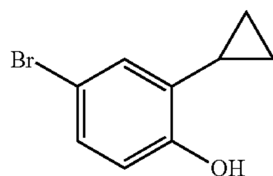
Part A: (S)-tert-butyl (1-(4-bromo-2-cyclopropylphenoxy)-2,4-dimethylpentan-2-yl)carbamate
