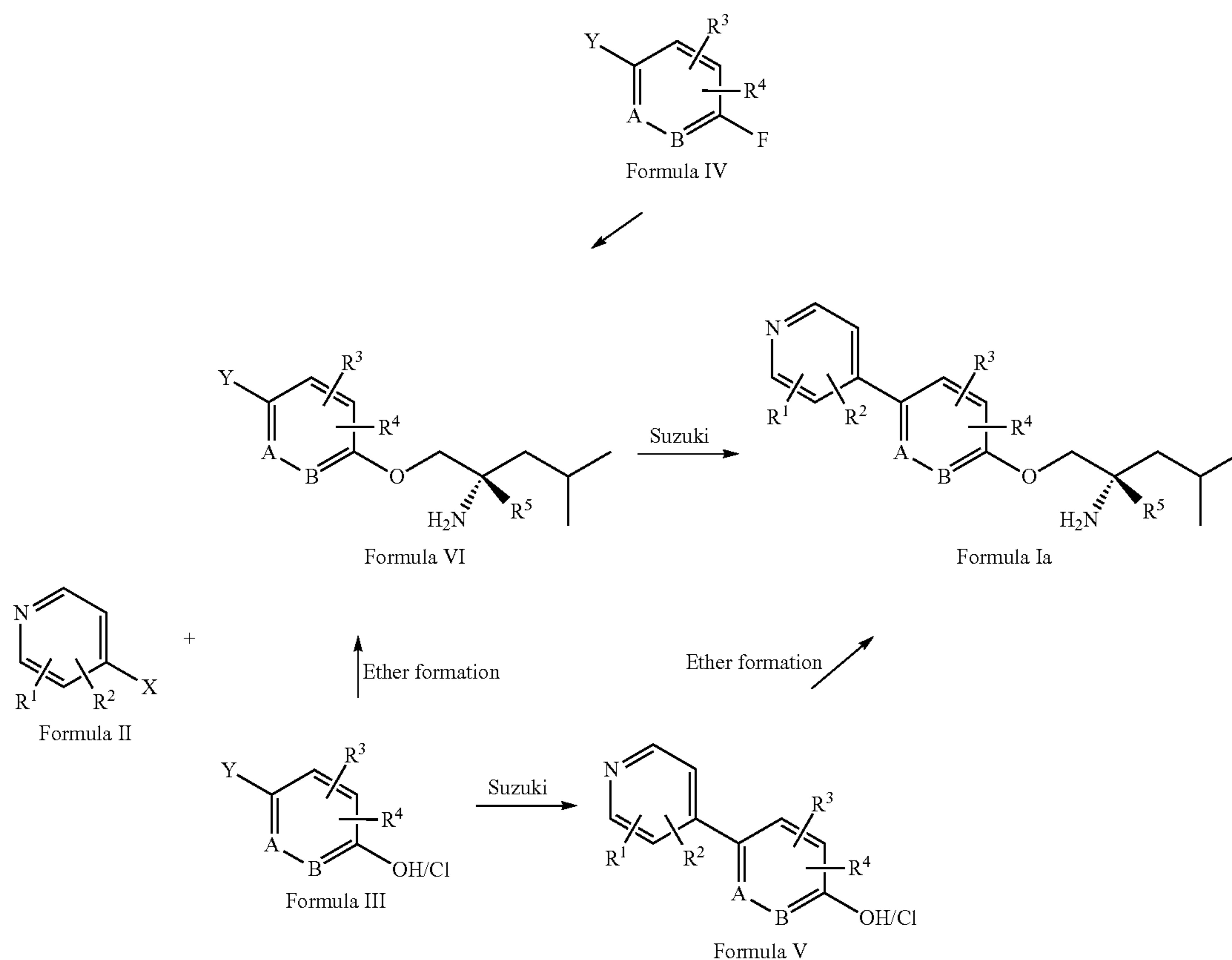
General Scheme I
