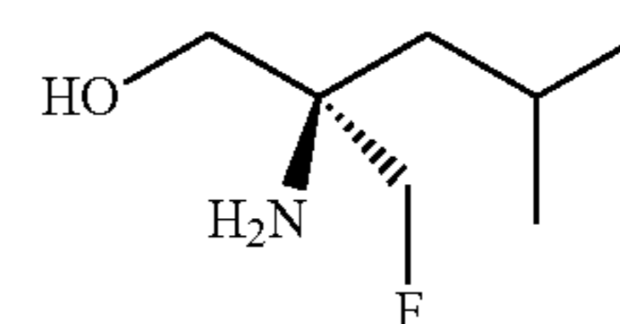
Part B: (R)-2-amino-2-(fluoromethyl)-4-methylpentan-1-ol
