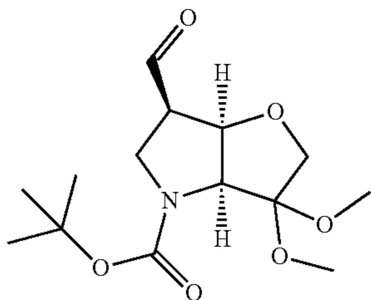
6-Formyl-3,3-dimethoxy-hexahydro-furo[3,2-b]pyrrole-4-carboxylic acid tert-butyl ester (1h)
