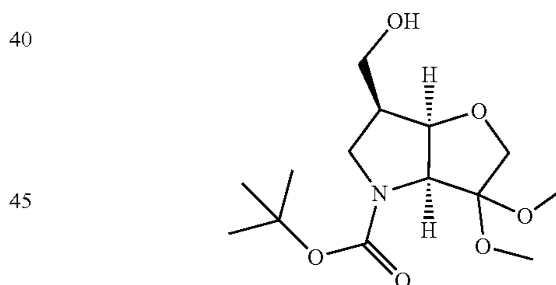
6-Hydroxymethyl-3,3-dimethoxy-hexahydro-furo[3,2-b]pyrrole-4-carboxylic acid tert-butyl ester (1q)
