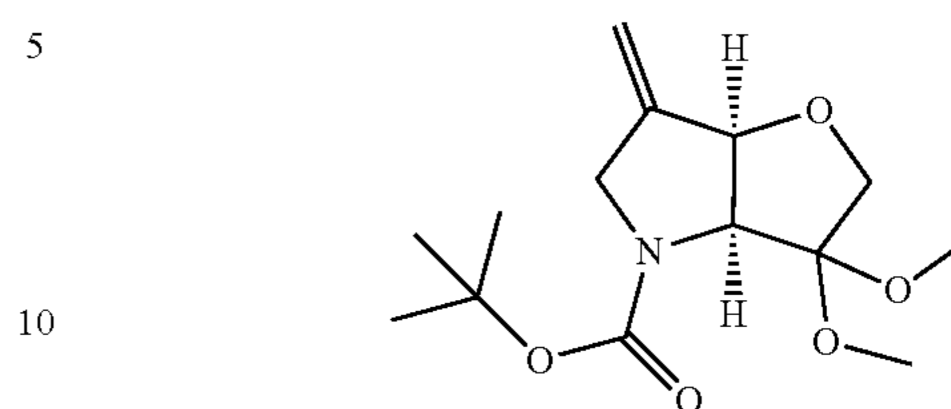
3,3-Dimethoxy-6-methylene-hexahydro-furo[3,2-b]pyrrole-4-carboxylic acid tert-butyl ester (1f)
