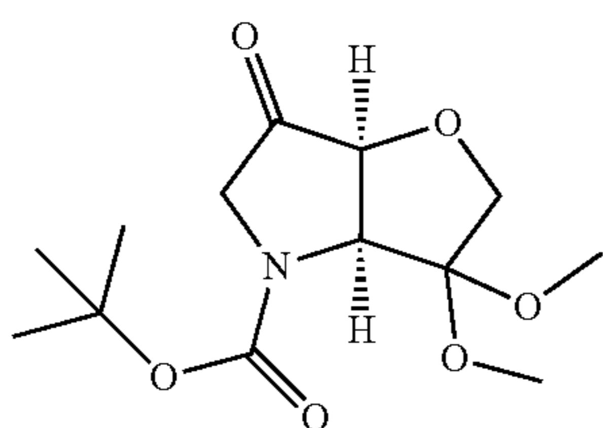
3,3-Dimethoxy-6-oxo-hexahydro-furo[3,2-b]pyrrole-4-carboxylic acid tert-butyl ester (1e)
