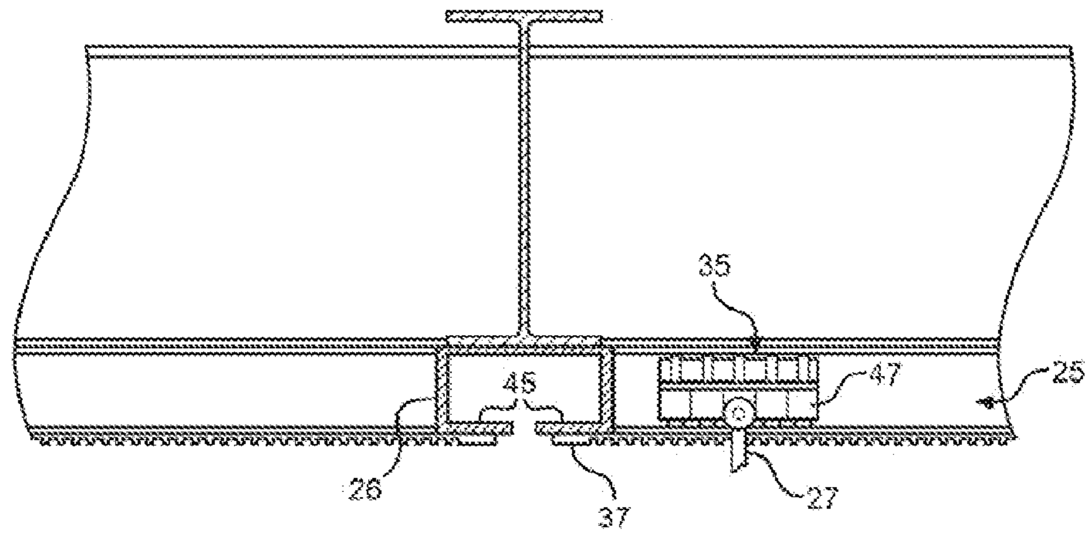
FIG. 4 PRIOR ART
