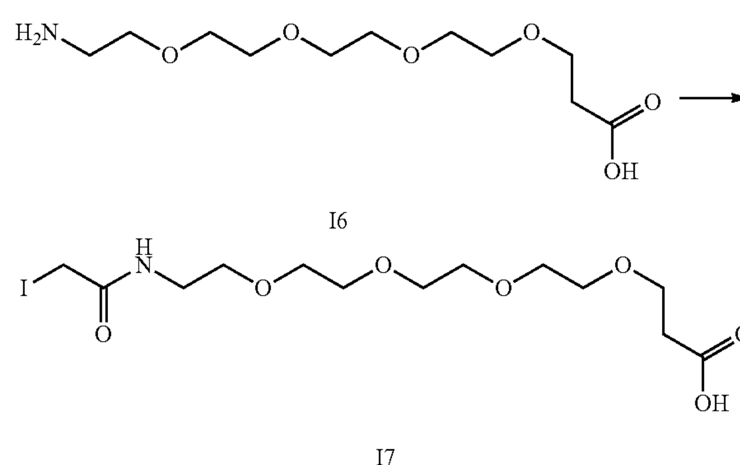
1-iodo-2-oxo-6,9,12,15-tetraoxa-3-aza-octadecan-18-oic acid (I7)
