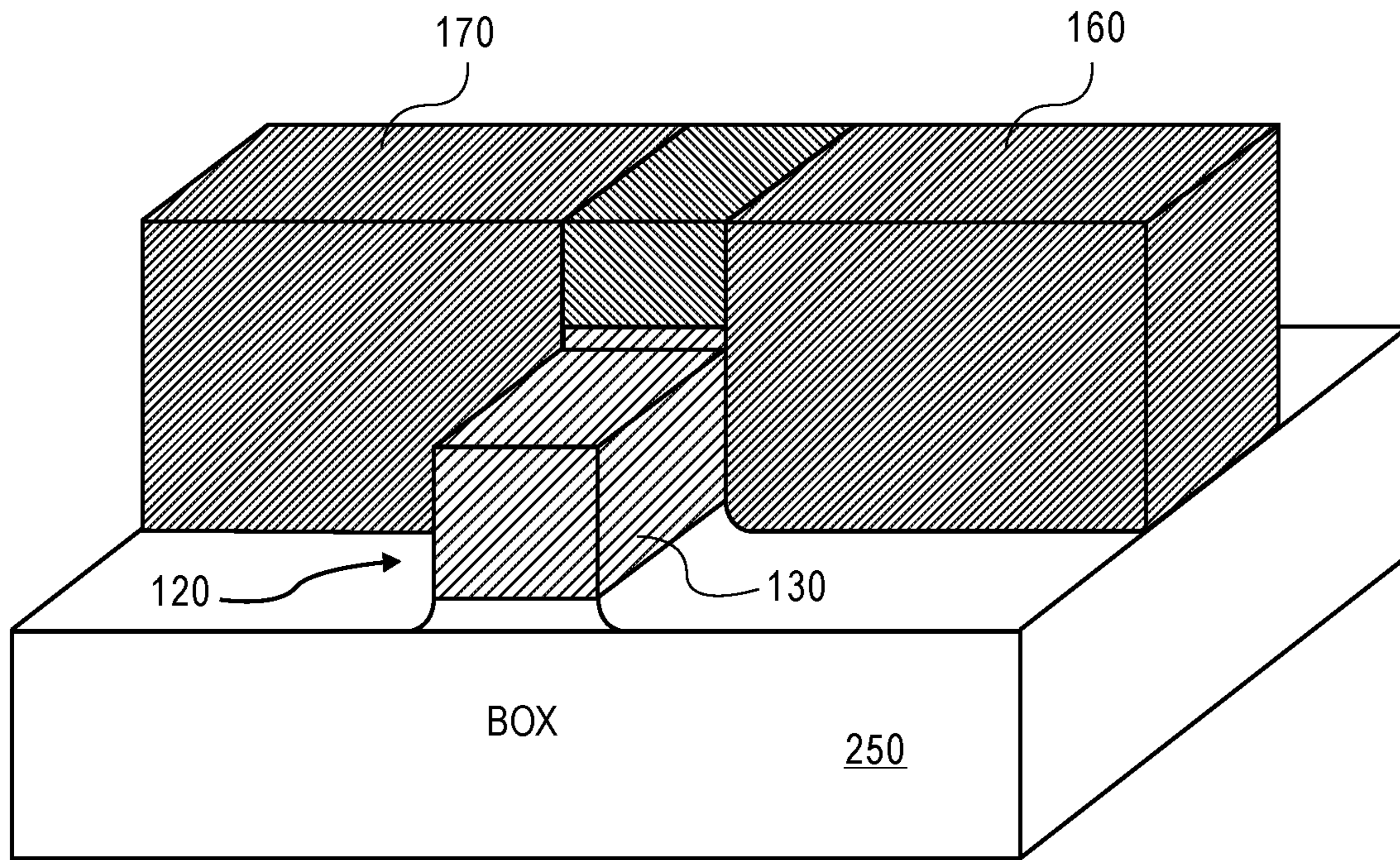
FIG. 2 (PRIOR ART)
