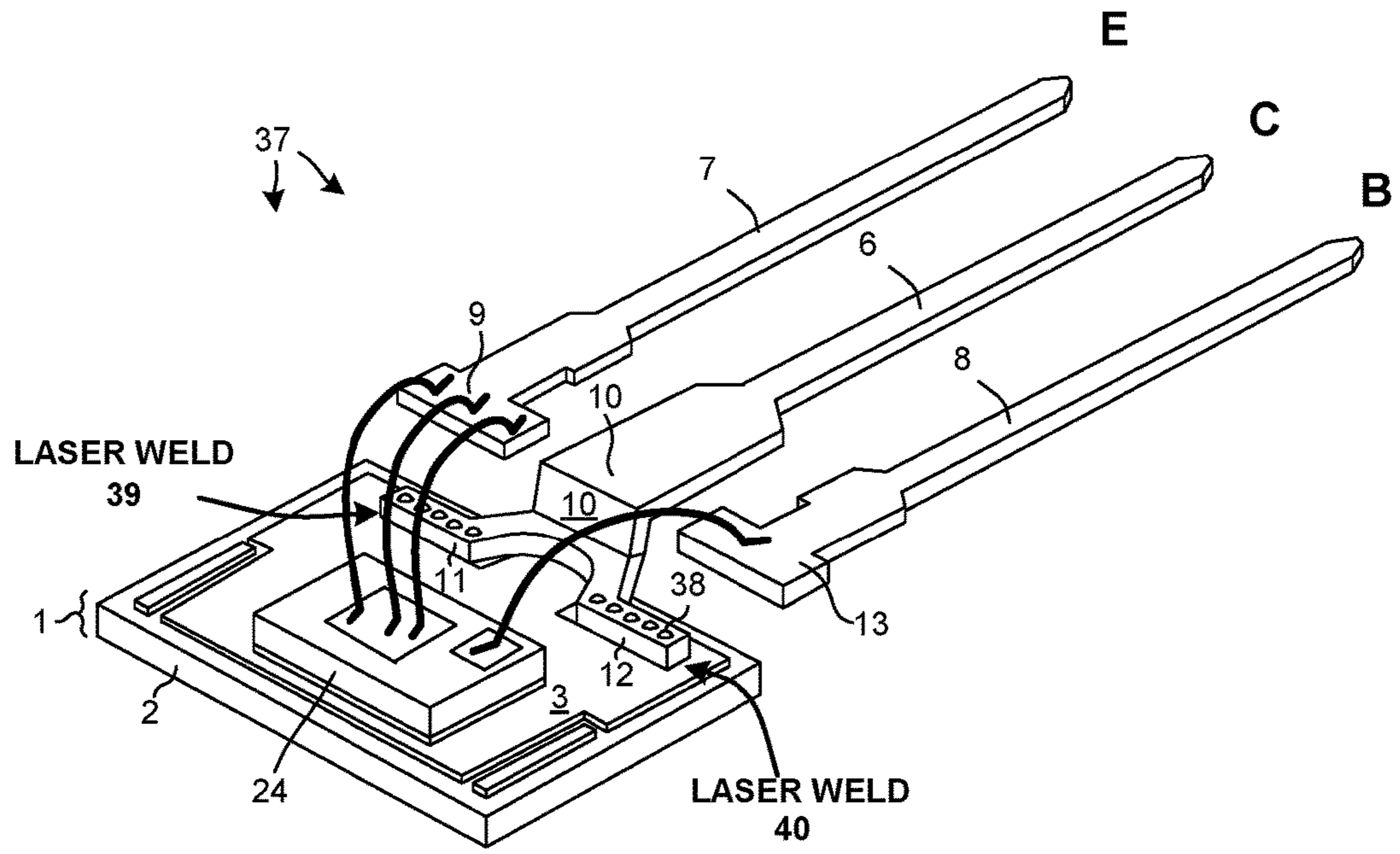
LASER WELD OF DBC SUBSTRATE TO LEADS FIG. 14
