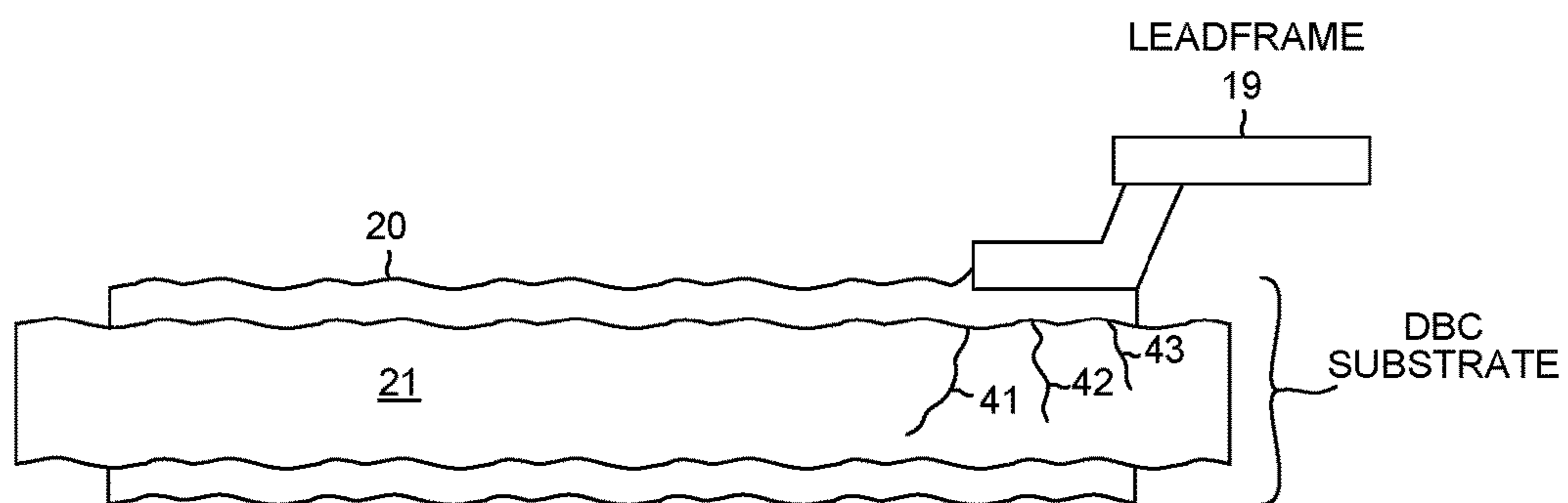
CRACKING OF ALUMINA FIG. 7
