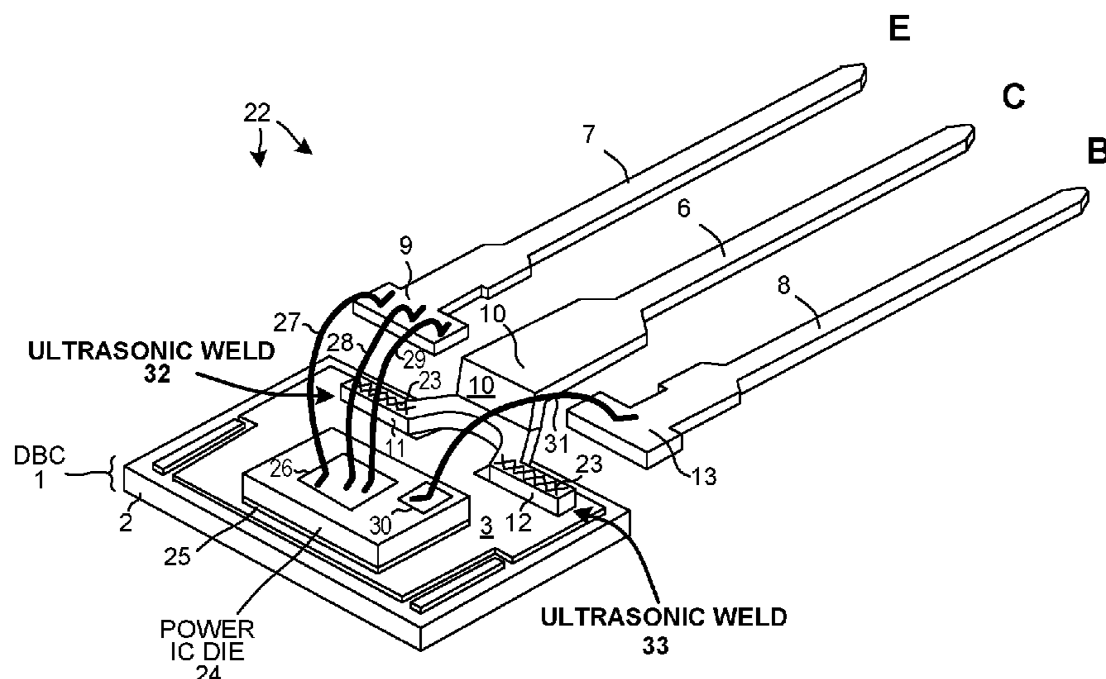
ULTRASONIC WELD OF DBC SUBSTRATE TO LEADS
