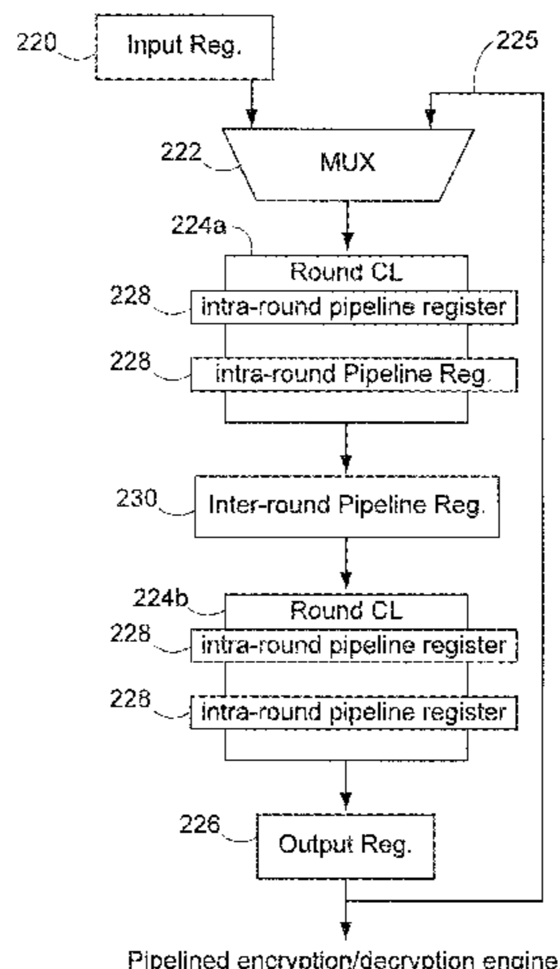
Pipelined encryption/decryption engine.
