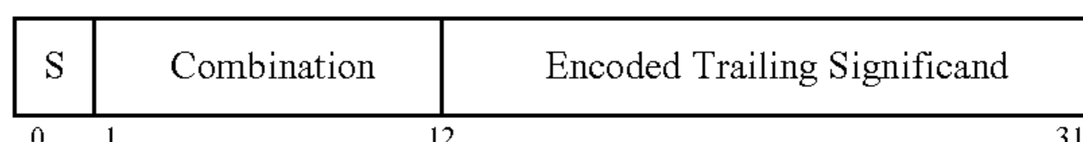
DFP Short Format
