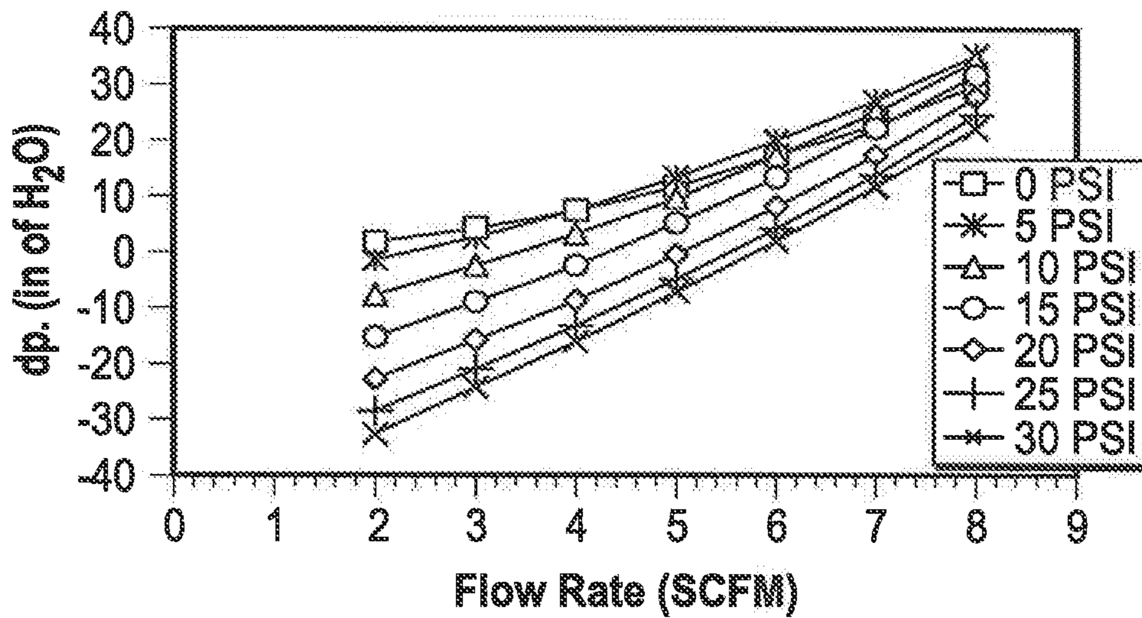
CFD Crankcase Pressure/dP 3mm Nozzle, 0.75 mm Motive Jet
