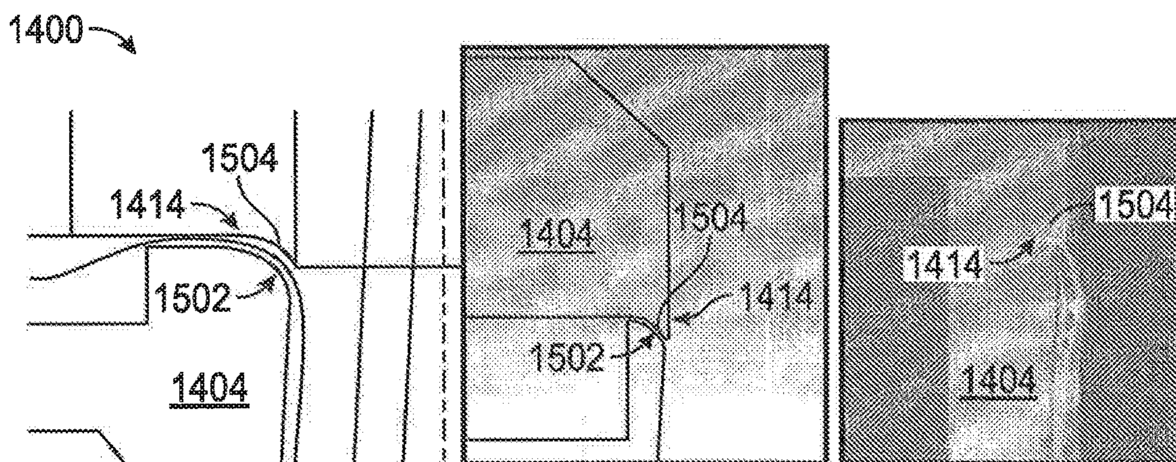
Close Up of the Narrow Gap and Rounded Edge Plus Lip that Creates Cylindrical Jet Which Adheres to the Mixing Bore Wall due to the Coanda Effect
