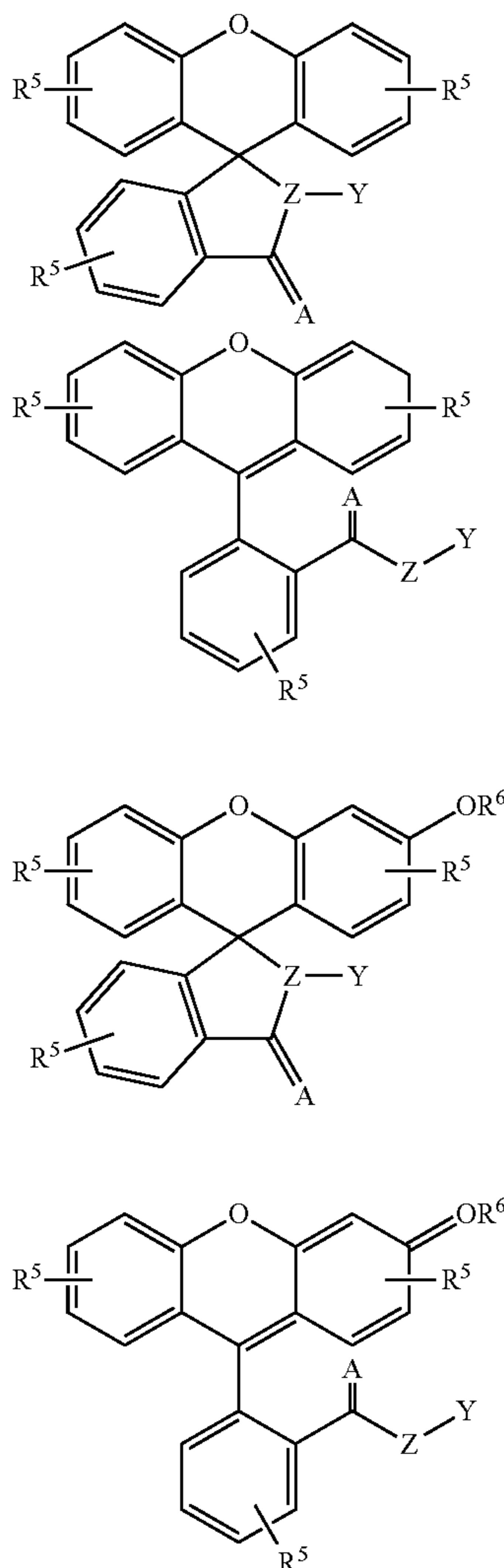
Scheme IV
