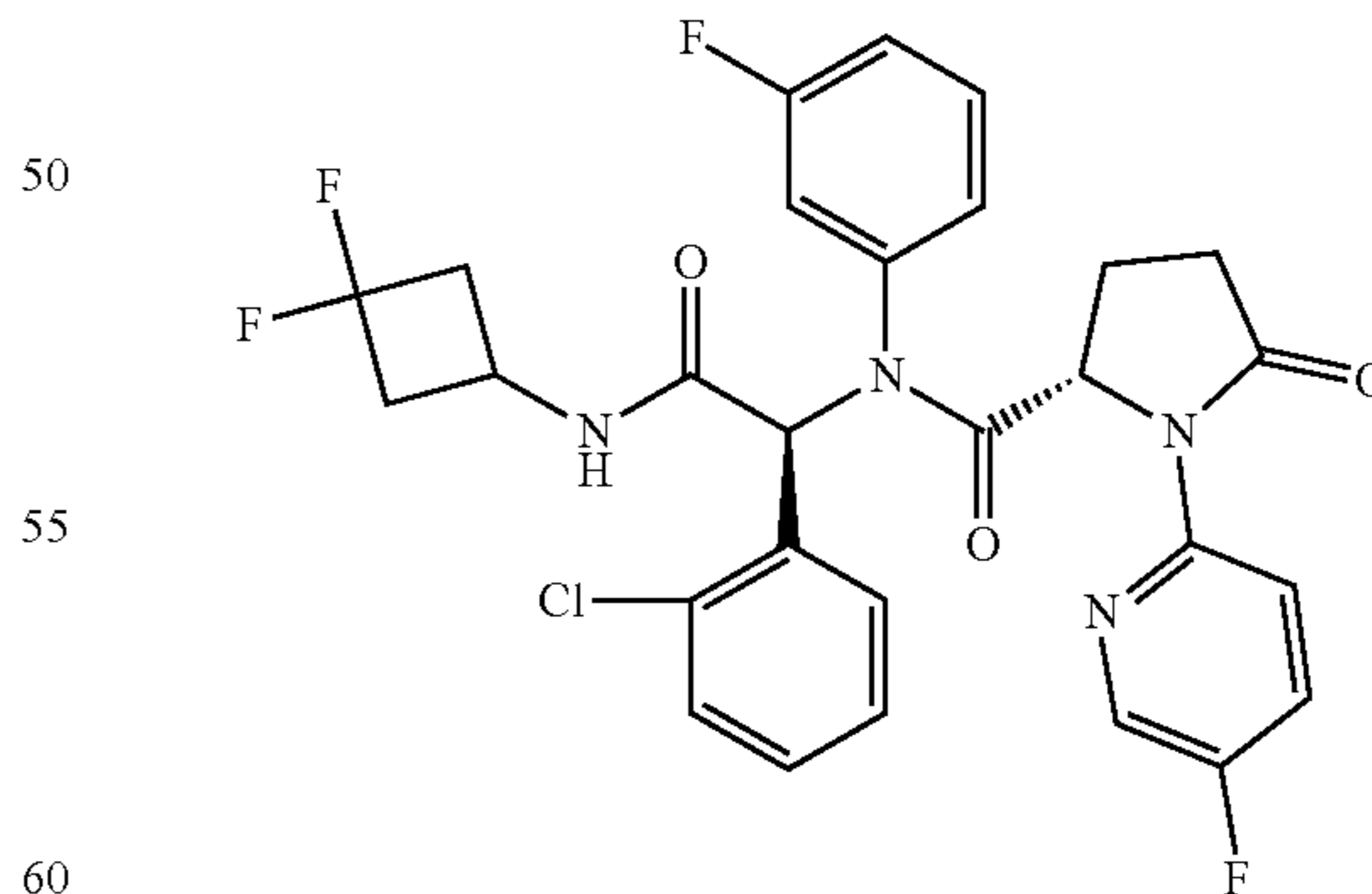
Compound 39
