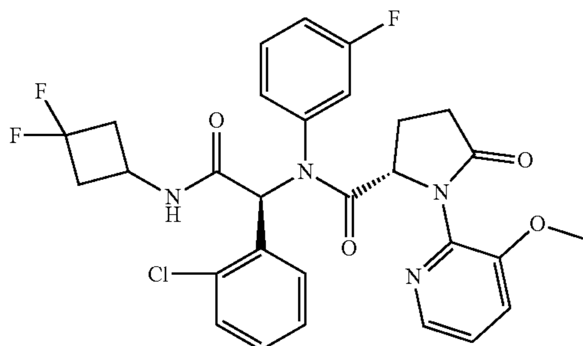
Compound 17
