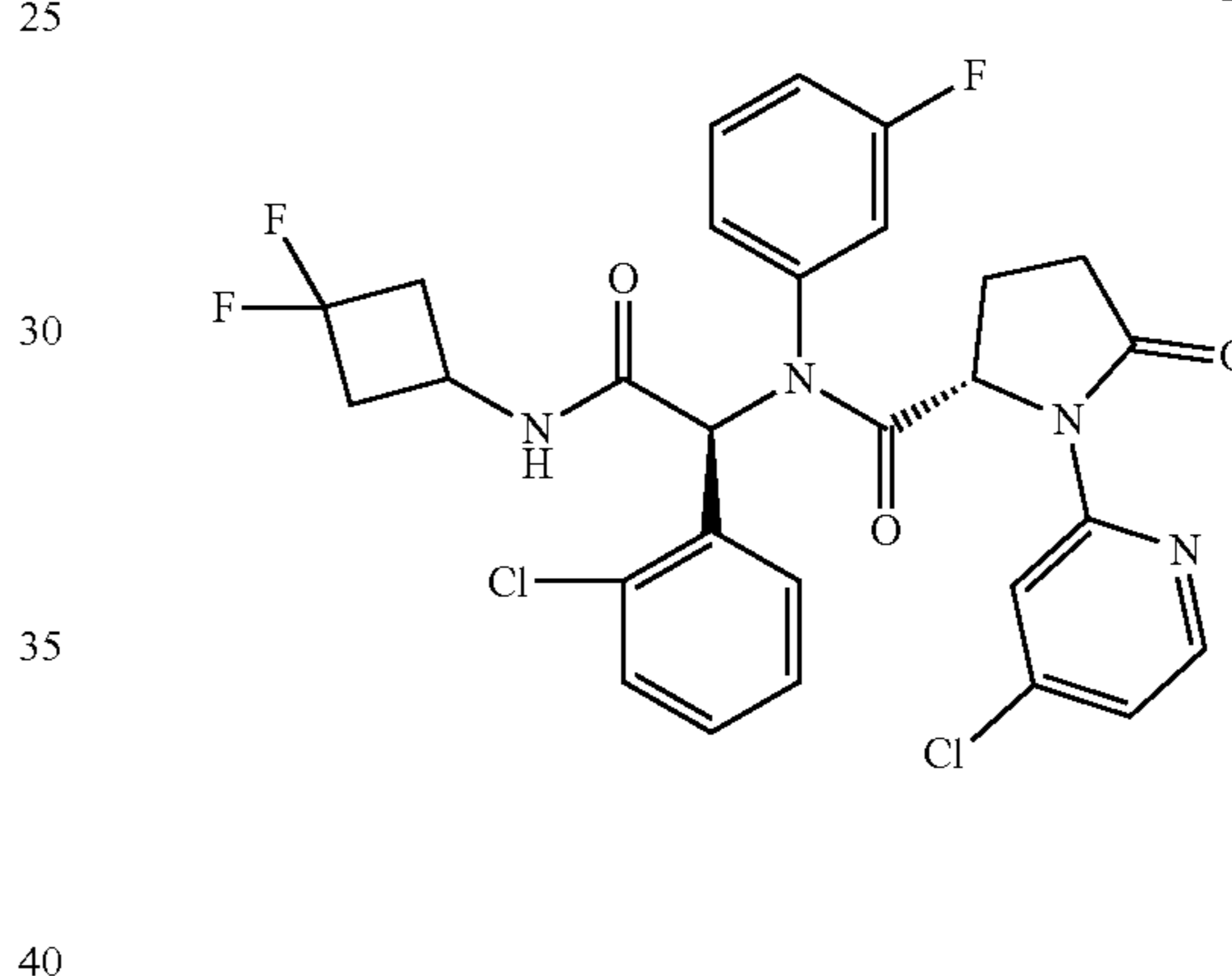
Compound 34
