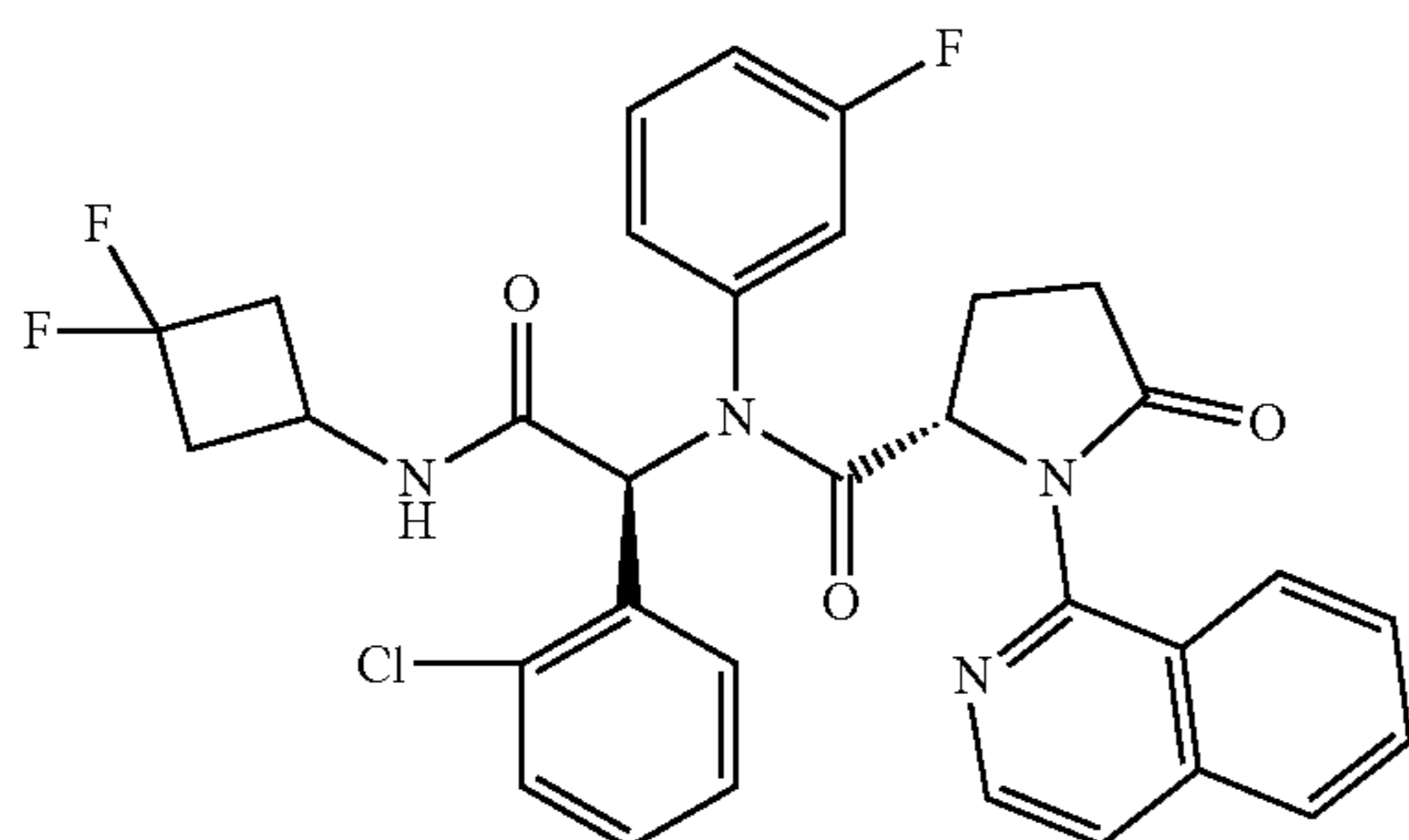
Compound 16
