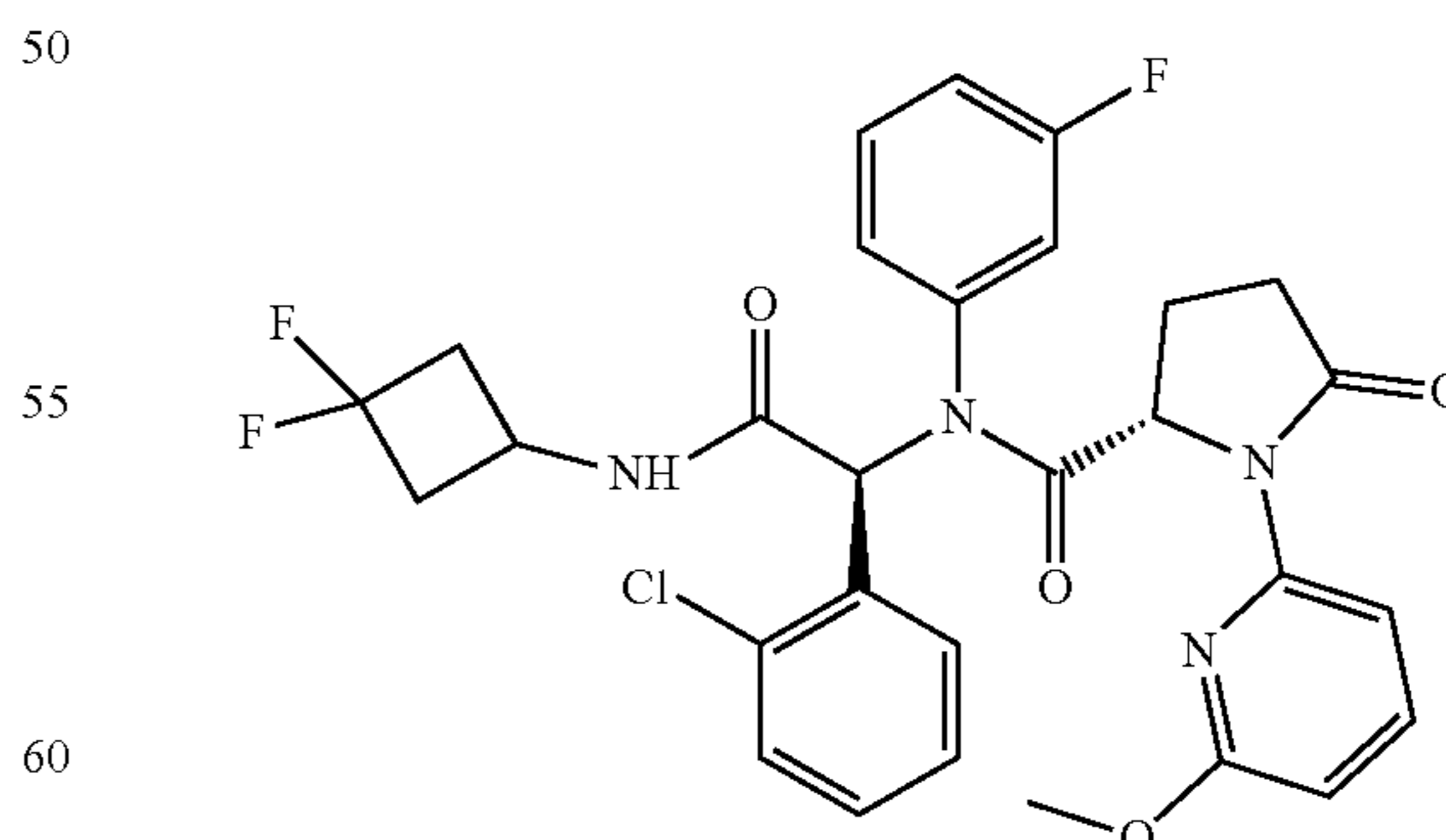
Compound 41
