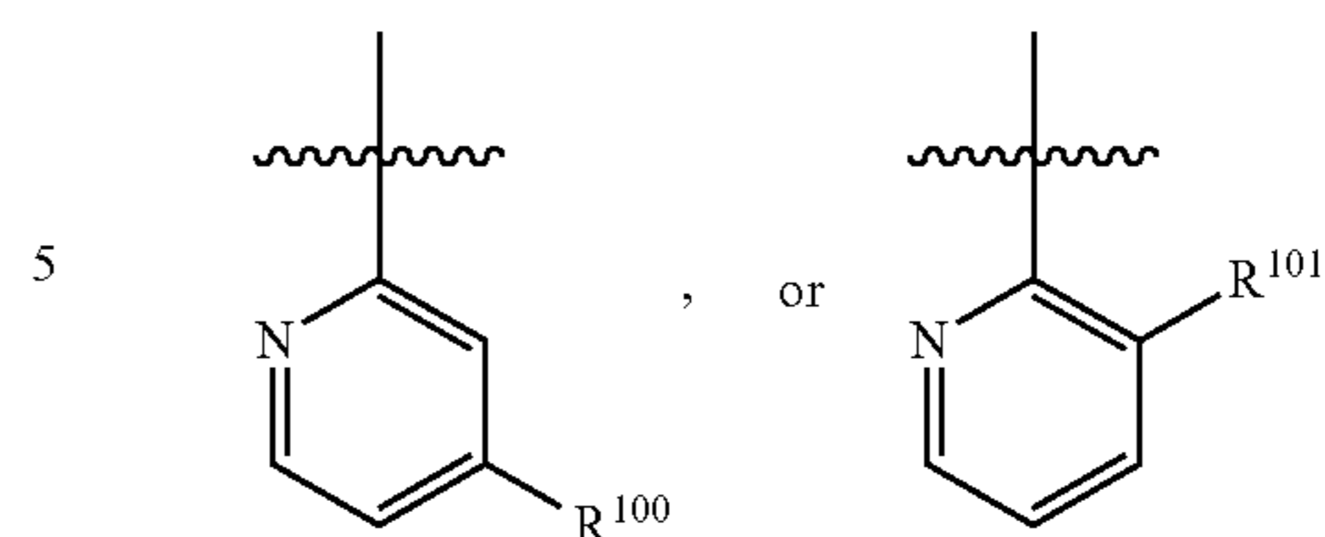
formula II-b-1
