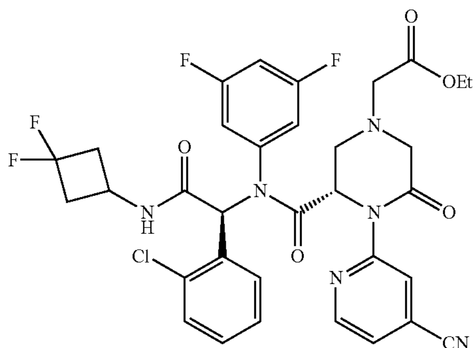
Compound 104
