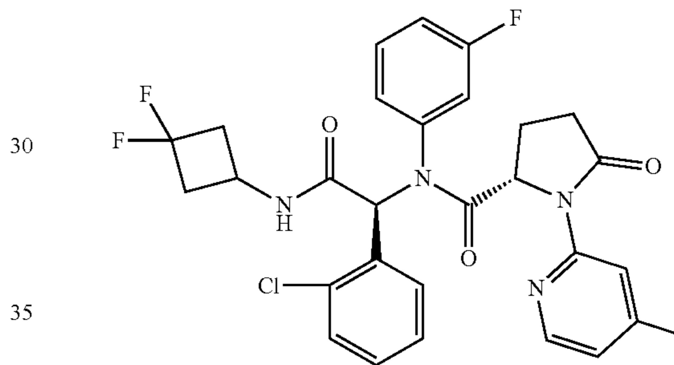
Compound 27
