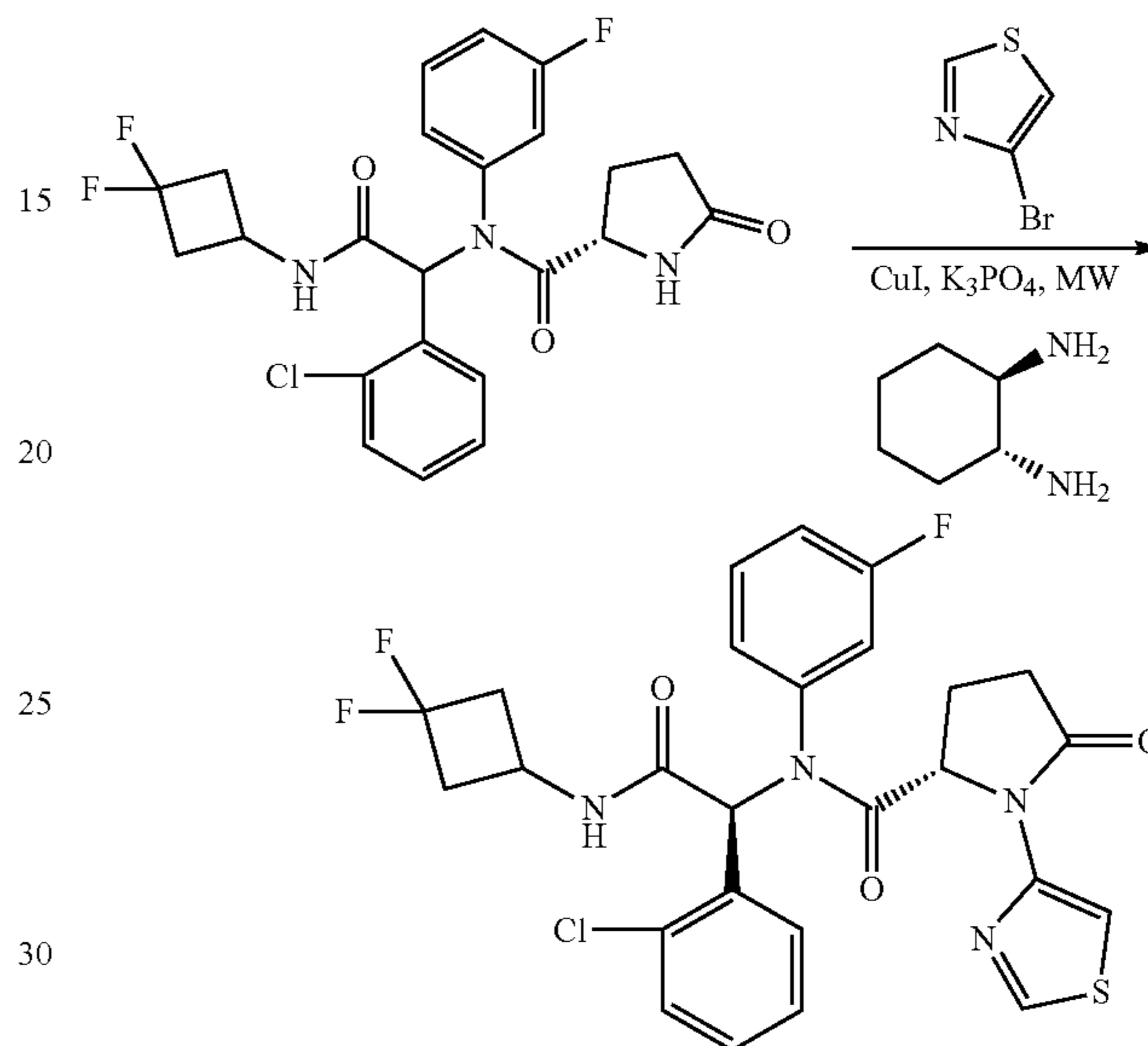
Compound 43
